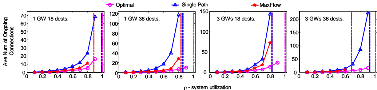
Figure 8.9: Average number of ongoing connections when subjected to Poisson connection arrivals and exponentially distributed connection size. Utilization of 1 corresponds to the maximum capacity provided by optimal routing
