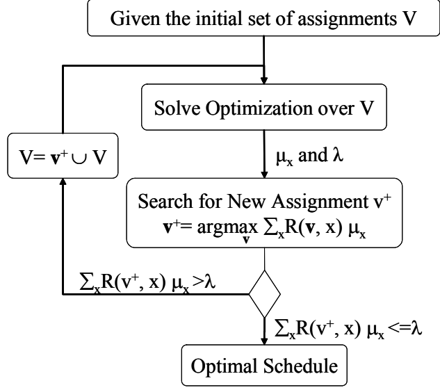
Figure 3.2: Algorithm for optimal scheduling
