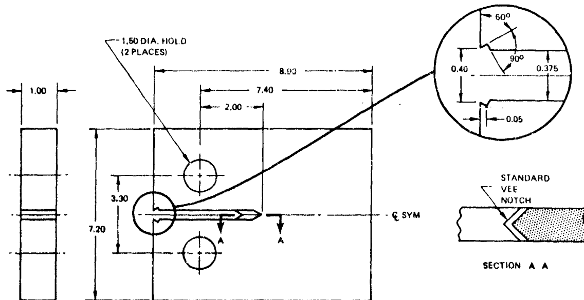
Figure B12: NAR Compact Tension Specimen Configuration
