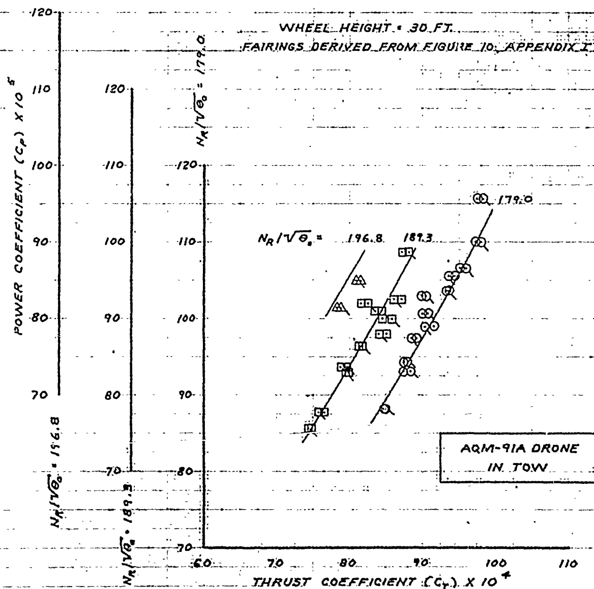
FIGURE 4. NONDIMENSIONAL HOVER PERFORMANCE
