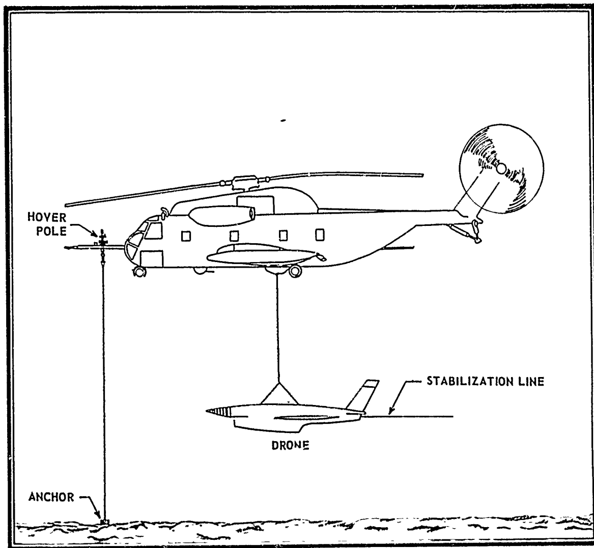
Figure 2 Hover Test Technique with Drone In Tow
