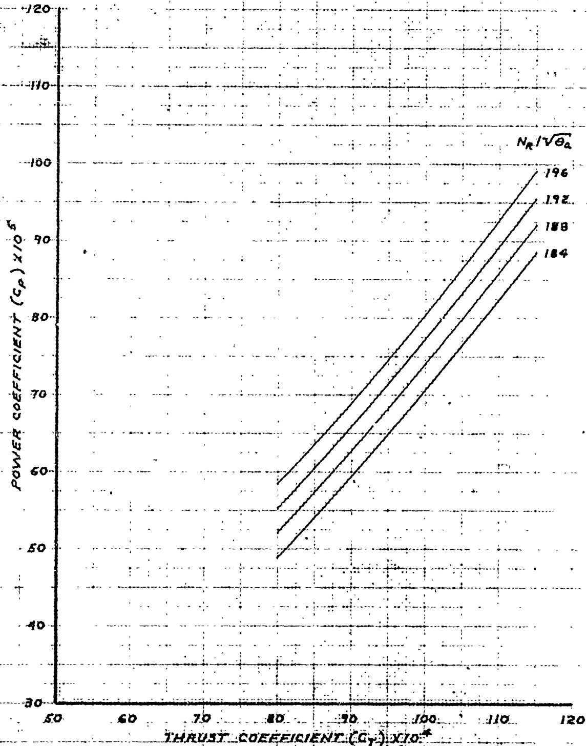
FIGURE 68. LEVEL FLIGHT PERFORMANCE SUMMARY (AQM-34R)
