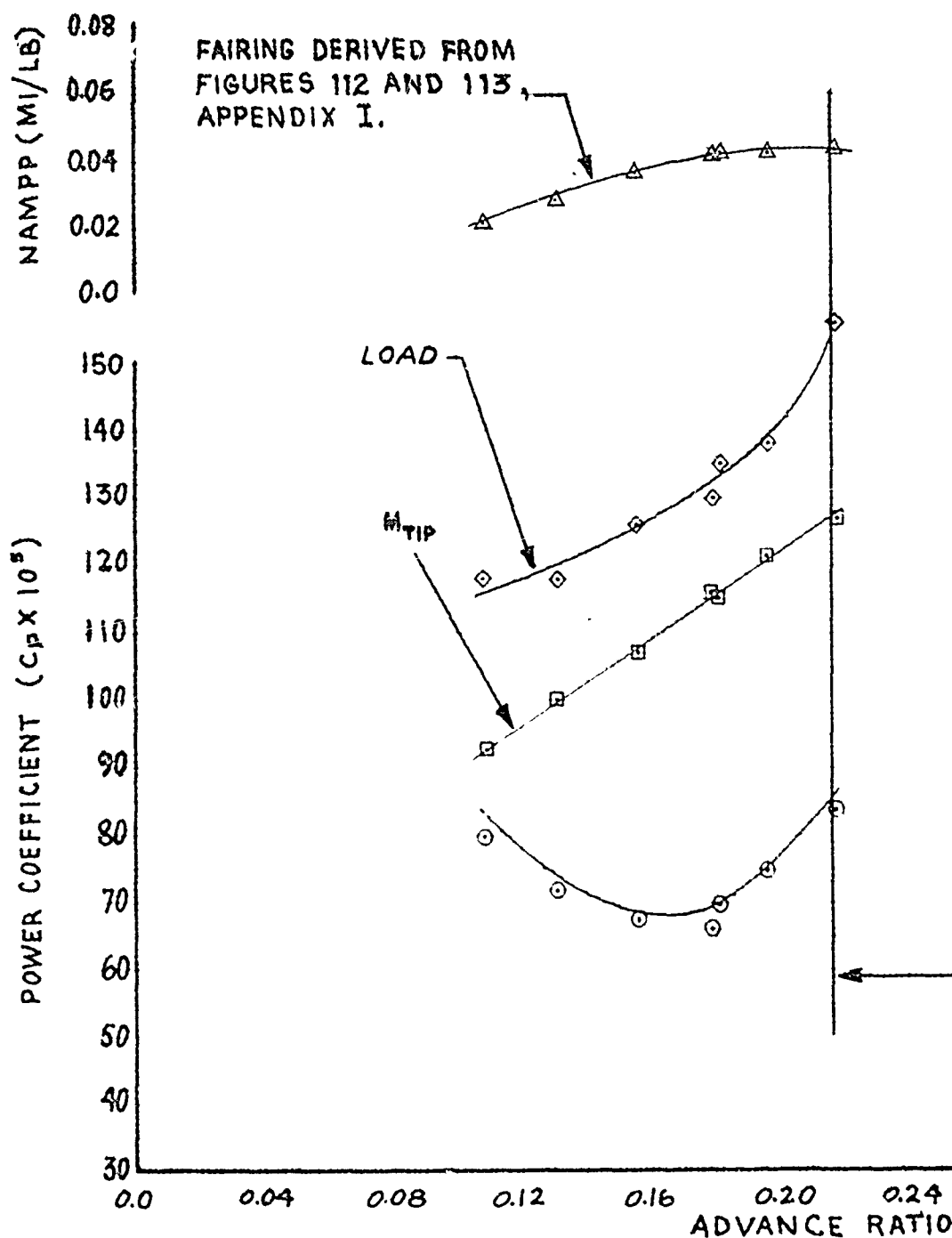
FIGURE 102 NONDIMENSIONAL LEVEL
