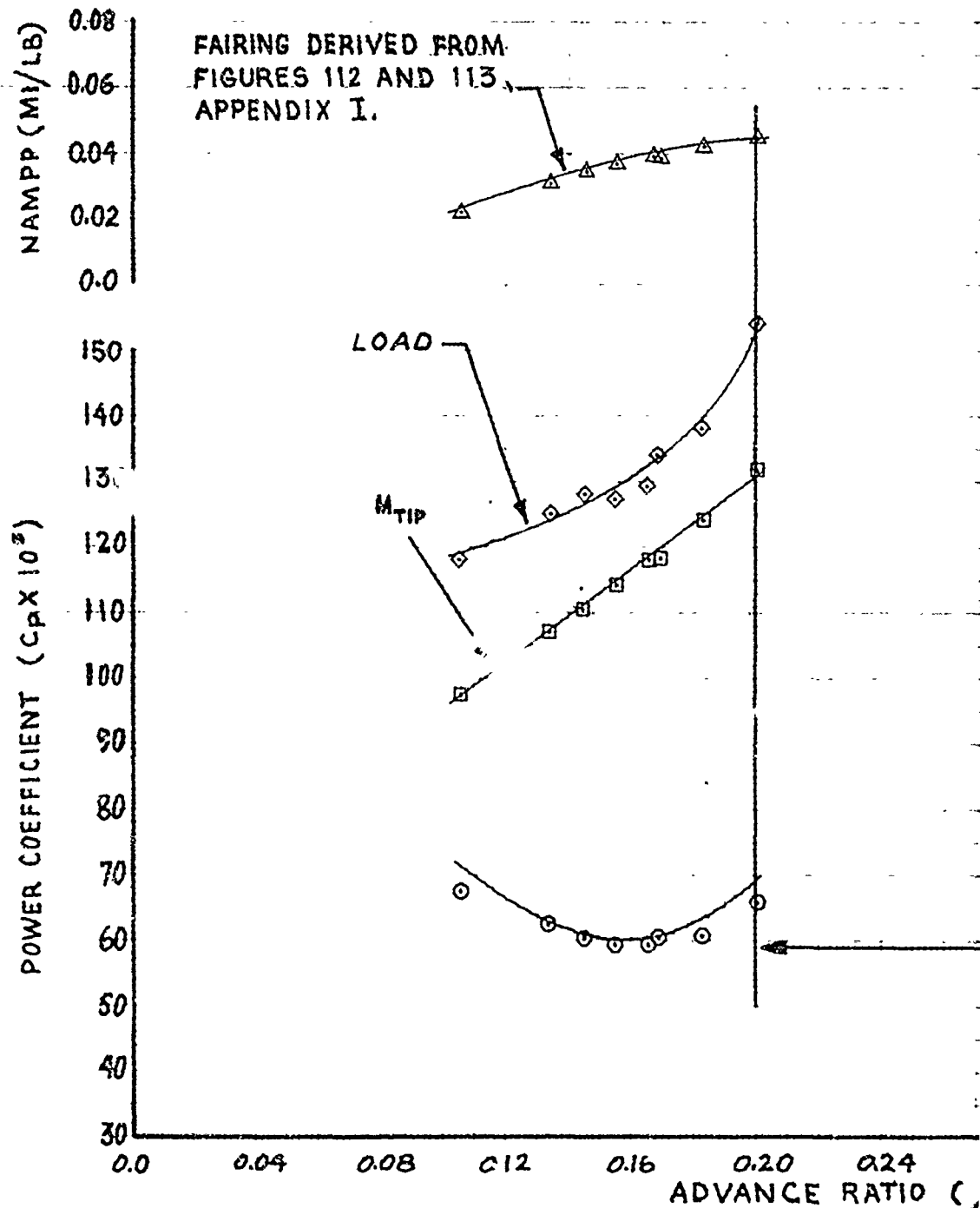
FIGURE 99 NONDIMENSIONAL LEVEL FLIG
