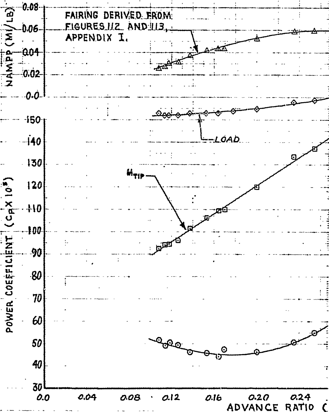
FIGURE 53. NONDIMENSIONAL LEVEL FLIGHT
