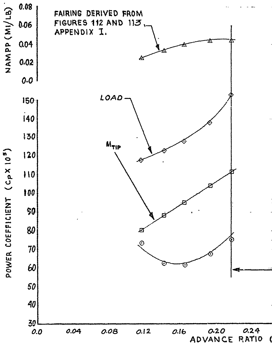
FIGURE 100 NONDIMENSIONAL LEVEL FL
