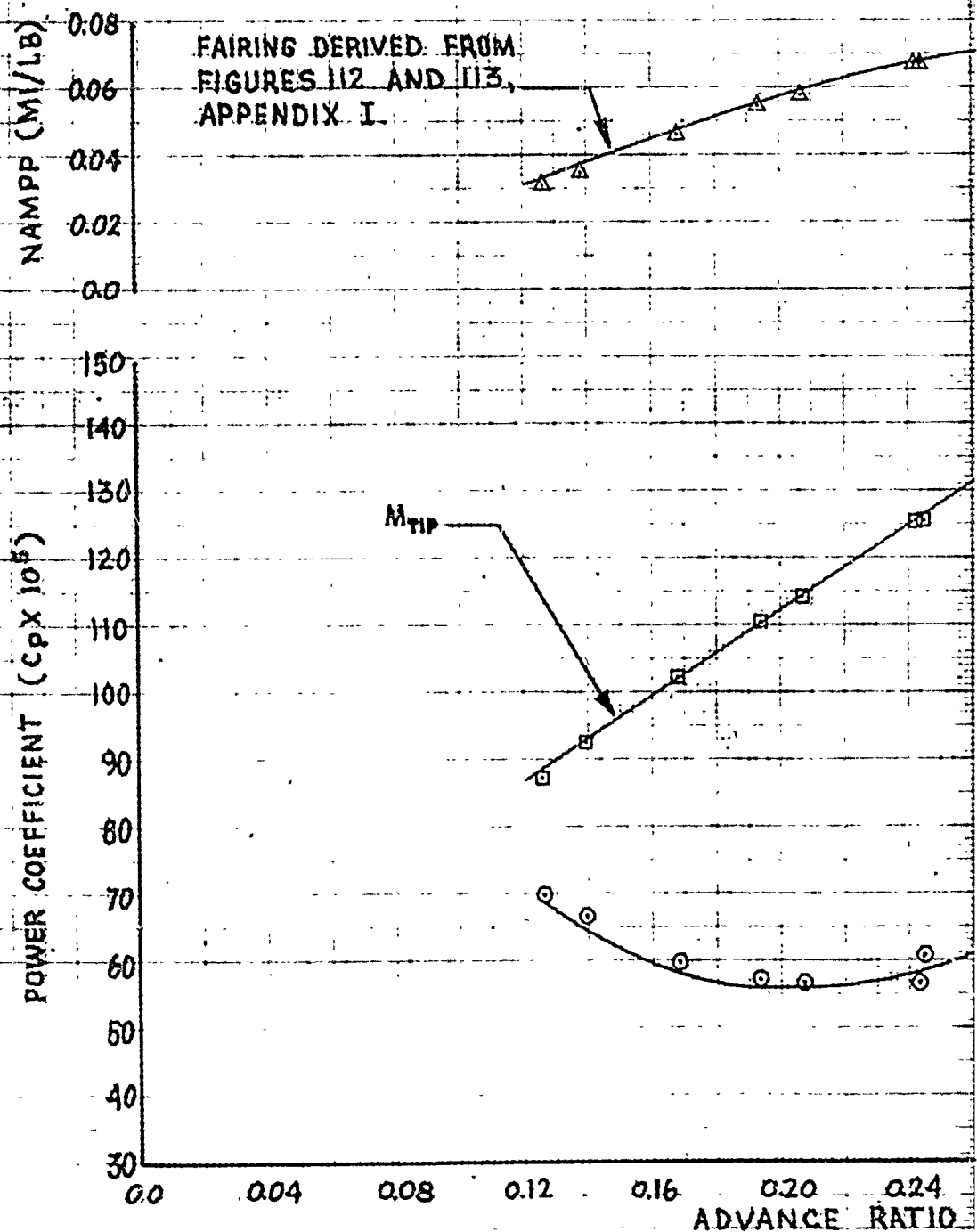
FIGURE 34 NONDIMENSIONAL LEVEL F
