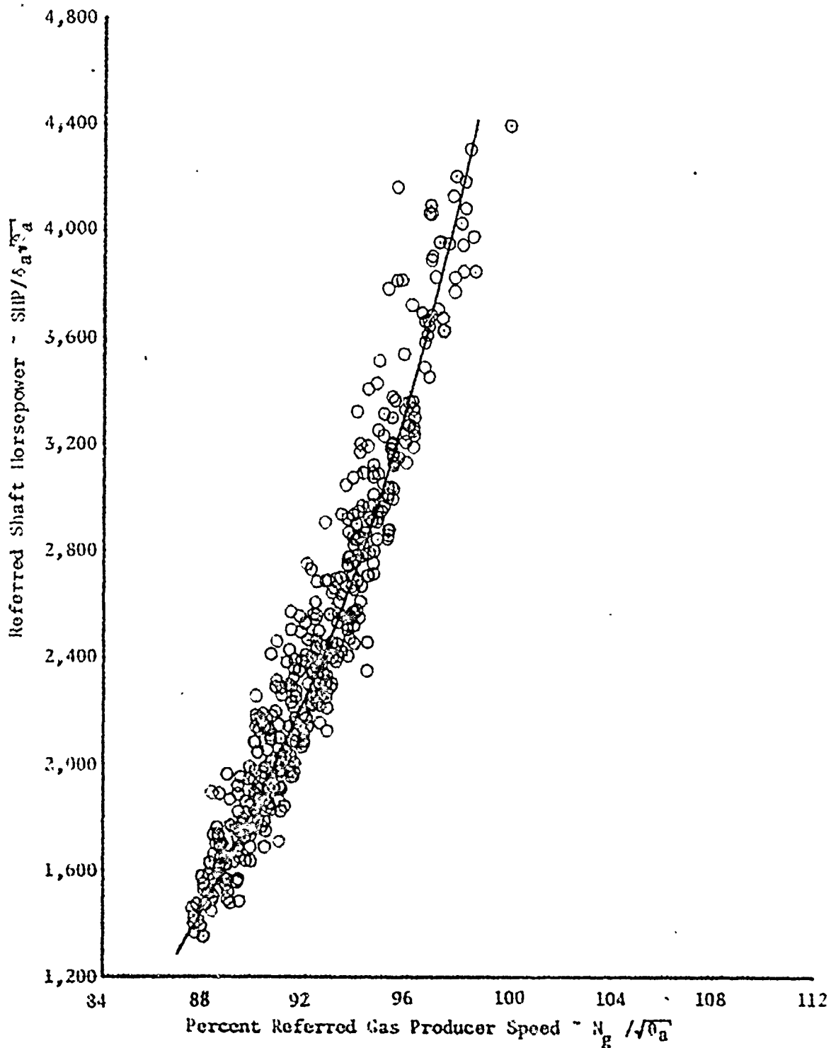
Figure 110. Engine Characteristics
