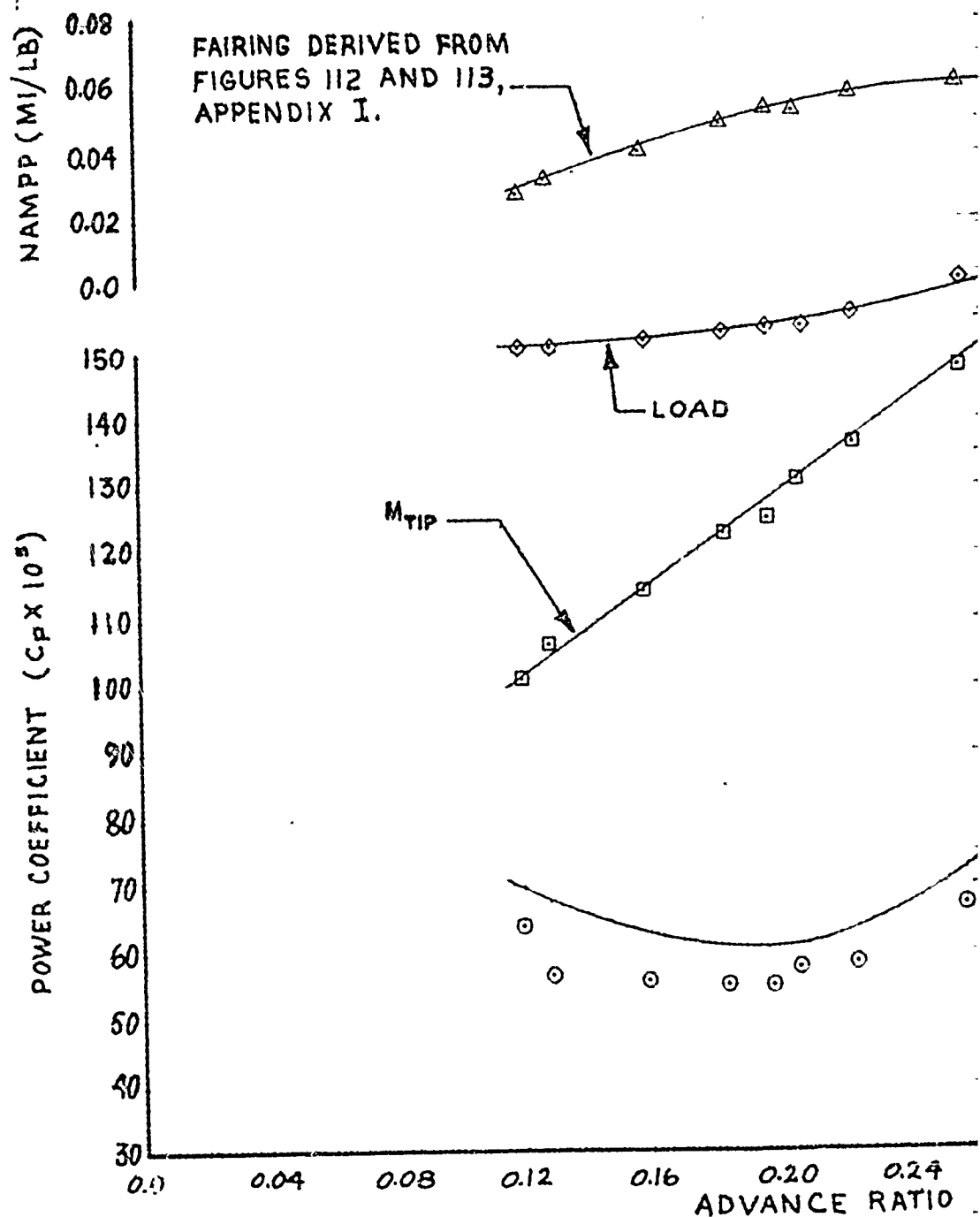
FIGURE 78. NONDIMENSIONAL LEVEL FLIGHT
