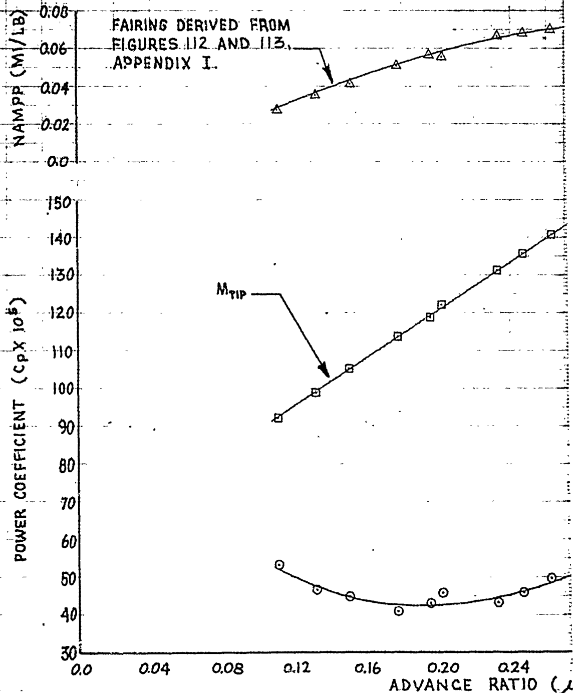
FIGURE 27 NONDIMENSIONAL LEVEL FLIGHT
