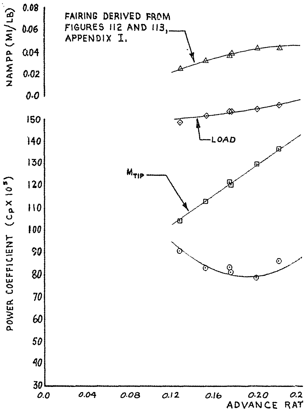
FIGURE 82. NONDIMENSIONAL LEVEL
