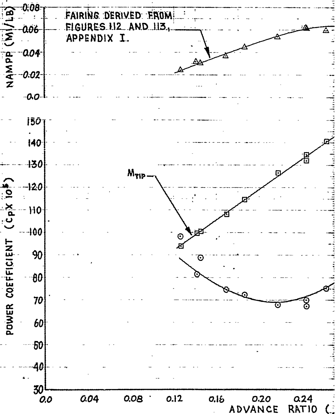
FIGURE 39 NONDIMENSIONAL LEVEL FLIGHT
