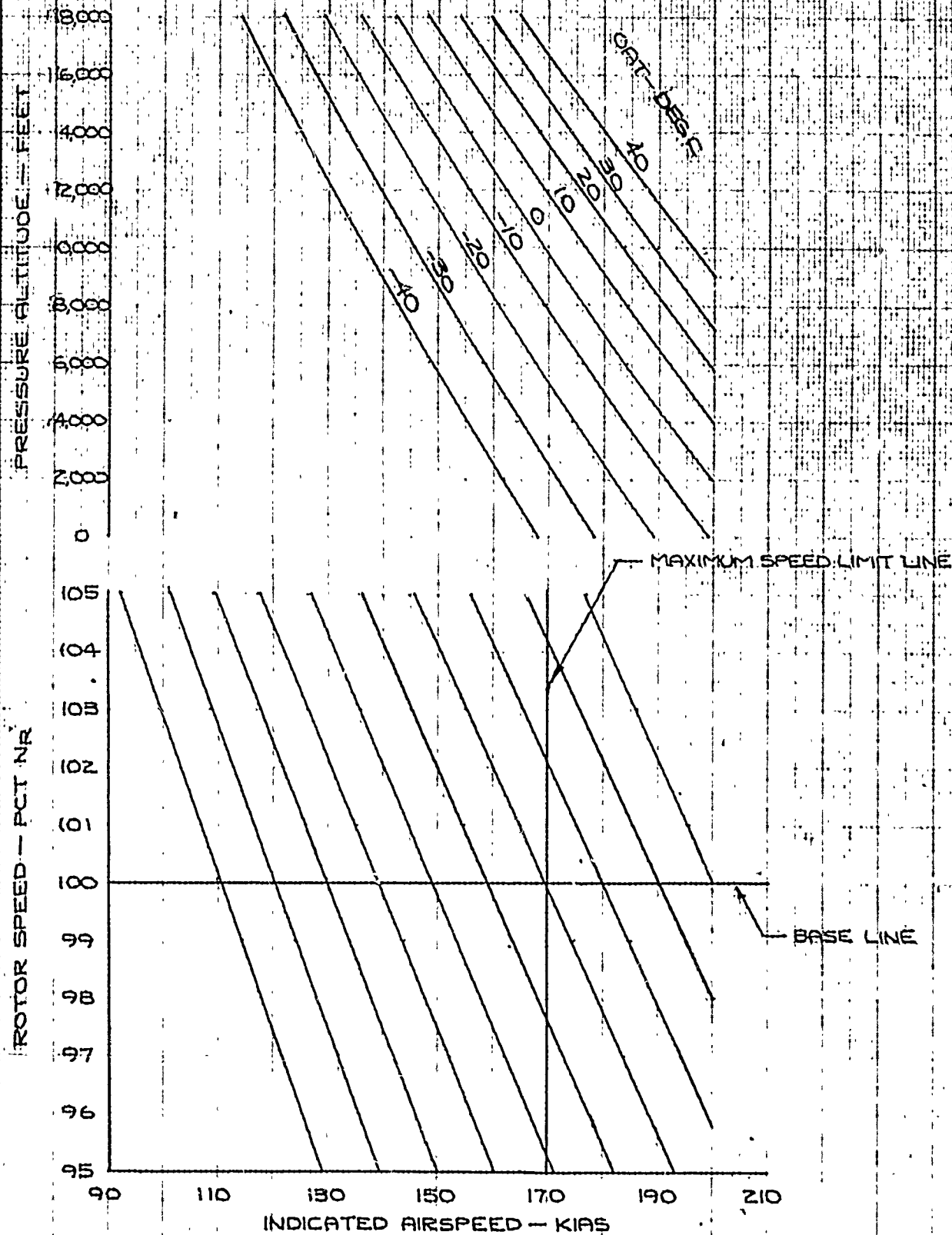
FIGURE 2. MAXIMUM AIRSPEED AS LIMITED BY MARS
