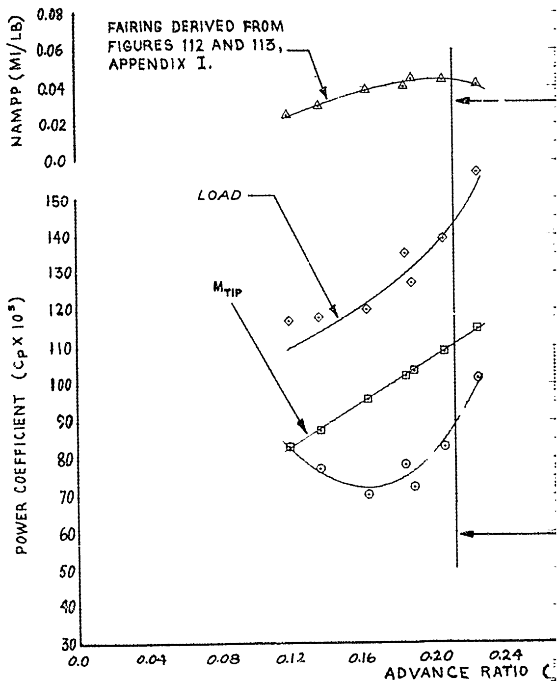
FIGURE 104 NONDIMENSIONAL LEVEL FLIGHT
