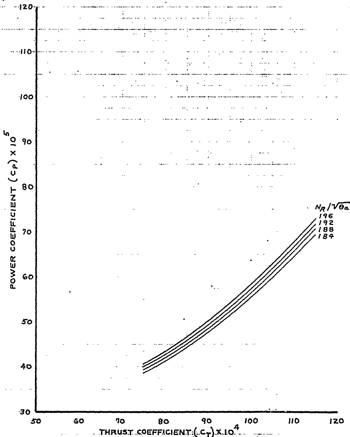
FIGURE 20. LEVEL FLIGHT PERFORMANCE SUMMARY (CLEAN)
