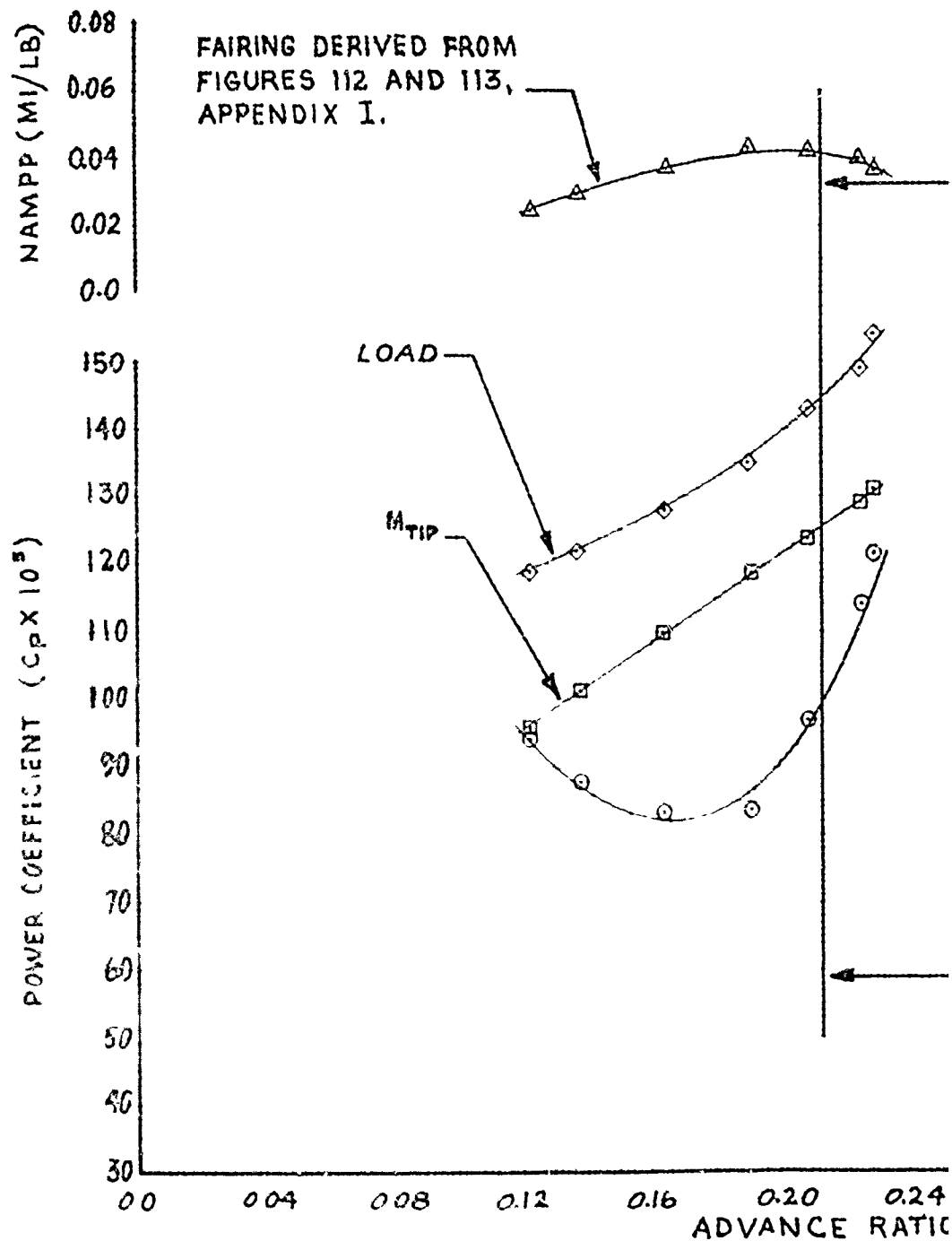
FIGURE 106 NONDIMENSIONAL LEVEL.
