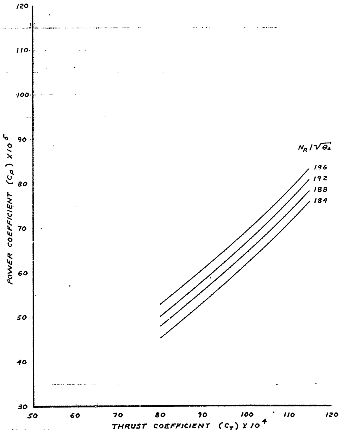
FIGURE 70. LEVEL FLIGHT PERFORMANCE SUMMARY (AQM-34R)
