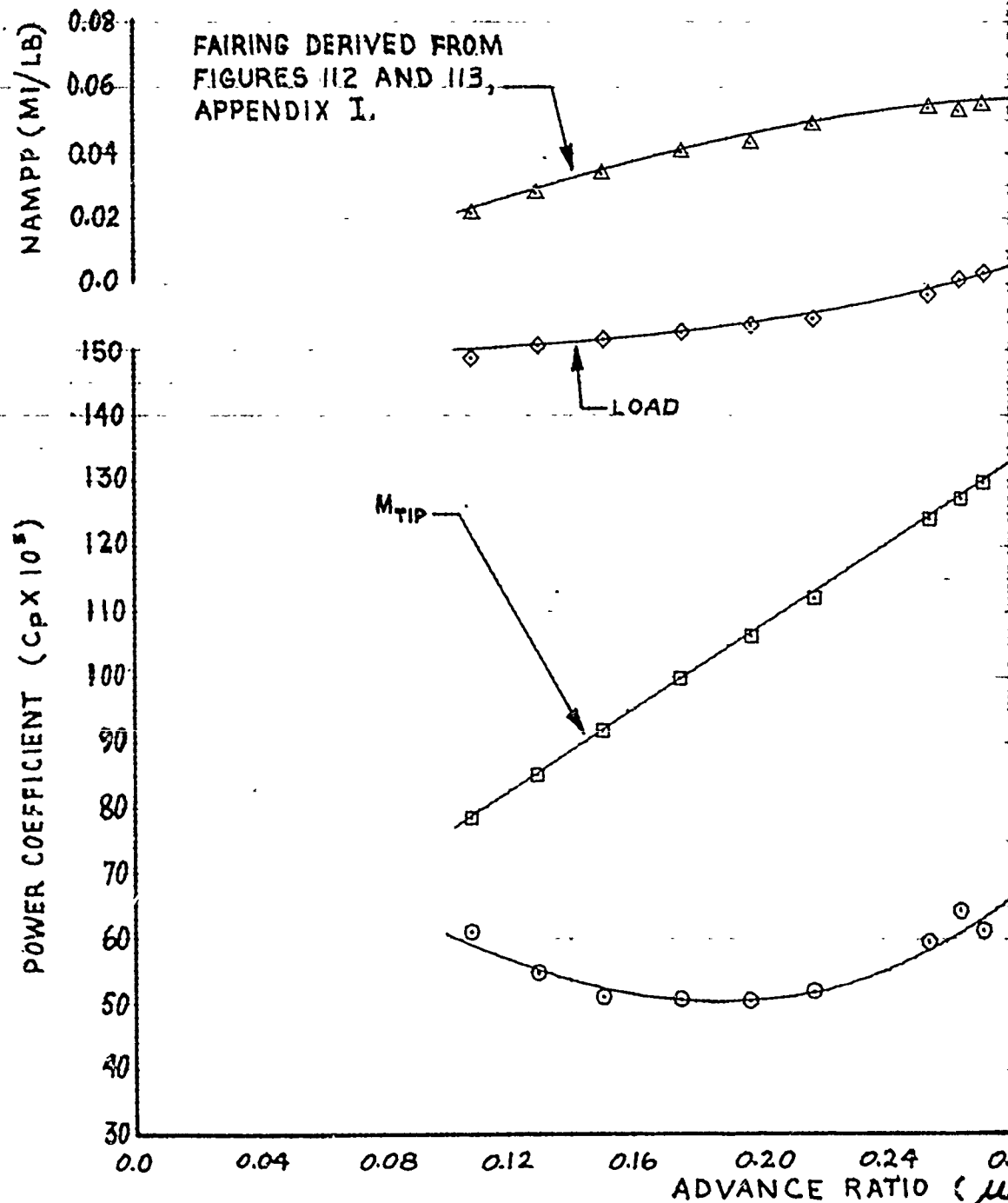
FIGURE 75. NONDIMENSIONAL LEVEL FLIGHT
