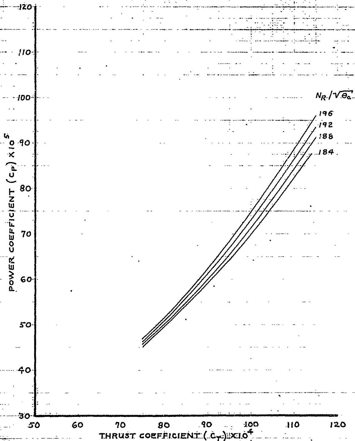
FIGURE 18. LEVEL FLIGHT PERFORMANCE SUMMARY (CLEAN)
