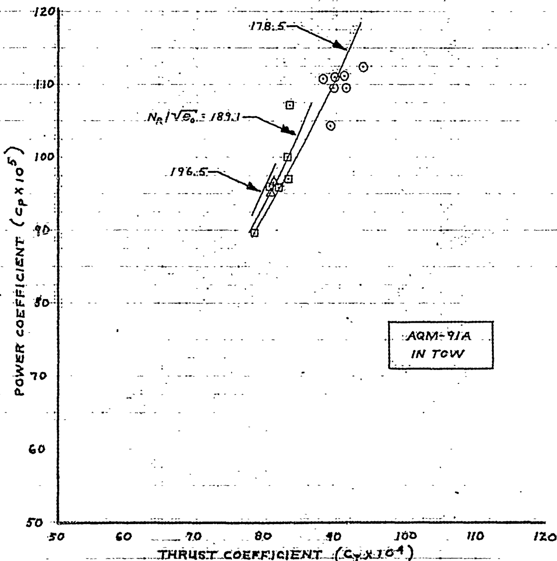
FIGURE 12. NONDIMENSIONAL HOVERING PERFORMANCE (AQM-91A)
