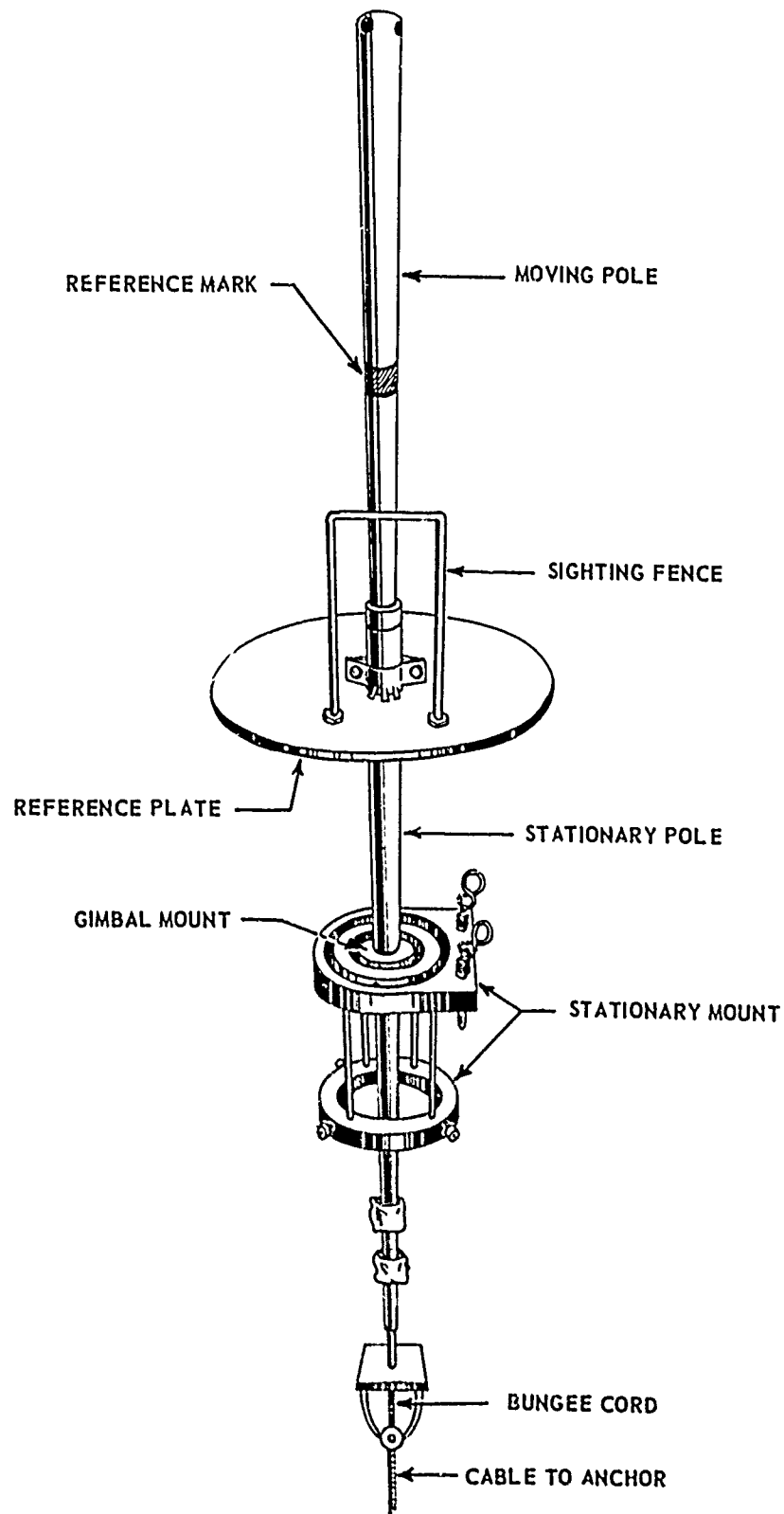
Figure 1 Hover Pole
