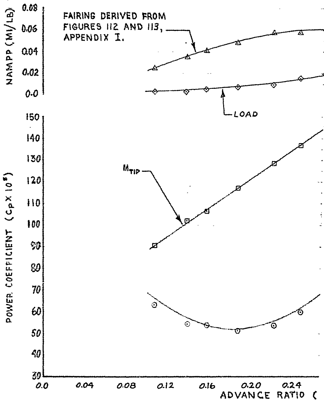
FIGURE 57. NONDIMENSIONAL LEVEL FLIGHT
