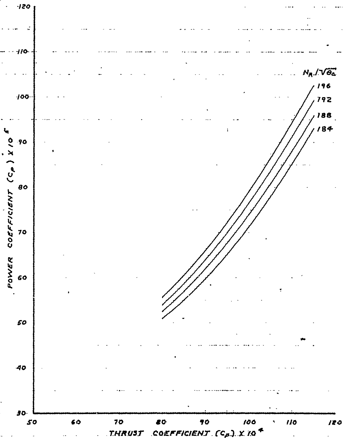
FIGURE 88. LEVEL FLIGHT PERFORMANCE SUMMARY (AQM-91A)
