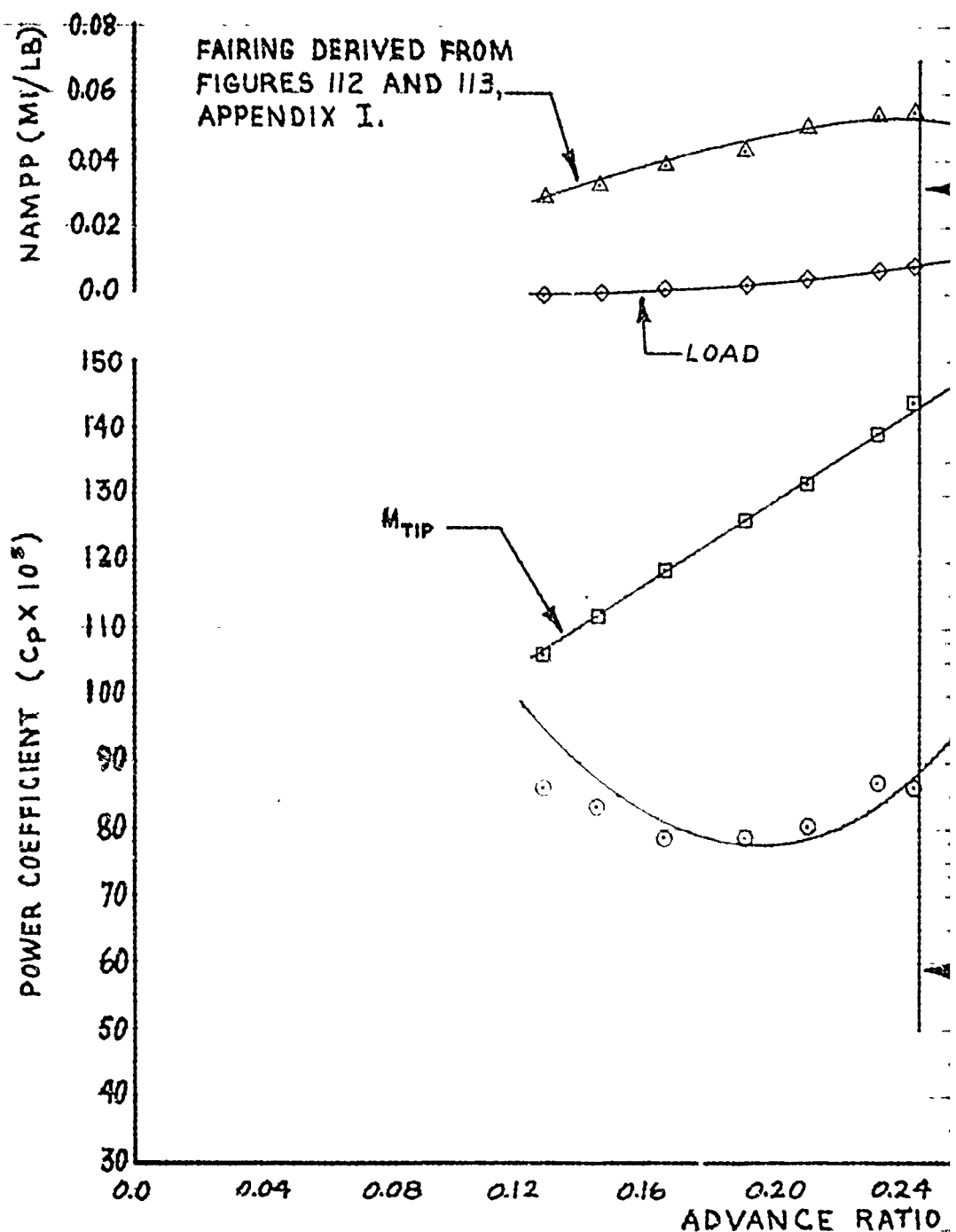
FIGURE 62. NONDIMENSIONAL LEVEL F
