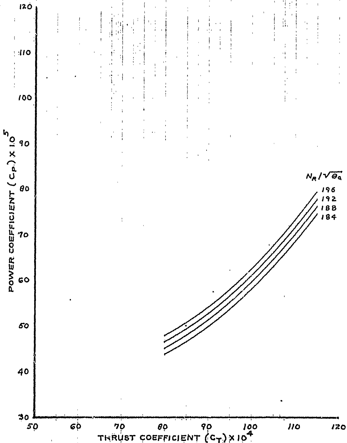
FIGURE 48. LEVEL FLIGHT PERFORMANCE SUMMARY (AQM-34L)
