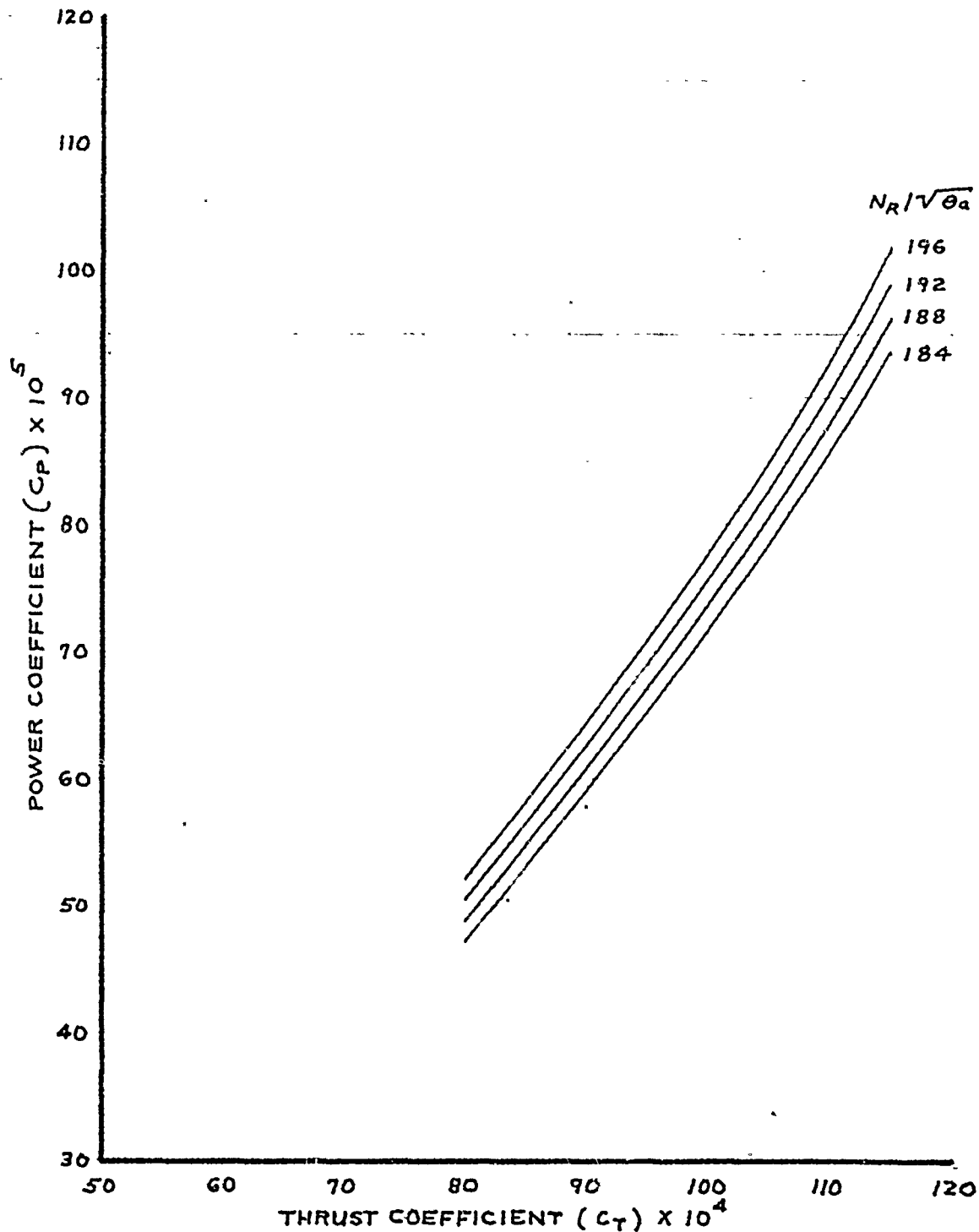
FIGURE 46. LEVEL FLIGHT PERFORMANCE SUMMARY (AQM-34L)
