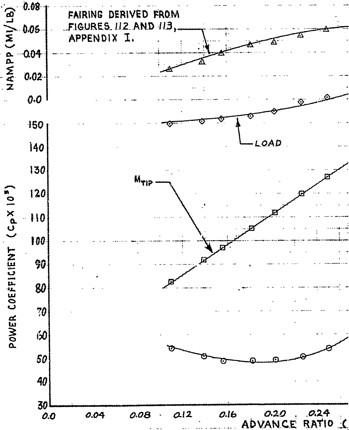
FIGURE 73. NONDIMENSIONAL LEVEL FLIGHT
