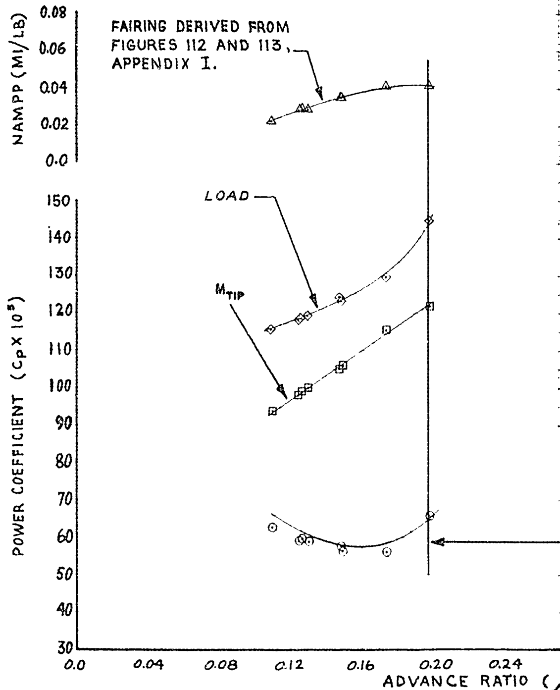
FIGURE 98 NONDIMENSIONAL LEVEL FLIGHT
