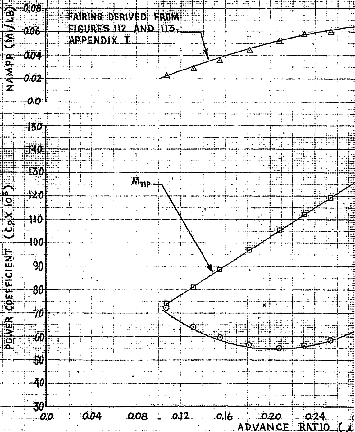
FIGURE 33 NONDIMENSIONAL LEVEL FLIGHT
