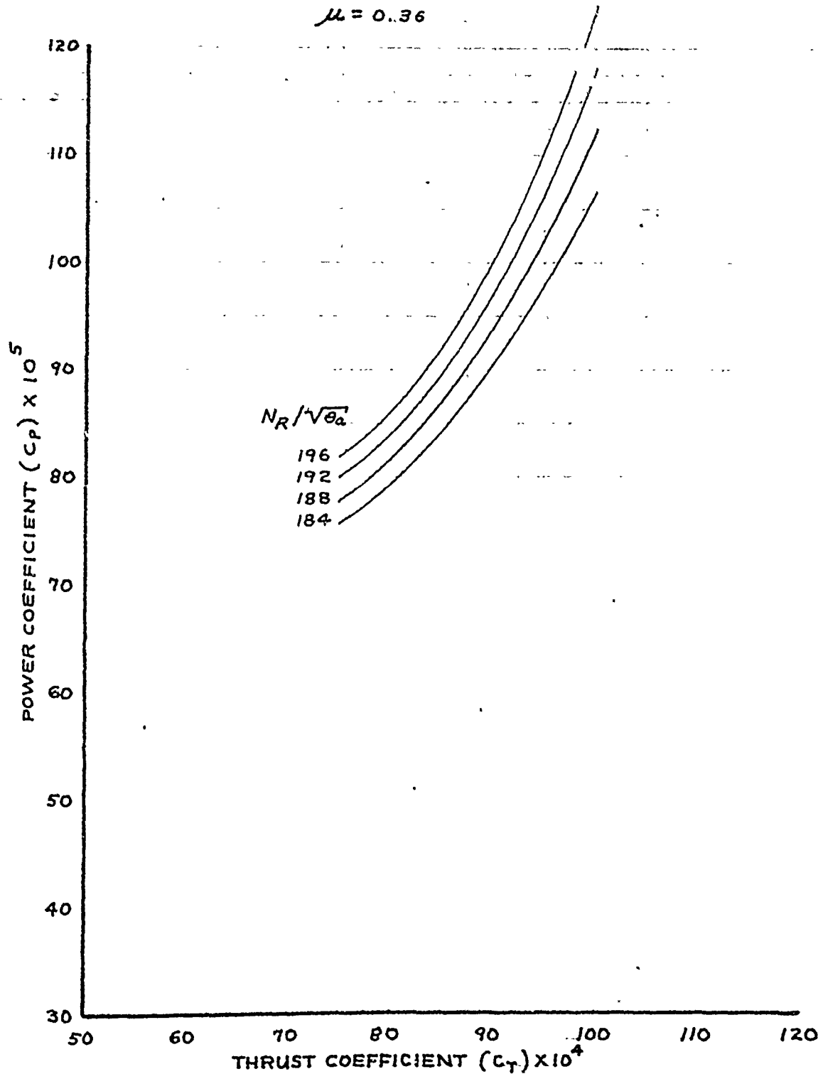
FIGURE 24. LEVEL FLIGHT PERFORMANCE SUMMARY (CLEAN)
