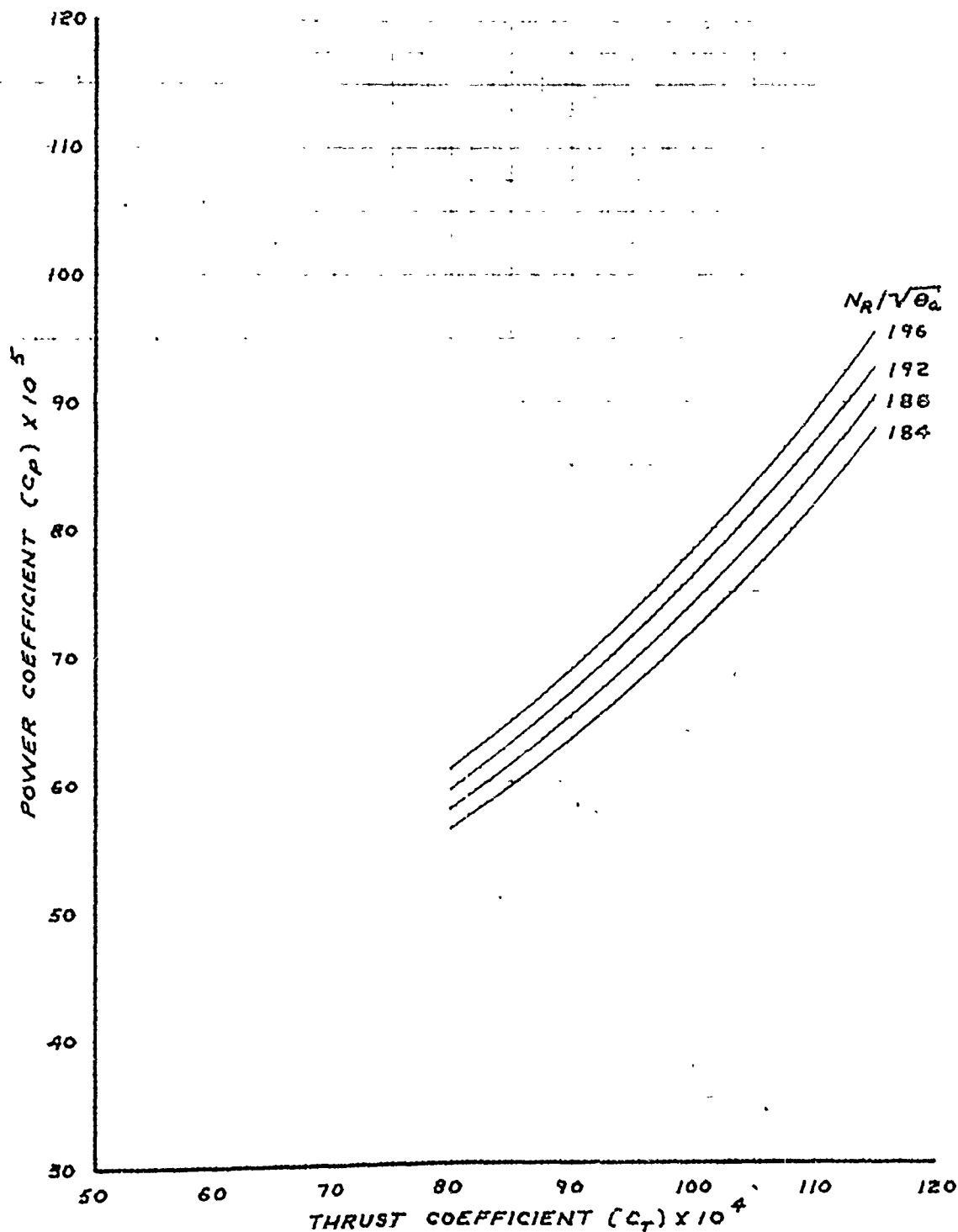
FIGURE 92. LEVEL FLIGHT PERFORMANCE SUMMARY (AQM-91A) 119
