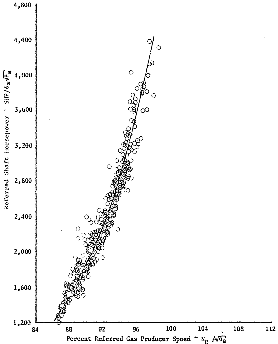
Figure 108. Engine Characteristics
