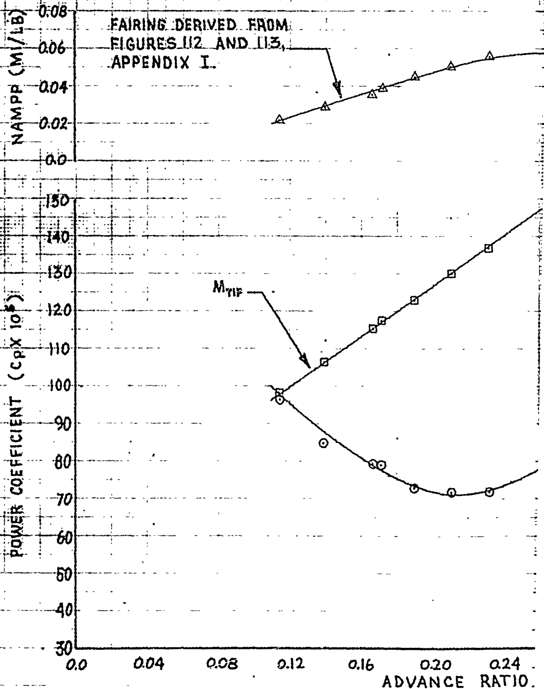
FIGURE 40 NONDIMENSIONAL LEVEL 1
