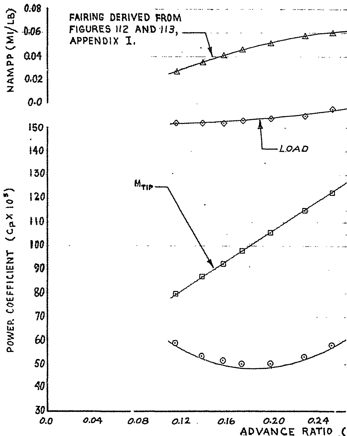
FIGURE 55. NONDIMENSIONAL LEVEL FLI
