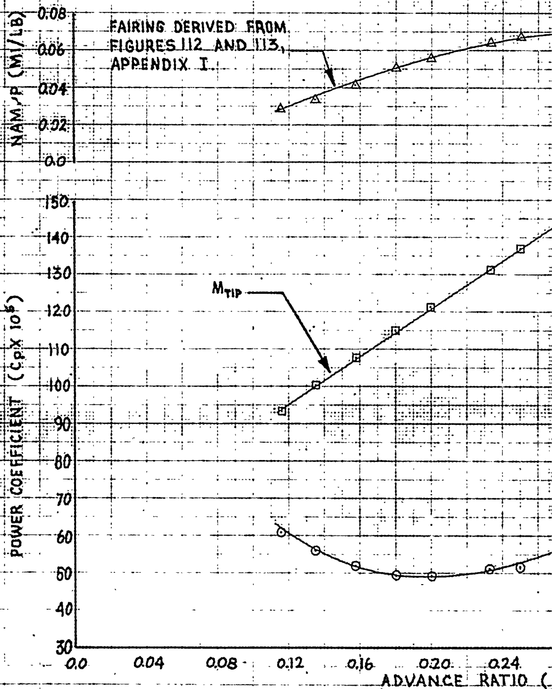
FIGURE 31 NONDIMENSIONAL LEVEL FLIGHT
