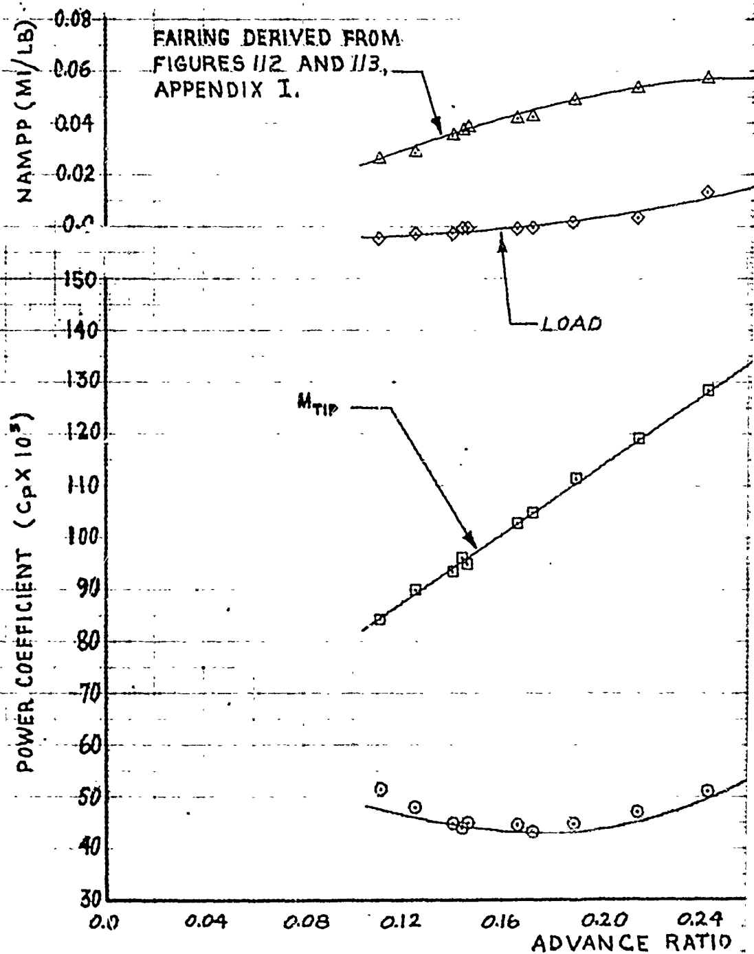
FIGURE 52. NONDIMENSIONAL LEVEL F
