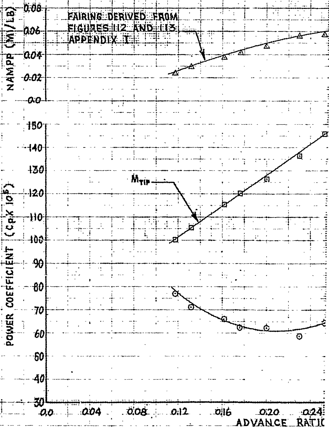
FIGURE 36 NONDIMENSIONAL LEVEL
