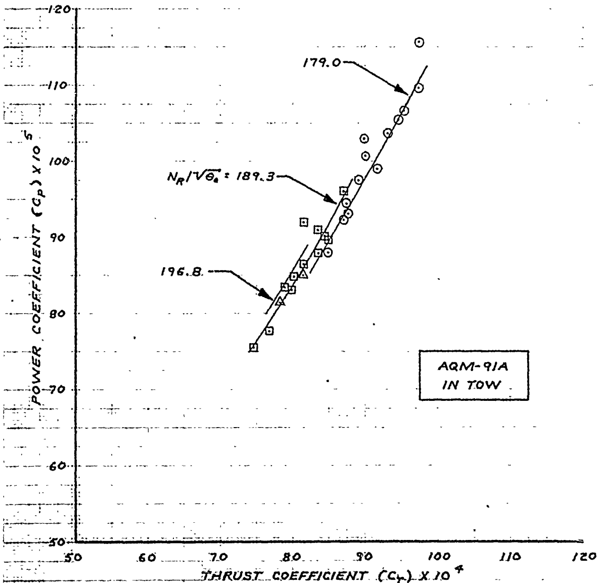
FIGURE 10. NONDIMENSIONAL HOVERING PERFORMANCE (AQM-91A)
