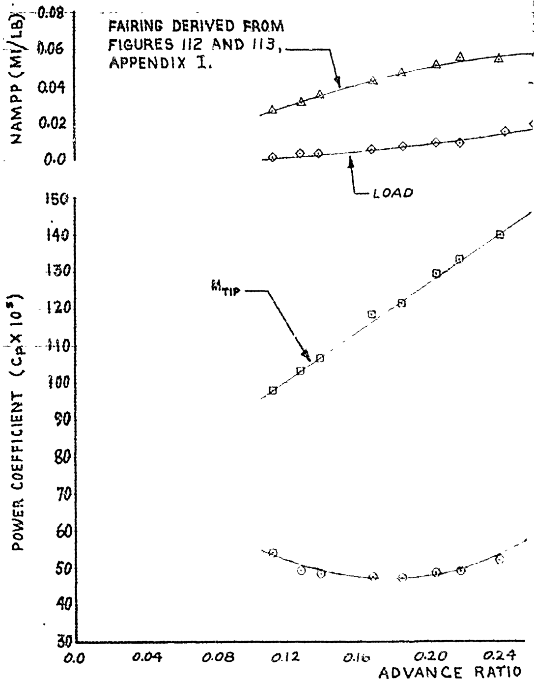
FIGURE 54. NONDIMENSIONAL LEVEL 1
