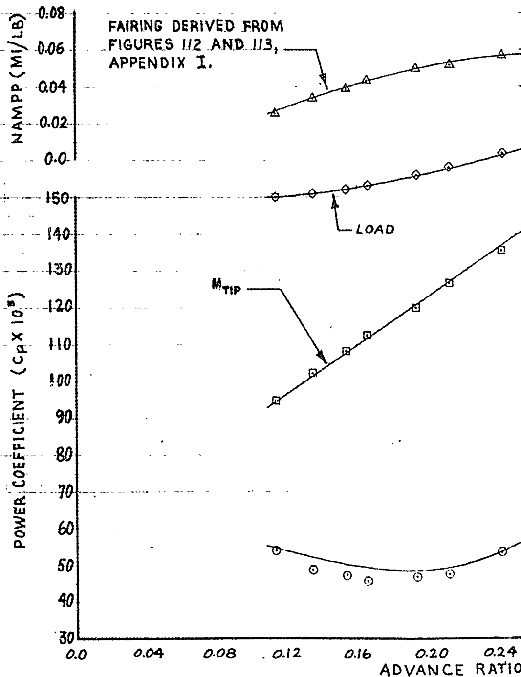
FIGURE 74. NONDIMENSIONAL LEVEL
