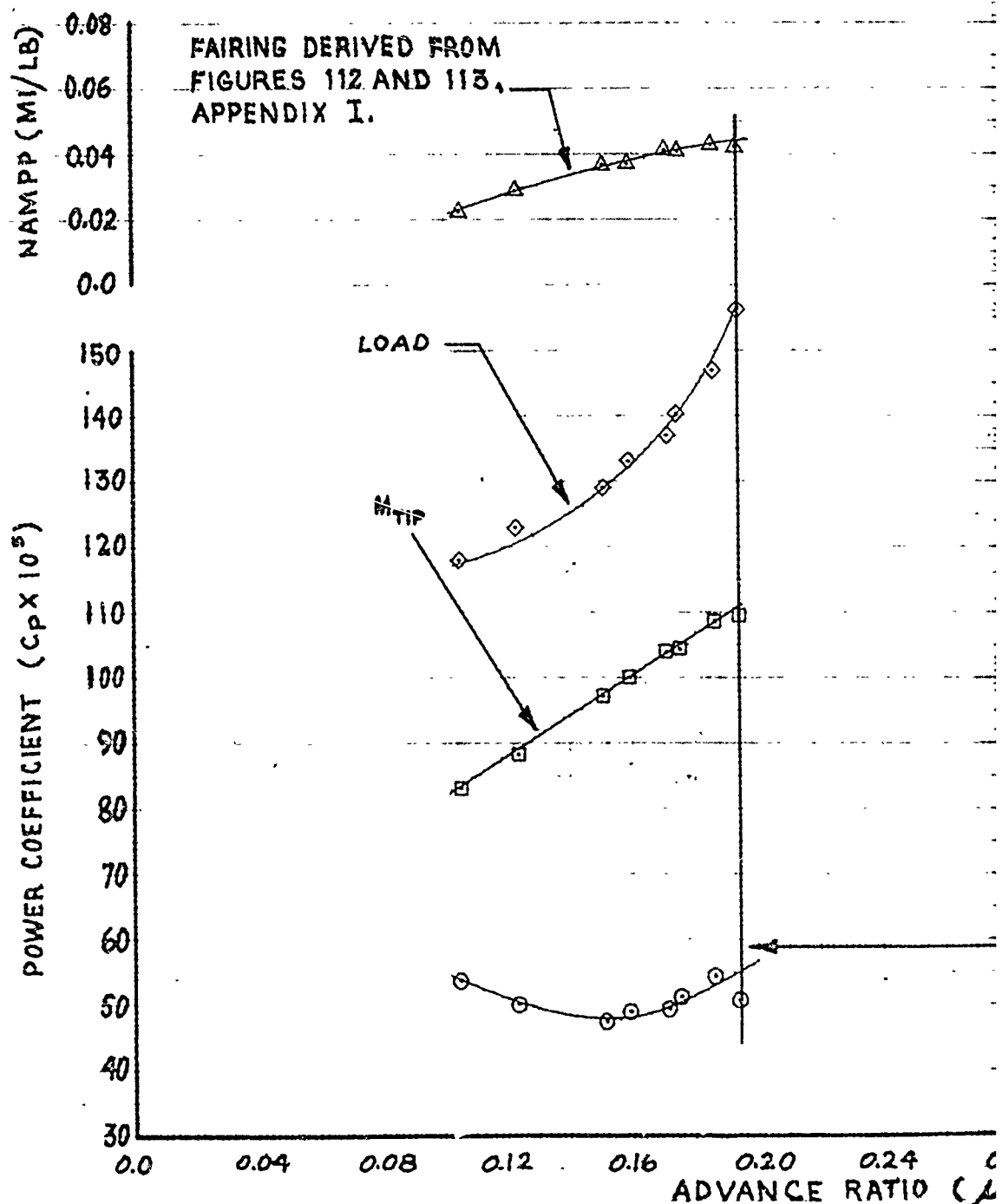
FIGURE 93 NONDIMENSIONAL LEVEL FLIGHT
