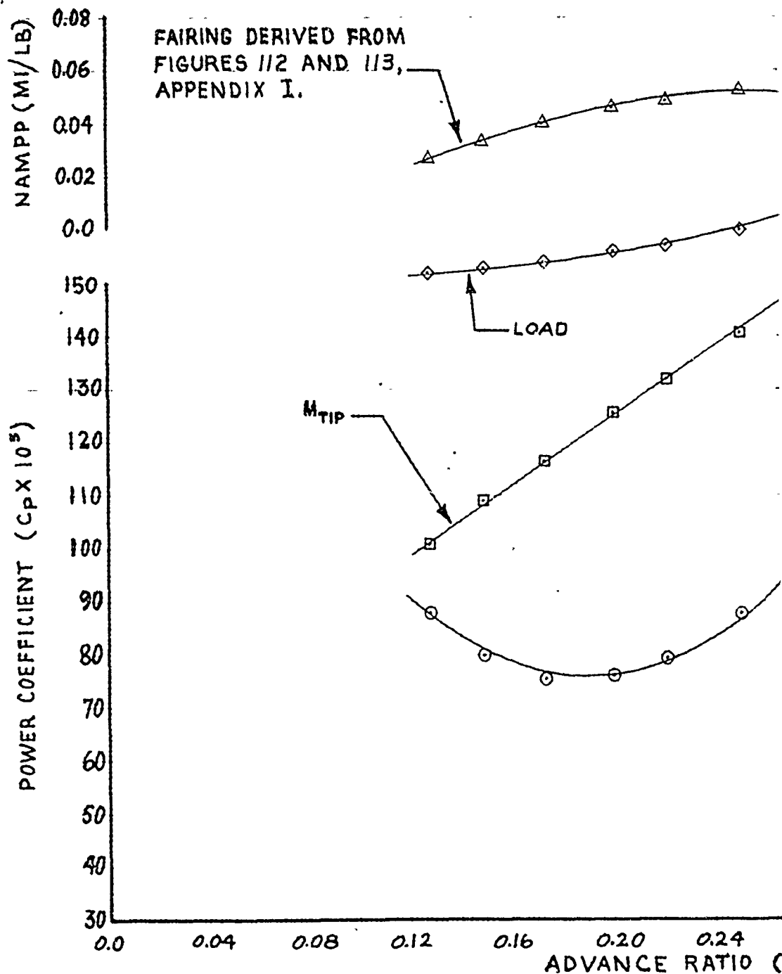
FIGURE 81. NONDIMENSIONAL LEVEL FLIGHT
