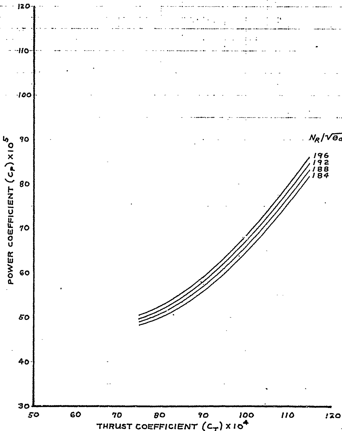
FIGURE 22. LEVEL FLIGHT PERFORMANCE SUMMARY (CLEAN)
