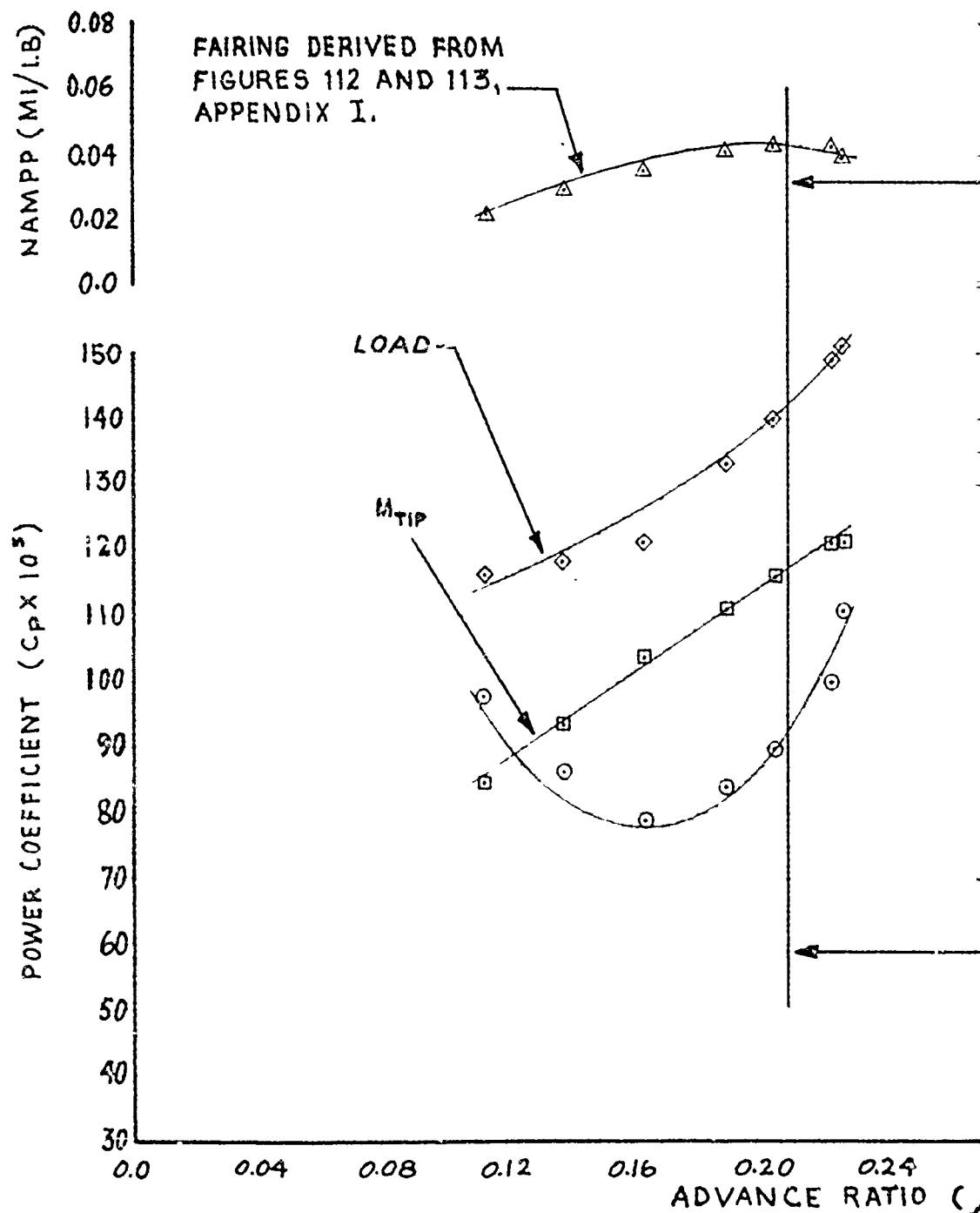
FIGURE 105 NONDIMENSIONAL LEVEL FLIGHT
