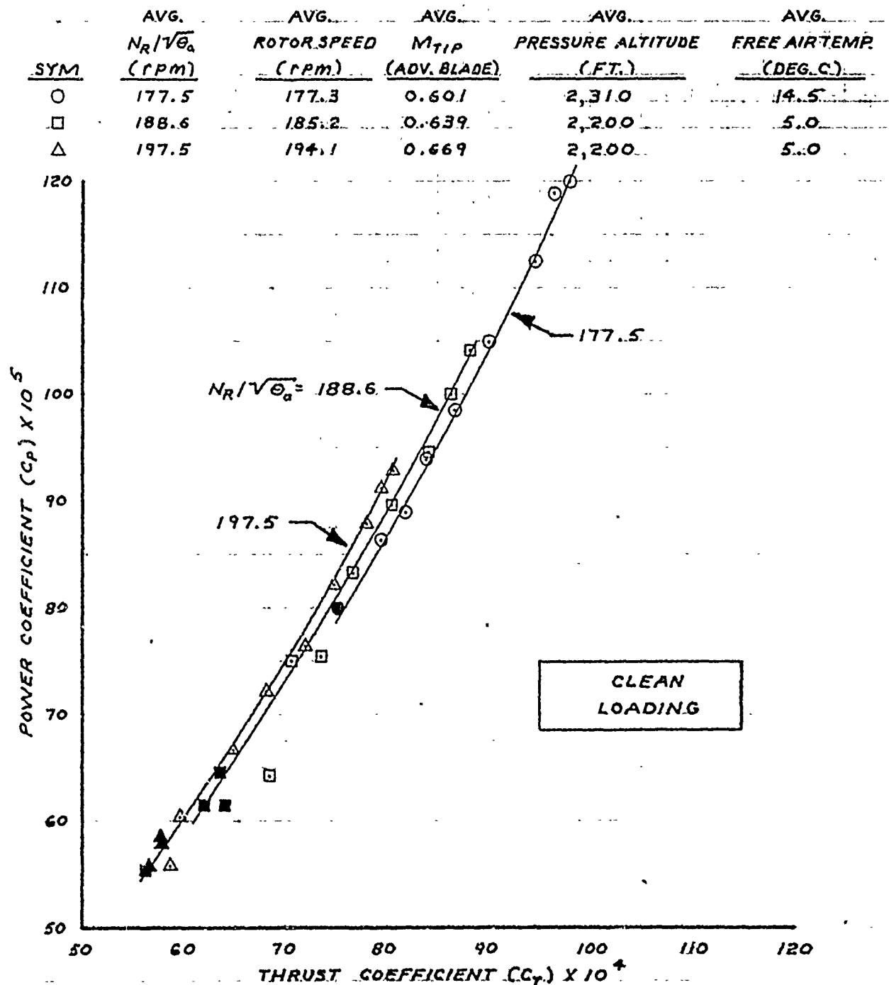
FIGURE 8. NONDIMENSIONAL HOVERING PERFORMANCE
