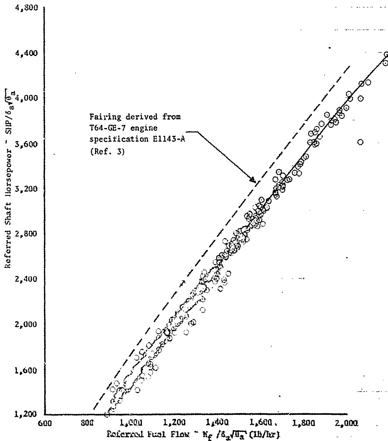
Figure 72. Engine Characteristics
