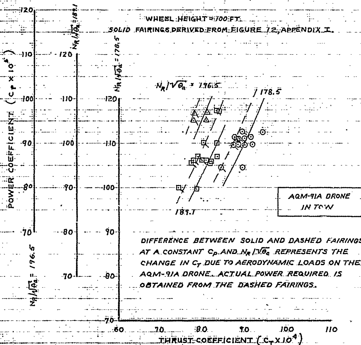
FIGURE 6. NONDIMENSIONAL HOVER PERFORMANCE
