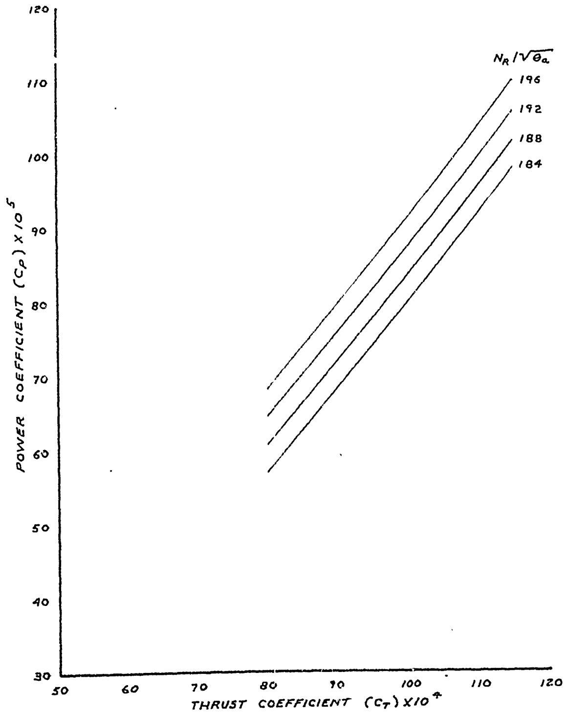
FIGURE 72. LEVEL FLIGHT PERFORMANCE SUMMARY (AQM-34R)
