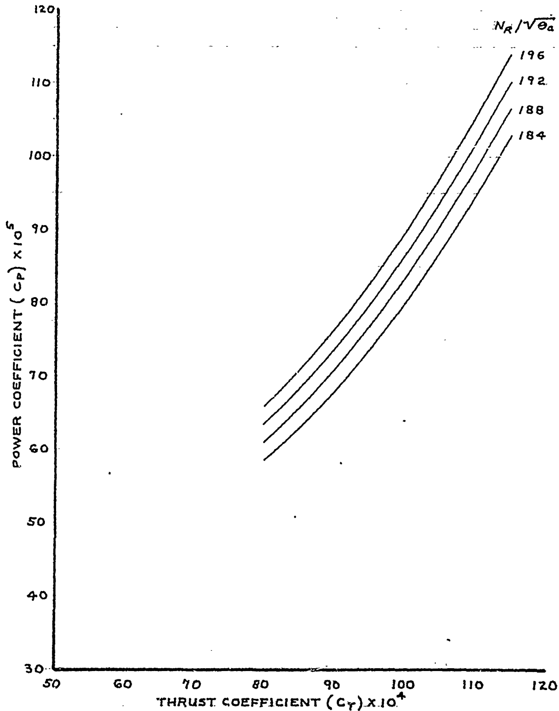
FIGURE 50. LEVEL FLIGHT PERFORMANCE SUMMARY (AQM-34L)
