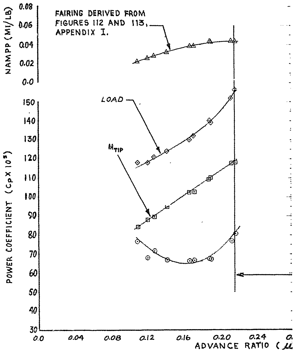
FIGURE 101 NONDIMENSIONAL LEVEL FLIGHT
