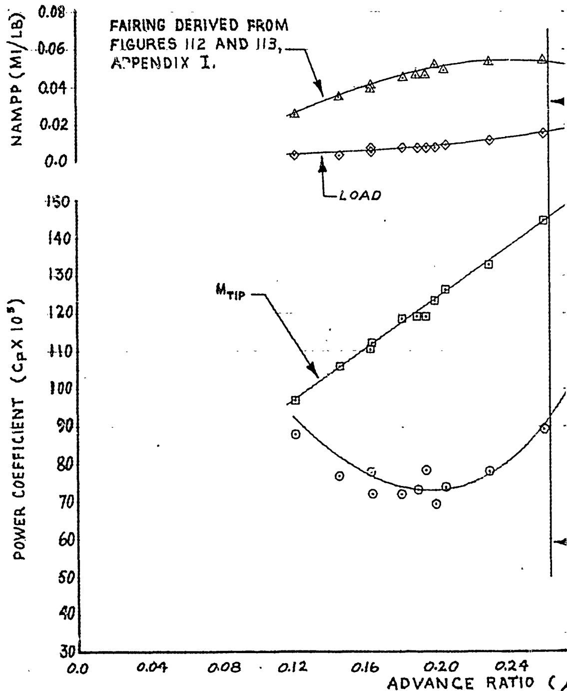
FIGURE 61. NONDIMENSIONAL LEVEL FLIGHT
