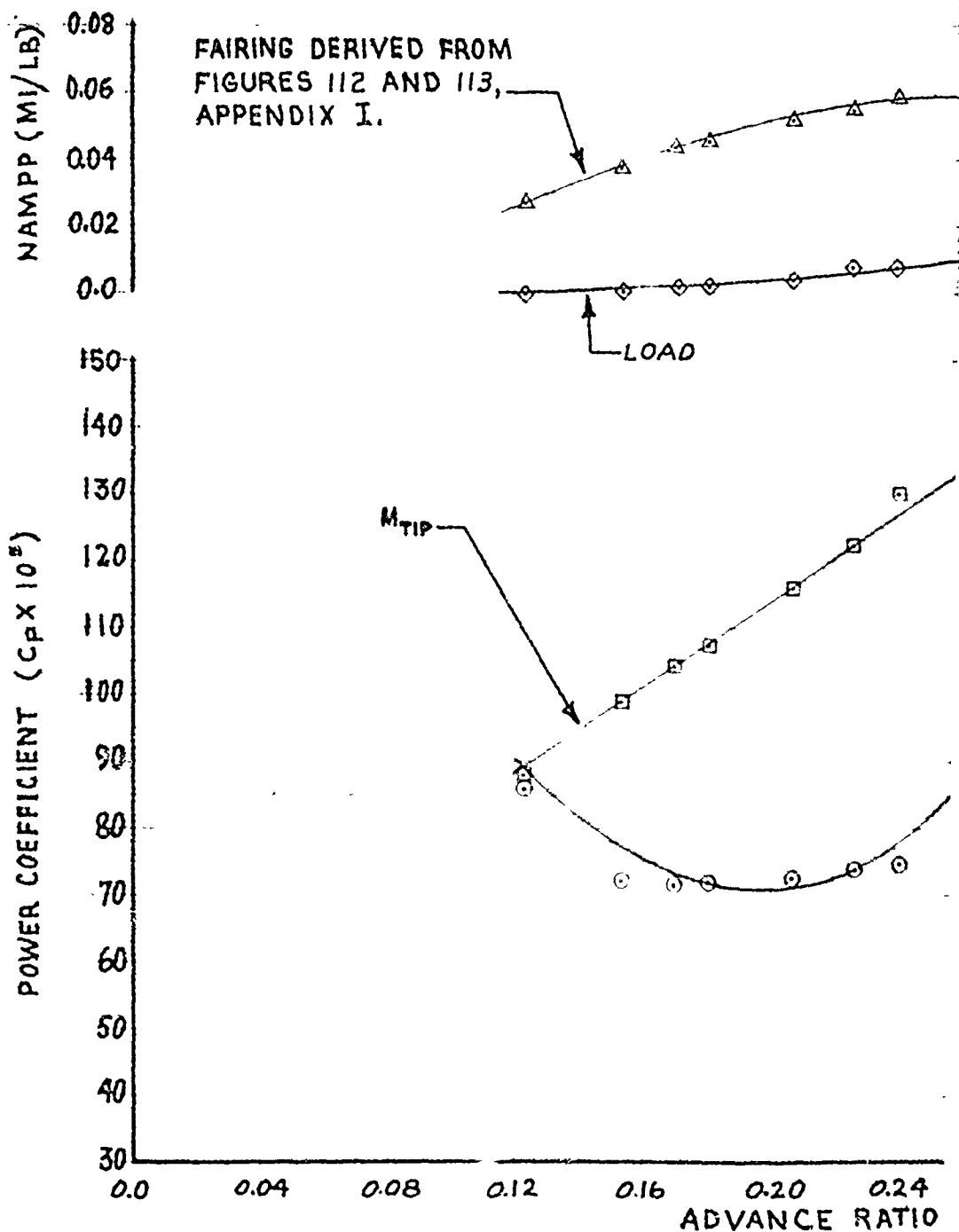
FIGURE 60. NONDIMENSIONAL LEVEL
