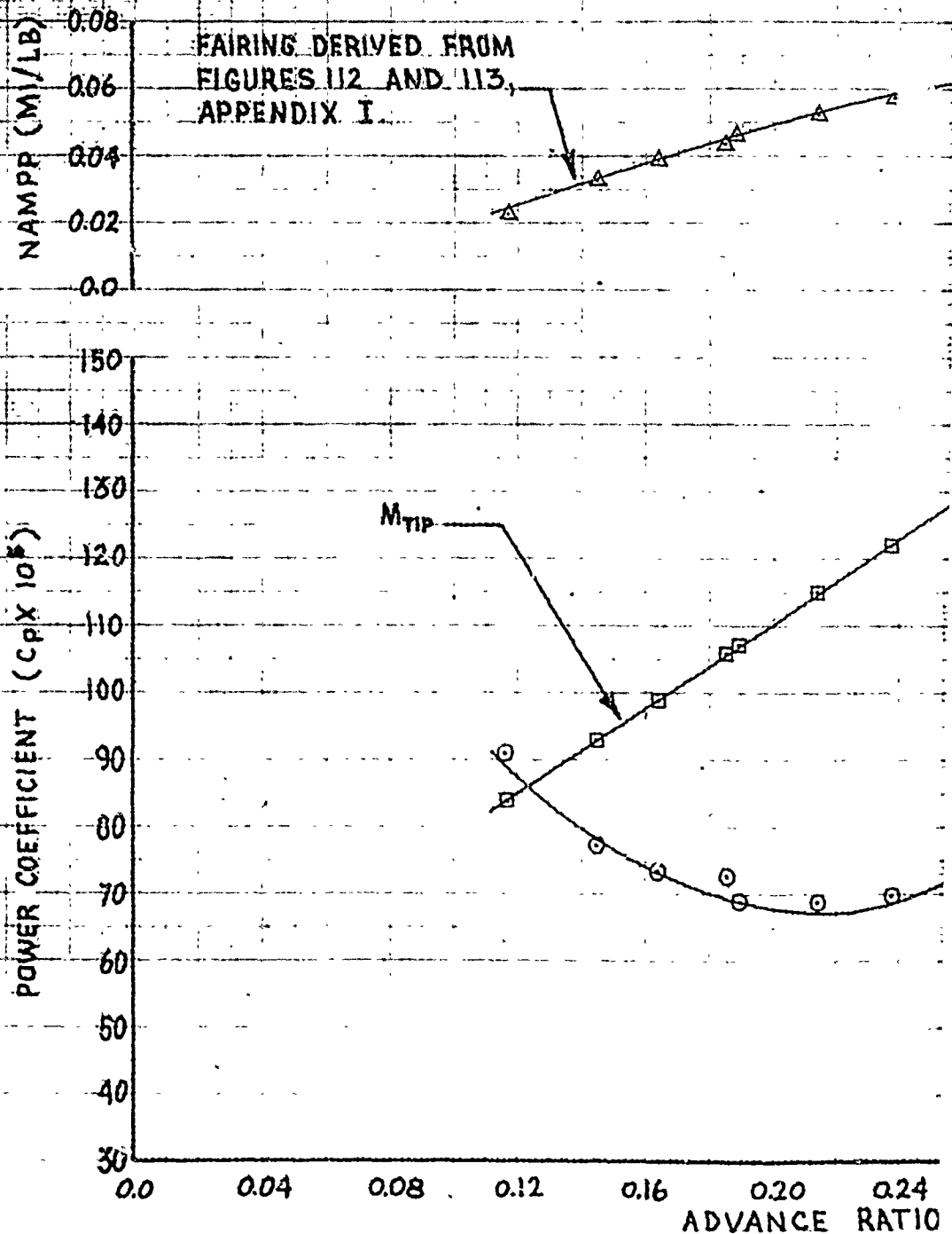
FIGURE 38 NONDIMENSIONAL LEVEL
