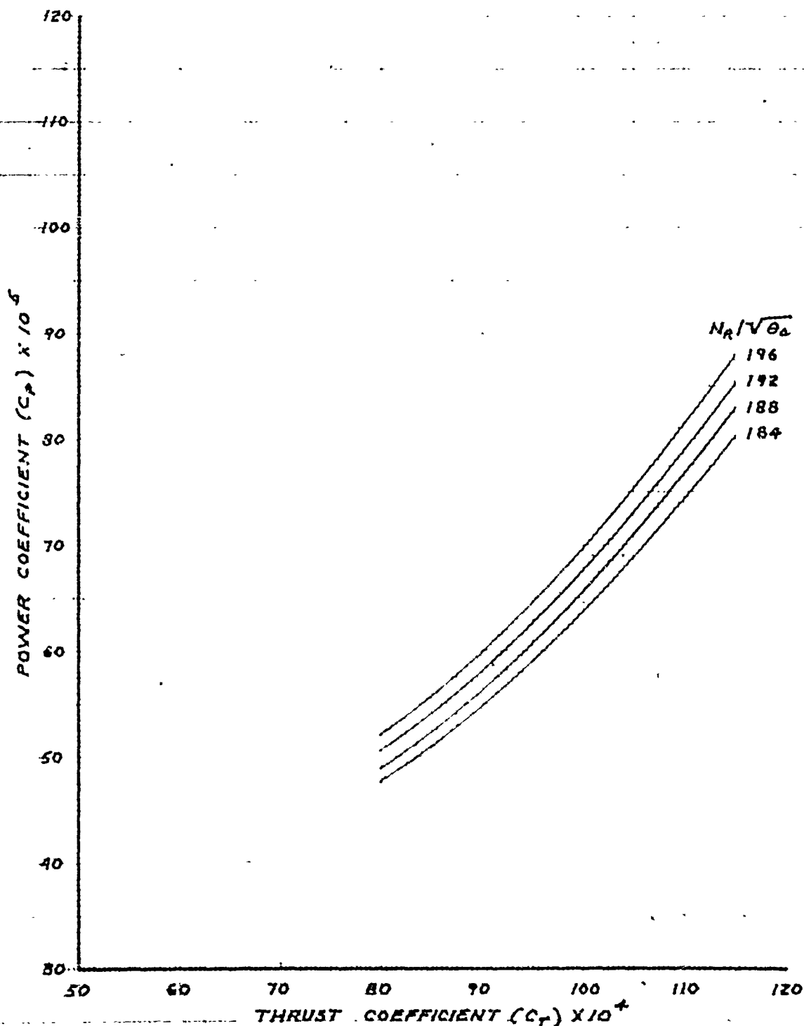
FIGURE 90. LEVEL FLIGHT PERFORMANCE SUMMARY (AQM-91A)
