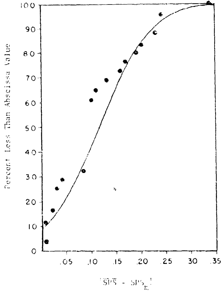
Figure 2-2. Cumulative Probability Distribution of SP_5 - SP_{5m}
