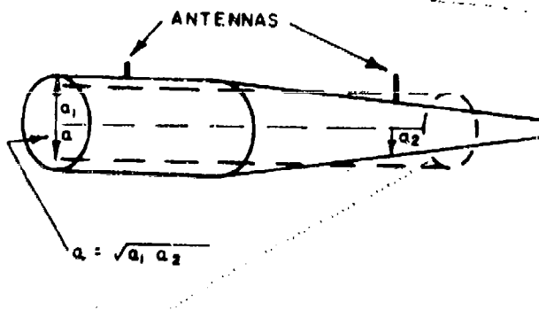
Figure III-6. Geometric Mean Cylinder
