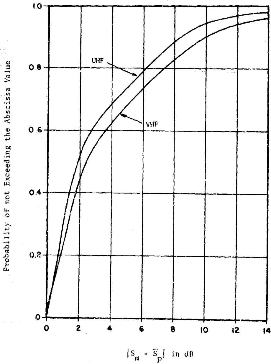
Figure II-1. Cumulative Probability Distribution of |S_m - \bar{S}_p|
