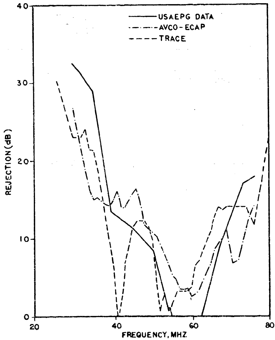
Figure IV-10. AT-912/VRC Band 7 Rejection
