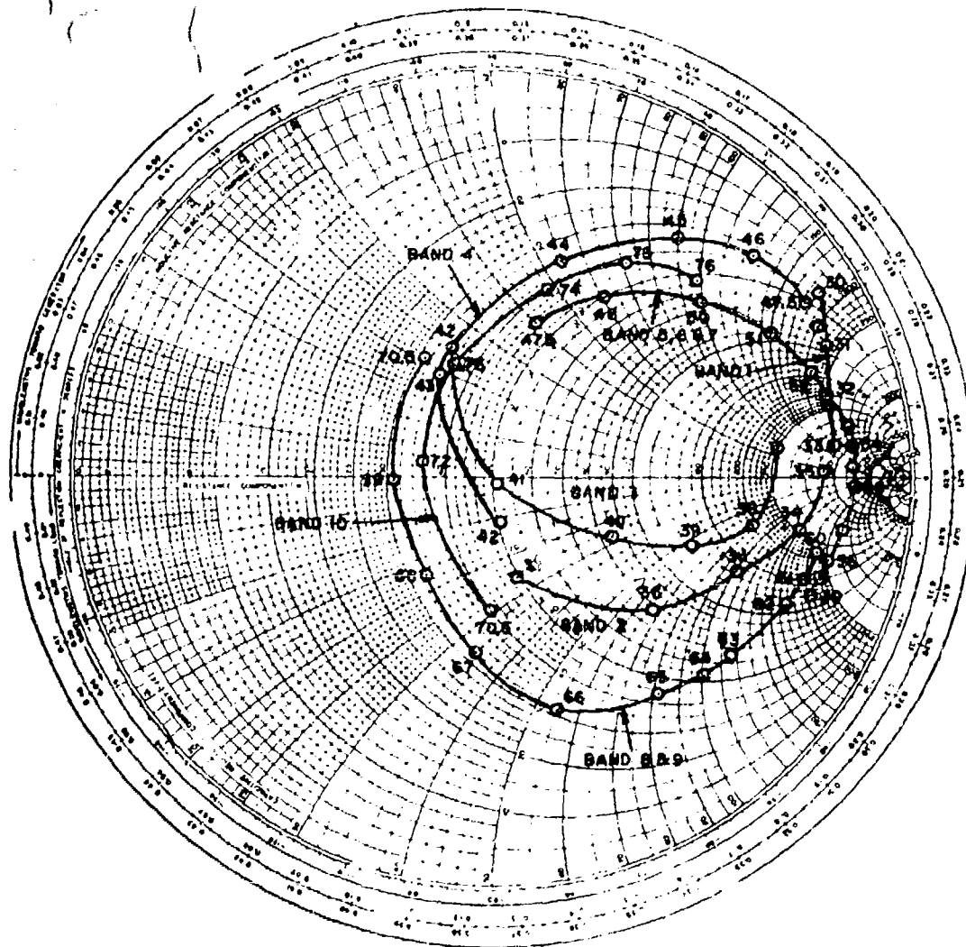
Figure IV-14. Measured Impedance of AT-912/VRC Center-Fed Antenna
