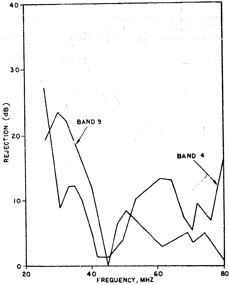
Figure IV-19. Recommended AT-912/VRC Band 4 & 9 Rejection Model
