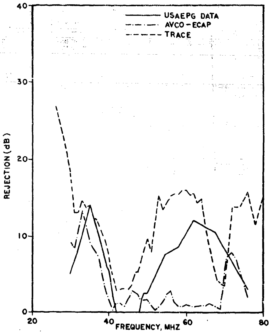
Figure IV-7. AT-912/VRC Band 4 Rejection
