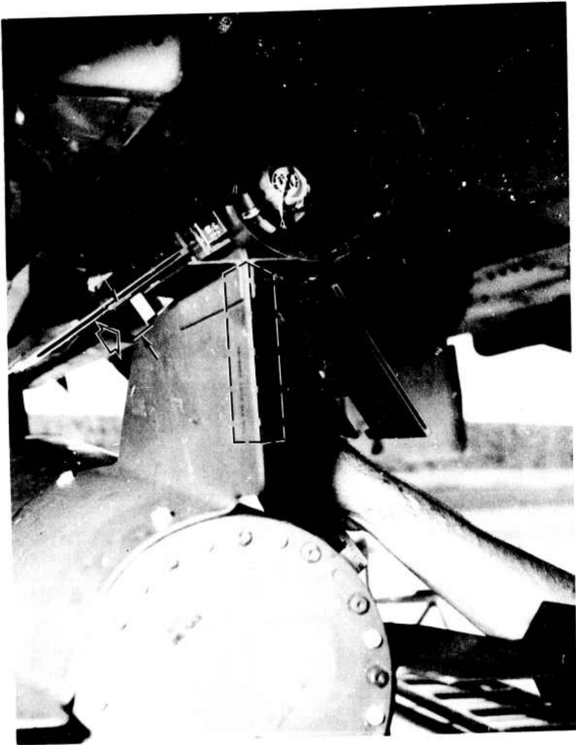
Figure 3. AIM-4D missile and CBU-67B/B on shoulder TER station with minimum missile-to-store clearance of 1 1/8 inches (arrow). Dotted lines show position of fin tabs on fins of CBU-67H/B
