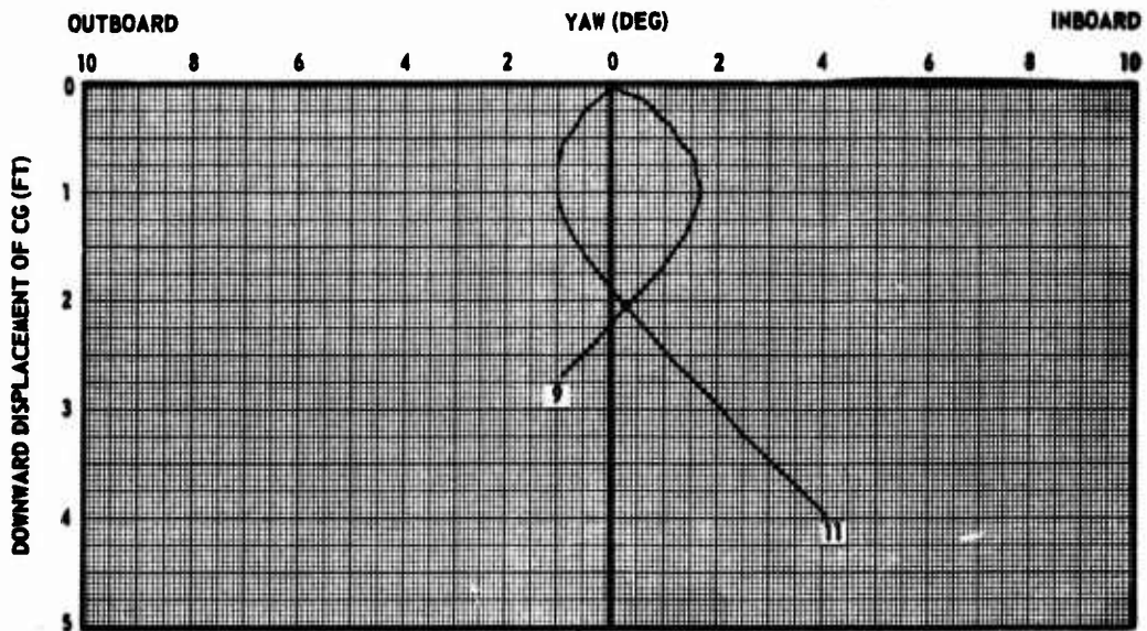
Figure I-1. Separation characteristics of MK 82 LDGP at 550 KCAS
