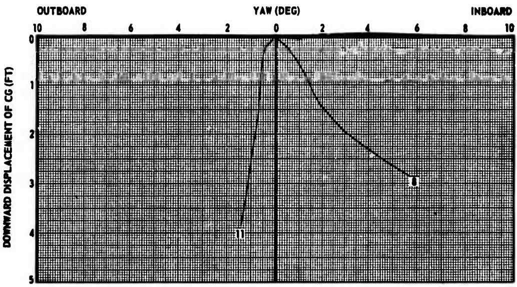
Figure I-3. Separation characteristics of CBU-67H/B at 475 KCAS
