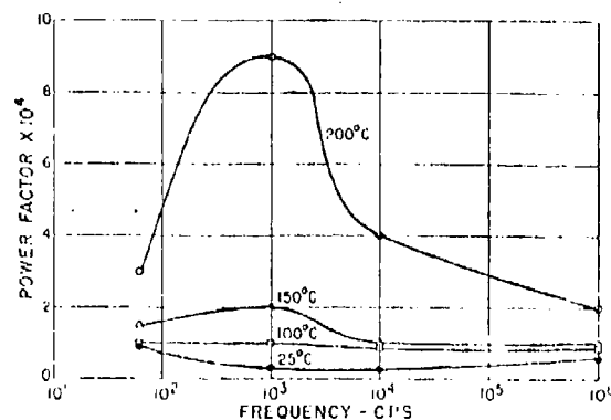
Figure 5.6 The effect of frequency on the power factor of SF96(40) silicone liquid at selected temperatures of test.
