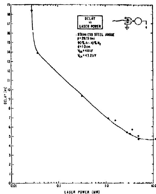
Figure 9.7 Delay versus laser power from 0.028 to 11 MW. Total laser duration 14-15 ns. The pulsewidth (FWHM) 5.5-6.5 ns.
