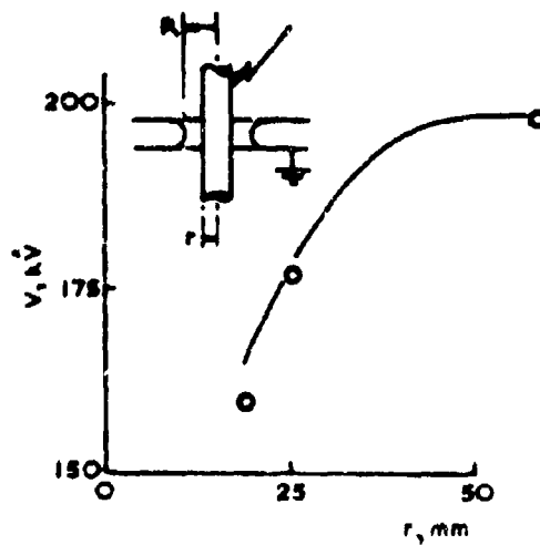
Figure 4.107 Conductor and earthed metal plate, air, 1 atmosphere, R = 140 mm. — experimental, o estimated.
