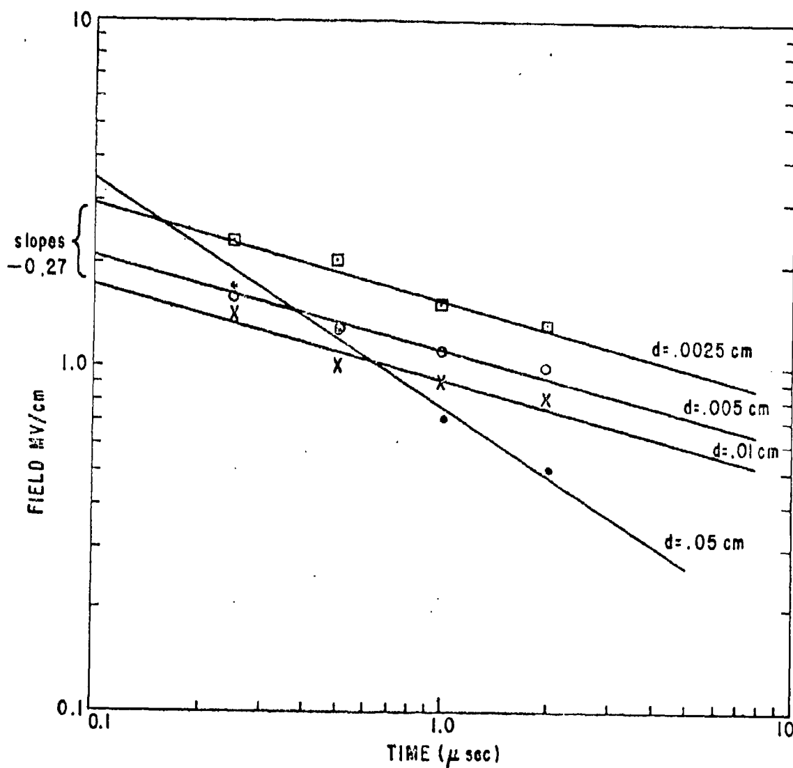
Figure 5.40 Russian data for small ball gaps.
