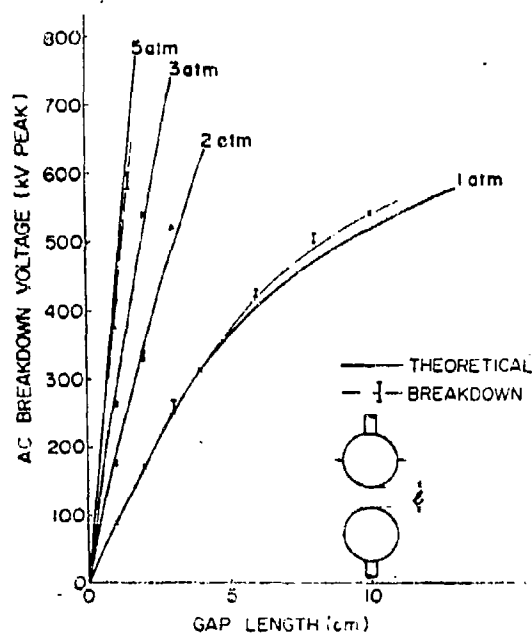
Figure 4.48 ac breakdown voltage for gap A (150 mm diameter spheres).
