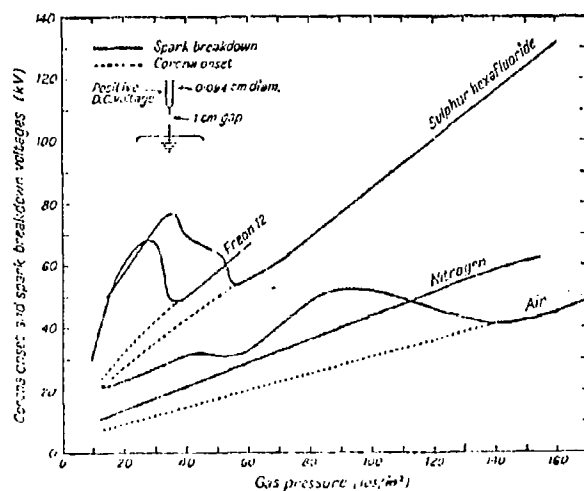
Figure 4.17 Voltage characteristics for a positive point-plane gap in compressed air, nitrogen, Freon, and sulphur hexafluoride.
