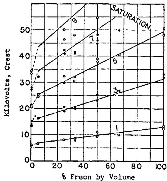
Figure 4.87 Sparking voltages in mixtures of Freon 12 and nitrogen.
