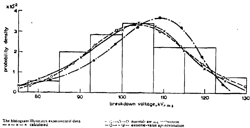
Figure 5.16 Breakdown probability density for circulating liquid subjected to 20s step-by-step test.
