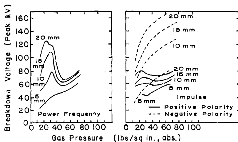
Figure 4.54 Breakdown voltage characteristics with point-sphere electrodes for \text{SF}_6 .
