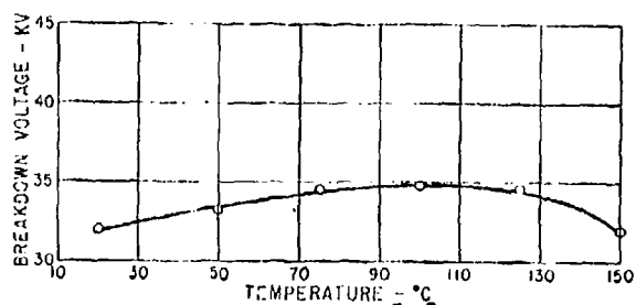
Figure 5.2 The effect of temperature on the breakdown voltage of transformer oil.
