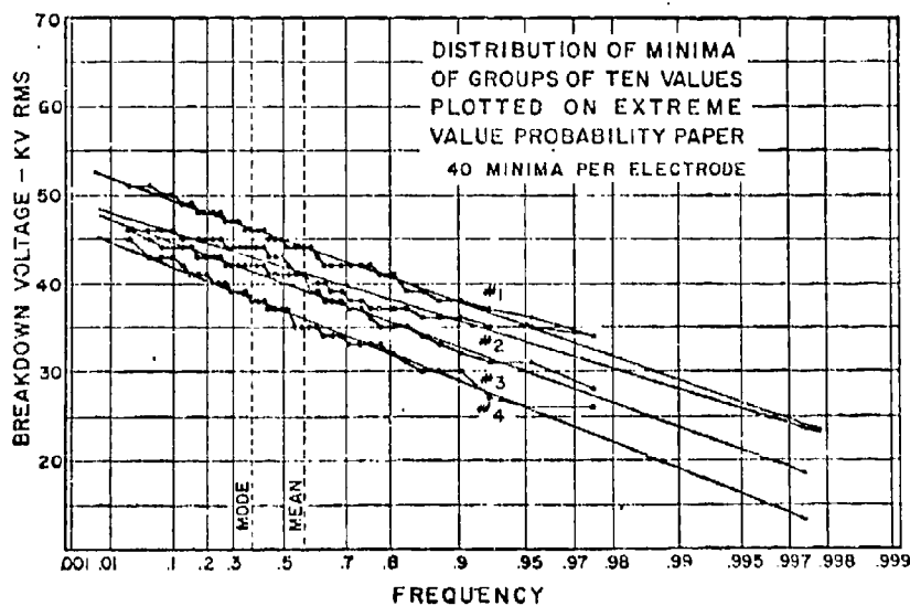
Figure 5.14 Minima-of-groups area effect. Breakdown voltage distributions of transformer oil for minima of successive groups of ten for data of Figure 5.13.
