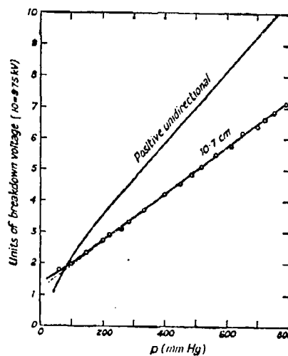
Figure 4.38 Variation of breakdown voltage with pressure for coaxial-line spark-gap.
