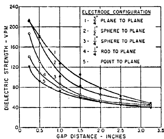
Figure 4.68 Showing the decrease in the voltage gradient at breakdown which accompanies the increase in the test gap for different electrode configurations for sulfur hexafluoride when tested by impulse voltage at atmospheric pressure. (VPM-volts per mil)
