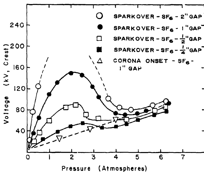
Figure 4.55 ac spark-over and corona onset voltages of sulfur hexafluoride for indicated gaps between 1/16 inch hemisphere point and 6 inch diameter plane in 12 inch diameter steel tank as a function of pressure.
