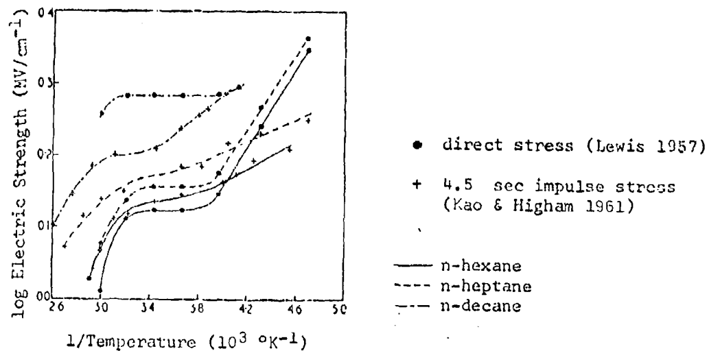
Figure 5.3 Temperature dependence of the electric strength of n-alkanes.
