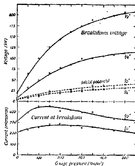
Figure 4.16 Voltage and current characteristics for a 0.25 inch and 0.5 inch gaps in air between a negative point and a plane. Broken curves show corona initiation potential.
