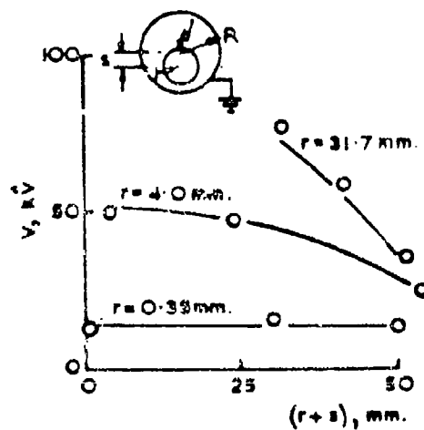
Figure 4.106 Concentric and eccentric cylinders, air, 1 atmosphere R = 63.5 mm. — experimental, o estimated.
