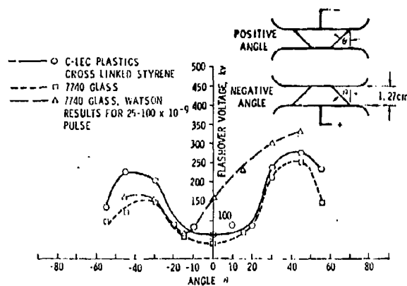
Figure 7.29 Flashover voltage versus angle \theta for 7740 glass and crosslinked styrene. Pulse risetime about 5 \mu s.
