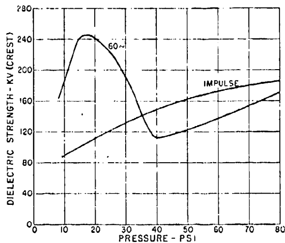
Figure 4.73 The effect of gas pressure on the breakdown of dichlorodifluoromethane (Freon 12).
