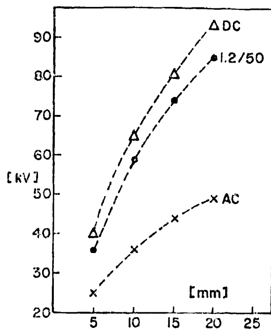
Figure 7.23 Comparison of dc, ac and 1.2/50 \mu sec. FO characteristics ( p = 1 \times 10^{-5} torr).
