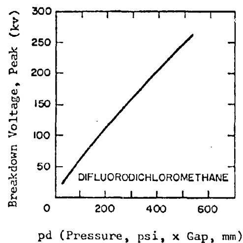
Figure 4.83 Paschen curve for Freon 12.
