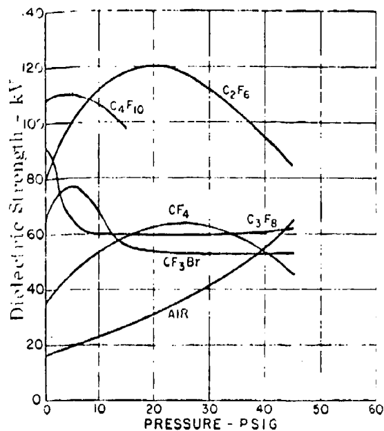
Figure 4.72 The dielectric strength of the fluorinated hydrocarbon gases as affected by pressure, tested under nonuniform field conditions.
