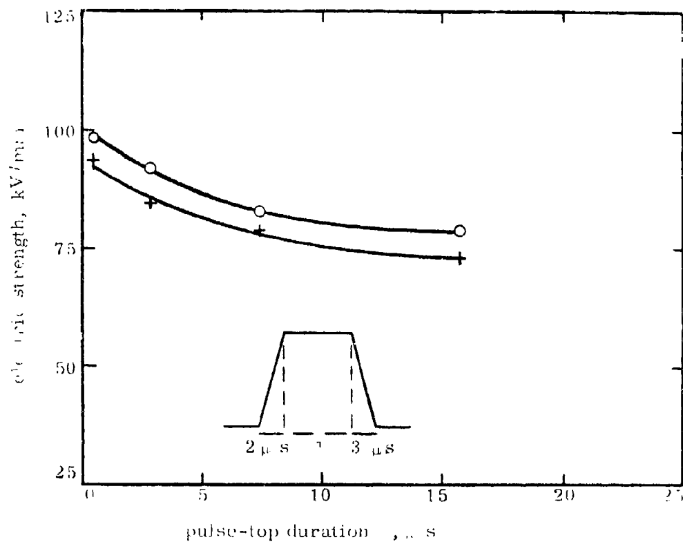
Variation in electric strength with pulse-top duration
