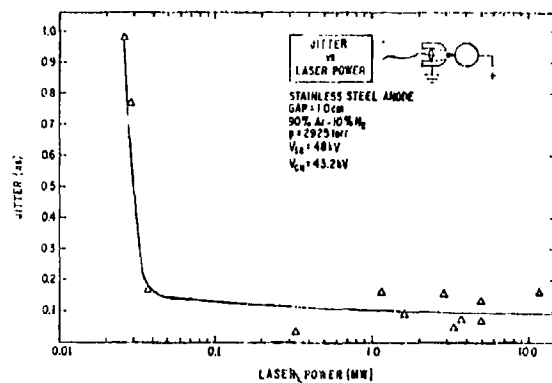
Figure 9.8 Jitter versus laser power.
