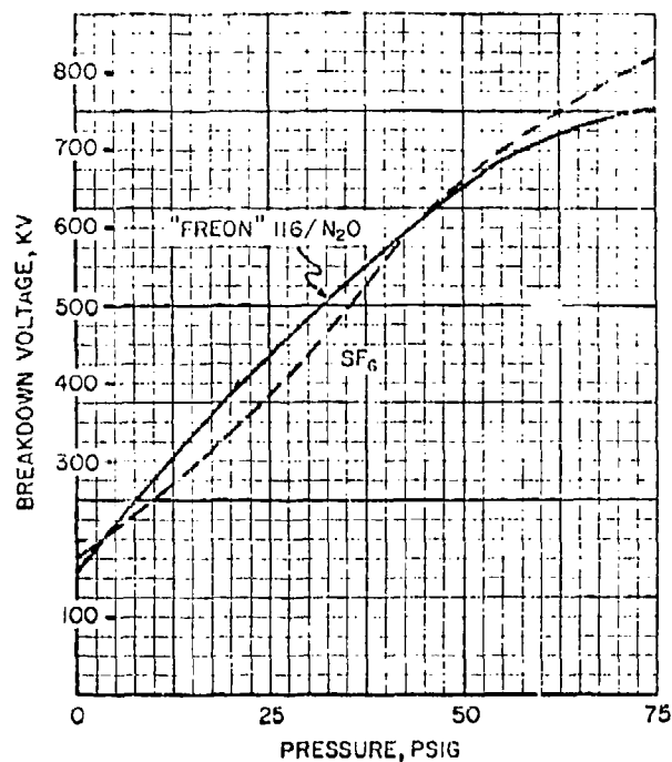
Figure 4.75 Comparison of breakdown voltage as a function of pressure for Freon 116/N 2 O (90/10 by wt) and SF 6 in a section of coaxial gas-filled transmission line. Inner conductor diameter - 3 inches, outer conductor diameter - 6 inches. The effective line length was 30 inches and the electrode gap was 1.5 inches.
