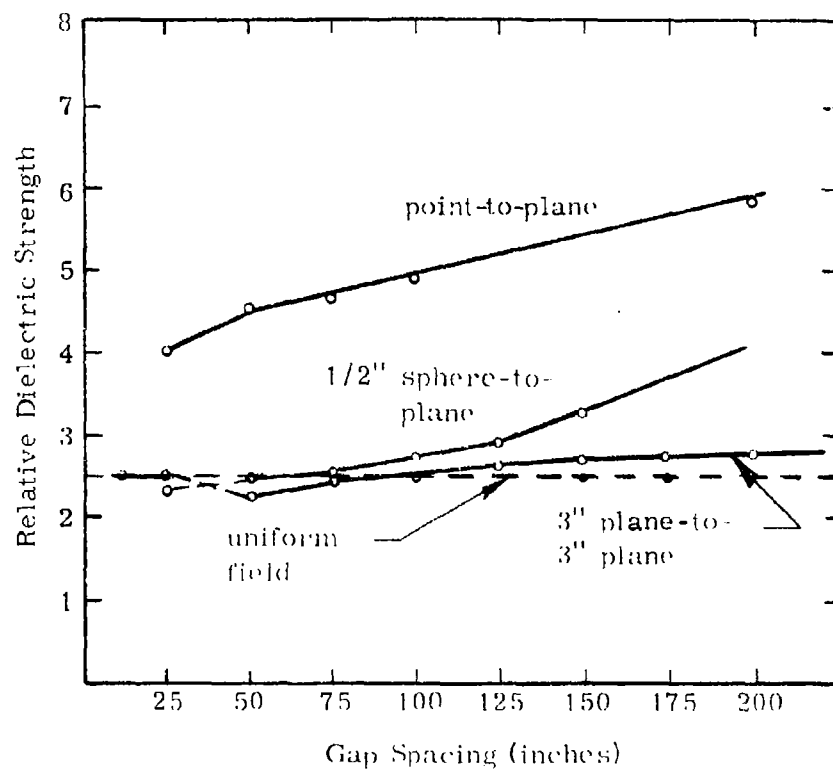
Figure 4.41 60-cycle relative strength of sulfur hexafluoride to dry air as a function of configuration and spacing of the electrodes. Gases at 25° C and at atmospheric pressure.
