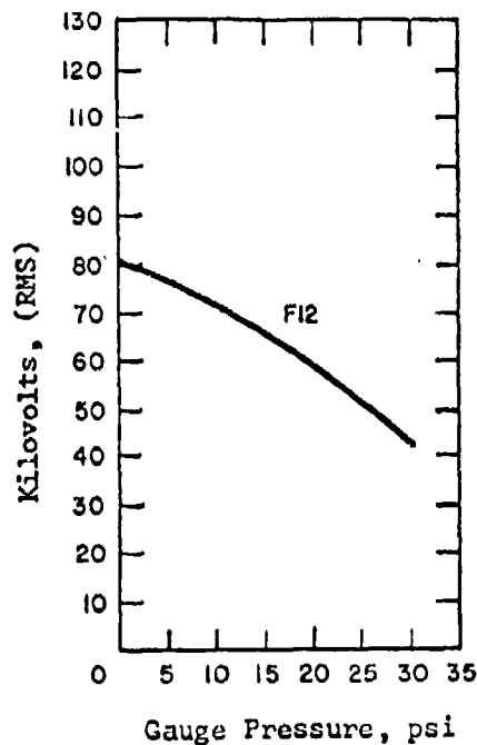
Figure 4.89 60 cycle dielectric strength of Freon 12, tested between tungsten rod and 1 inch diameter sphere spaced 1 inch.
