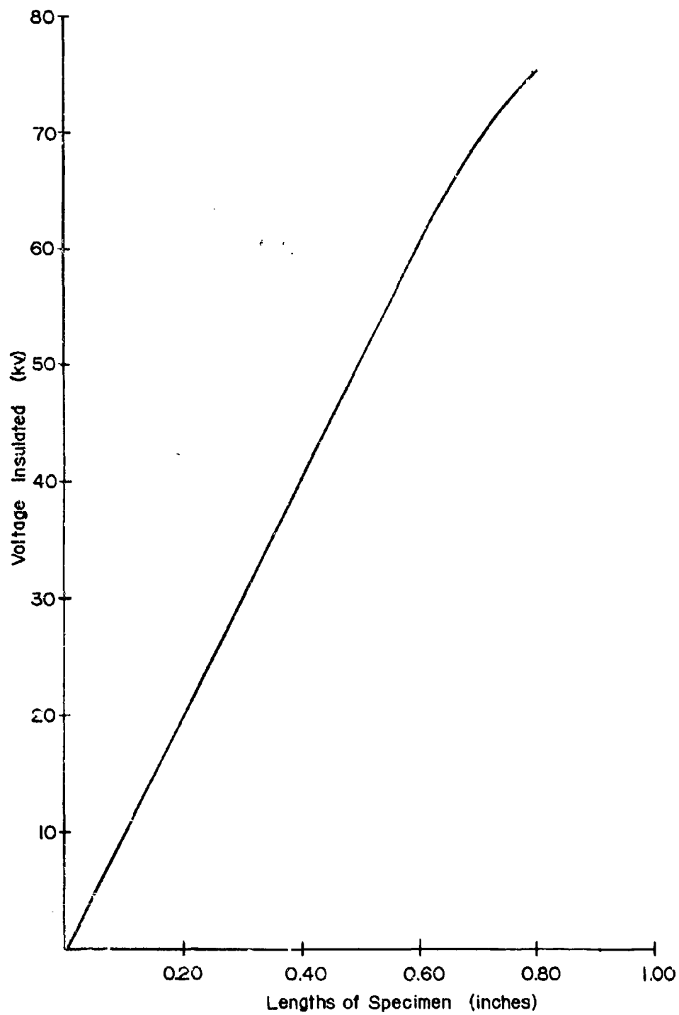
Figure 7.15 Insulation strengths over \text{Al}_2\text{O}_3 surfaces in vacuum.
