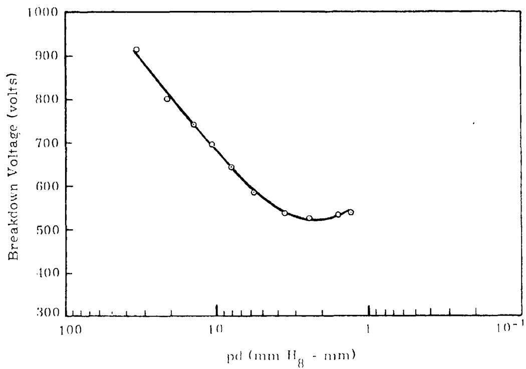
Figure 4.19 Faschen curve for sulfur hexafluoride (gap 1 mm, parallel circular brass plates, 4 inches in diameter and 1/4 inch thick with rounded edges of 1/8 inch radius.)
