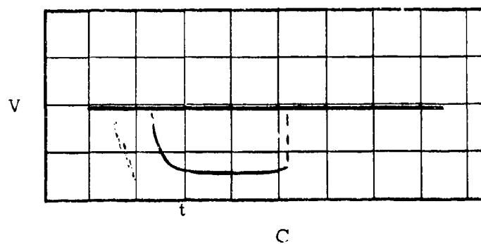
Figure 7.20 Oscillograms showing three types of breakdown. (Time base \sim 1 \mu\text{s/cm} )
