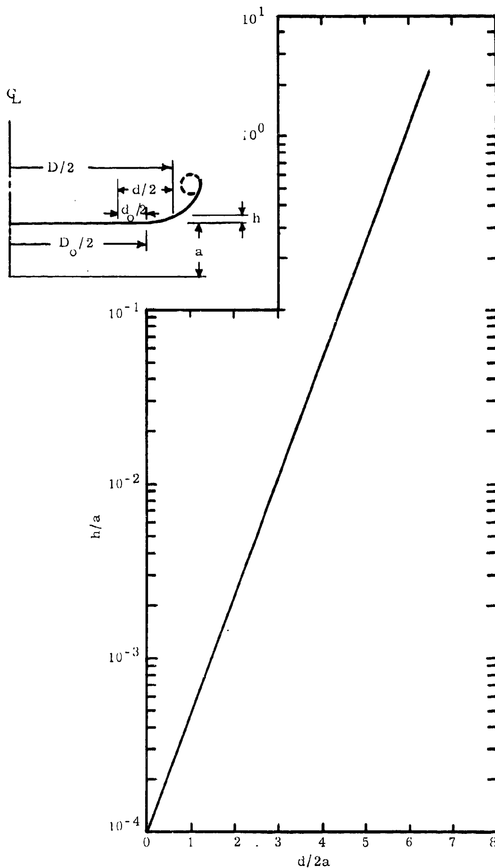
Figure 2.7 Curve for Constructing Rogowski Profiles
