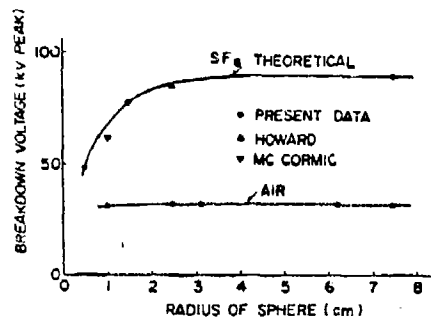
Figure 4.47 ac breakdown voltages of sphere-sphere gap as a function of sphere radius.
