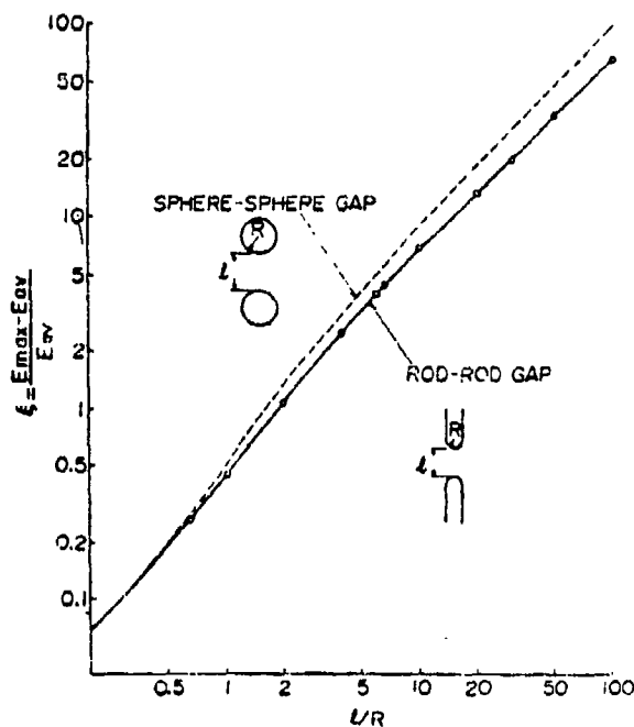
Figure 4.51 Field uniformity factor of sphere-sphere and rod-rod gaps.
