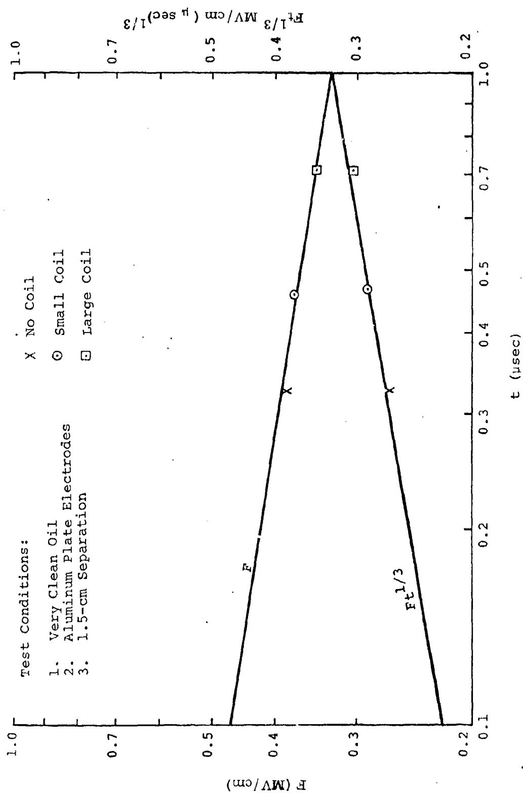
Figure 5.42 Breakdown strength of oil with aluminum electrodes constant breakdown phase.
