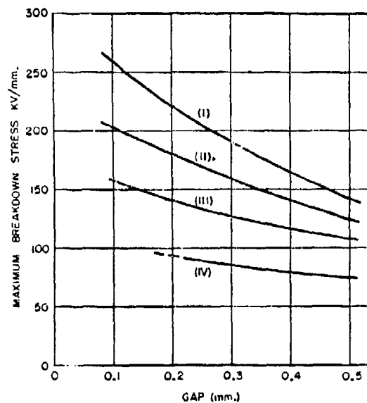
Figure 7.18 Maximum breakdown stresses and insulation strength, steel: (i) impulse voltage, 12/50 waveform; (ii) alternating voltage, 50 cps; (iii) direct voltage, rate of rise 6 kV/second; (iv) insulation strength (maximum dc voltage for zero breakdown in 1 hour).
