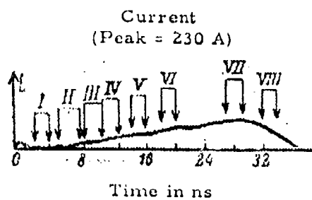
Figure 7.22 Development of gap luminosity in nanosecond breakdown of vacuum gaps.
