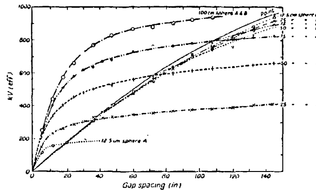
Figure 4.39 Breakdown voltage and corona onset voltage curves for sphere-plane gaps. The point-plane breakdown voltage curve is added for comparison. (Curves A are for corona onset. Curves B are for breakdown.)
