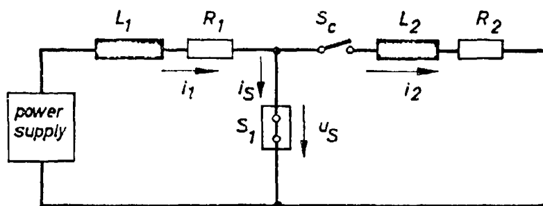
Circuit diagram
