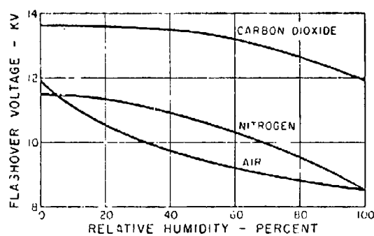
Figure 4.93 The flashover of porcelain insulators as affected by the surrounding gas and its moisture content.
