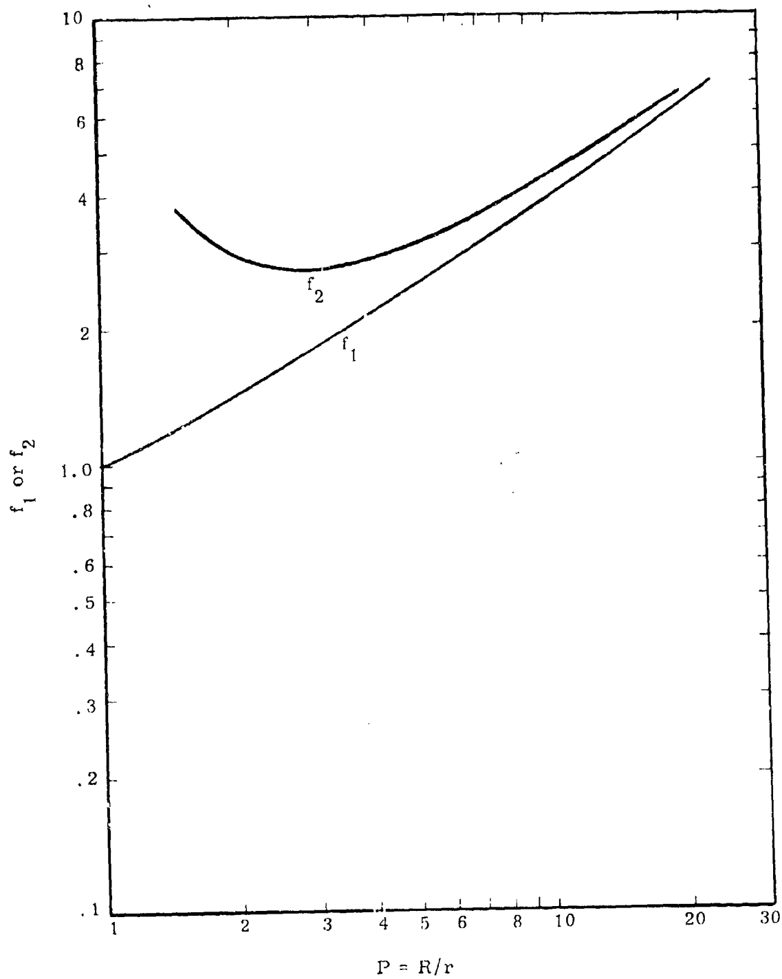
Figure 2.3 Field Enhancement Factors for Concentric Cylinders
