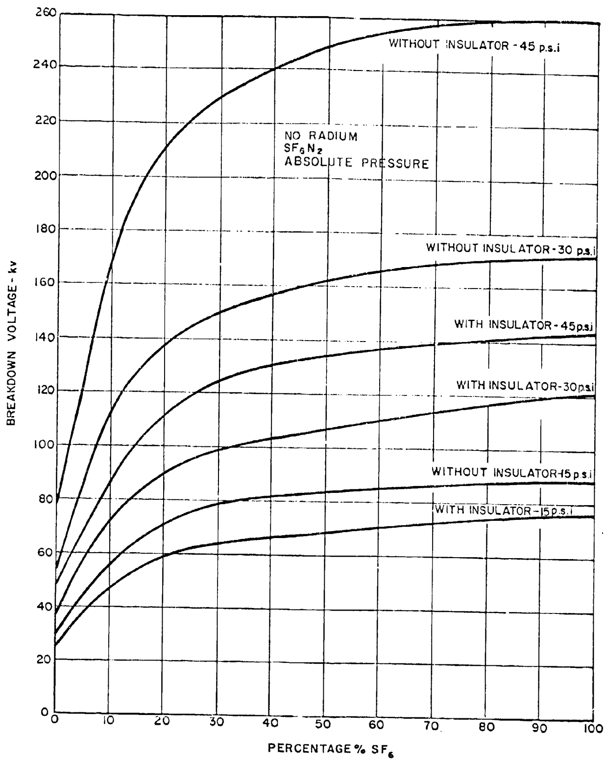
Figure 4.22 dc breakdown versus SF 6 uniform field--1 cm gap (15 cm diameter uniform field electrodes and porcelain insulator).
