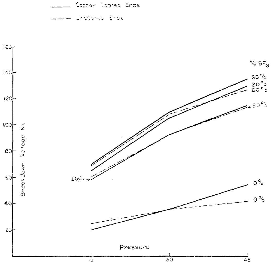
Figure 4.96 — Breakdown versus pressure across 1 cm porcelain insulator in mixtures of \text{SF}_6 with \text{N}_2 .
