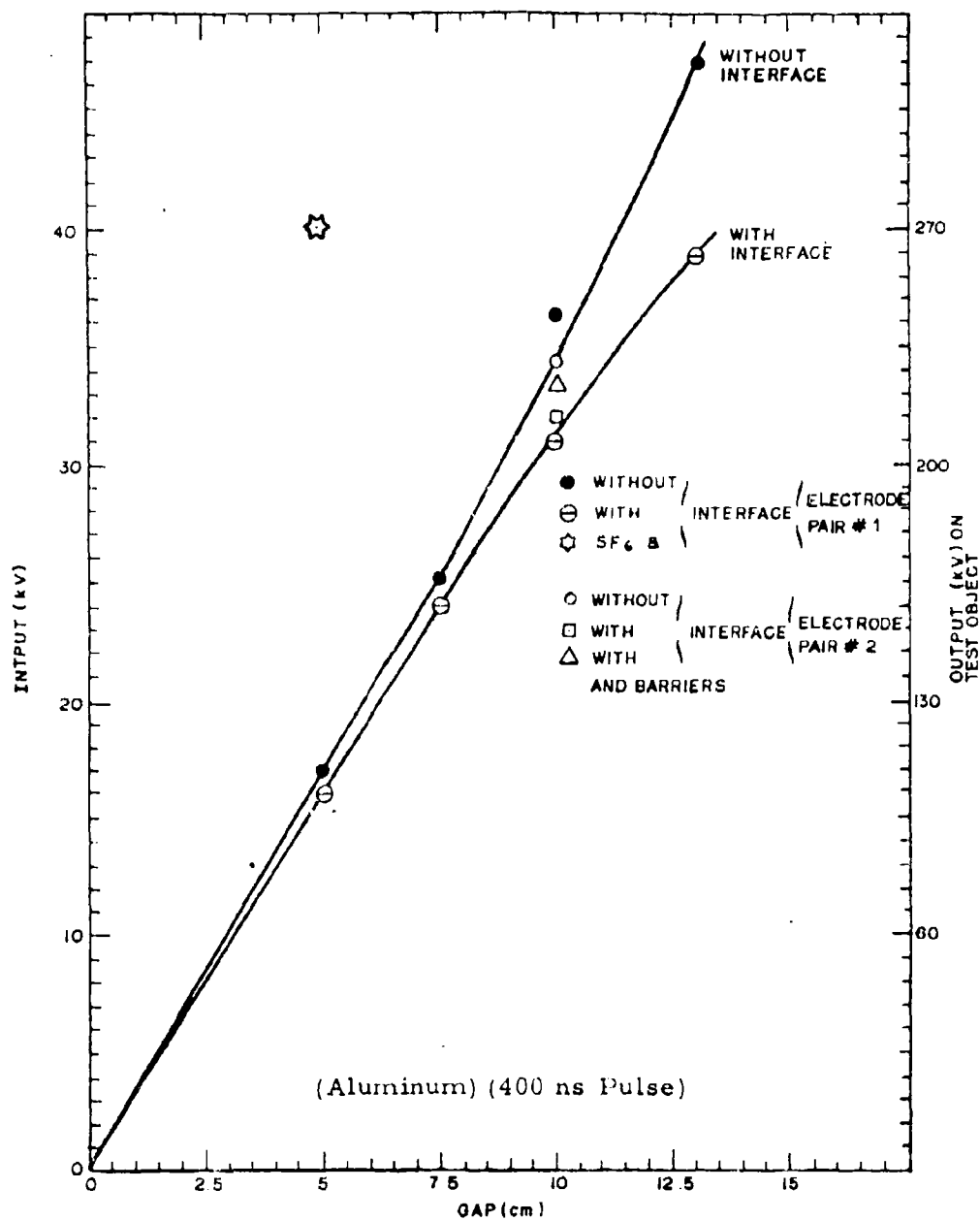
Figure 4.103 Test results of negative polarity on electrodes.
