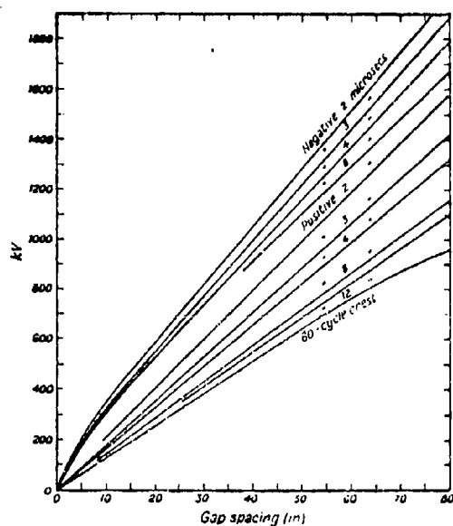
Figure 4.59 Positive and negative impulse voltage characteristics of rod-to-plane gap.
