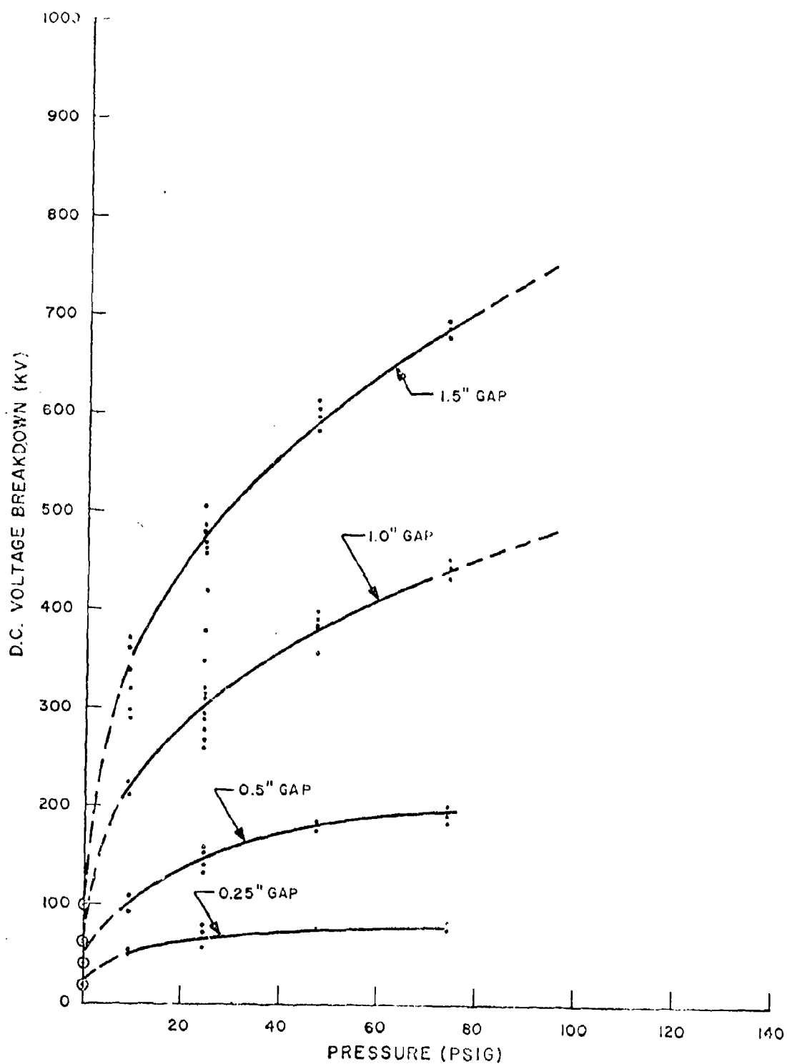
Figure 4. 25 dc voltage breakdown versus gauge pressure of \text{SF}_6 for 12 inch diameter brass parallel plane electrodes at gap spacings of 0.25 inch, 0.5 inch, 1.0 inch, and 1.5 inch.
