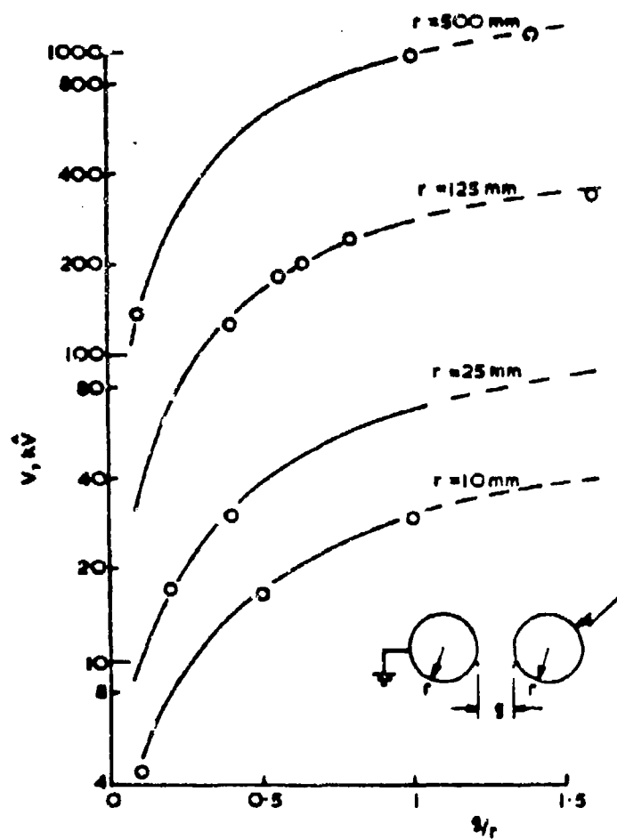
Figure 4.104 Sphere/sphere, air, 1 atmosphere. — B.S. 358:1960, o estimated.
