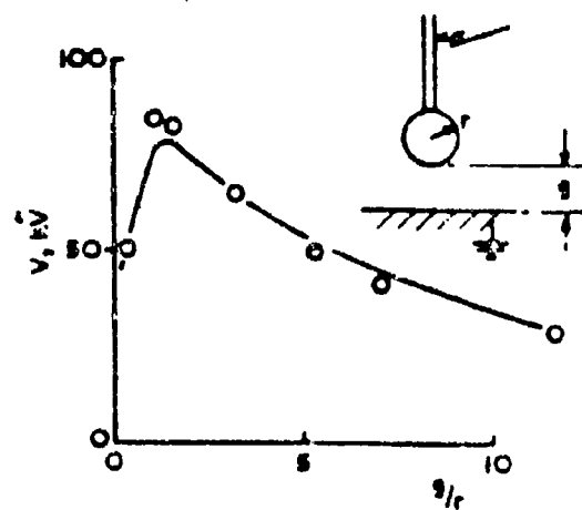
Figure 4.105 Sphere/plane, air, 1 atmosphere r = 80 mm. — experimental, o estimated.
