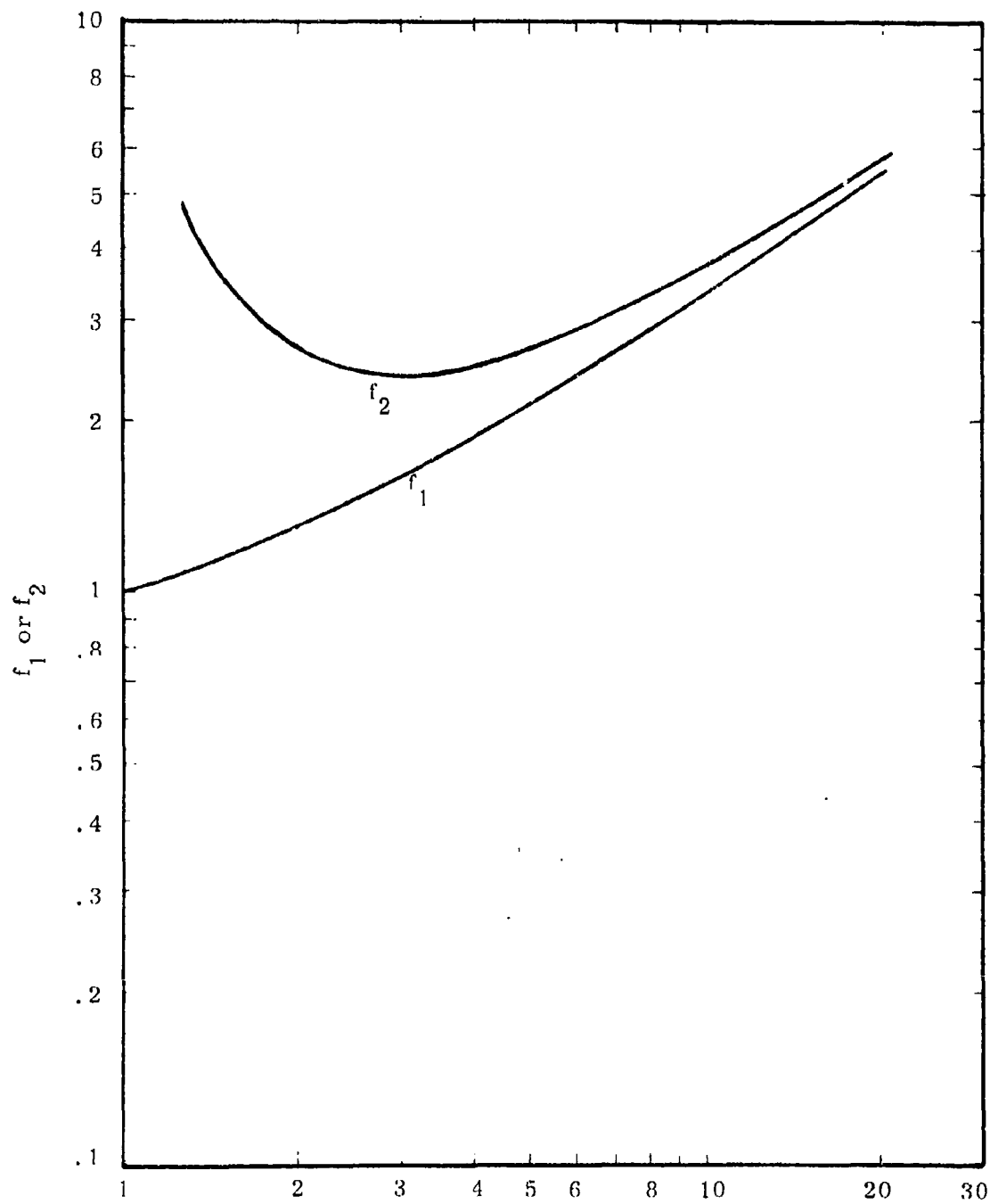
Figure 2.5 Field Enhancement Factors for Cylinder-Plane Geometry
