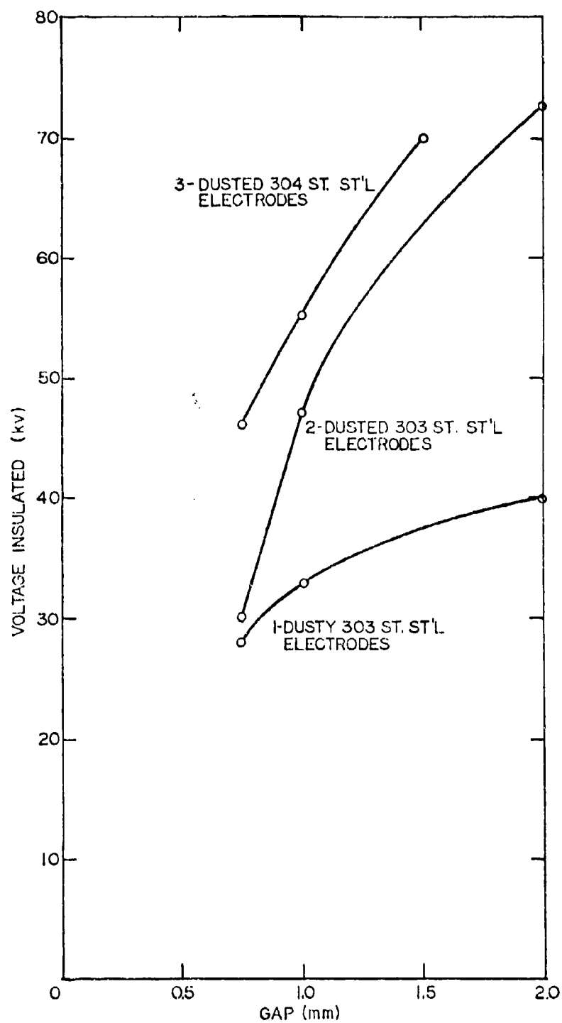
Figure 7.5 Voltage insulated vs gap for 303 & 304 stainless steel electrodes.
