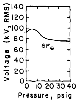
Figure 4.56 Breakdown voltage, nonuniform field, 1/5 inch rod.
