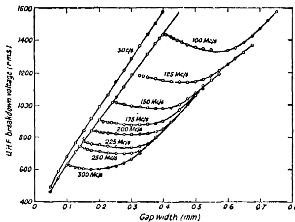
Figure 4.36 Variation of breakdown voltage with gap length between plates in air at different frequencies.
