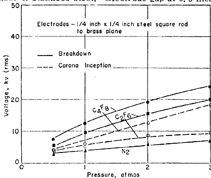
Figure 4.78 Corona inception and breakdown voltages versus pressure at power frequency. Gap spacing 0.1 inch.
