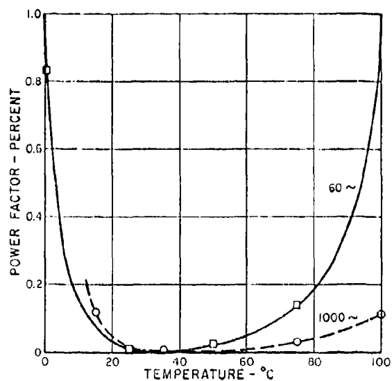
Figure 5.4 The effect of temperature on the dissipation factor of a typical European transformer oil over a range of frequency (cps).
