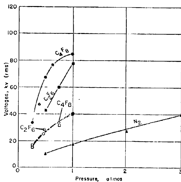
Figure 4.81 Corona inception and breakdown voltages versus pressure. Gap spacing 1.0 inch.
