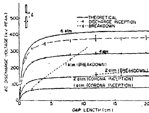
Figure 4.50 ac breakdown or corona inception voltage for gap C (10 mm diameter rods).
