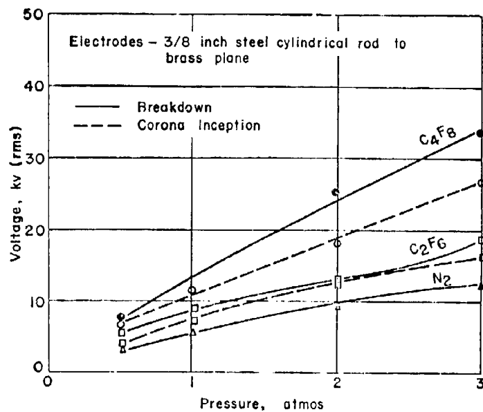
Figure 4.80 Corona inception and breakdown voltages versus pressure. Gap spacing 0.1 inch.
