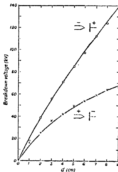
Figure 4.13 dc breakdown voltage curves for air between a 30^\circ conical point and a plane (atmospheric pressure).
