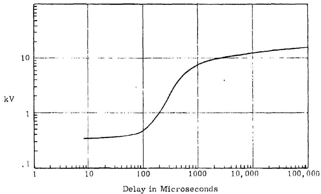
Figure 9.2 Arc recovery strength in N_2 at 1 atmosphere.
