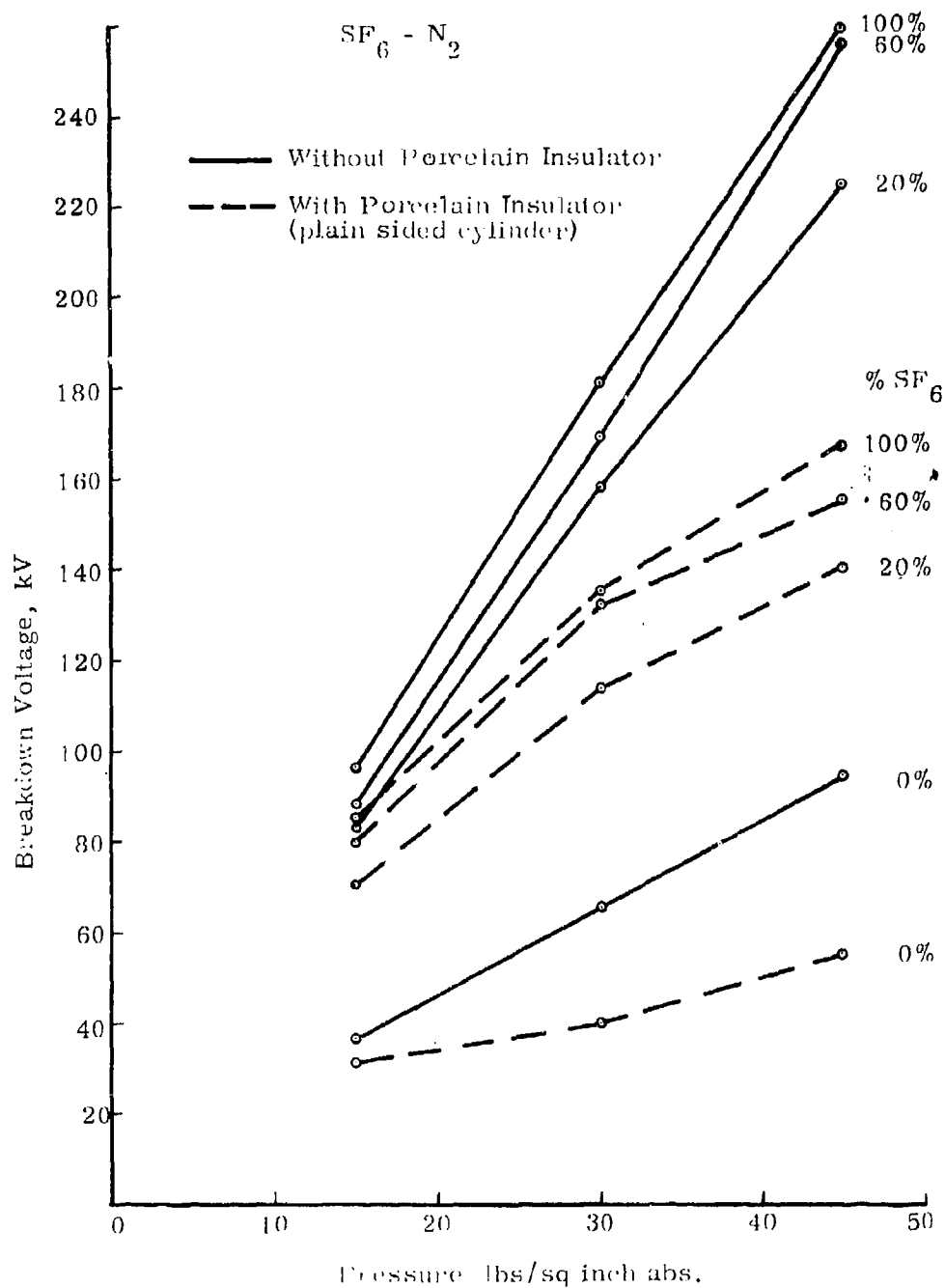
Figure 4.64 Negative impulse breakdown versus pressure. Uniform field 1 cm gap. No radius.
