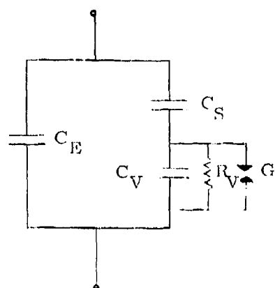
(a) Equivalent circuit of sample with a void present.
