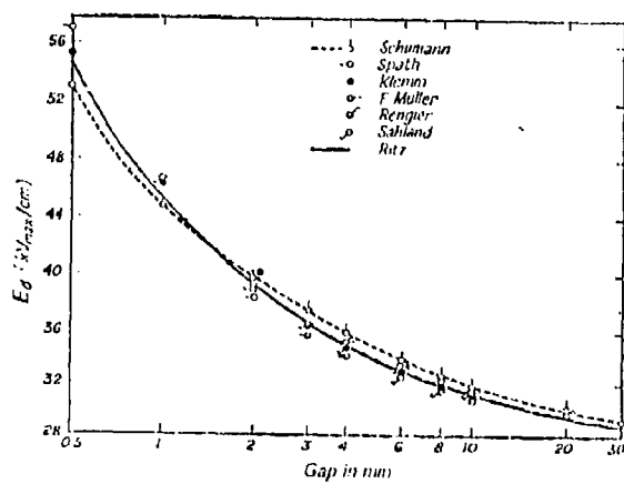
Figure 4.2 Breakdown voltage gradient in air at 1 atm, as a function of gap length between parallel plates.
