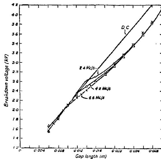
Figure 4.35 Breakdown voltage curves in nitrogen as a function of gap length between spheres of 2.0 cm diameter.
