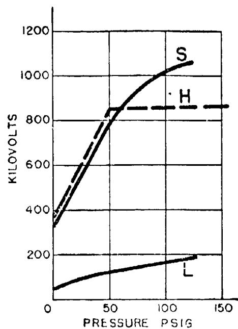
Figure 4.112 Negative inner conductor, SF 6 .
