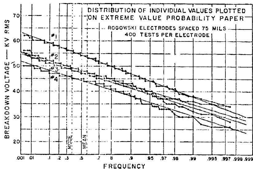
Figure 5.13 Breakdown voltage distributions of transformer oil for electrodes of four different areas.
