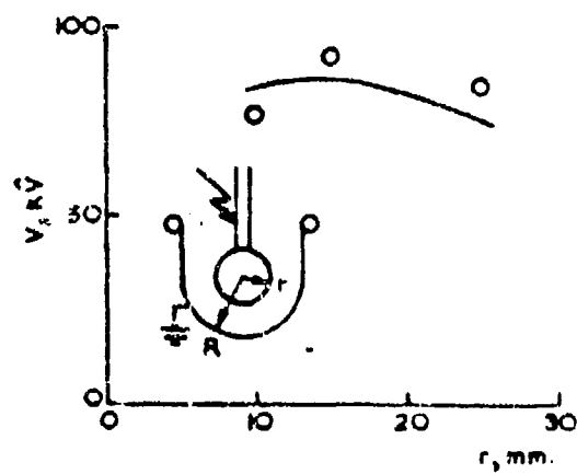
Figure 4.109 Concentric sphere/hemisphere, \text{SF}_6 , 1 atmosphere, R = 38.1 \text{ mm} . — experimental, o estimated.
