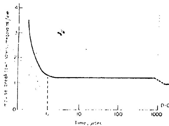
Figure 5.10 Breakdown strength of liquids as a function of applied pulse length.
