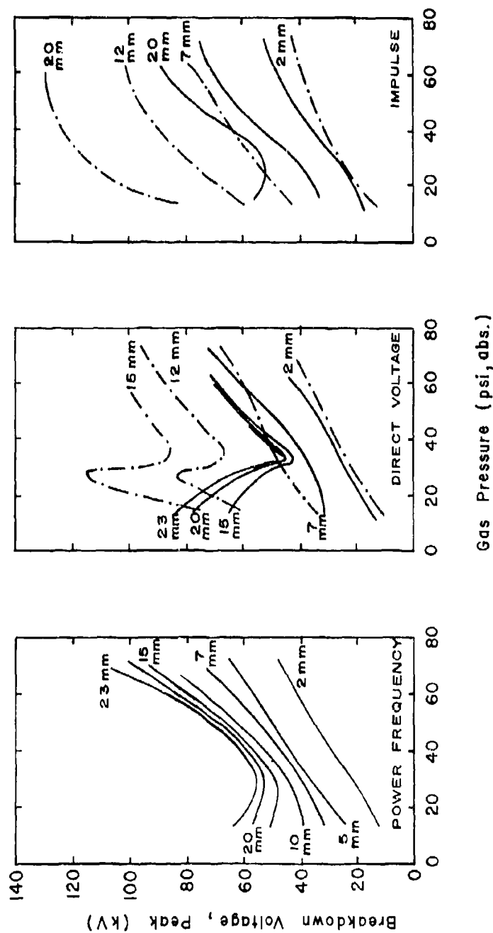
Figure 4.92 Breakdown voltage with difluorodichloromethane and non-irradiated point-sphere electrodes.
