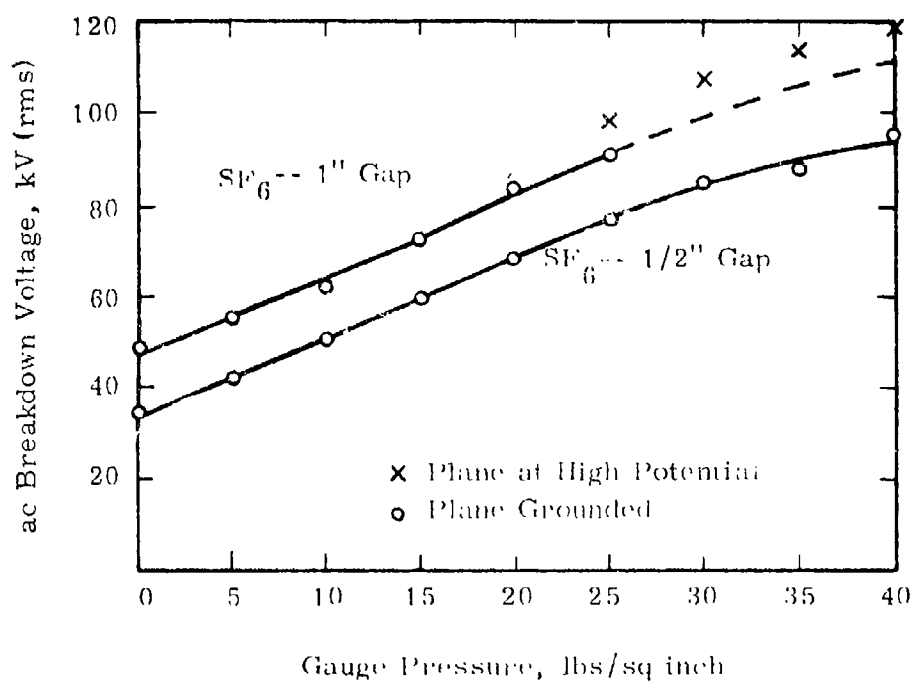
Figure 4.44 60-cycle breakdown voltages of SF 6 at 100° C as a function of pressure. Electrodes: 0.5 inch stainless steel spheres to 3 inch diameter plane.
