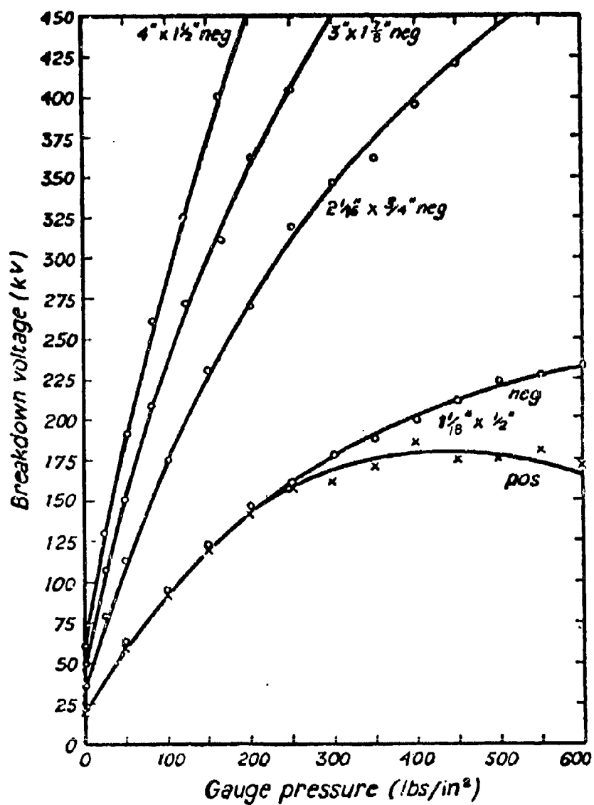
Figure 4.10 Breakdown voltage curves for coaxial cylinders in compressed air. The cylinder diameters, and the inner cylinder diameter, are shown.
