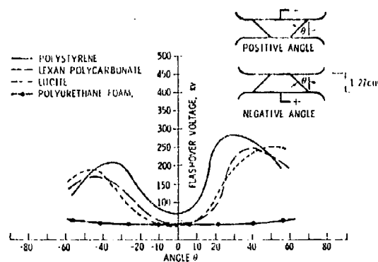
Figure 7.28 Flashover voltage versus angle \theta for some insulators. Pulse risetime about 5 \mu s.
