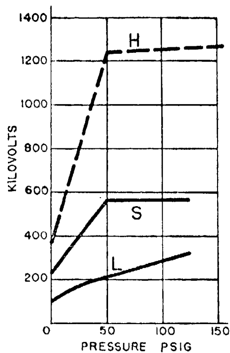
Figure 4.113 Positive inner conductor, SF 6 .
