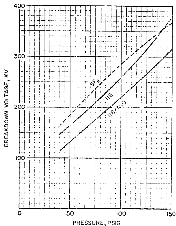
Figure 4.77 Breakdown voltage with SF 6 , Freon 116, and Freon 116/N 2 O (90/10 by wt) in a uniform field as a function of pressure in a steel tube, 36 inches long and with an ID of 20 inches. The electrodes were discs 4 inches in diameter and made of stainless steel. Electrode gap at 0.5 inches.
