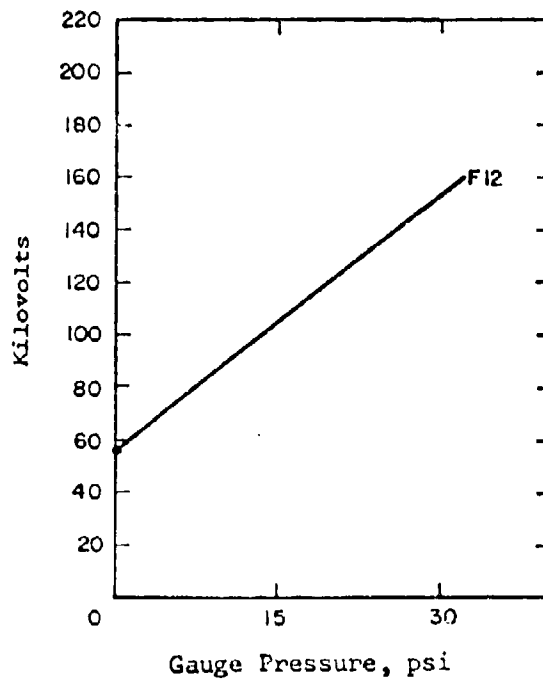
Figure 4.85 Impulse dielectric strength of Freon 12, tested between two 1 inch diameter spheres spaced 1/4 inch.
