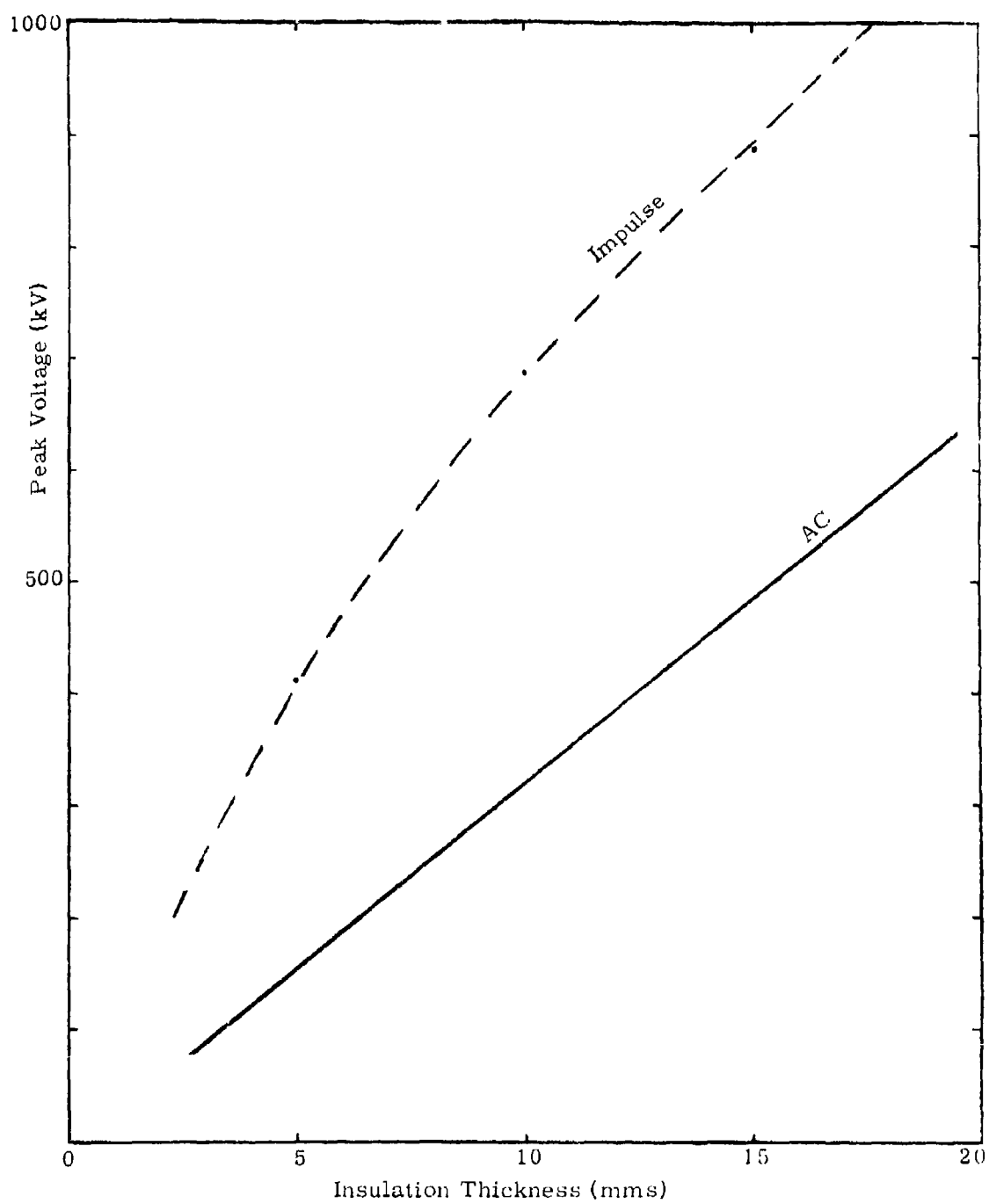
Figure 6.7 Breakdown voltage versus insulation thickness for polyethylene cable (27) (two layers extruded in tandem).
