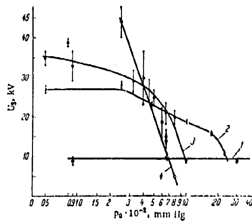
Figure 12.2 Dependence of the spontaneous breakdown voltage ( U_g ) of a partitionless spark gap on the initial pressure ( p_0 ) for various interelectrode spacings. 1) 5; 2) 15; 3) 25; 4) 35 mm.
