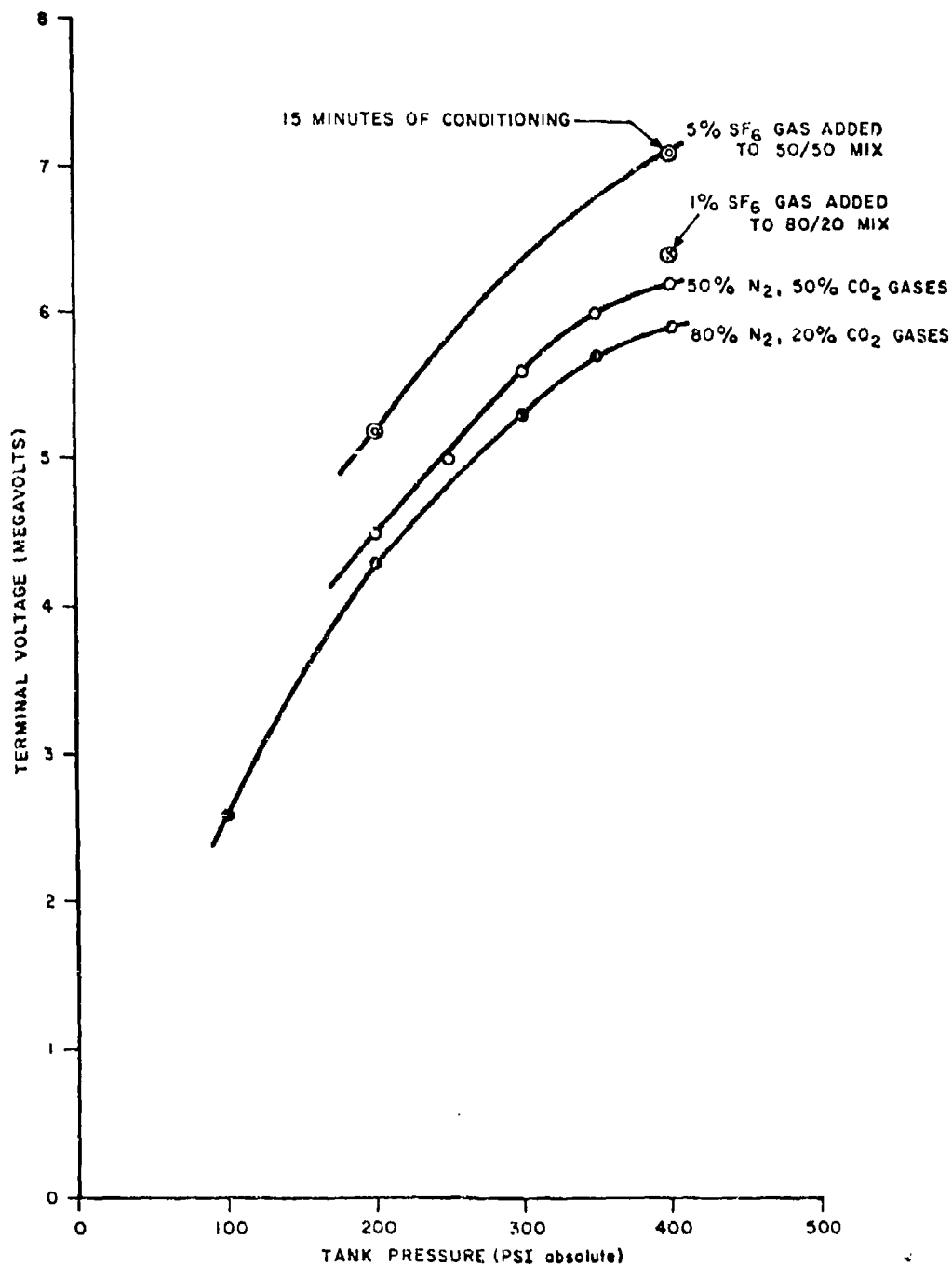
Figure 4. 23 Preliminary dc breakdown characteristics for \text{SF}_6 , \text{N}_2 and \text{CO}_2 gas mixtures between concentric cylinder electrodes with a gap spacing of 58.5 cm
