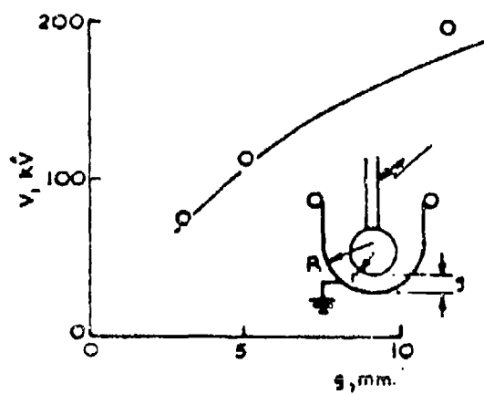
Figure 4.110 Eccentric sphere/hemisphere, \text{SF}_6 , 3 atmospheres, r = 15 \text{ mm} , R = 38.1 \text{ mm} . — experimental, o estimated.
