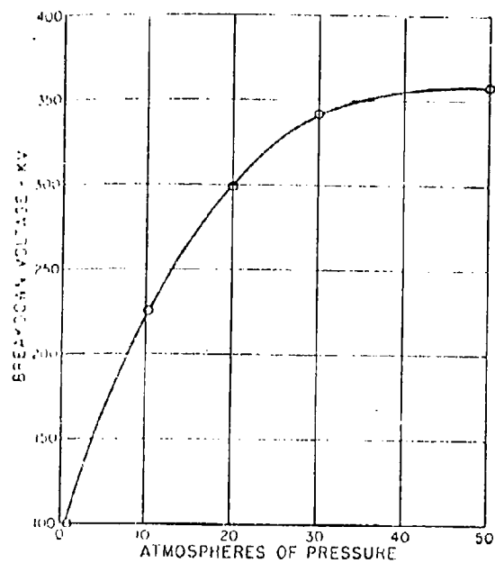
Figure 5.9 The effect of high values of air pressure on the breakdown voltage of mineral oil.
