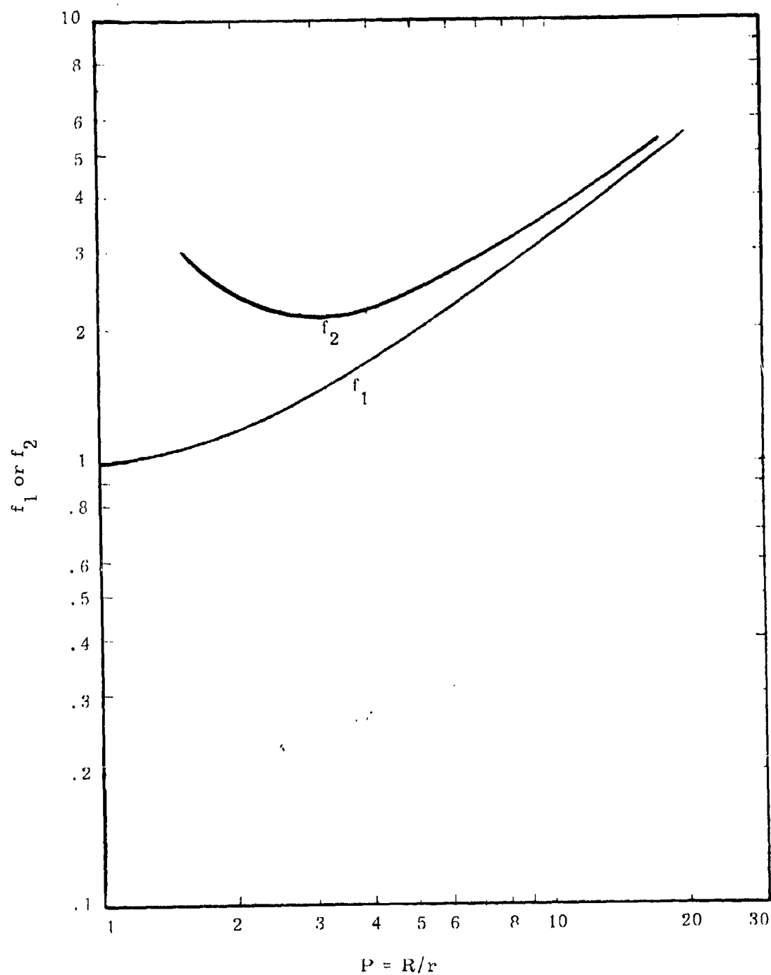
Figure 2.6 Field Enhancement Factors for Cylinder Passing Through Radiused Hole
