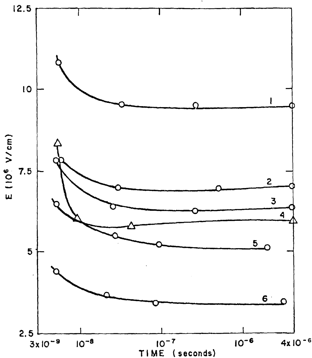
Figure 6.13 Variation of the dielectric strength of styroflex (1), teflon (2), mica (3), lucite (4), polystyrene (5), and bulk teflon (6), with the voltage rise time; uniform field (Ref. Mel'nikov 45).
