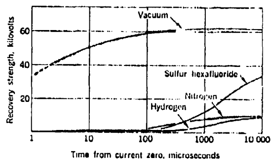
Figure 12.1 Recovery strength for vacuum and gas; 1600 amperes, 6.35 mm gap, gas pressure 1 atmosphere.
