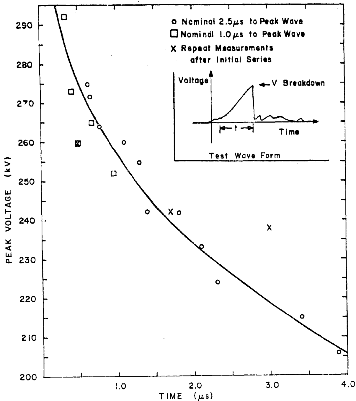
Figure 4.65 Time and voltage dependence of breakdown under impulse conditions for uniform field stainless steel in 150 psig, 10% \text{SF}_6 , 40% \text{N}_2 , 50% Ar gas mixture - 0.58 cm gap.
