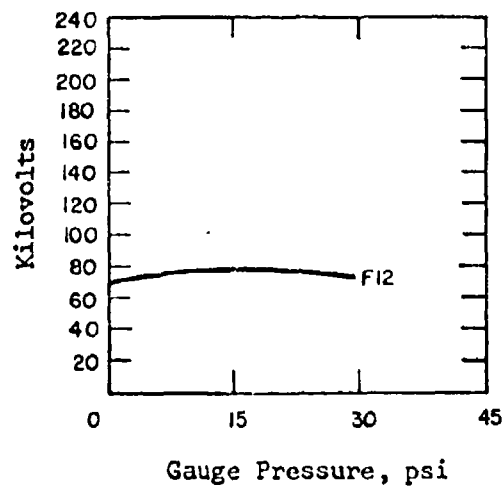
Figure 4.90 Impulse dielectric strength of Freon 12. Positive tests made between tungsten rod and 1 inch diameter sphere spaced 1 inch, 1.5/40 microseconds wave form.
