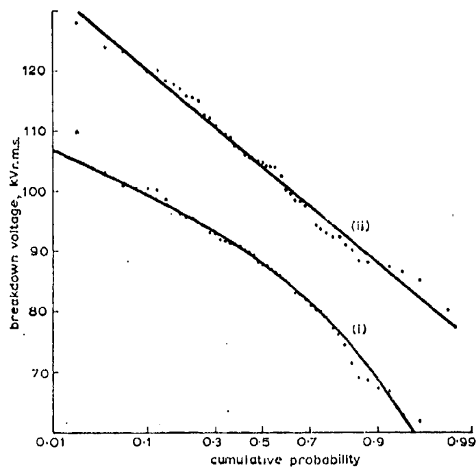
Figure 5.23 Cumulative probability for stationary and circulating-oil samples.
