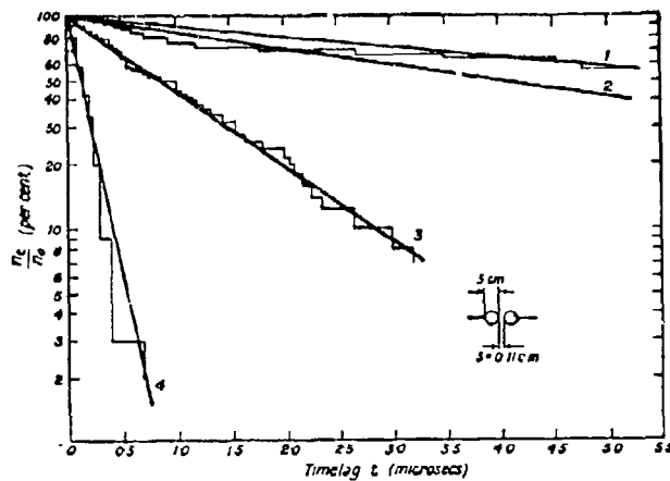
Figure 4.57 Influence of the nature of the electrode surfaces on the time-lag distribution curves for a gap of 1.1 mm between 5 cm diameter spheres. The gap is subjected to an impulse voltage of 6.5 kV, the dc breakdown voltage being 5.0 kV.
