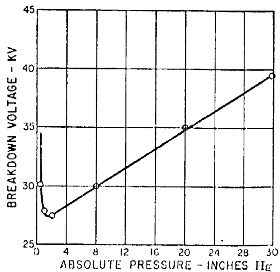
Figure 5.8 The breakdown voltage of transformer oil as affected by the absolute pressure.
