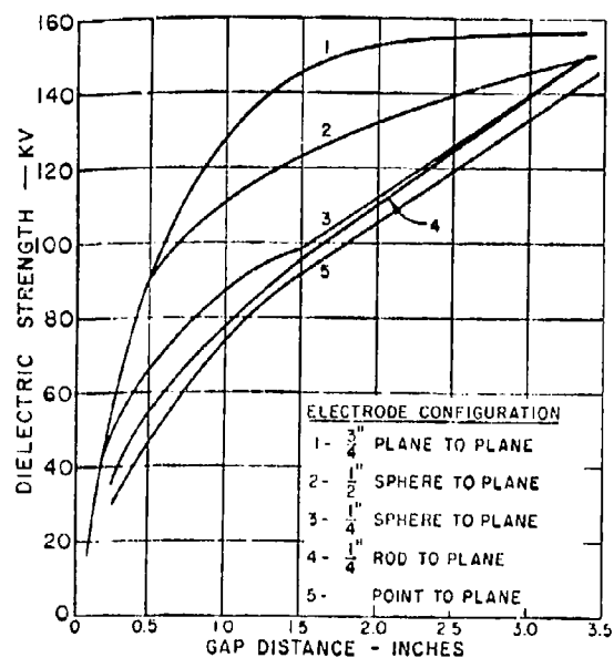
Figure 4. 67 The dielectric strength-gap distance relation for sulfur hexafluoride gas as a function of the electrode configuration measured at atmospheric pressure.
