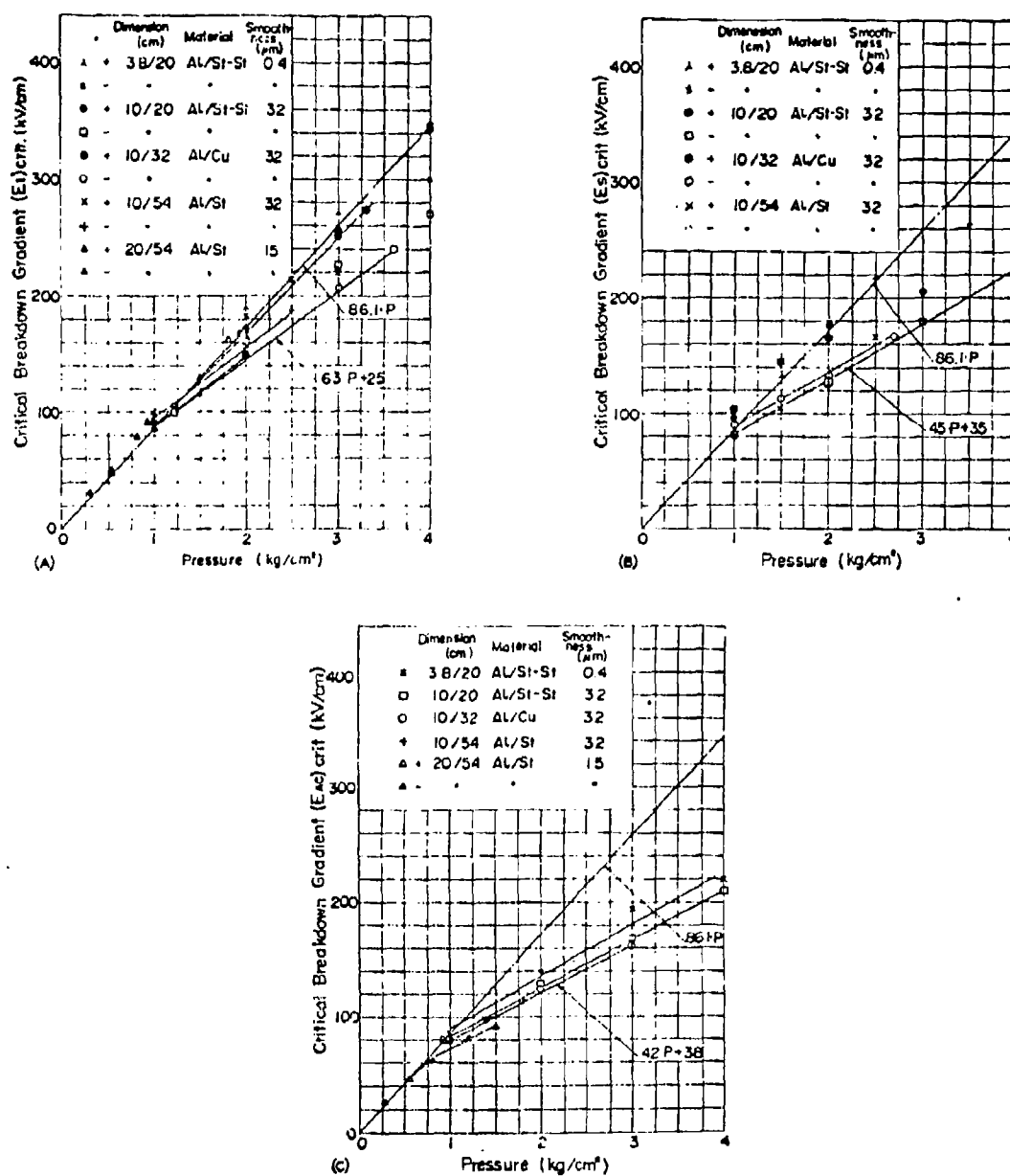
Figure 4.69 Critical breakdown gradient E_{crit} between coaxial cylinder electrodes as a function of pressure (corrected to 20° C).
