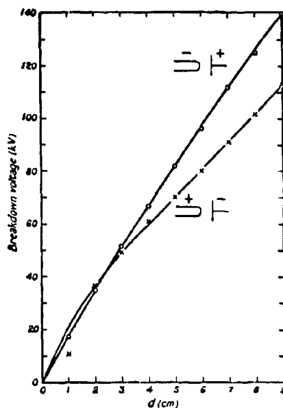
Figure 4.14 dc breakdown voltage curves for air between a hemispherically-ended rod, of 0.4 cm diameter, and a plane (atmospheric pressure).
