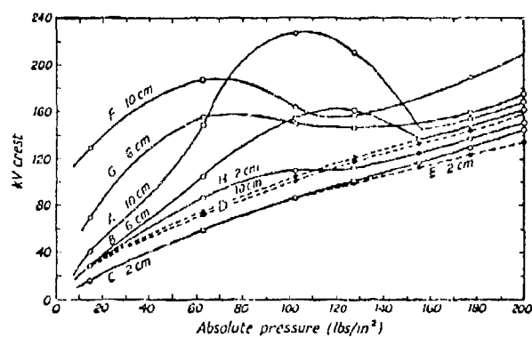
Figure 4. 40-60 c/s and impulse breakdown voltage curves between 0.5 in. square-cut rods in compressed nitrogen. The figures against the curves give the gap lengths.
