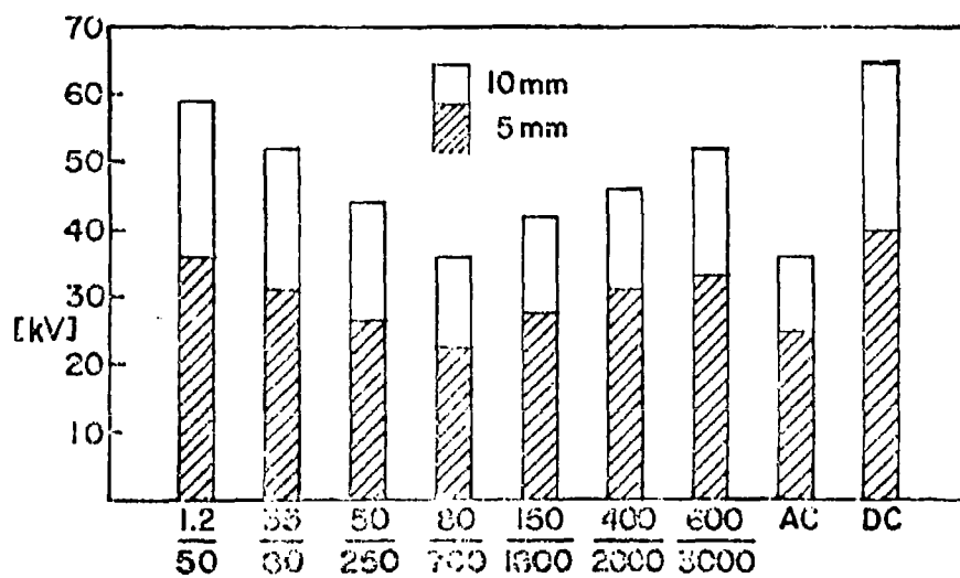
Figure 7.24 Effect of surge front duration on FO voltages. (Pressure 1 \times 10^{-5} torr sample thickness 5 mm and 10 mm).
