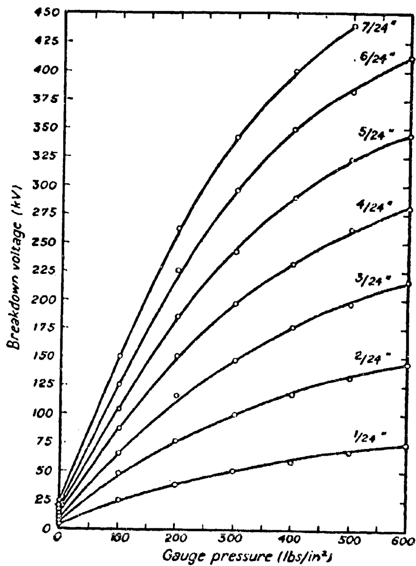
Figure 4.5 Breakdown voltages for plane electrodes in air at various constant spacings.
