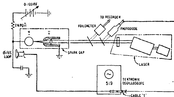
Figure 9.6 Schematic diagram of the laser-triggered switching apparatus.
