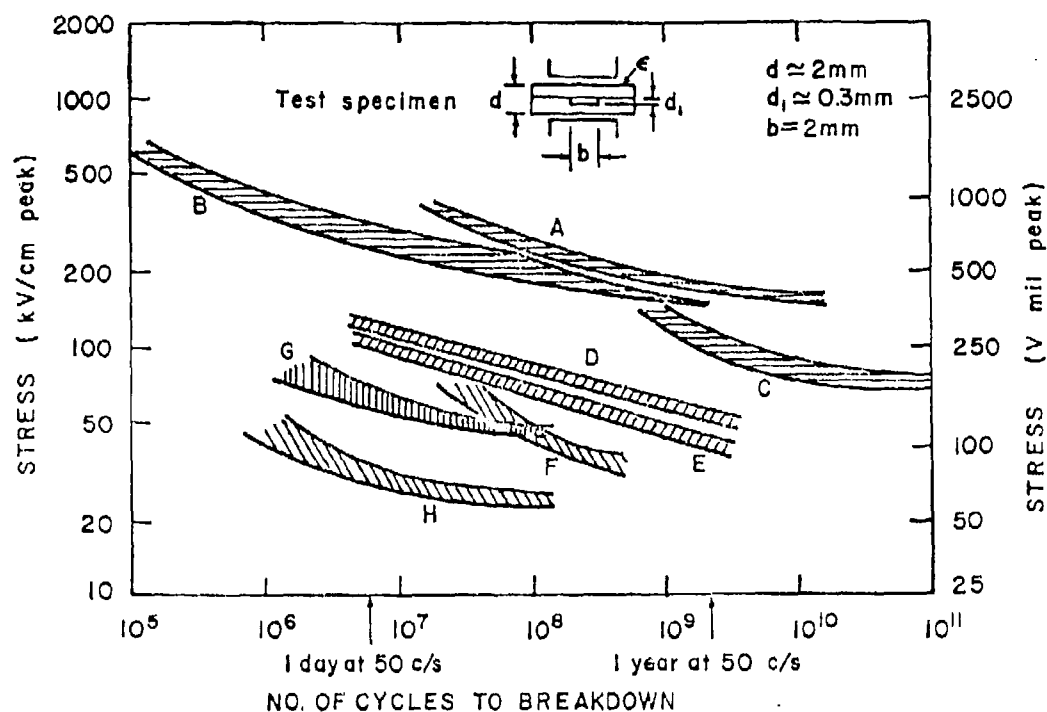
Figure 6.4 Life data for plastics with internal discharges (Ref. 15).
