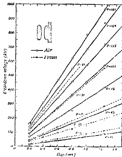
Figure 4.7 Variation of dc breakdown voltage of air and of Freon-12 with electrode separation at several absolute pressures in pounds per square inch. Uniform field.
