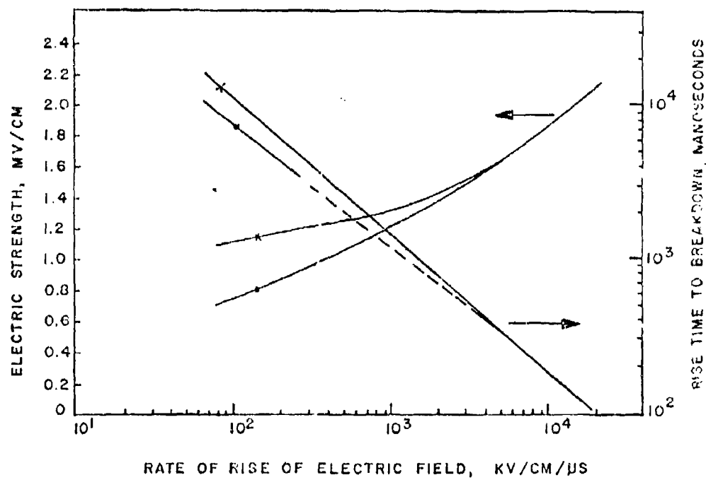
Figure 5.48 Pressure effect in oil.
