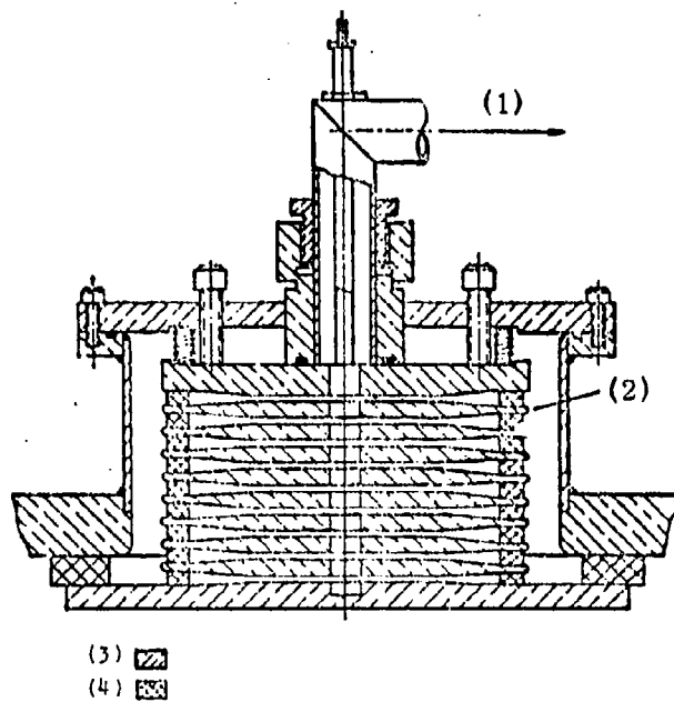
Figure 12.3 Design of sectioned spark gap.
