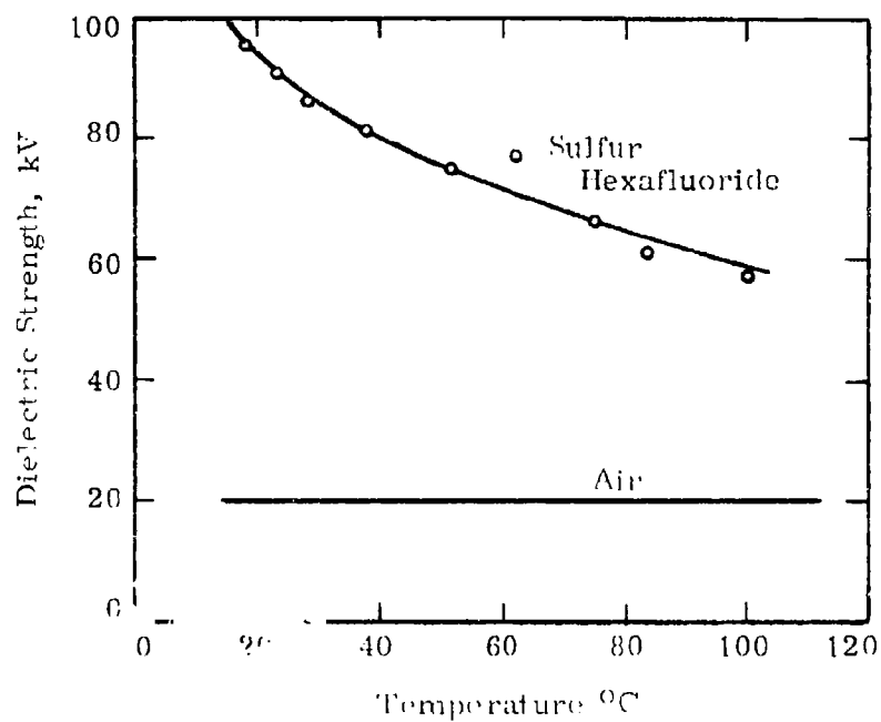
Figure 4.66 The dielectric strength-temperature relation for sulfur hexafluoride tested at atmospheric pressure.
