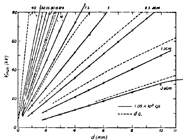
Figure 4.34 Breakdown voltage as a function of gap length between plates in compressed air for dc and 1.05 \times 10^5 c/s voltages.
