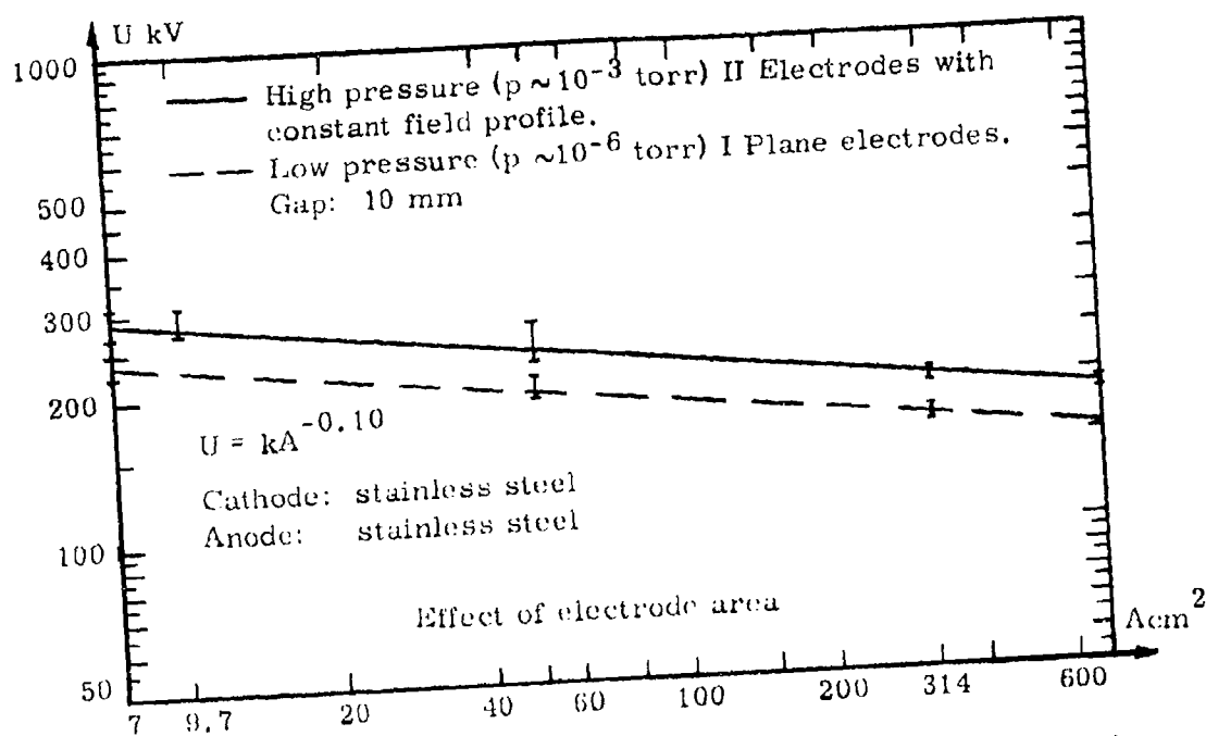
Figure 7.10 Effect of electrode areas (cathode, SS and anode SS).
