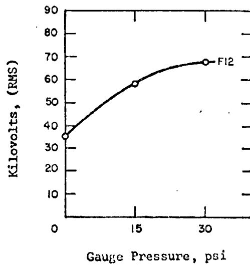
Figure 4.84 60 cycle dielectric strength of Freon 12, tested between two 1 inch diameter spheres spaced 1/4 inch.
