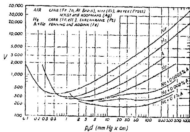
Figure 4.1 Typical breakdown voltage curves for different gases between parallel plate electrodes. p_0 is the gas pressure in mm. Hg corrected to 0° C.
