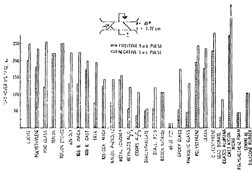
Figure 7.26 Flashover voltage for some dielectrics.
