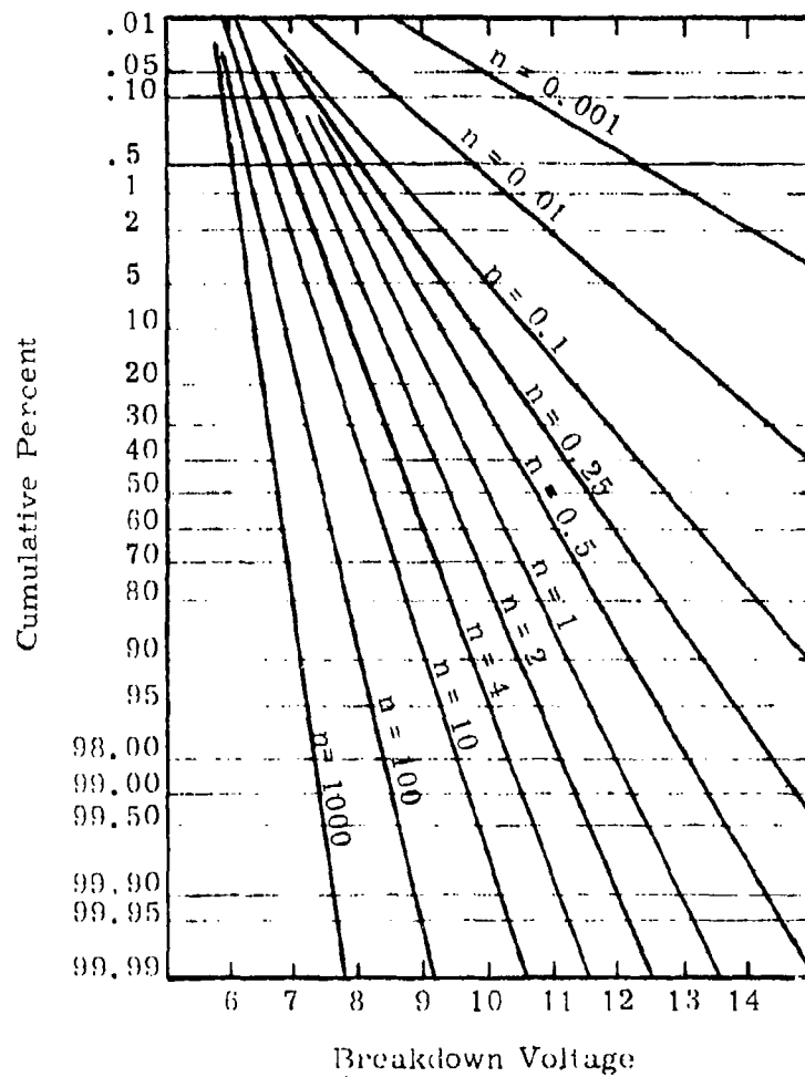
Figure 3.1 Voltage breakdown distributions for partial and multiple areas of an elemental area ( n = 1 ) when the distribution for the elemental area has an average value of ten units and a standard deviation of one unit.
