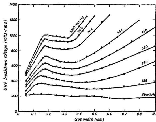
Figure 4.37 Variation of breakdown voltage with gap length between plates in air at 200 Mc/s for different gas pressures.
