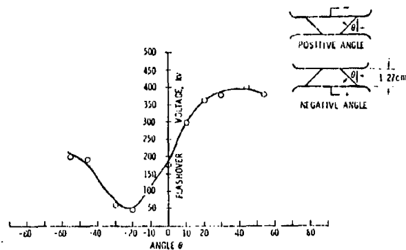
Figure 7.30 Flashover voltage versus angle \theta for lucite. Pulse risetime about 50 ns.
