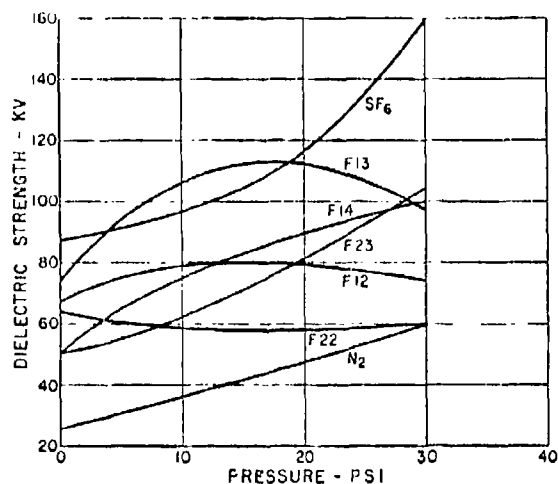
Figure 4.71 Comparing the impulse dielectric strength of fluorinated hydrocarbon gases.
