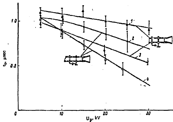
Figure 12.6 Variation of the time lag of the discharge with the voltage for negative (4) and positive (2) polarities of the high voltage electrode. Ring electrodes. (3, 1) The same for cases where electrode II is represented by a solid disk and electrode I is a disk with a hole of diameter 6 cm.
