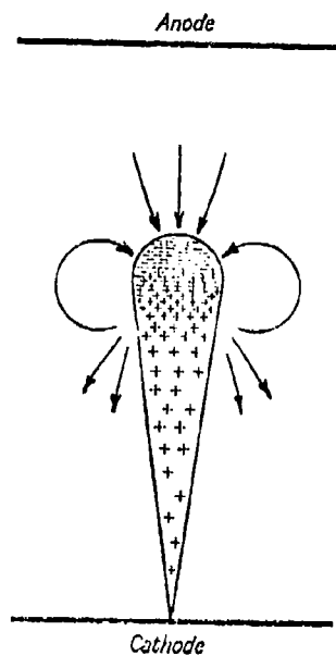
Figure 4.3 Representation of the distribution of electrons and positive ions in an electron avalanche. The arrows denote the direction of the resultant electric field surrounding the avalanche.
