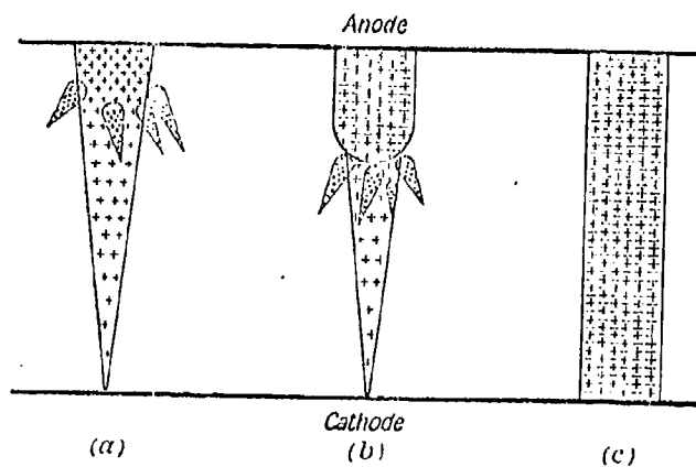
Figure 4.4 Transition from an electron avalanche to a streamer and the subsequent growth of a streamer across the gap.
