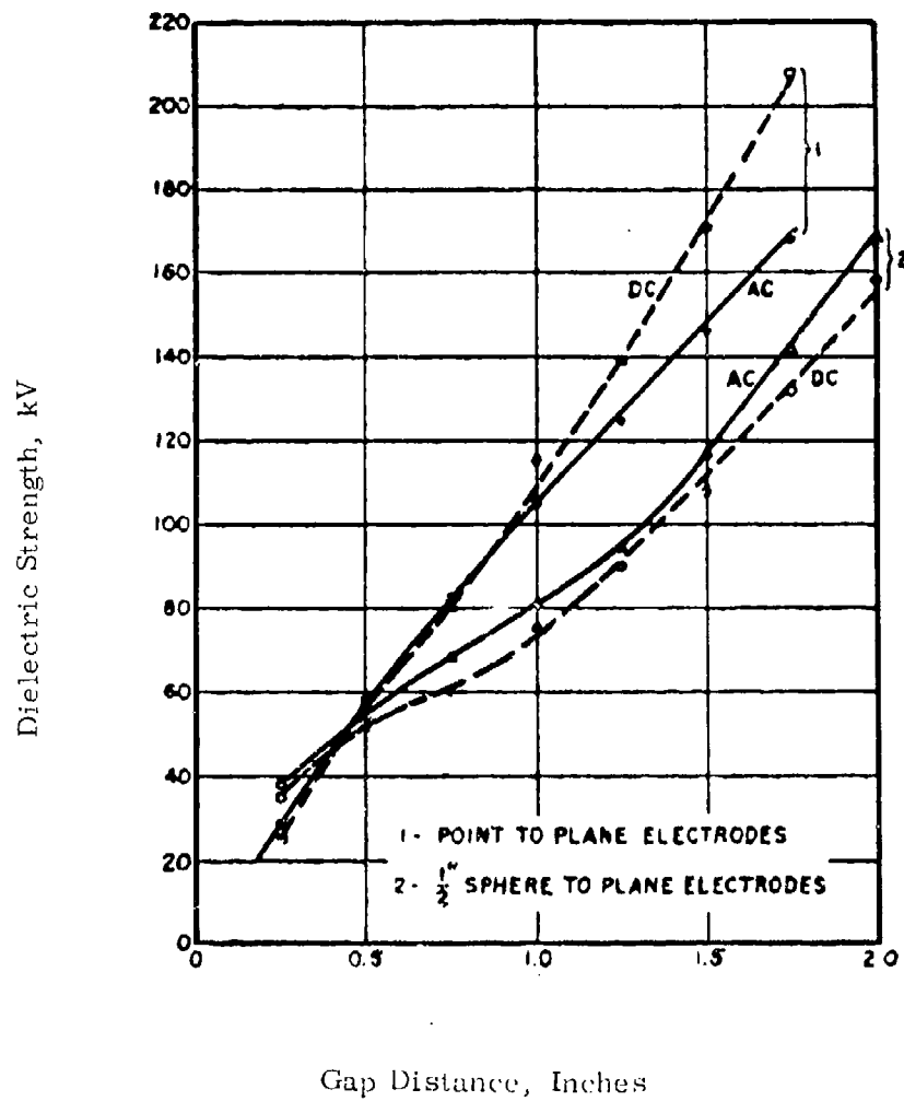
Figure 4.27 The comparative dielectric strength of sulfur hexafluoride gas tested under dc and ac voltage at room temperature and pressure.
