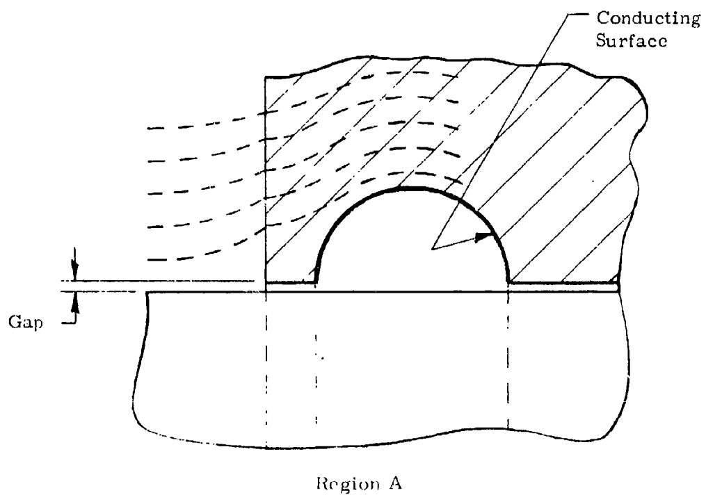
Figure 4.98 Concept of internal shielding.
