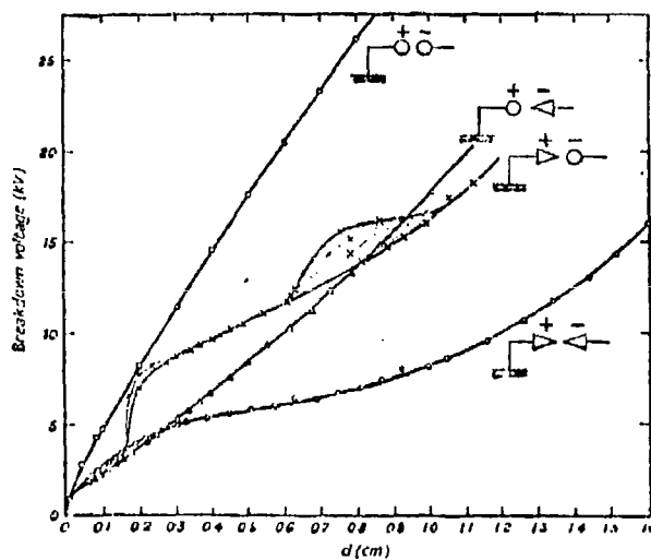
Figure 4.15 dc breakdown voltage curves in air at atmospheric pressure for various combinations of point and sphere electrodes. The sphere diameter is 5 cm. The shaded area indicates an unstable region.
