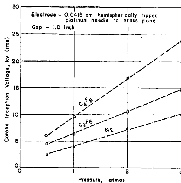
Figure 4.82 Corona inception voltages versus pressure.
