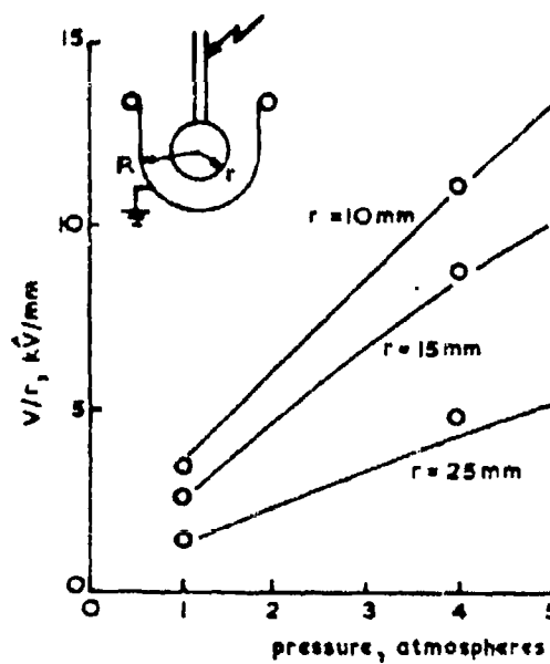
Figure 4.108 Concentric sphere/hemisphere, air, R = 38.1 mm. — experimental, o estimated.
