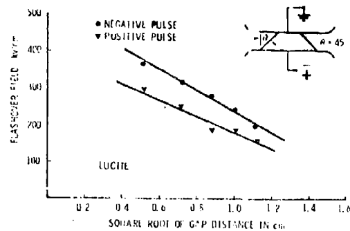
Figure 7.27 Flashover strength versus gap distance for lucite. Pulse risetime about 5 \mu s.
