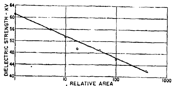
Figure 5.1 The electrode area effect on the dielectric strength of transformer oil.
