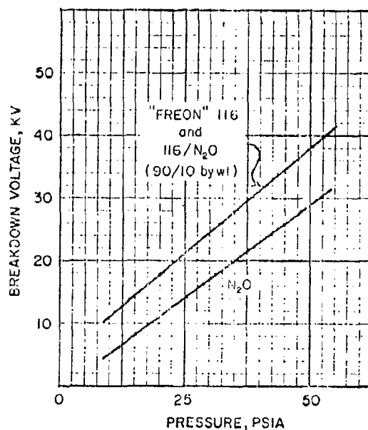
Figure 4.76 Breakdown voltages measured in a Seavy cell, ASTM D-2477-66T. The electrode gap was 0.1 inch, steel sphere (0.75 inch diameter) to brass plane (1.5 inch diameter). In this test pure Freon 116 and a mixture of Freon 116 and nitrous oxide (90/10 by wt) gave equivalent results.
