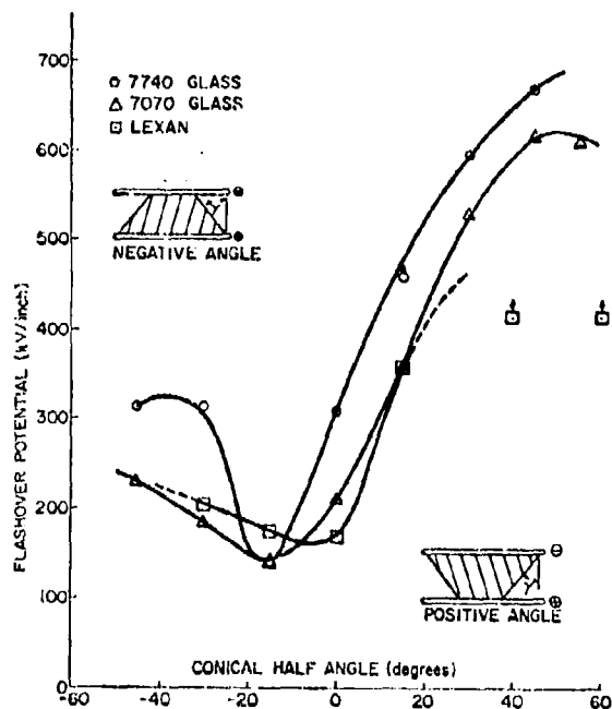
Figure 7.25 The flashover strength of glass and lexan as a function of geometry.
