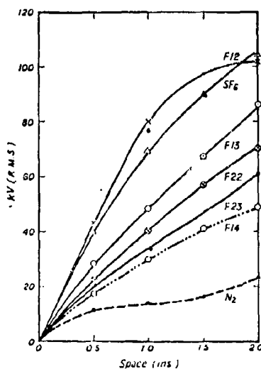
Figure 4.52 Breakdown voltage curves for various gases between a hemispherically-ended rod, of 0.1 inch diameter, and a sphere of 1.0 inch diameter. The gas pressure is 1 atm.
