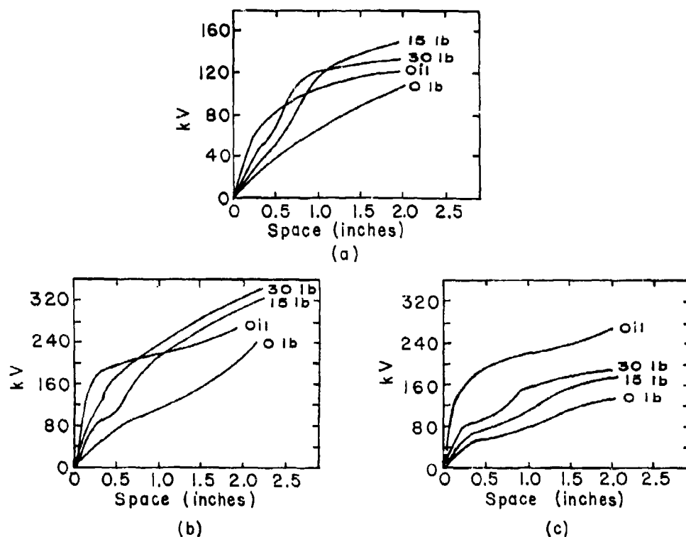
Figure 4.53 Breakdown voltage curves for \text{SF}_6 at various pressures as a function of the spacing between a hemispherically-ended rod of 0.1 inch diameter and a sphere of 1.0 inch diameter. (a) 60 Hz. (b) Negative rod-plane (impulse). (c) Positive rod-plane (impulse).
