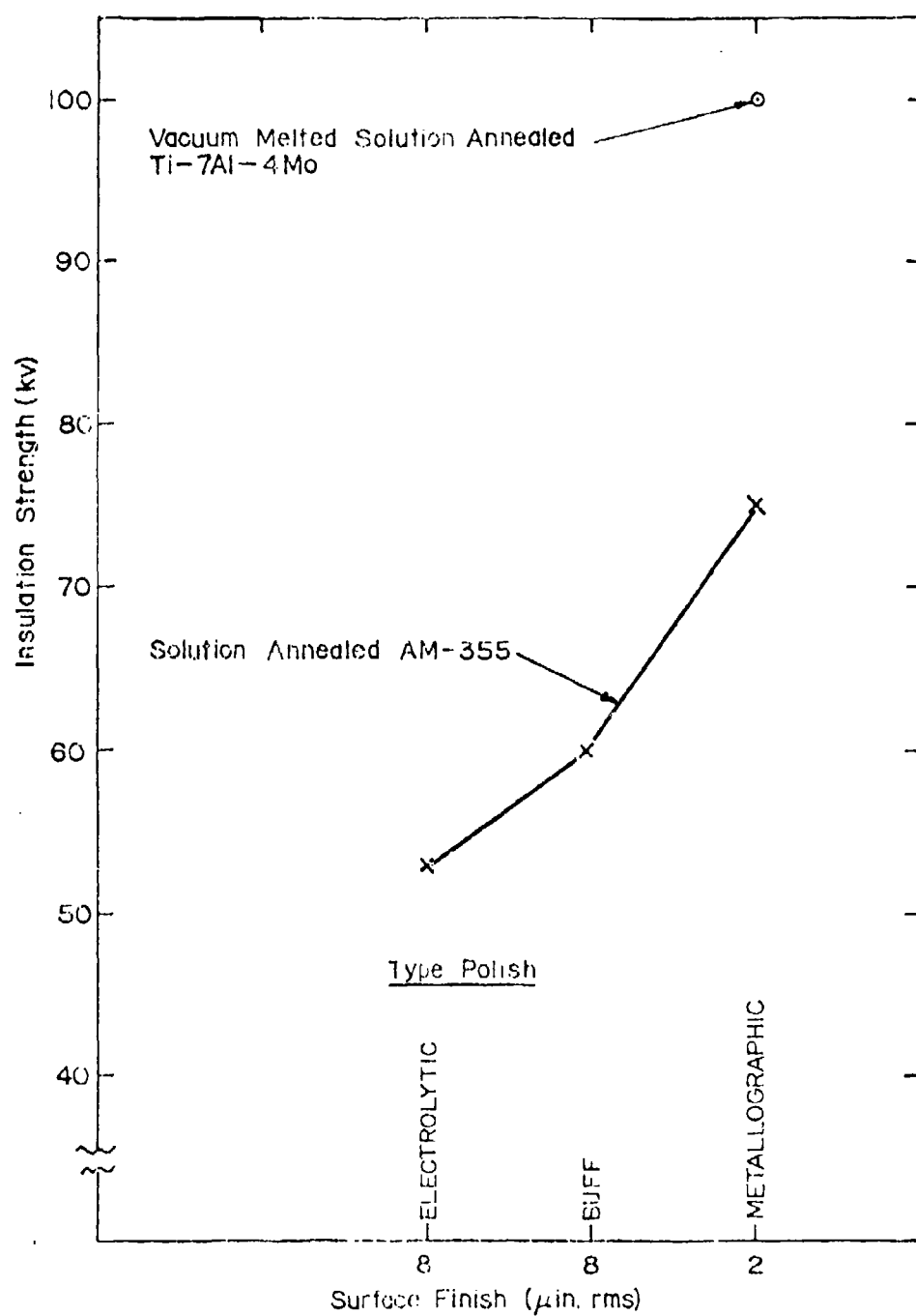
Figure 7.6 Insulation strength as a function of electrode surface finish
