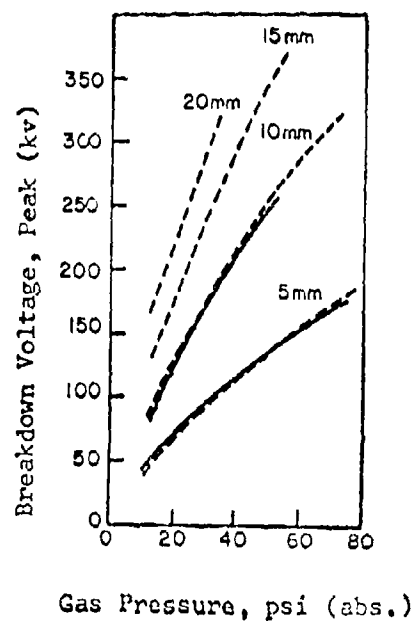
Figure 4.86 Breakdown voltage between 5 cm diameter spheres for Freon 12 as a function of pressure. Gaps as noted.
