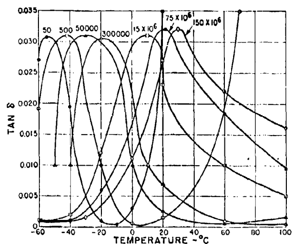
Figure 5.4 The effect of temperature on the dissipation factor of a typical European transformer oil over a range of frequency (cps).
