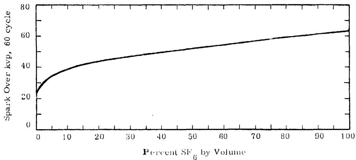
Figure 4.45 Effect of air on dielectric strength of SF 6 .
