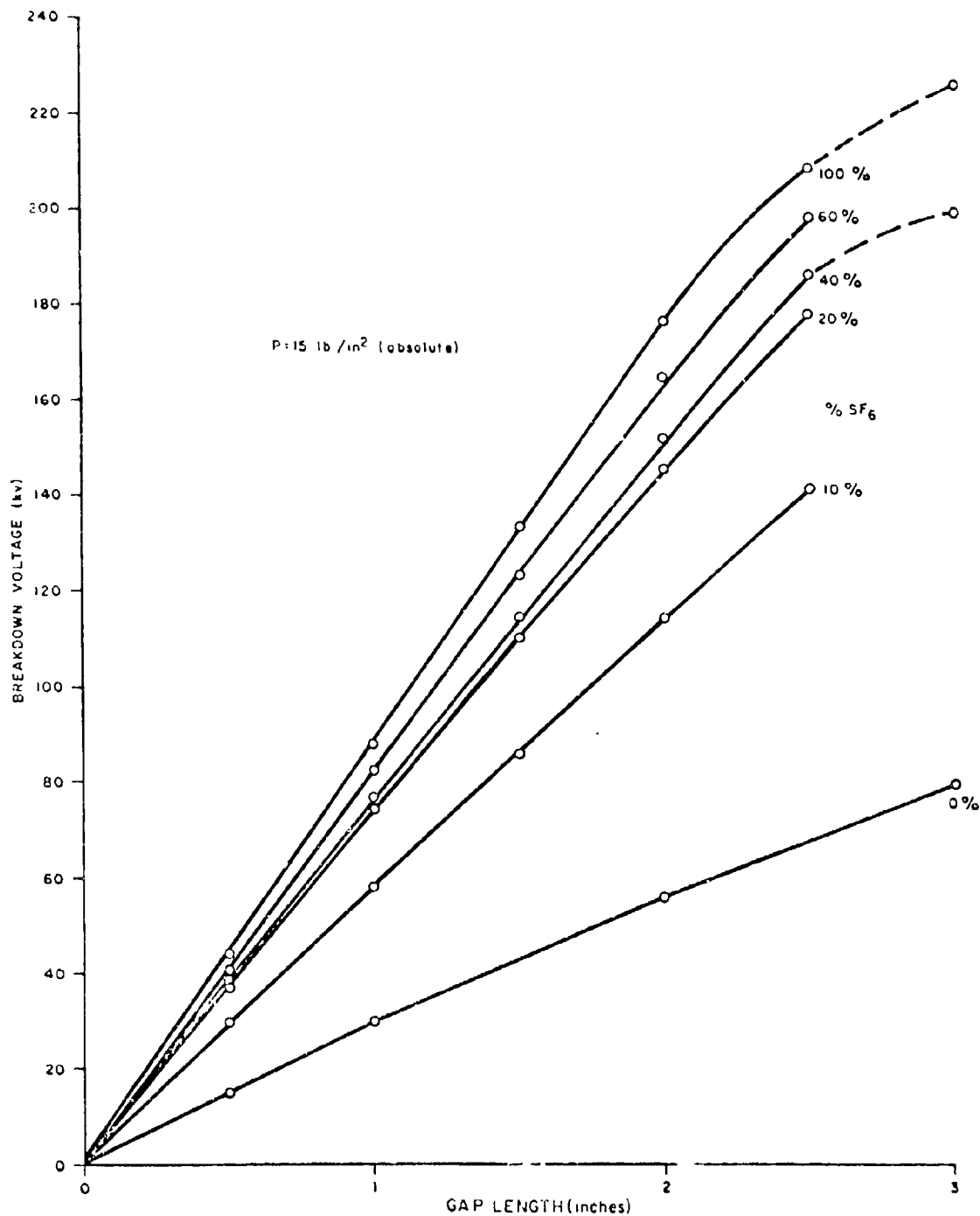
Figure 4.21 dc breakdown versus gap length in \text{SF}_6 - \text{N}_2 mixtures (15 cm diameter uniform field electrodes).
