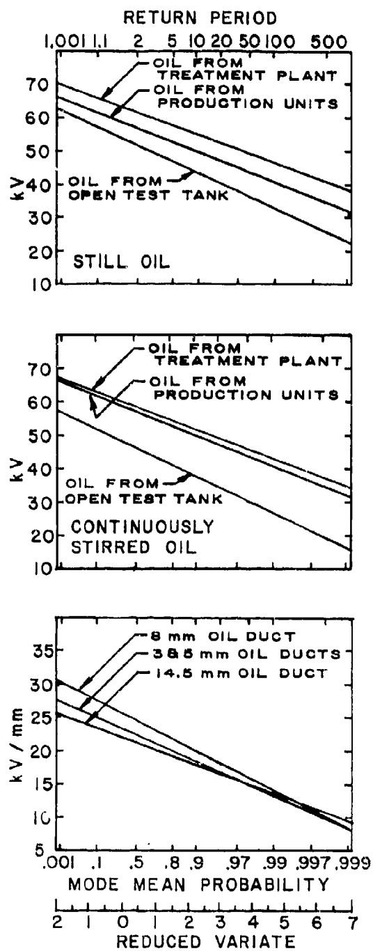
Figure 5.19 Breakdown strengths under various conditions.
