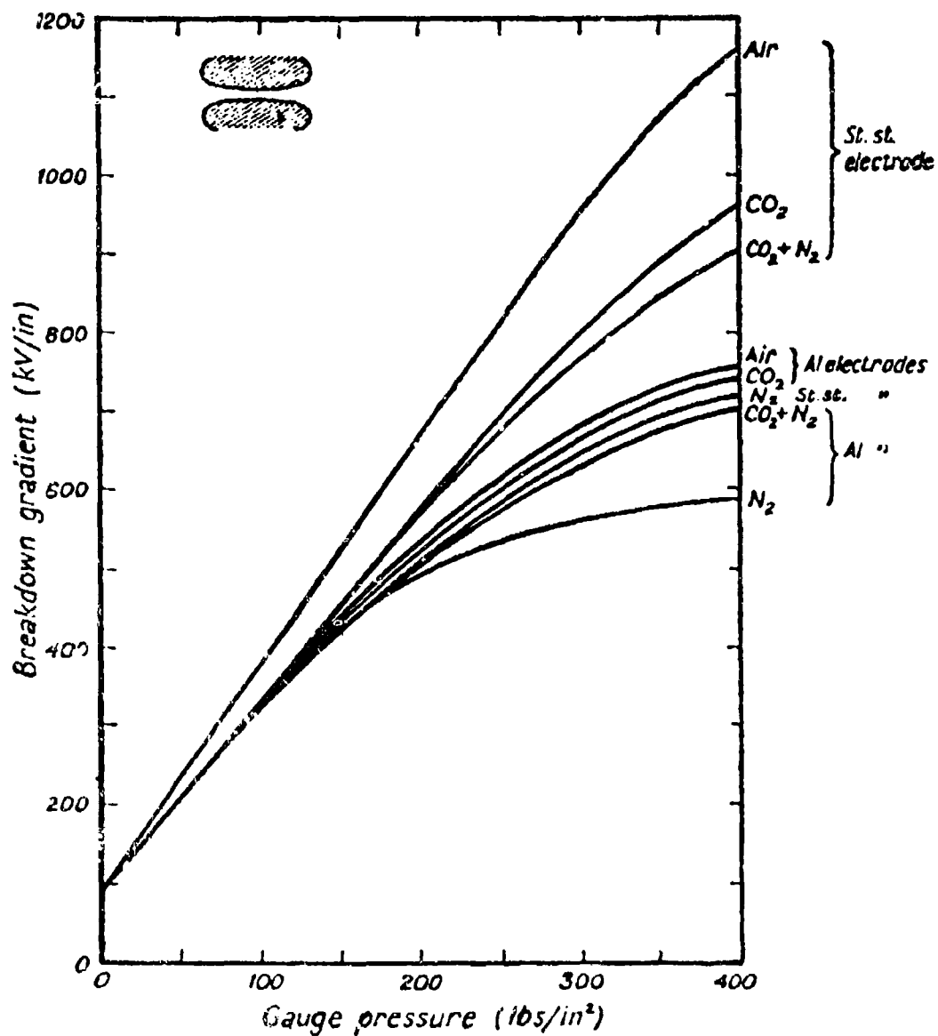
Figure 4.6 Breakdown voltage gradients for several gases at high pressures for uniform fields between stainless-steel electrodes and between aluminum electrodes. (Gradient is the mean values obtained from 1/4 inch, 1/2 inch and 3/4 inch gaps--no gap dependence was seen.)
