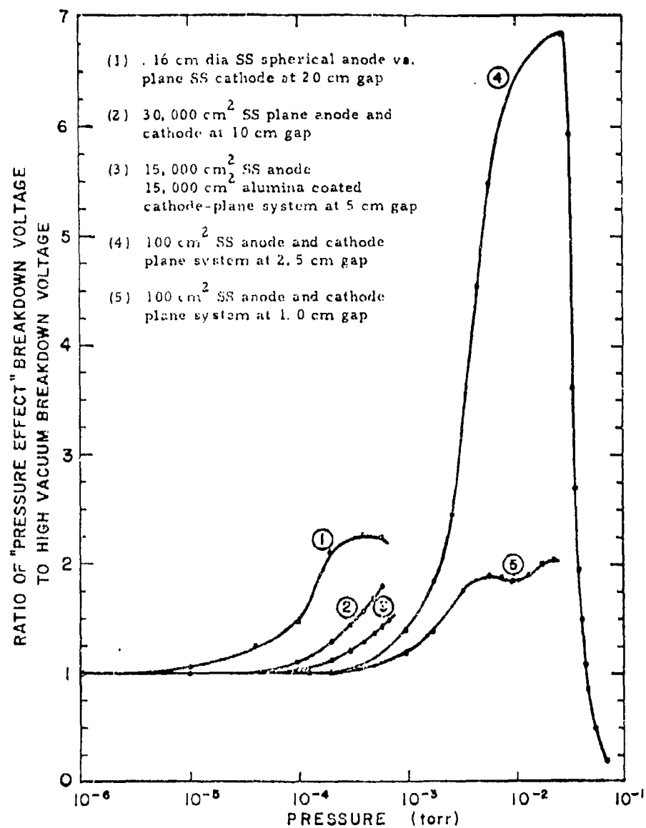
Figure 7.31 Pressure effect for various electrode systems.
