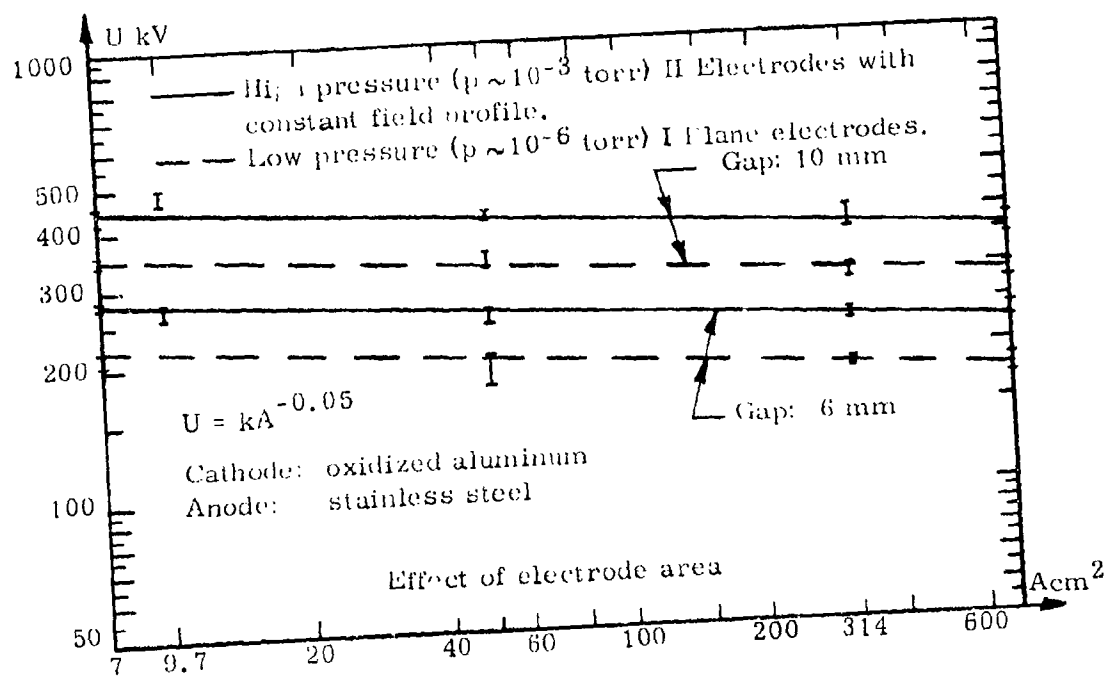
Figure 7.11 Effect of electrode areas (cathode oxidized aluminum, and anode SS).
