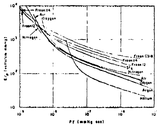
Figure 4.58 Summary of formative-time measurements in nine gases.
