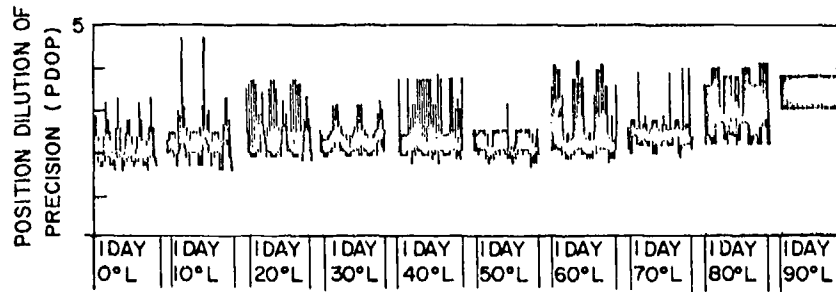
Fig. 32 — PDOP plot for a 3 \times 12 constellation inclined at 53^\circ with a period of 8 hr and a 15^\circ mask
