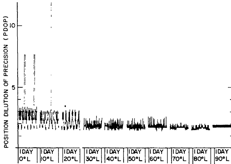
Fig. 14 — PDOP plot for a 3 × 8 constellation inclined at 90° with a period of 8 hr and a 5° mask
