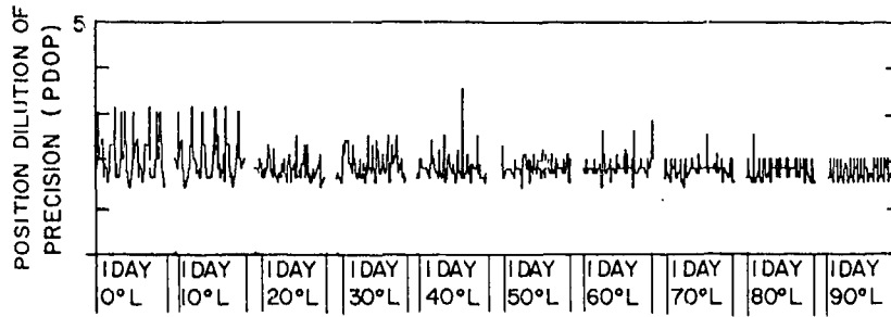
Fig. 10 — PDOP plot for a 3 \times 7 constellation inclined at 90^\circ with a period of 24 hr and a 5^\circ mask
