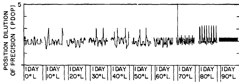
Fig. 12 — PDOP plot for a 3 × 7 constellation inclined at 53° with a period of 24 hr and a 5° mask
