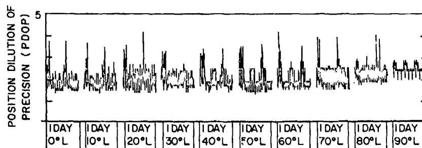
Fig. 35 — Inoperative satellite PDOP plot of a 3 \times 9 constellation with satellite (2,2) inoperative and a 5^\circ mask
