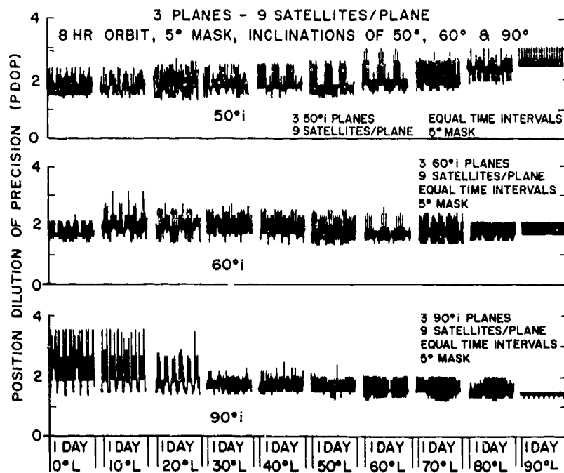
Fig. 28 — Comparison of 50°, 60°, and 90° inclinations for a 3 x 9 constellation with 8-hr orbits and 5° masks
