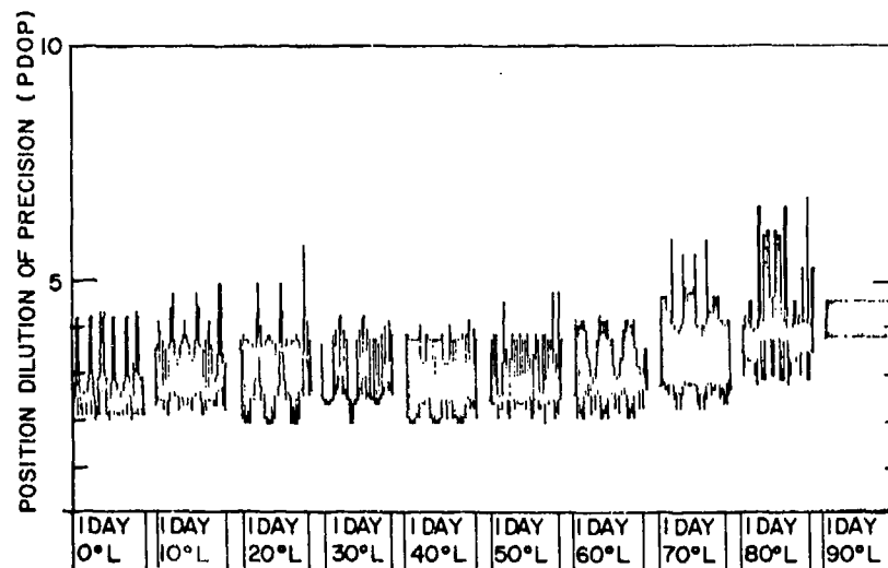
Fig. 33 — PDOP plot for a 3 \times 12 constellation inclined at 53^\circ with a period of 8 hr and a 20^\circ mask
