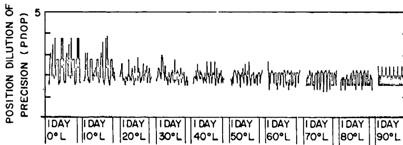
Fig. 22 — PDOP plot for a 3 \times 8 constellation inclined at 90^\circ with a period of 24 hr and a 10^\circ mask
