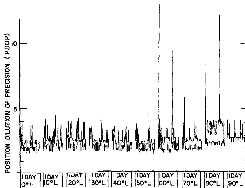
Fig. 36 — Inoperative satellite PDOP plot of a 3 \times 9 constellation with satellite (2,2) inoperative and a 10^\circ mask
