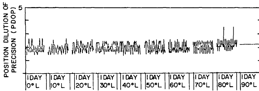
Fig. 19 - PDOP plot for a 3 x 8 constellation inclined at 53° with a period of 12 hr and a 5° mask
