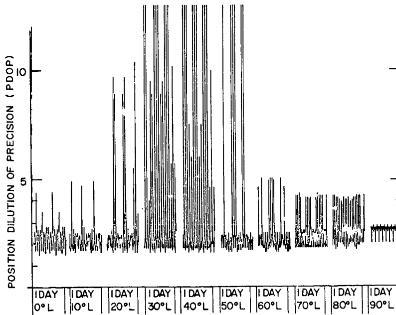
Fig. 7 — PDOP plot for a 3 \times 7 constellation inclined at 53^\circ with a period of 8 hr and a 5^\circ mask
