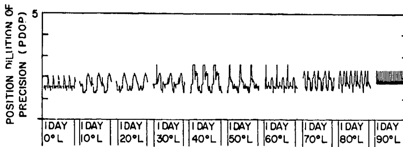
Fig. 23 — PDOP plot for a 3 \times 8 constellation inclined at 53^\circ with a period of 24 hr and a 5^\circ mask
