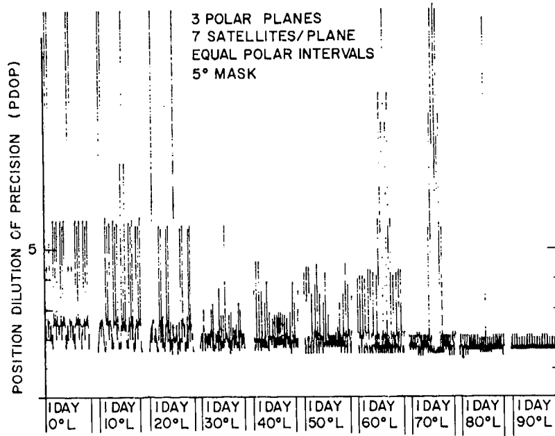
Fig. 6 — PDOP plot for a 3 \times 7 constellation inclined at 90^\circ with a period of 8 hr and a 5^\circ mask. A four-parameter solution is used instead of a three-parameter xyz solution.
