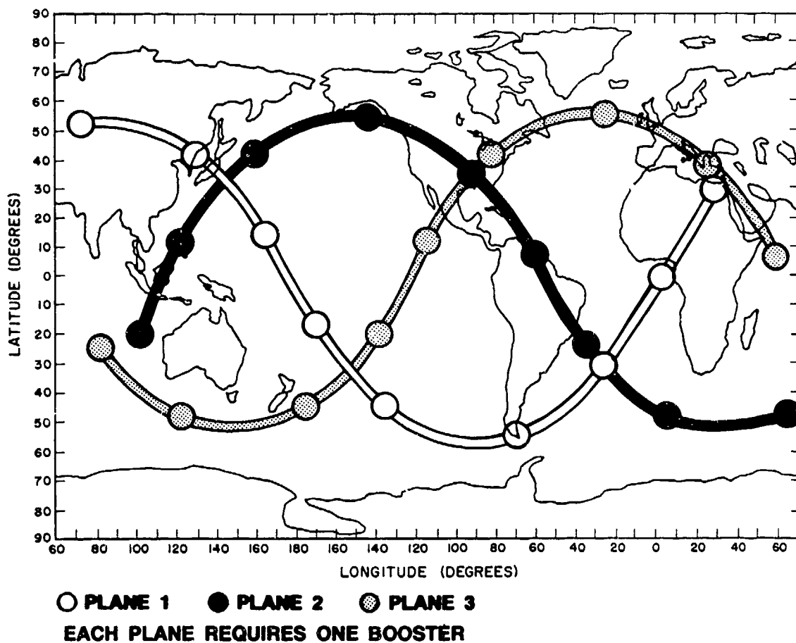
Fig. 3 -- Coverage for a 3 x 9 constellation with an 8-hr period at a 53° inclination. The lead satellites in each plane are staggered with initial argument of perigee equal to 40/3, 0, -40/3 degrees, respectively.
