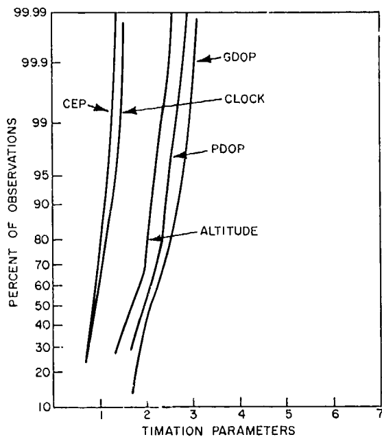
Fig. 37 — Percentile coverage versus Timing parameters of a 3 \times 9 constellation at 53^\circ inclination with an 8-hr period and 5^\circ mask
