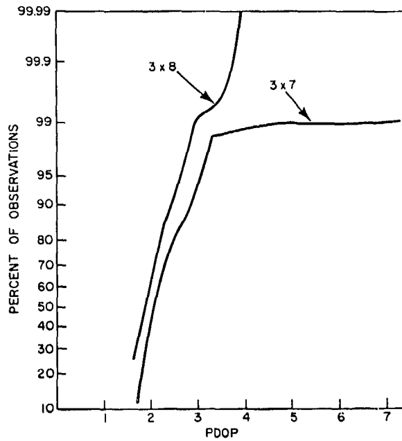
Fig. 45 — Percentile coverage versus PDOP value plot of 3 \times 7 and 3 \times 8 constellations at 90^\circ inclination with a 24-hr period and a 10^\circ mask
