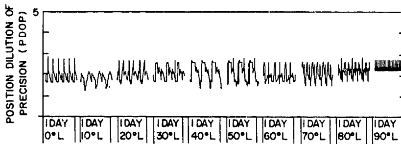
Fig. 24 — PDOP plot for a 3 \times 8 constellation inclined at 53^\circ with a period of 24 hr and a 10^\circ mask
