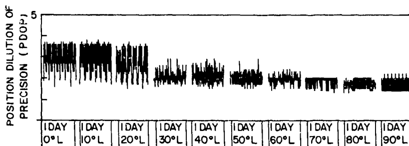
Fig. 26 — PDOP plot for a 3 × 9 constellation inclined at 90° with a period of 8 hr and a 10° mask
