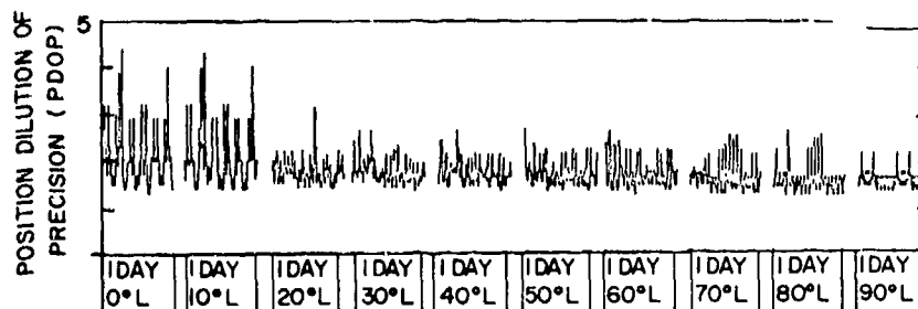
Fig. 34 — Inoperative satellite PDOP plot of a 3 × 9 constellation with satellite (2,1) inoperative and a 5° mask
