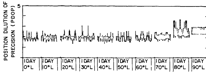
Fig. 31 — PDOP plot for a 3 \times 12 constellation inclined at 53^\circ with a period of 8 hr and a 10^\circ mask
