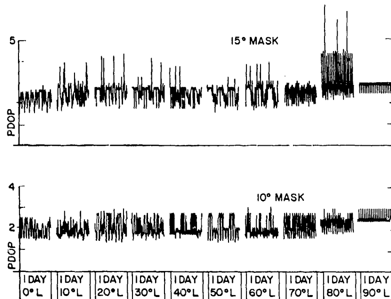
Fig. 29 — Comparison of 10° and 15° masks for a 3 × 9 constellation with 12-hr orbits at 53° inclinations
