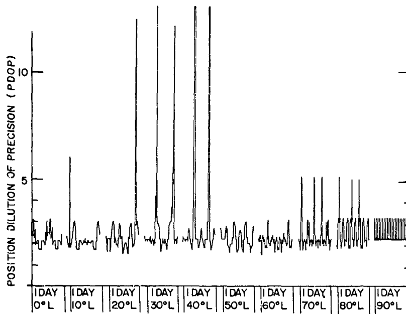
Fig. 13 — PDOP plot for a 3 × 7 constellation inclined at 53° with a period of 24 hr and a 10° mask
