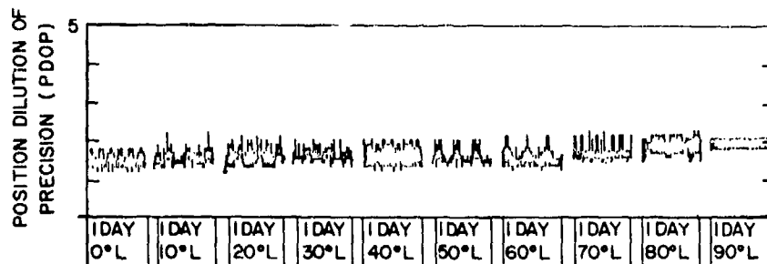
Fig. 30 — PDOP plot for a 3 × 12 constellation inclined at 53° with a period of 8 hr and a 5° mask
