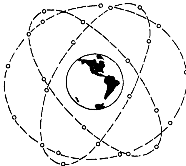
Fig. 2 — 3 \times 9 constellation (3 planes, 9 satellites per plane) inclined at 33^\circ to the equator with a plane-to-plane spacing of 120^\circ
