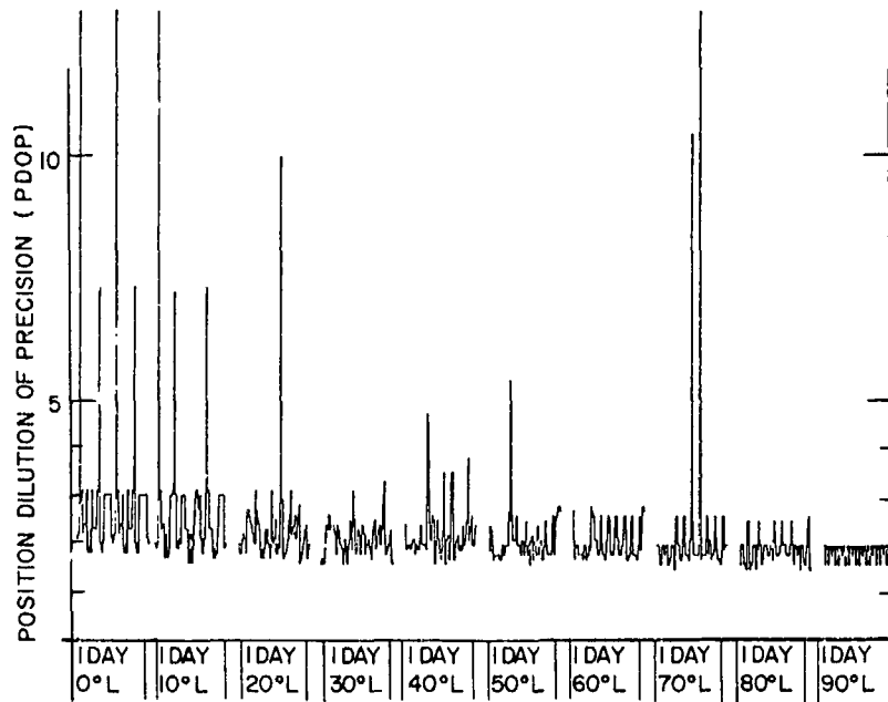
Fig. 11 — PDOP plot for a 3 \times 7 constellation inclined at 90^\circ with a period of 24 hr and a 10^\circ mask
