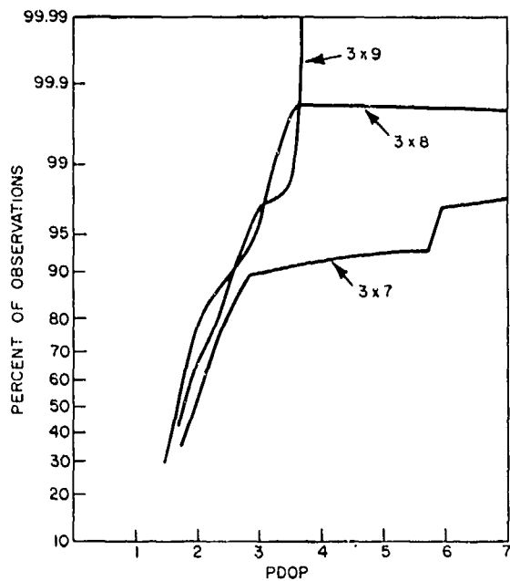
Fig. 42 — Percentile coverage versus PDOP value plot of 3 \times 7 , 3 \times 8 , and 3 \times 9 constellations at 90^\circ inclination with an 8-hr period and a 5^\circ mask
