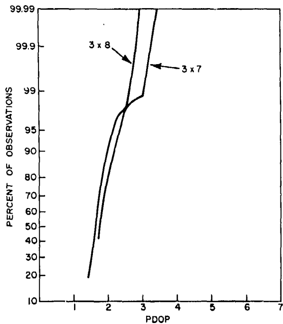
Fig. 44 — Percentile coverage versus PDOP value plot of 3 \times 7 and 3 \times 8 constellations at 90^\circ inclination with a 24-hr period and a 5^\circ mask
