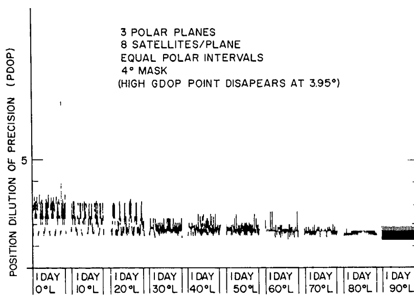
Fig. 15 — PDOP plot for a 3 x 8 constellation inclined at 90° with a period of 8 hr and a 4° mask
