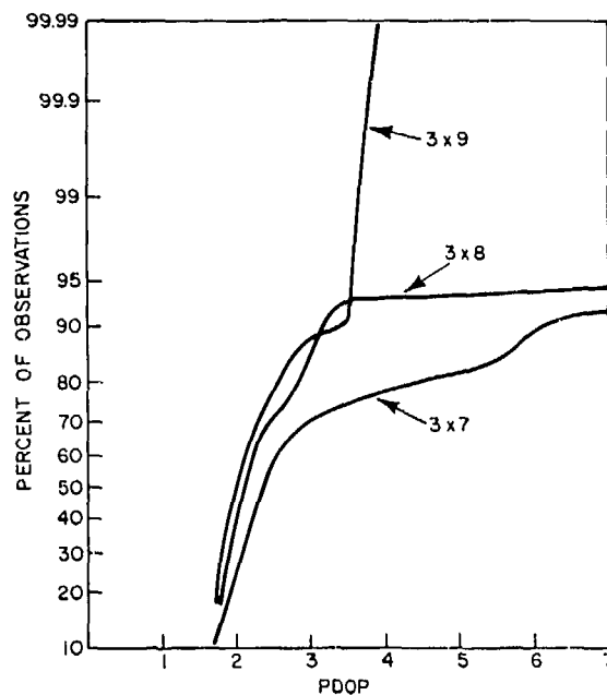
Fig. 43 — Percentile coverage versus PDOP value plot of 3 \times 7 , 3 \times 8 , and 3 \times 9 constellations at 90^\circ inclination with an 8-hr period and a 10^\circ mask
