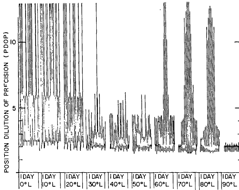
Fig. 8 — PDOP plot for a 3 x 7 constellation inclined at 9° with a period of 8 hr and a 10° mask
