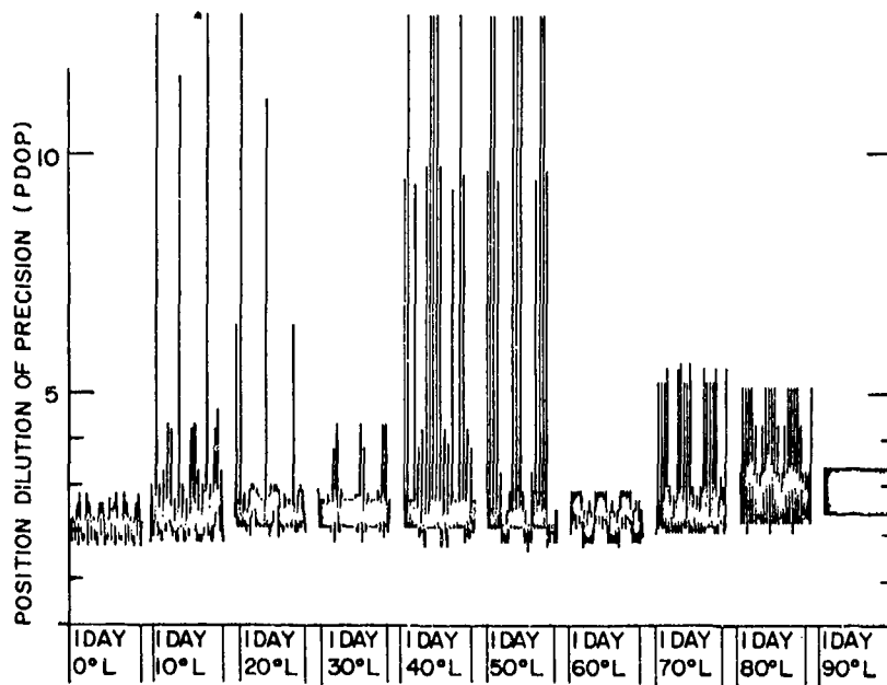
Fig. 18 -- PDOP plot for a 3 \times 8 constellation inclined at 53^\circ with a period of 8 hr and a 10^\circ mask
