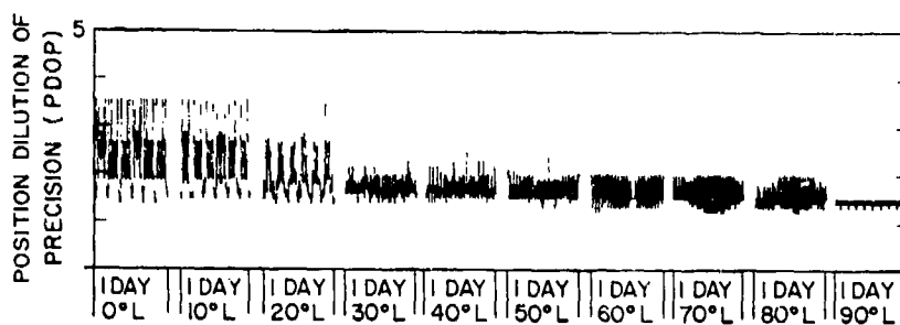
Fig. 25 — PDOP plot for a 3 × 9 constellation inclined at 90° with a period of 8 hr and a 5° mask
