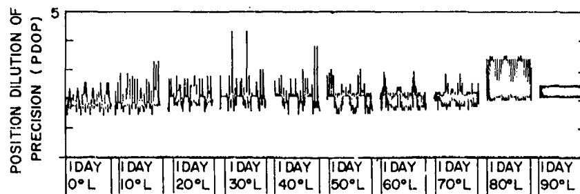
Fig. 17 -- PDOP plot for a 3 \times 8 constellation inclined at 53^\circ with a period of 8 hr and a 5^\circ mask
