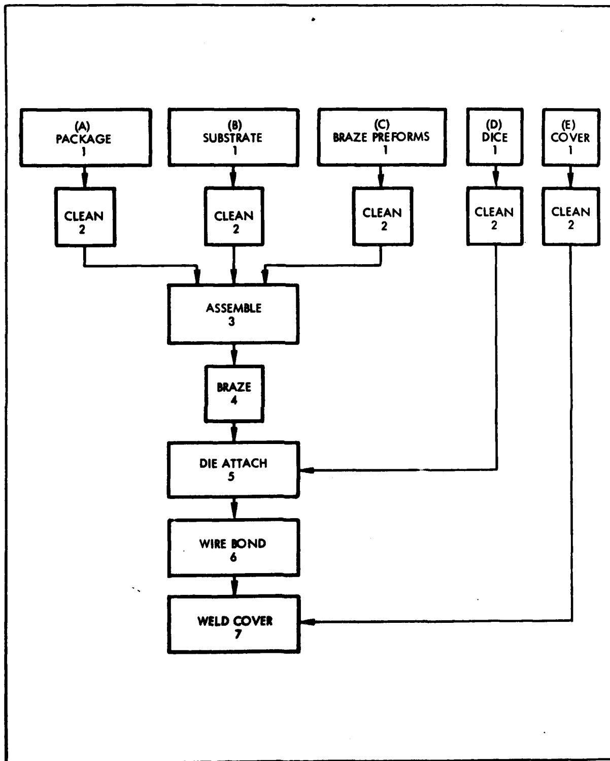
Figure 10 - Type 1 Package - Process Sequence
