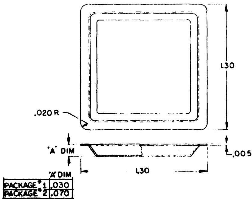
Figure 13 - Coined Cover
