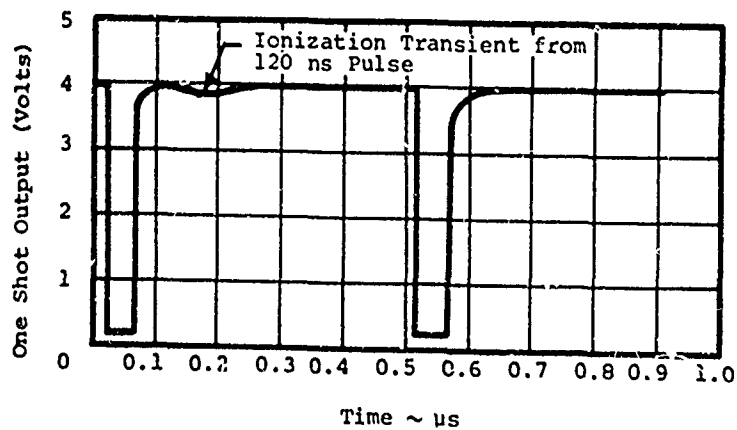
Figure 6-2. 5401 One-Shot Ionization SFXR Prediction
