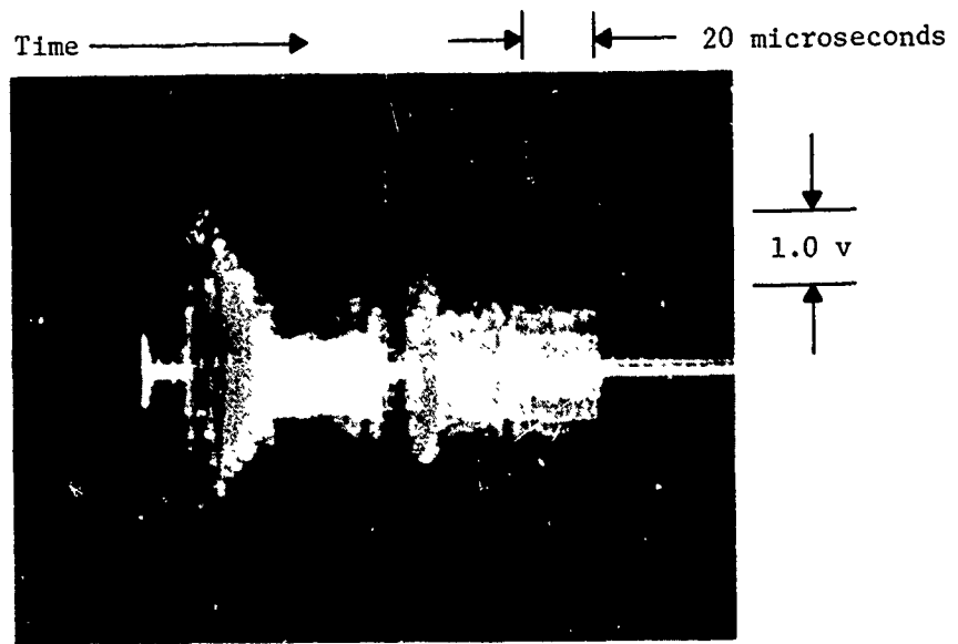
Figure 8. EMI Pulse Obtained During Test 13, Step
