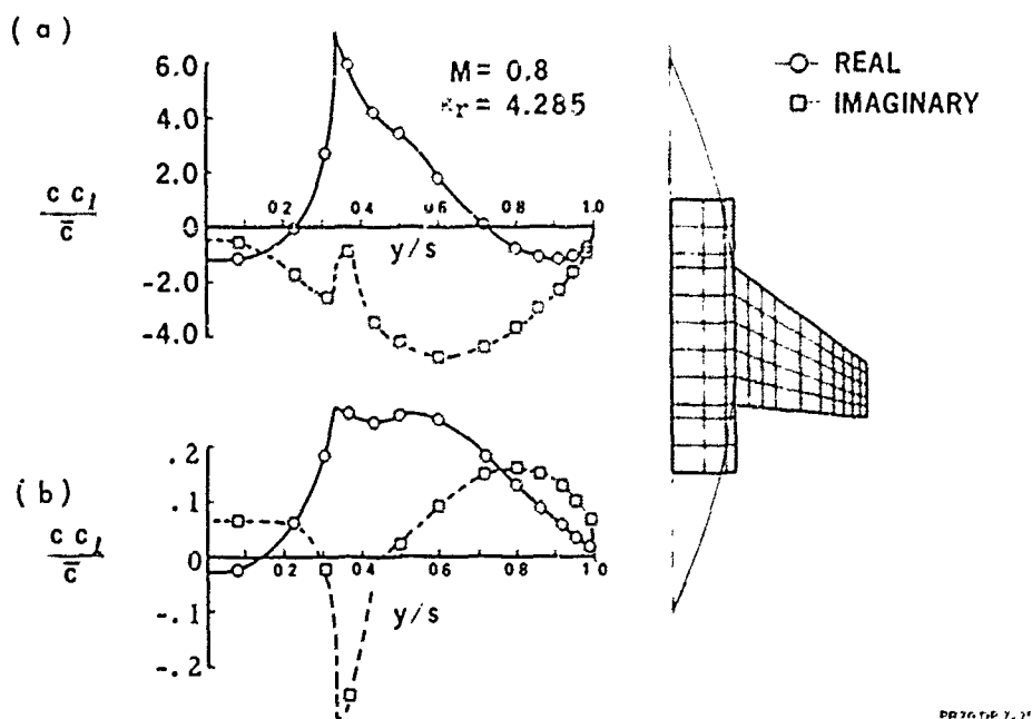
Figure 6. Span Load Distribution for a Wing-Body Combination in Unsteady Flow: (a) Body Pitching, Wing Stationary; (b) Body Cambering, Wing Stationary.
