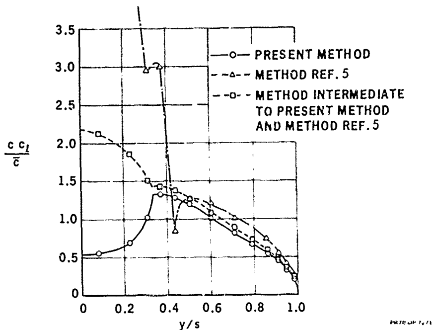
Figure 5. Span Load Distribution as Calculated by Three Different Methods.
