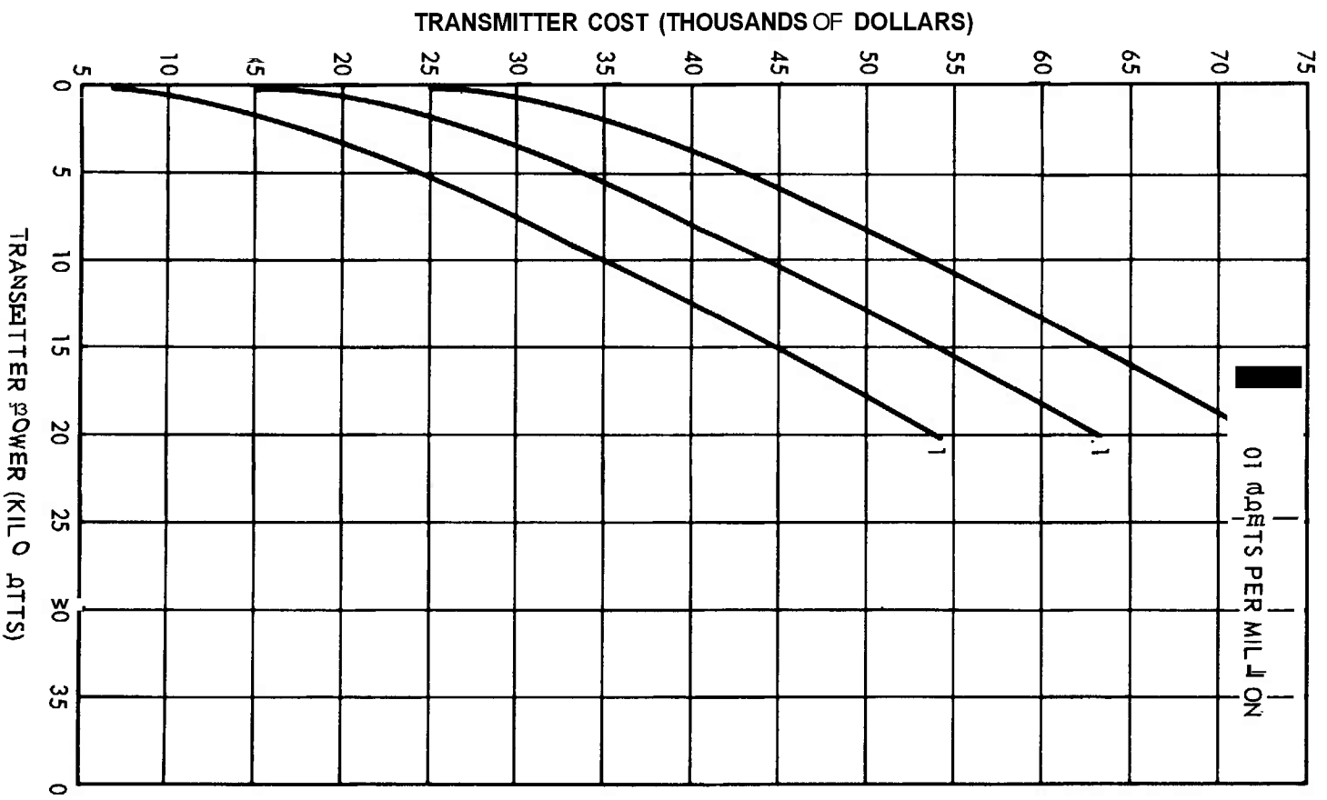
Figure 7. H f shore transmitter cost versus power for various values of transmitter stability.
