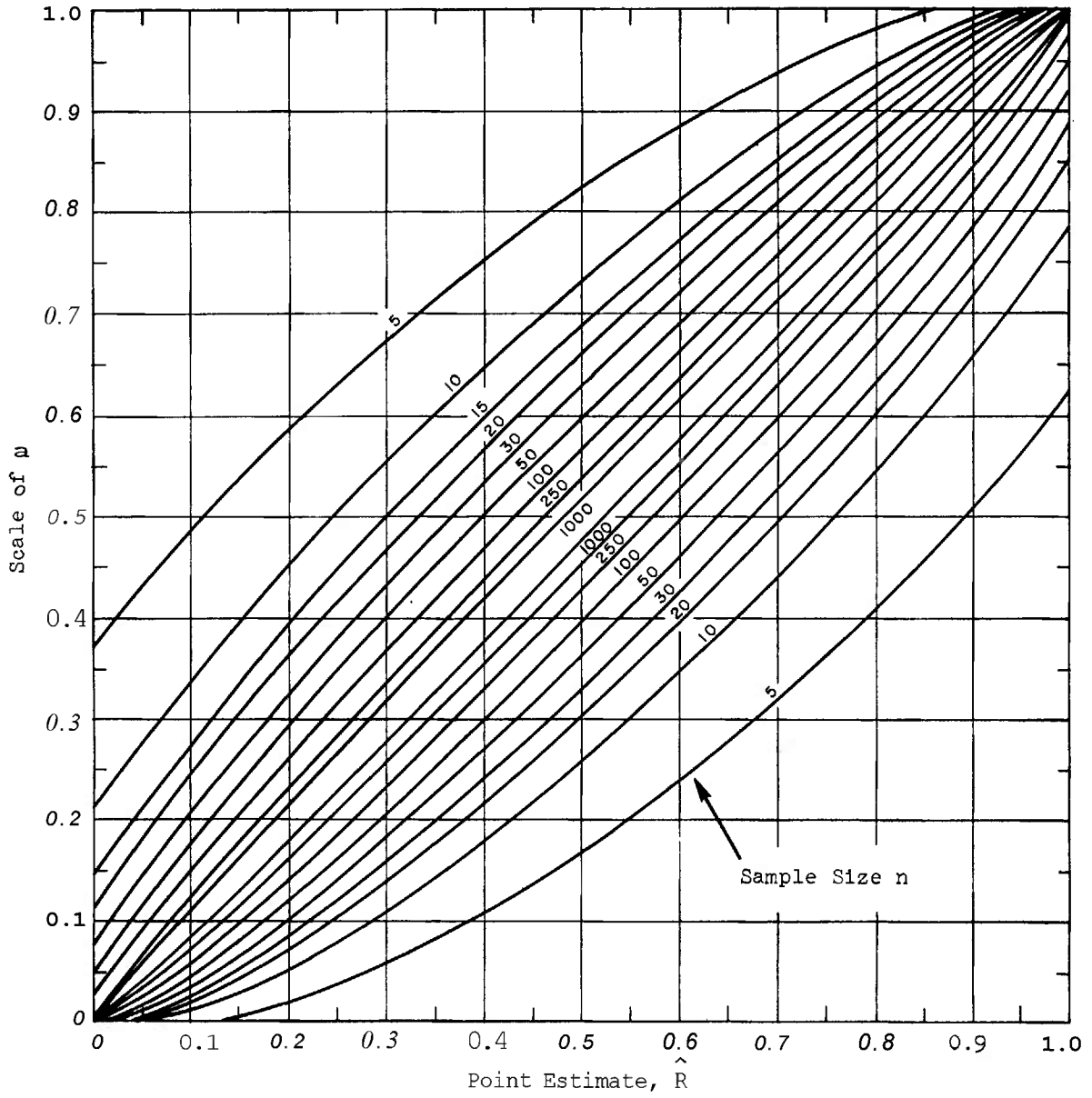
FIGURE C-1A CONFIDENCE BELTS FOR PROPORTIONS Confidence Coefficients: 0.80 for Two-sided Estimation, 0.90 for One-Sided Estimation
