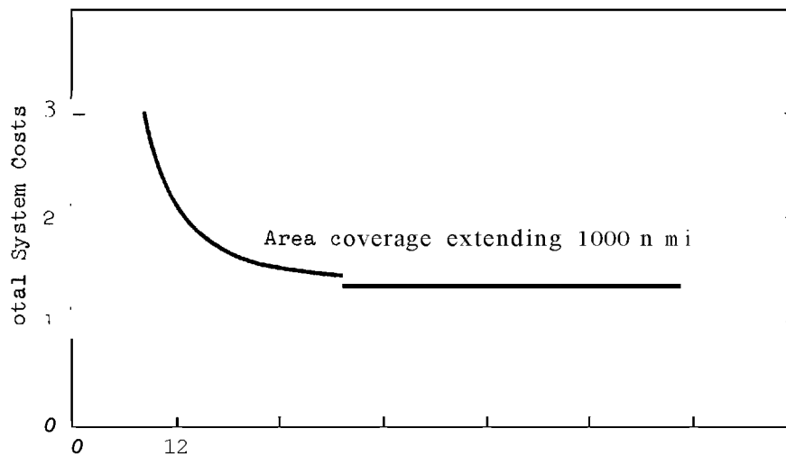
FIGURE 2-12 SENSITIVITY ANALYSIS
