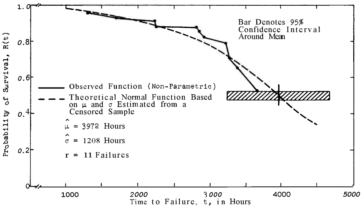
FIGURE 4-5 NONPARAMETRIC AND THEORETICAL NORMAL RELIABILITY FUNCTIONS
