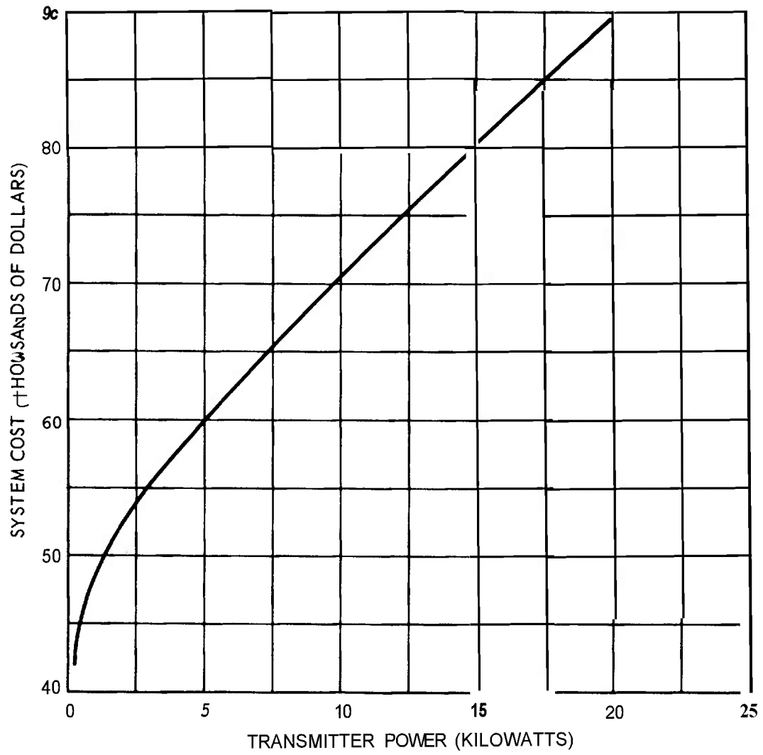
Figure 12. System cost versus transmitter power.
