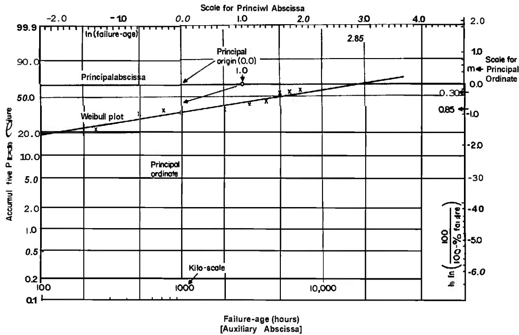
FIGURE 4.7 GRAPHIC PROCEDURE FOR OBTAINING ESTIMATES OF PARAMETERS ASSOCIATED WITH THE WEIBULL DISTRIBUTION
