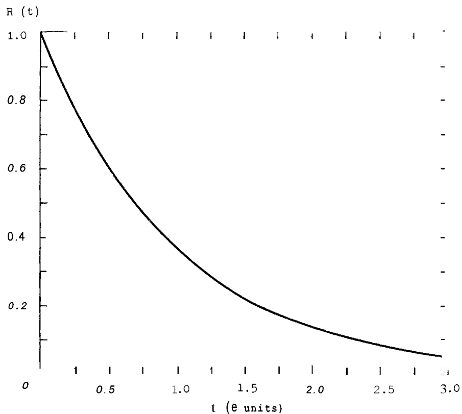
FIGURE 4.1 THE EXPONENTIAL RELIABILITY FUNCTION
