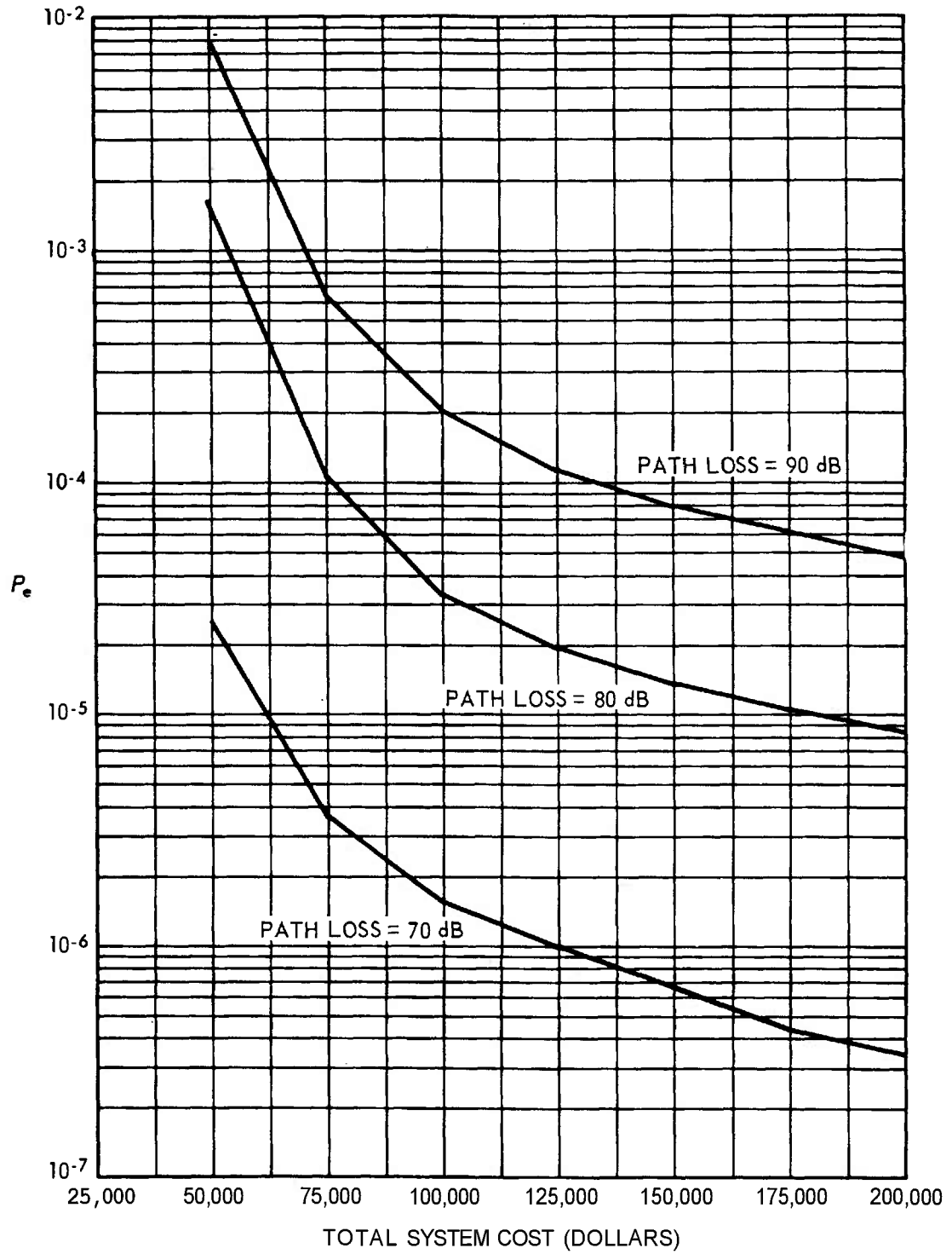
Figure 5. System cost versus P_e for various path losses.
