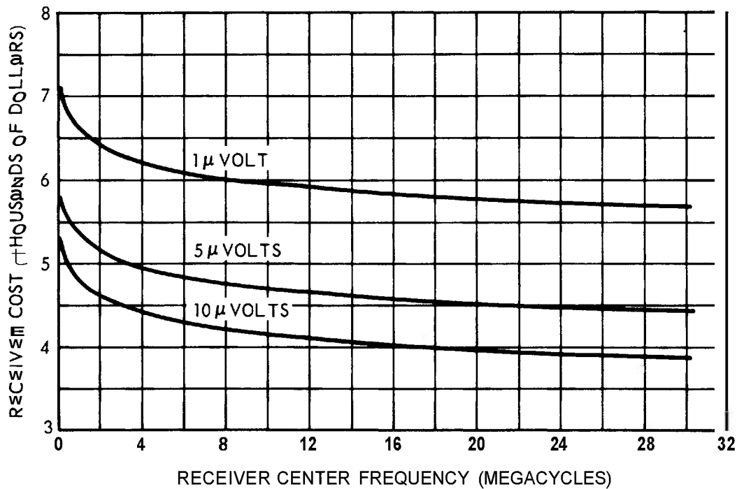
Figure 6. Receiver cost versus center frequency for various values of receiver sensitivity.
