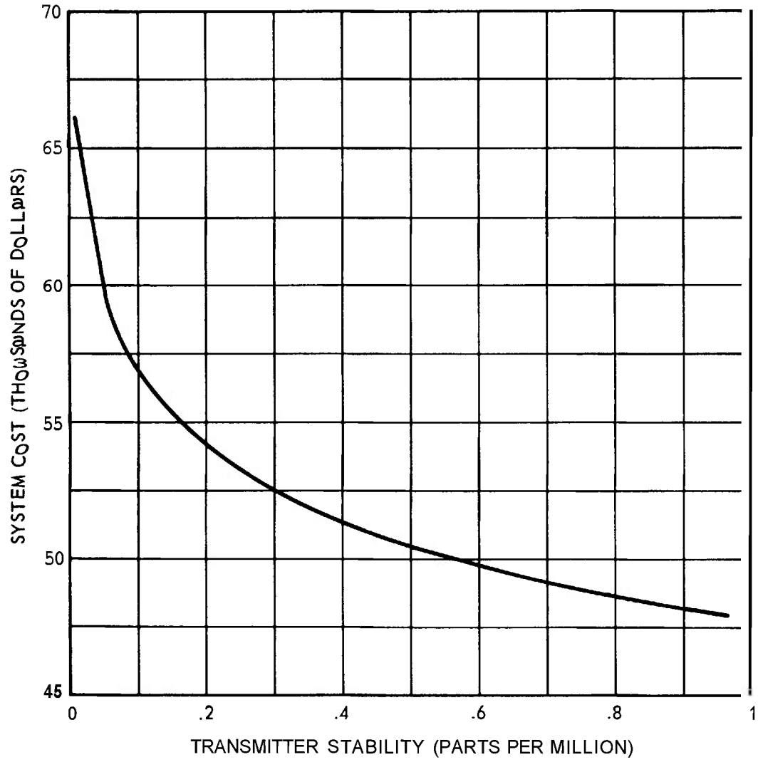
Figure 9. System cost versus transmitter stability.
