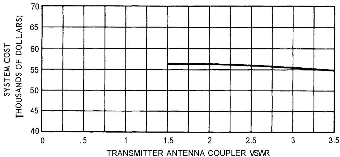
Figure 8. System cost versus transmitter antenna coupler VSWR.
