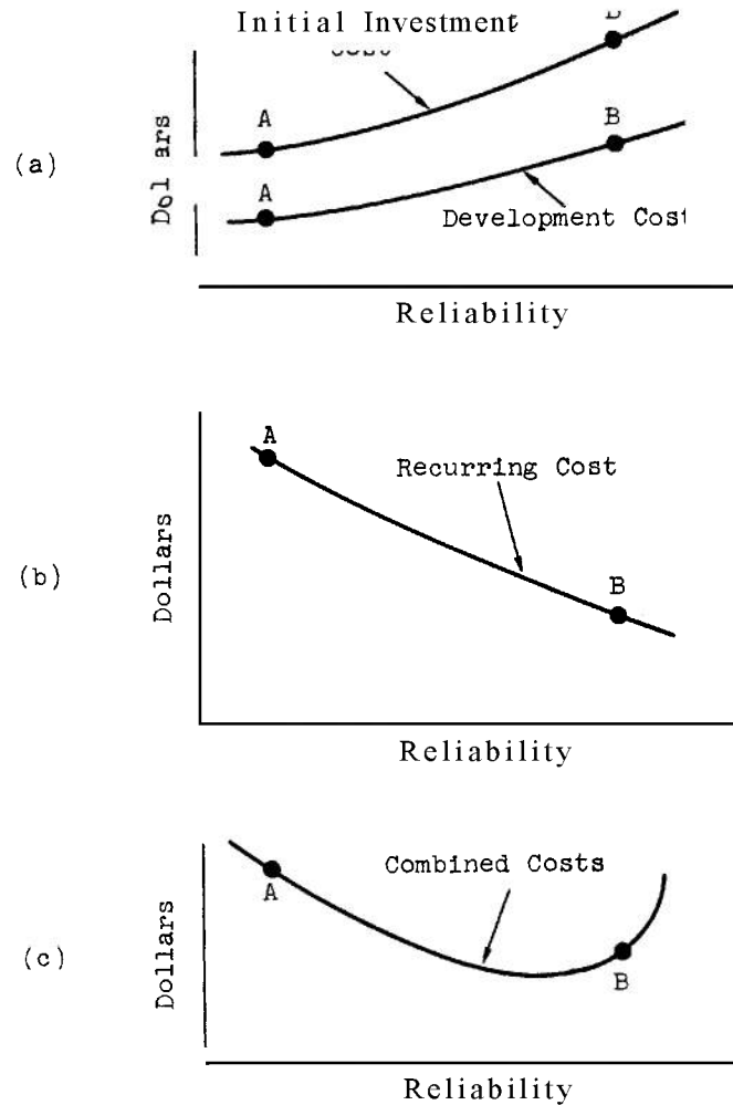
FIGURE 2-10 TRADE-OFF CURVES
