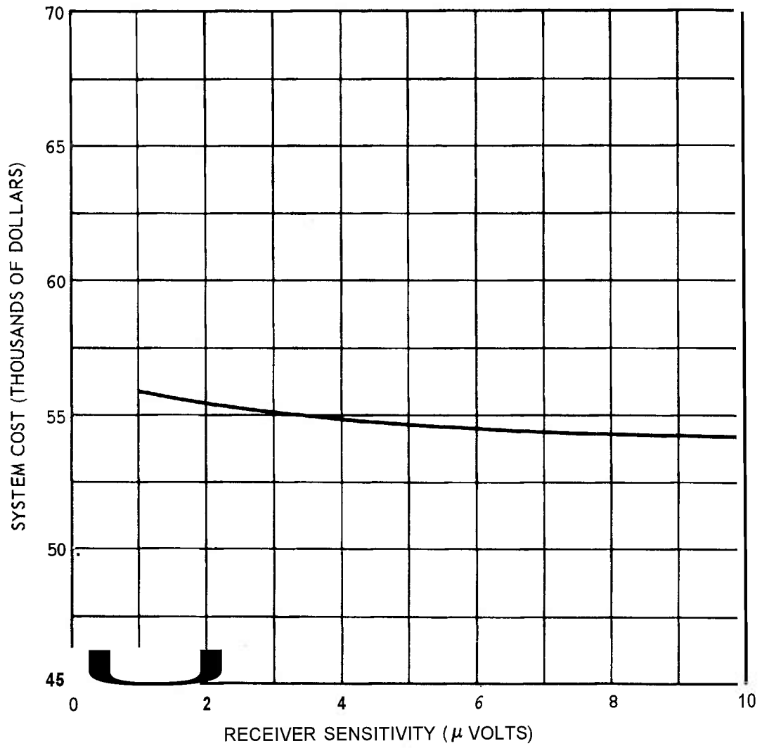
Figure 11. System cost versus receiver sensitivity.
