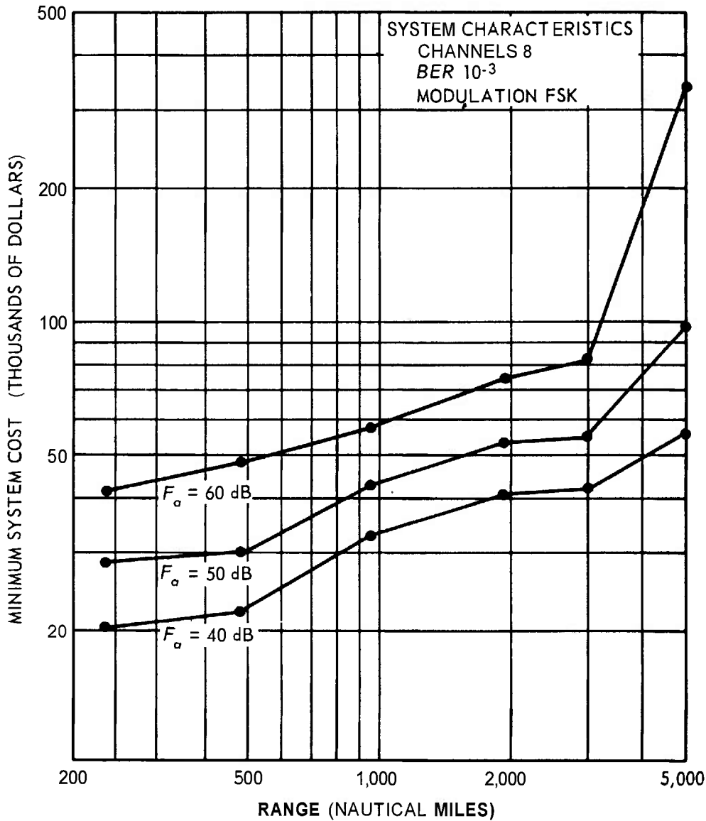
Figure 3. System cost versus range for various values of F_a .
