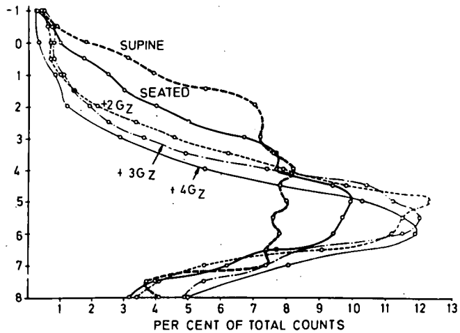
Fig. 7-3 The distribution of ^{131}\text{I} -MAA following i.v. injection in subjects supine, seated and at +2, +3 and +4G z .
