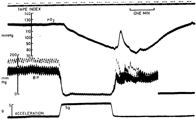
Fig. 10-17 Effect of an acceleration of +5G_z lasting two minutes on an anaesthetised dog, relaxed and ventilated at a constant rate and depth with oxygen. From above, downwards, the traces record tape index, arterial oxygen tension ( P_{O_2} ), systemic blood pressure referred to heart level (B.P.), and imposed acceleration. Note progressive fall in oxygen tension during acceleration, transient recovery on return to one G, and the slow final recovery. The pressure transducer was open to atmosphere for the last 90 seconds of the recording. (From (104), by courtesy of Aerospace Med.).
