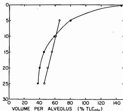
Fig. 3-6 Relationship between vertical distance and alveolar volume in greyhound dogs frozen head-up at FRC (solid circles). From data of Glazier et al. Open circles indicate results obtained on normal seated men at FRC from fig. 3-1.
