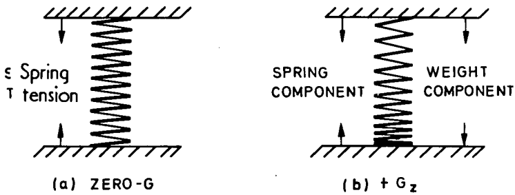
Fig. 11-1 Behaviour of a loosely coiled spring when weightless (a) and when exposed to acceleration (b). Coil spacing is taken to indicate the relative sizes of alveoli within the lung.
