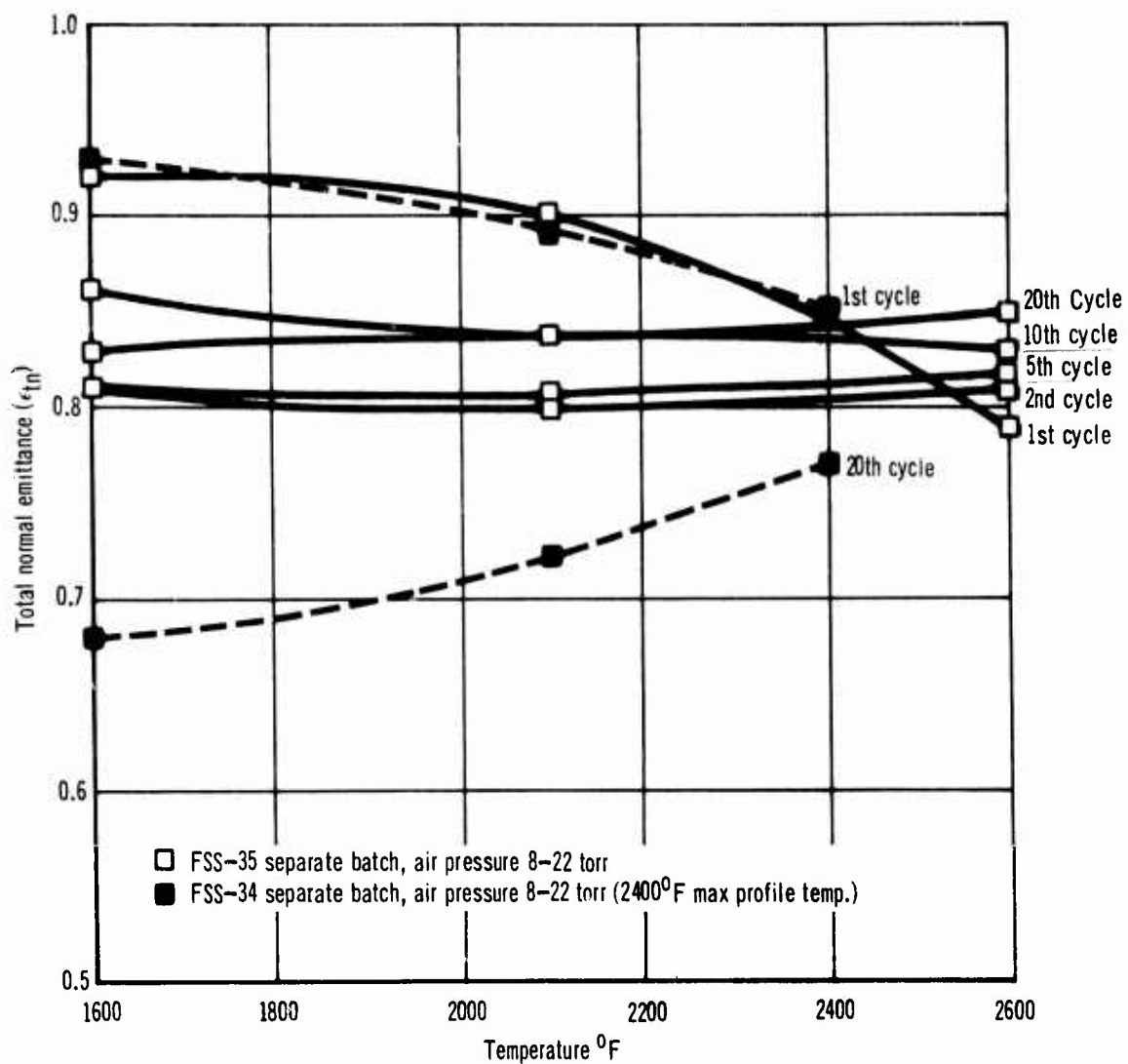
Figure 108 Emittance of R-512E Coated Columbium (Separate Batch) Versus Temperature (2600 ^{\circ}\text{F} Max)
