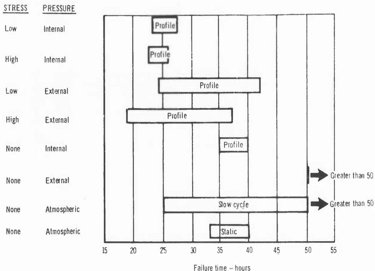
Figure 34 Baseline Oxidation Comparison (2600°F Tmax. For All Tests)
