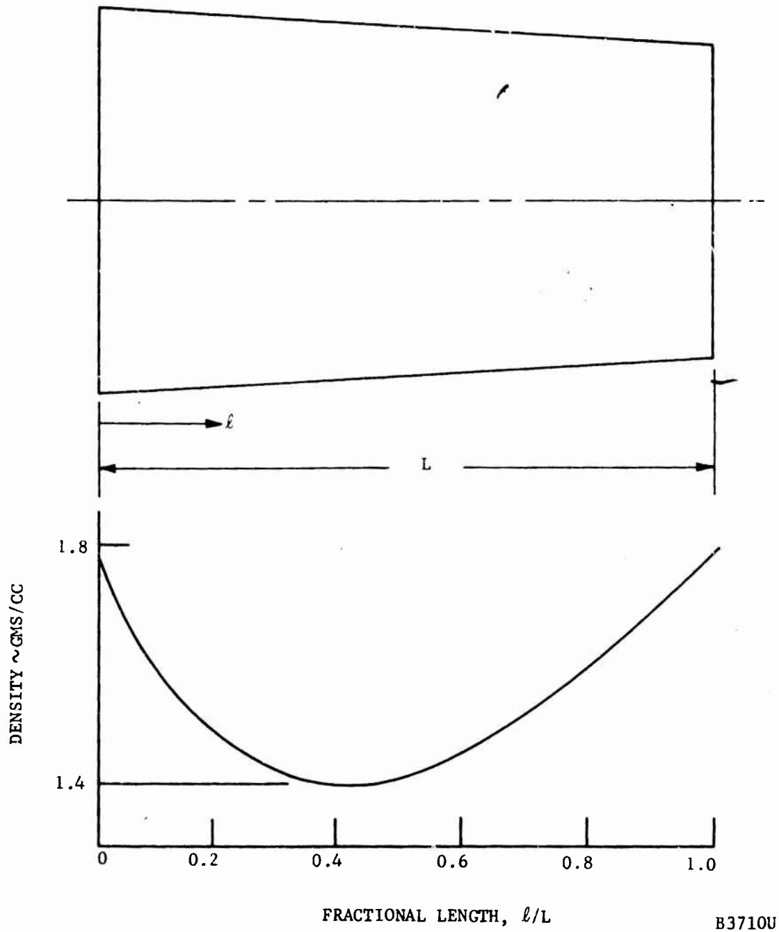
FIGURE 5. APPROXIMATE DENSITY VARIATION OF IMPREGNATED FRUSTA
