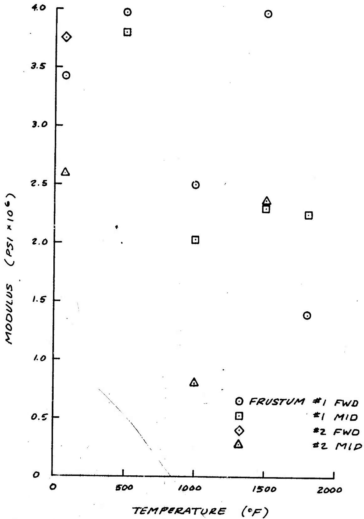
FIGURE 19. AS-3DC CIRCUMFERENTIAL COMPRESSIVE MODULUS
