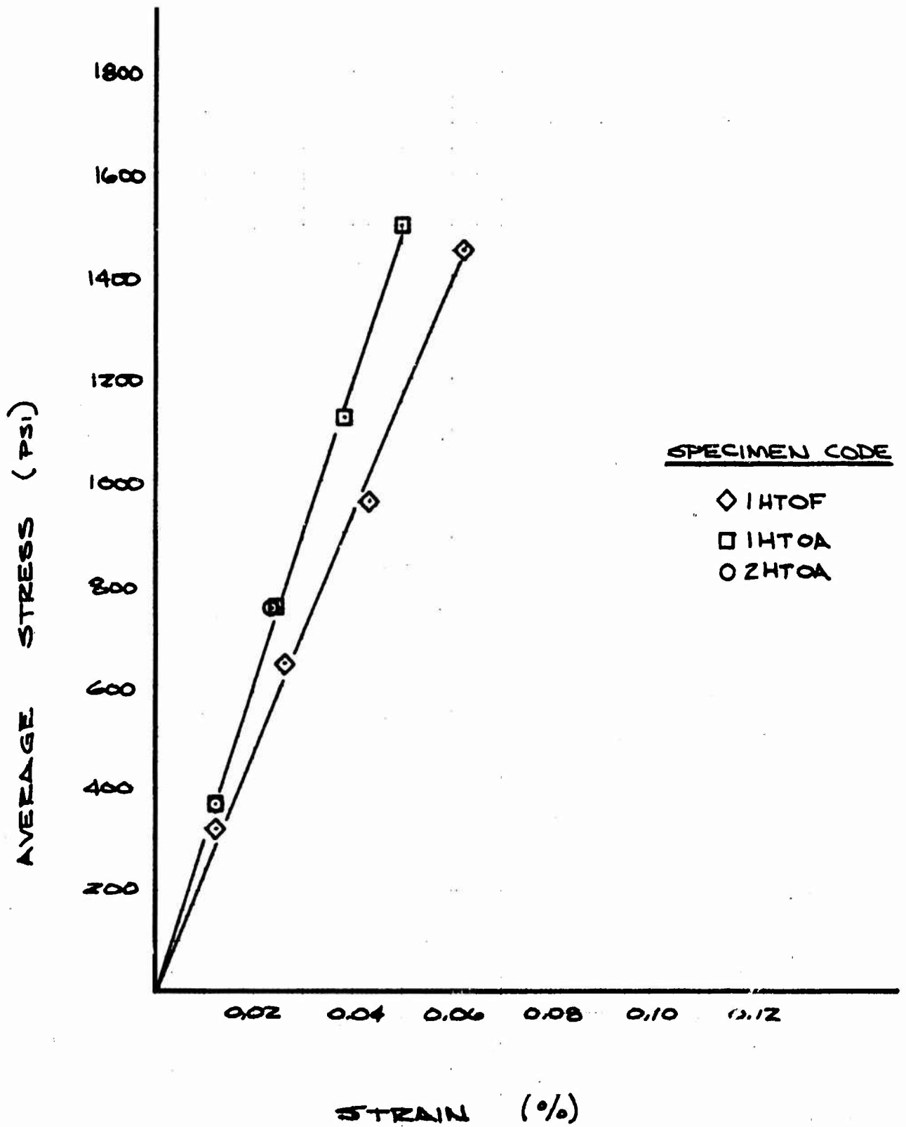
FIGURE 23. AVERAGE STRESS VERSUS STRAIN AS-3DC HOCF TENSILE SPECIMENS
