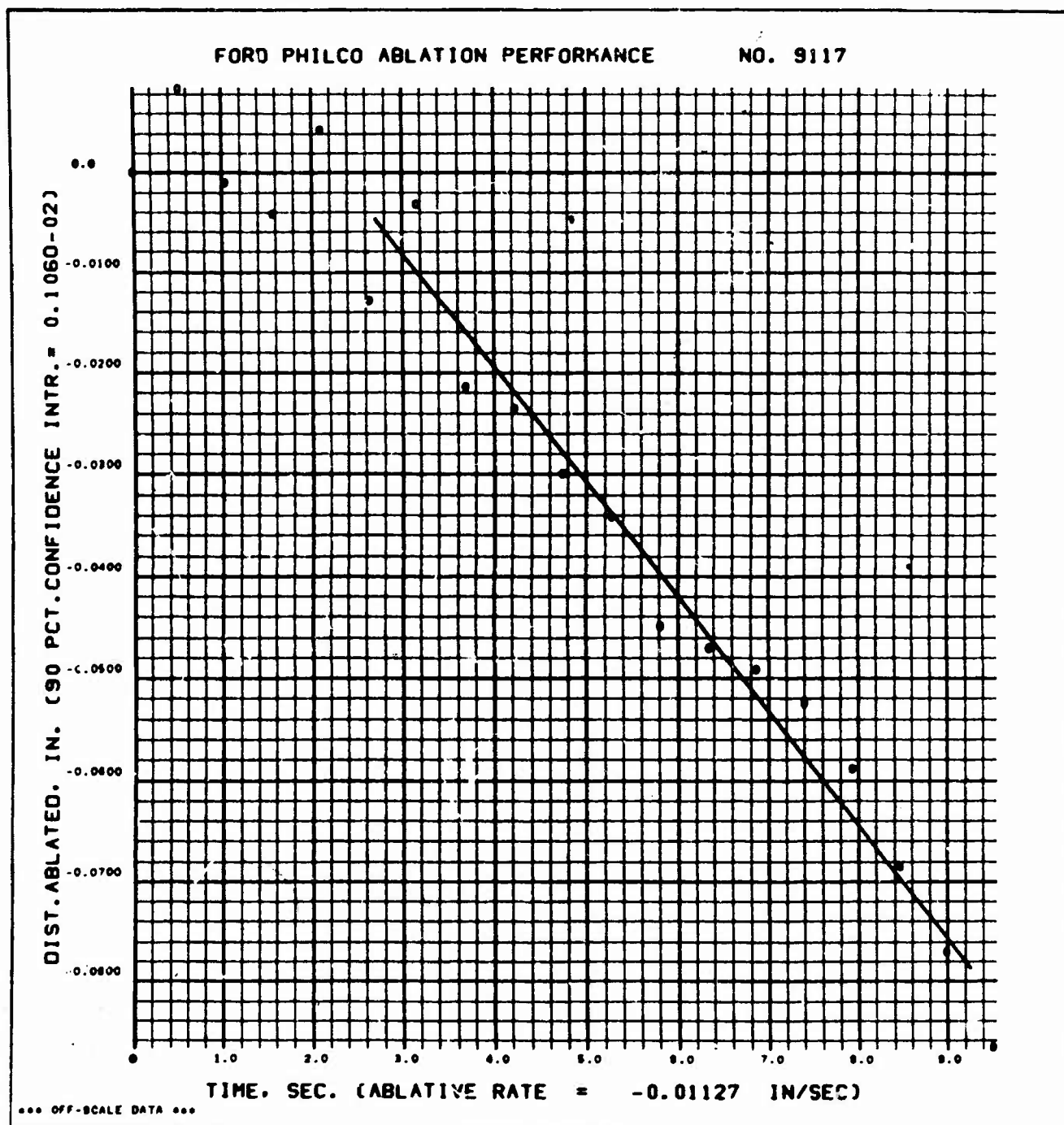
FIGURE 15 SURFACE RECESSION DATA - TEST SPECIMEN AS-2
