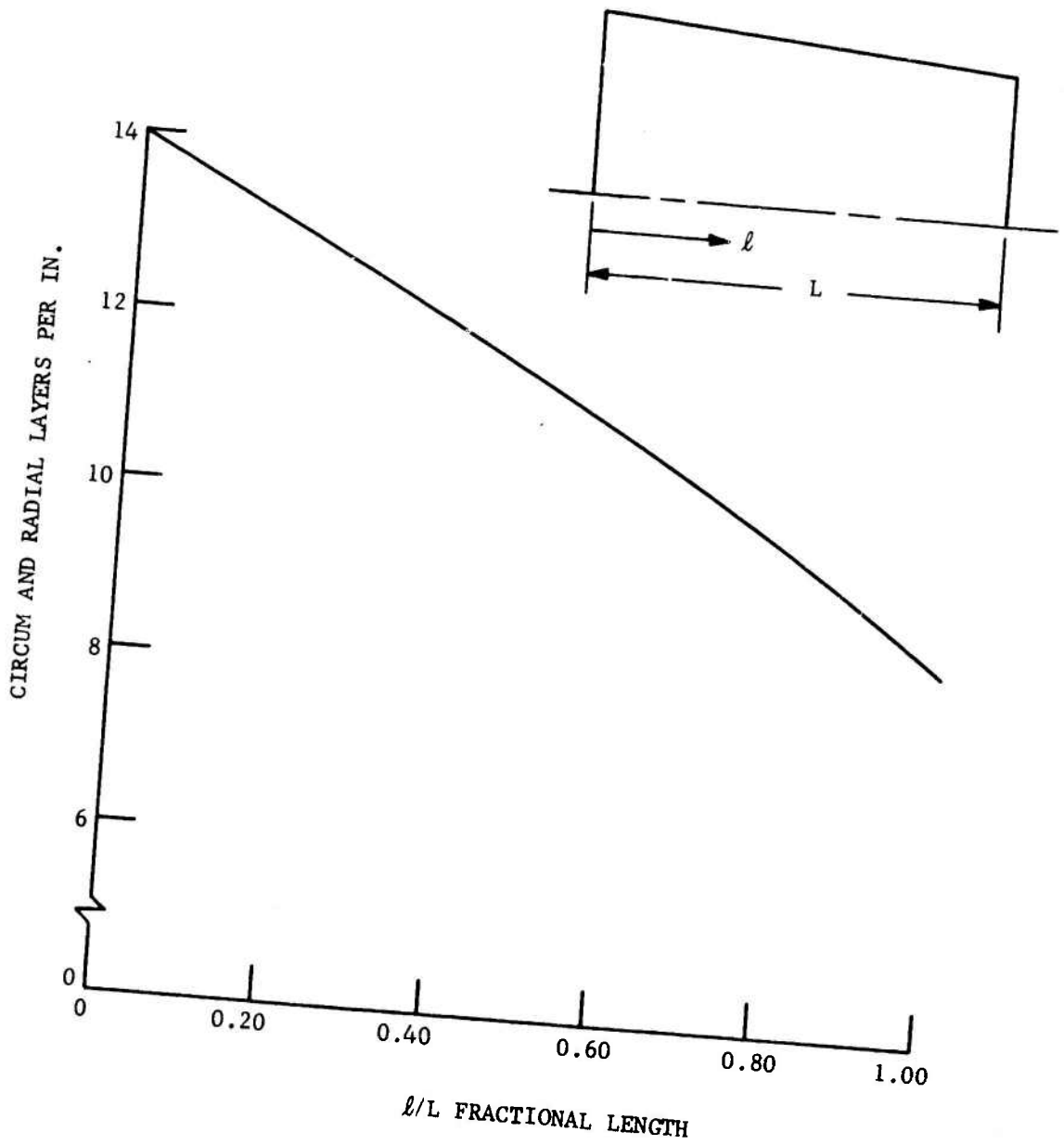
FIGURE 8. AS-3DC WEAVE REQUIREMENTS
