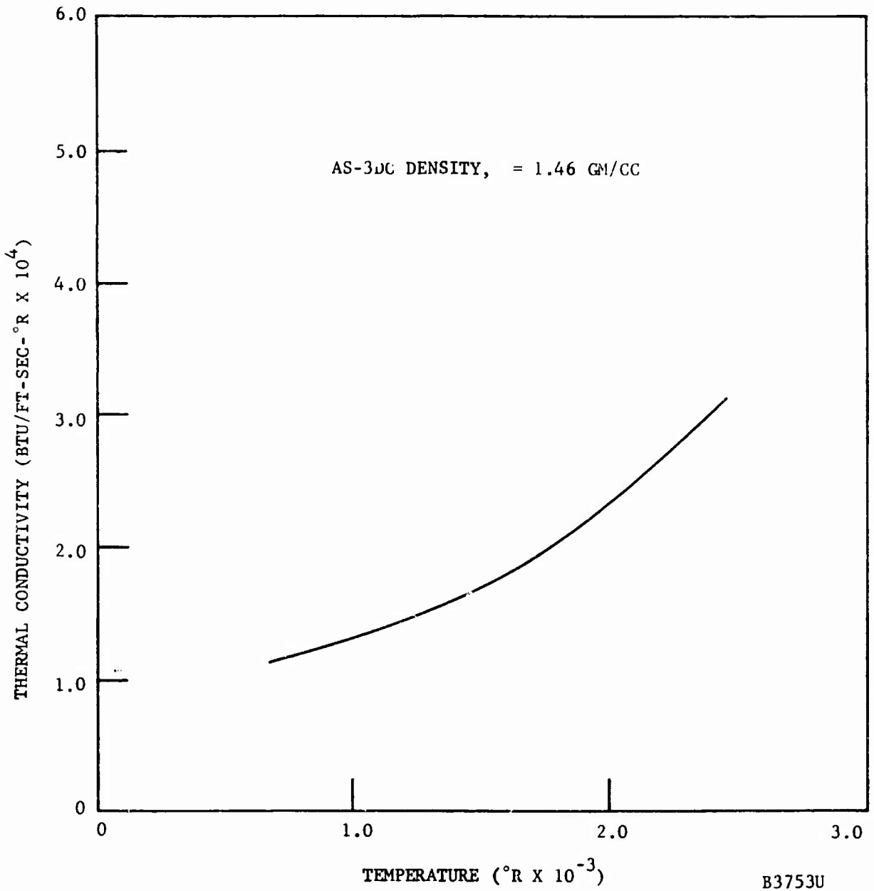
FIGURE 6. THERMAL CONDUCTIVITY VERSUS TEMPERATURE AS-3DC QUARTZ
