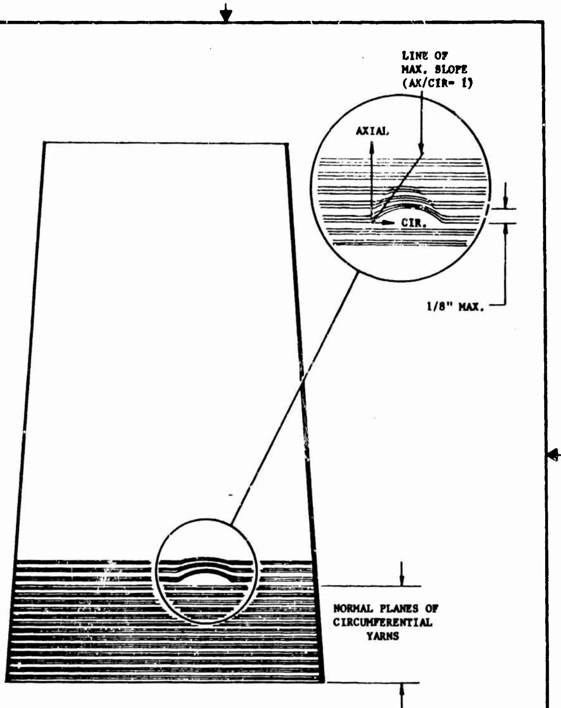
FIGURE 3. ALLOWABLE WAVINESS OF CIRCUMFERENTIAL YARNS
