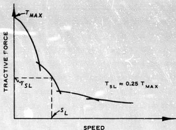
Fig. 9. Traction-speed-spacing analysis
