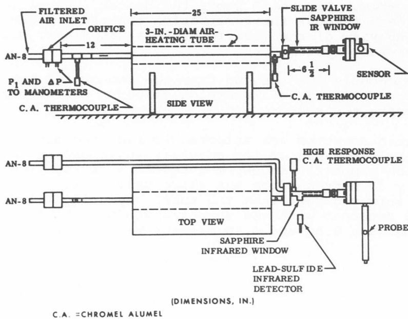
Figure 18. Temperature-Sensing System Bench-Test Diagram.
