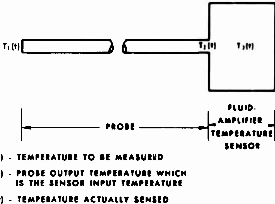
Figure 11. Physical Arrangement of Probe and Temperature Sensor.
