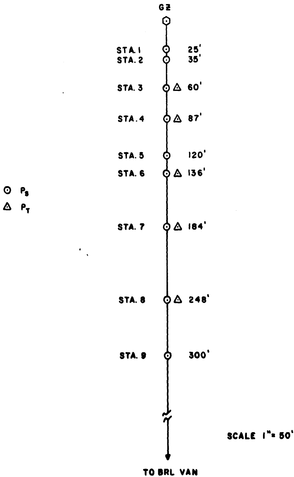
Figure 2.4 Instrument Layout, AN/FC 3
