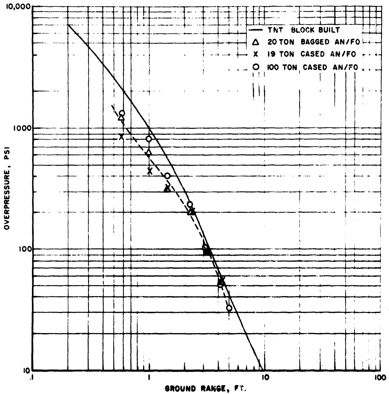
Figure J.2 AN/FO Overpressure Data Compared with TNT (Scaled to 1 lb. Sea Level)
