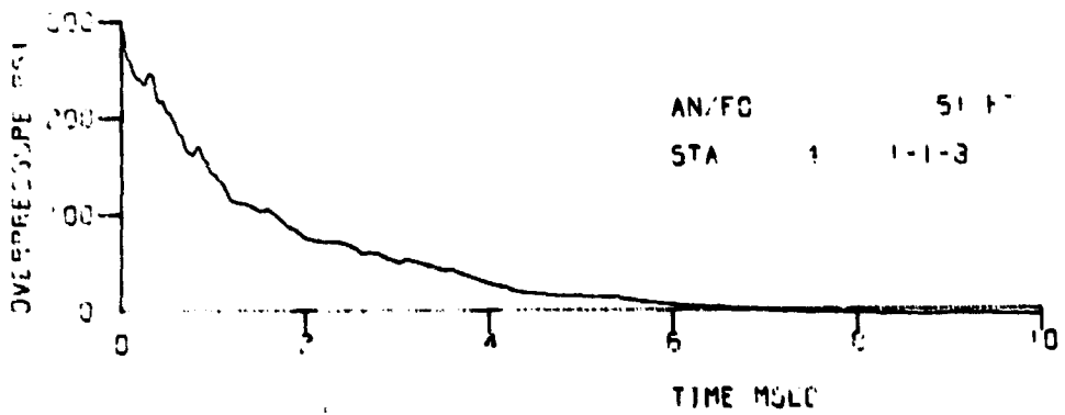
Figure A.1 Overpressure-Time Records, Stations 1-4, AN/FO 1
