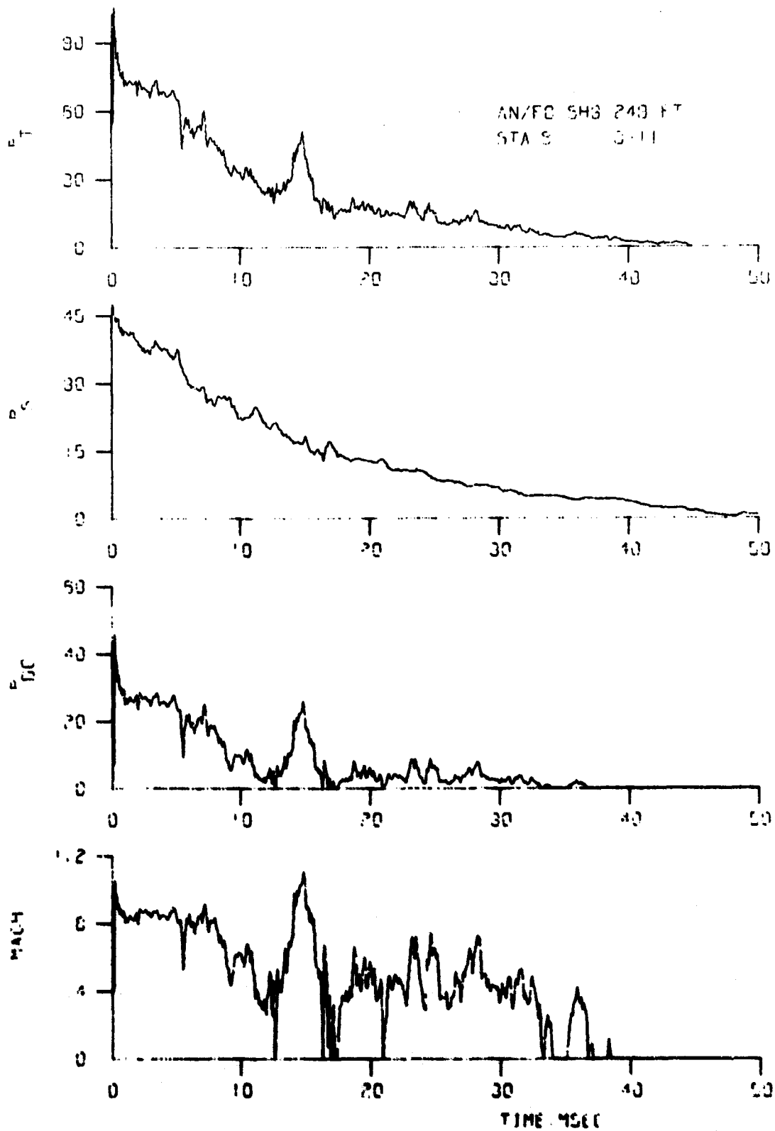
Figure A.12 Dynamic Pressure Data, Station 8, AN/PO: 3
