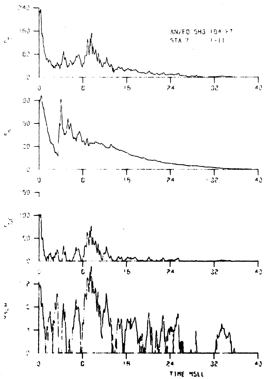
Figure A.11 Dynamic Pressure Data, Station 7, AN/PO 3
