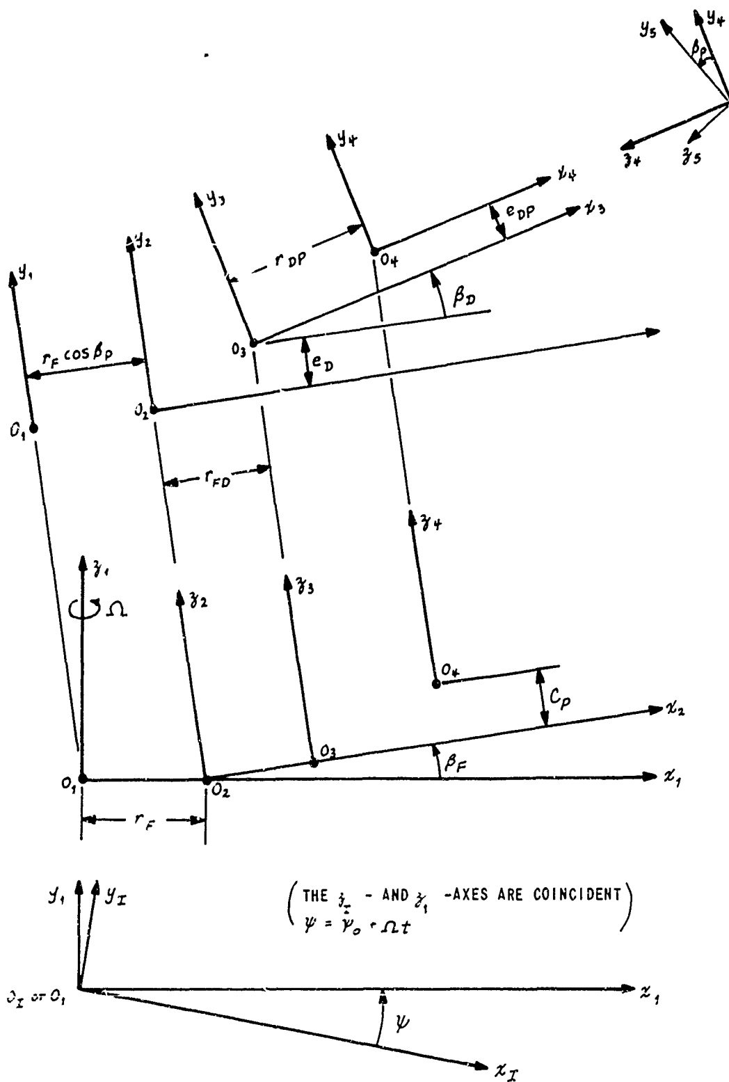
Figure 3. COORDINATE SYSTEMS.
