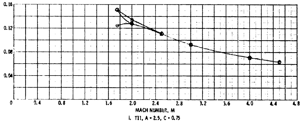
FIGURE 9. EFFECT OF RINGTAIL GEOMETRY AND LONGITUDINAL POSITION ON THE VARIATION OF \Delta C_N WITH MACH NUMBER, \delta = 4 deg, \psi = 4 deg (Concluded)
