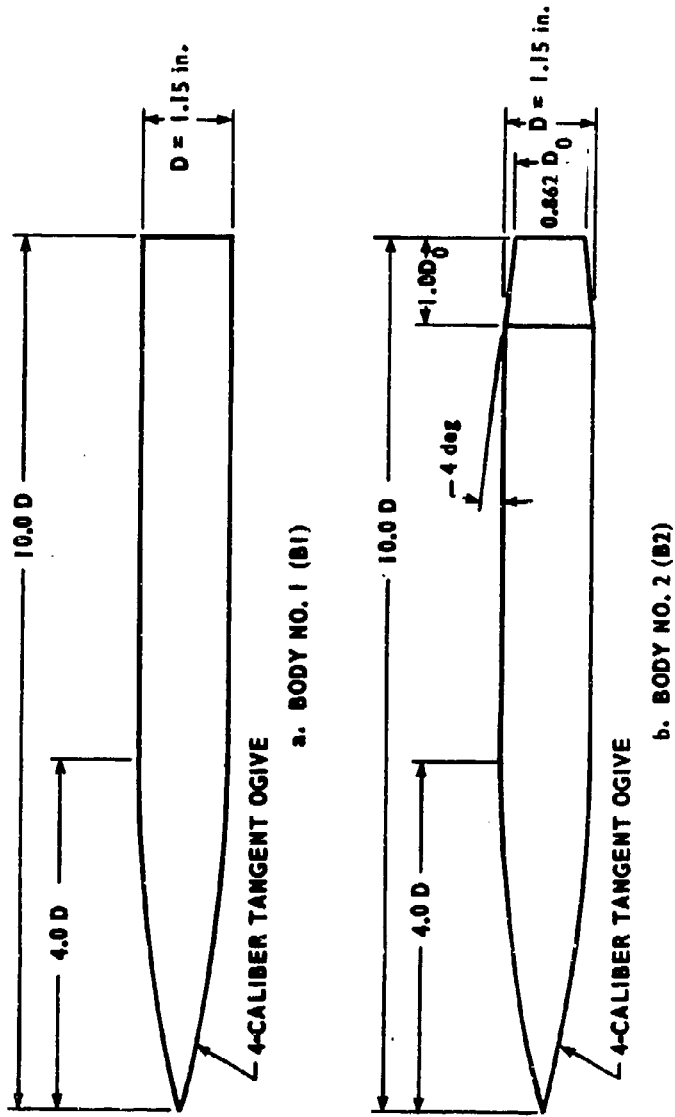
FIGURE 1. BODY CONFIGURATIONS
