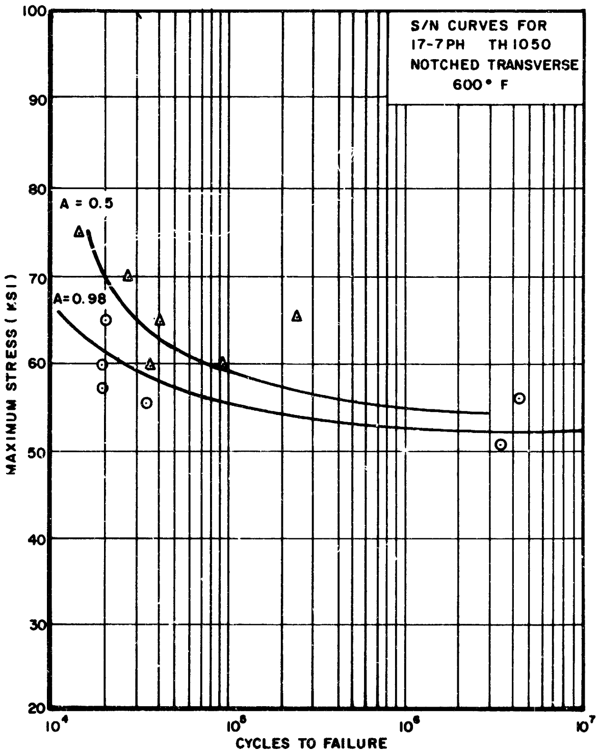
Figure 13. S/N Curves for 17-7 PH TH 1050, Notched Transverse, 600° F
