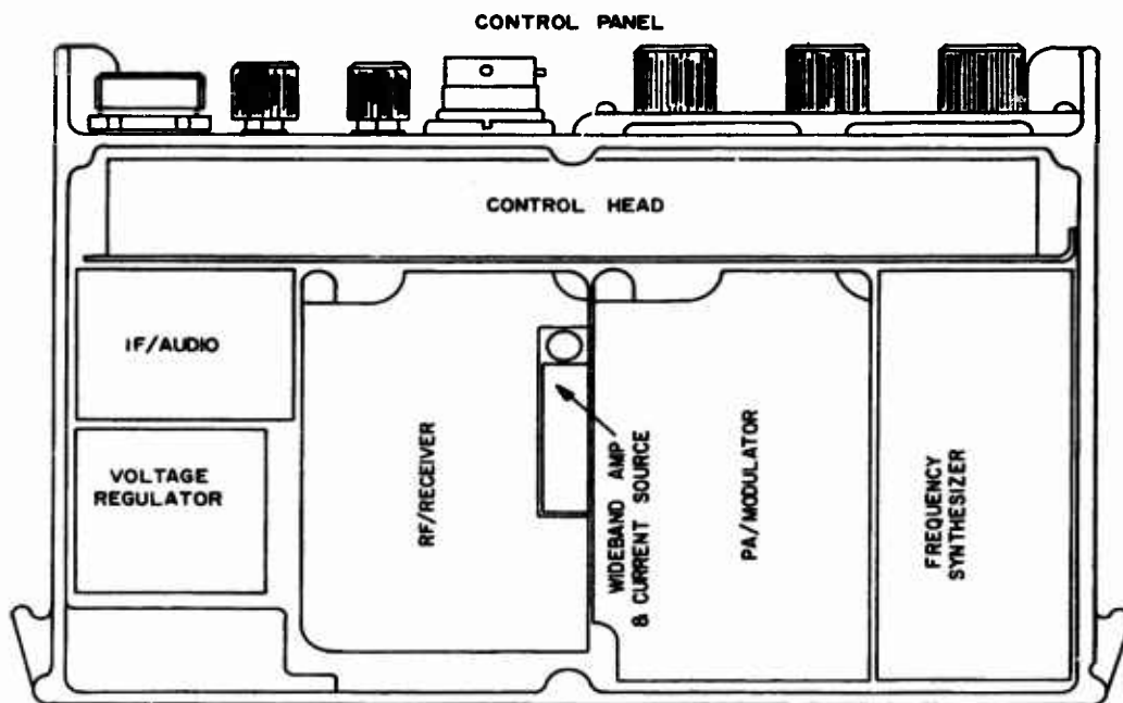
FIG 6-1 CHASSIS LAYOUT, CONFIGURATION "A"
