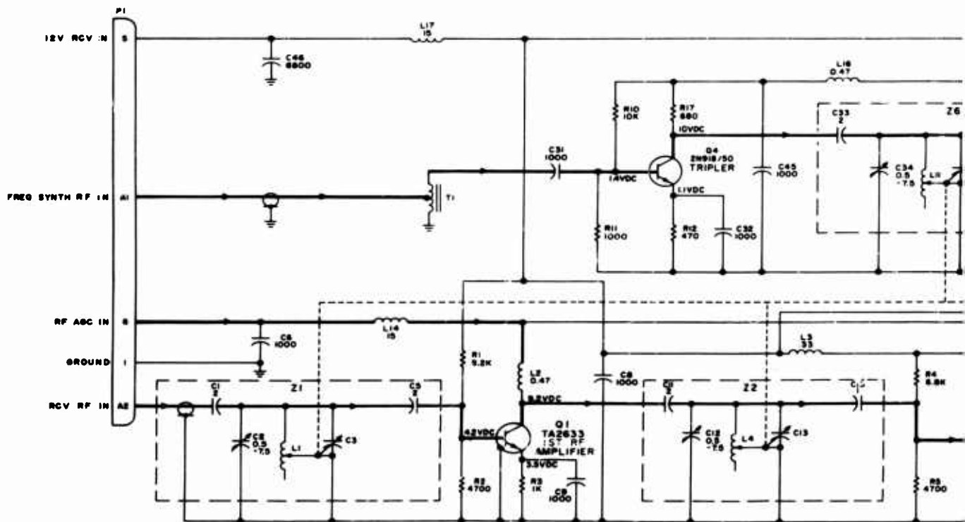
Figure AP-2 Receive RF Module 1A6, Schematic Diagram
