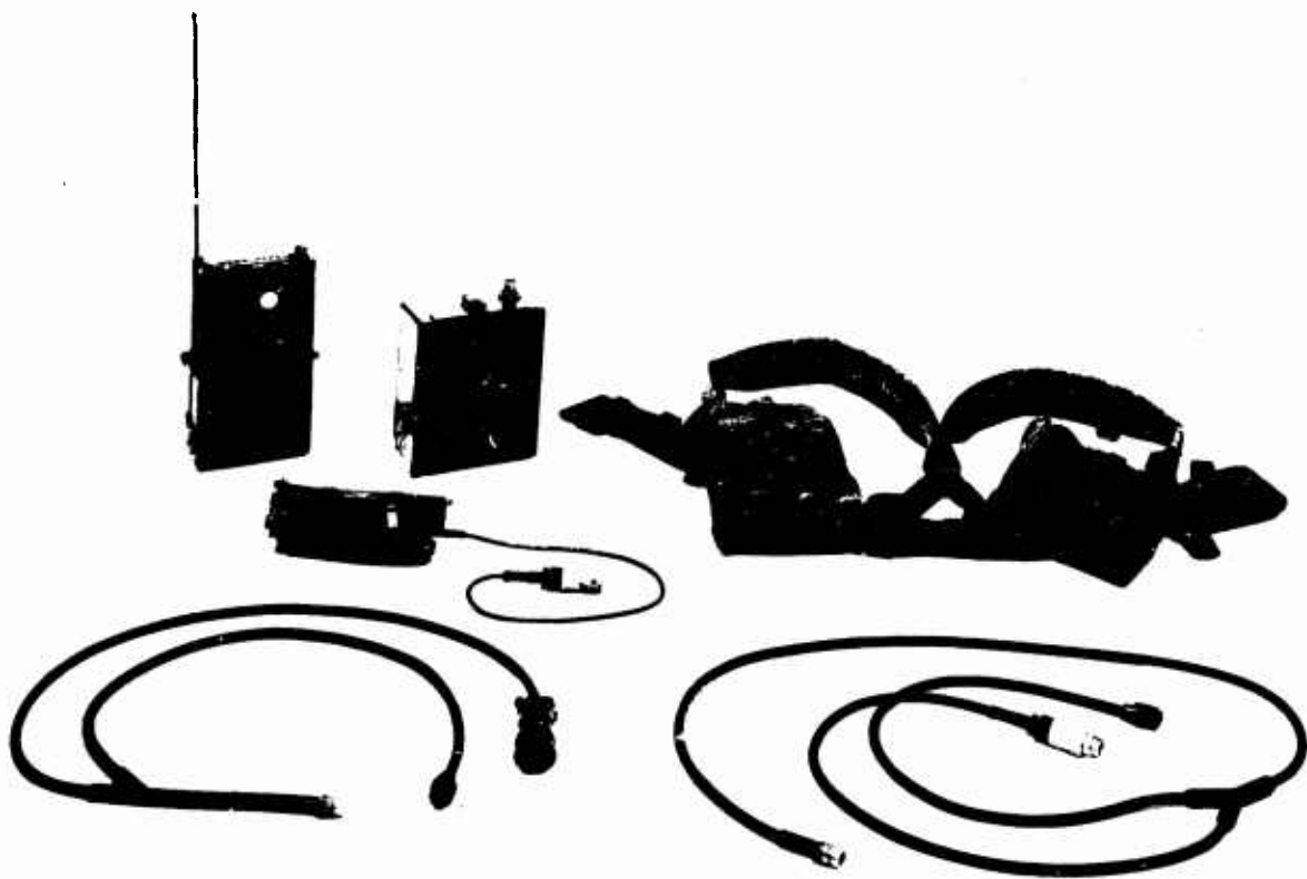
FIG. 2-5 AN/PRC-75 SYSTEM
