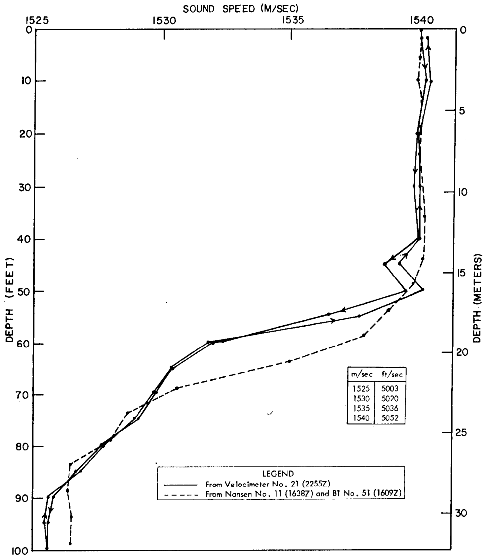
FIGURE 3. SOUND SPEED PROFILE - CONSECUTIVE STATION 24
