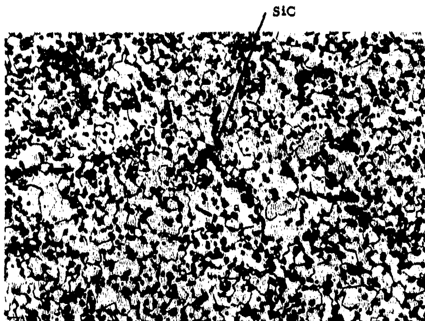
Figure 6. HfB 2 + SiC (A-4), 1/2" Diam. Bar, Transverse Section.
