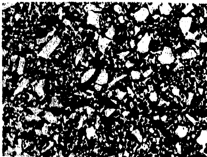
Figure 12. Microstructural Characteristics of HfB 2.1 + SiC (A-7) (Twenty Volume Per Cent SiC) Density = 7.84 gms/cm 3 , 82.5% of Theoretical Density.
