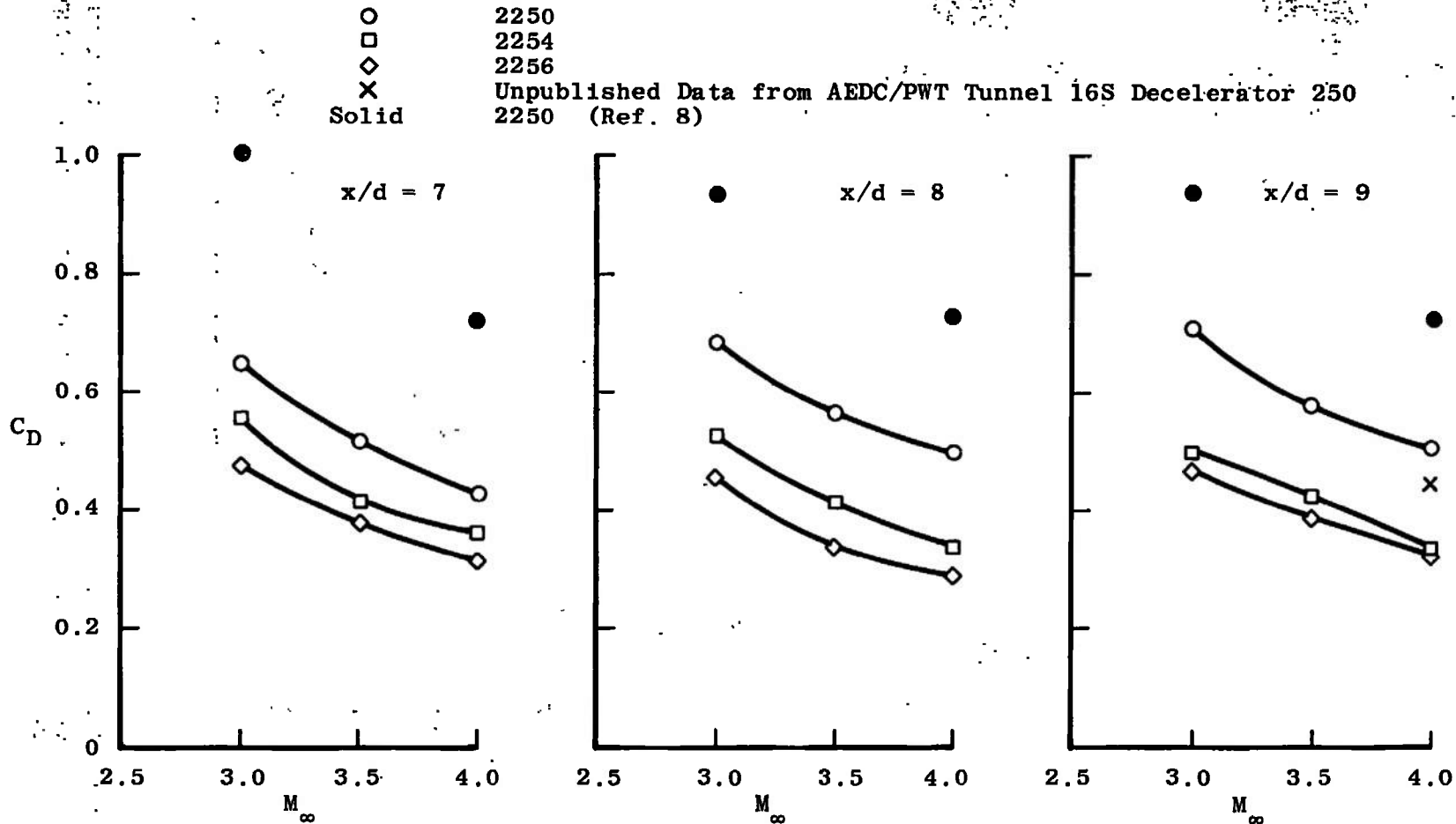
a. Variation of Drag Coefficient with Mach Number Fig. 4 Performance Data for Supersonic X Configurations Located in the Wake of a Cone-Cylinder Model
