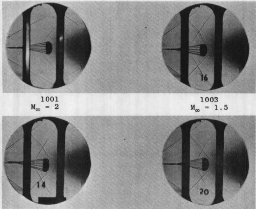
1002 M_\infty = 1.5
