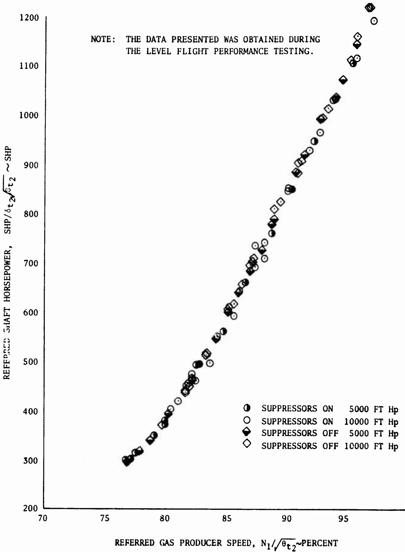
FIGURE 7 ENGINE CHARACTERISTICS T53-L-7 ENGINE S/N LE05249
