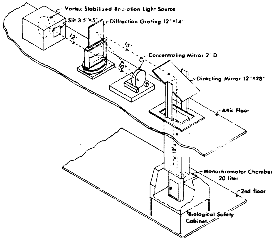
FIGURE 3. Monochromator Chamber System.
