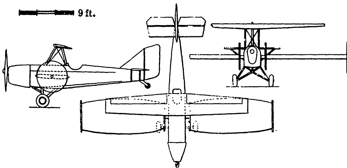
Figure 9. The Chappedelaine-Desgrandechamps-Caudron "Aérogyre" Being Rigged and Shown in Three Views. Several Flights in 1934. Lower Wings Rotate and Lock for STOL Conversion. (Refs. 16C through 26C).
