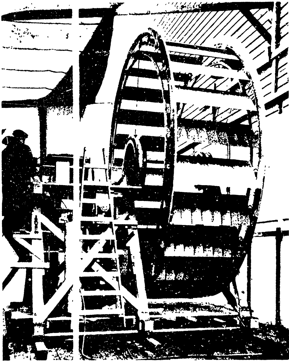
Figure 74. 15-Foot-Diameter Kirsten-University of Washington Pi-Pitch Cyclogiro Wheel. Designed and Constructed During 1922. Number of Blades Variable up to 24. See Ref. 24K.
