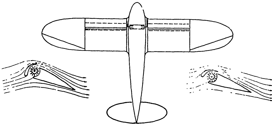
Figure 40. Lippisch Patent (Ref. 56L) Describing Rotating Airfoil Slat (RAS) Device and Boundary Layer Energizer.
