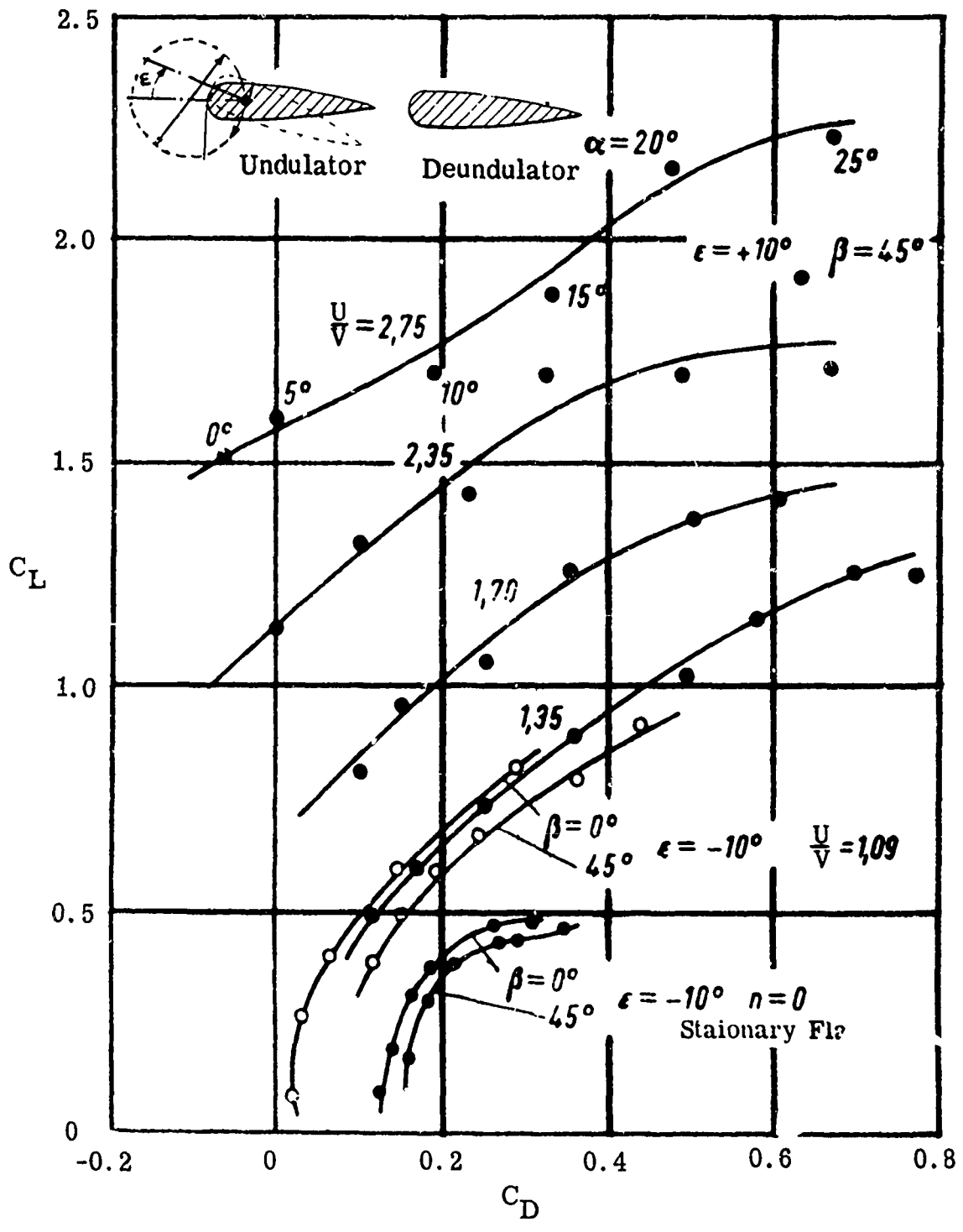
Figure 54. Wind Tunnel Results by Schmidt on Air Vehicle of Figure 55. Curves Are Aerodynamic Polars With Undulator in Rotation and Stopped. Note Thrust at U/V = 2.75 , C_L = 0^\circ (Ref. 54S).
