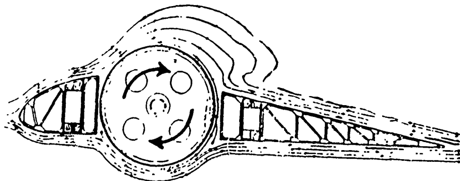
Figure 28. Typical Rotating Cylinder In Wing (RCIW) Arrangement by Thompson (Ref. 29 T).
