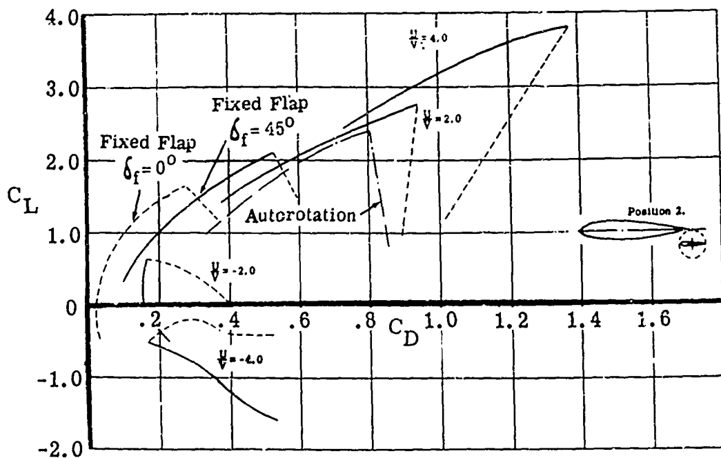
Figure 45. Lift and Drag Polars of a Fixed Wing with Trailing-Edge Rotating Airfoil Flap. Flap in Powered Rotation, Autorotation, and in Braked (Spoiler) Rotation. From Crabtree (Ref. 52C) and Küchemann (Ref. 51K).
