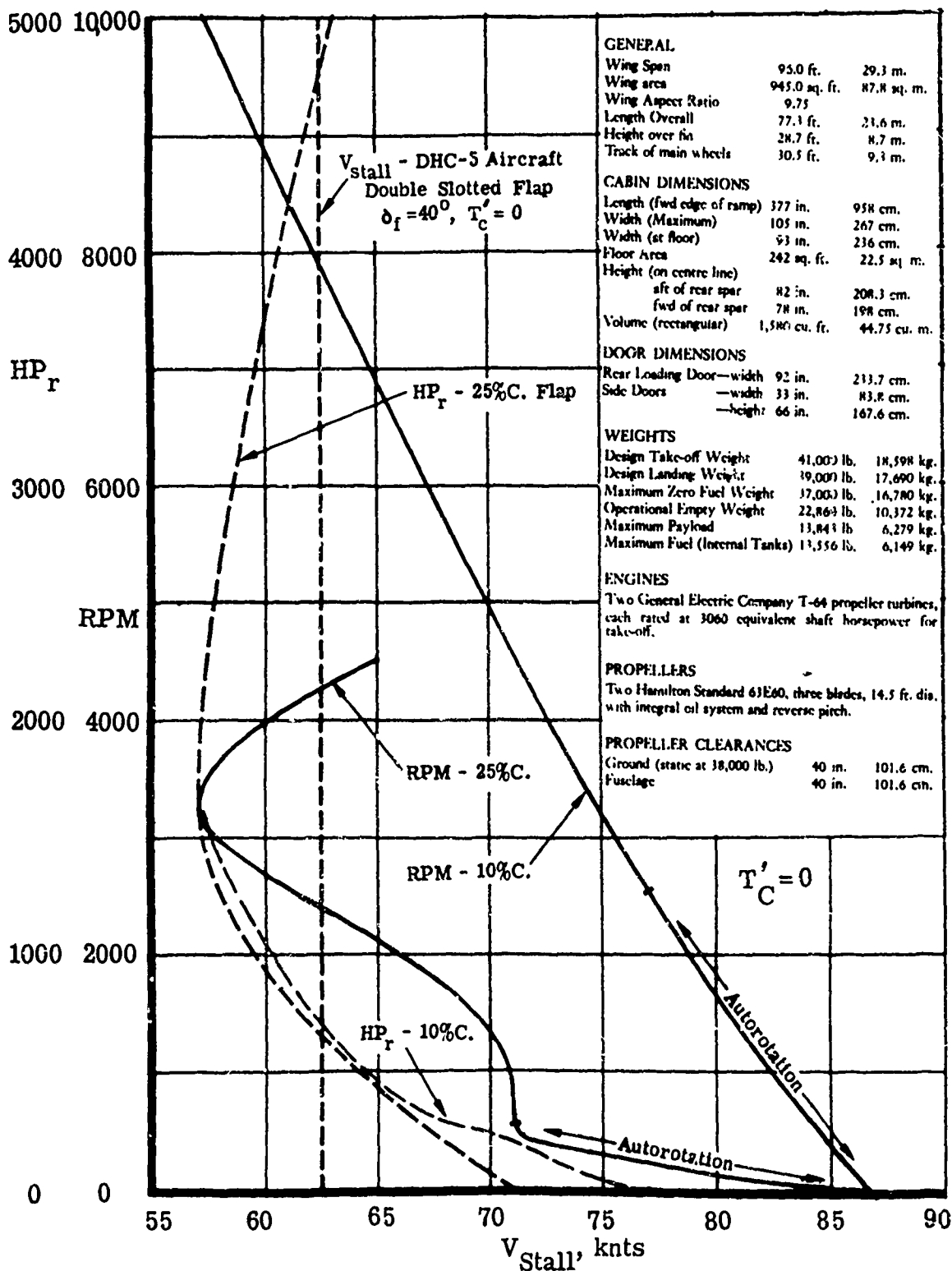
Figure 139. General Characteristics and Horsepower Required to Achieve C_{Lmax} . ( V_{Stall} ) With RAF on DHC-5 STOL-Type Aircraft.
