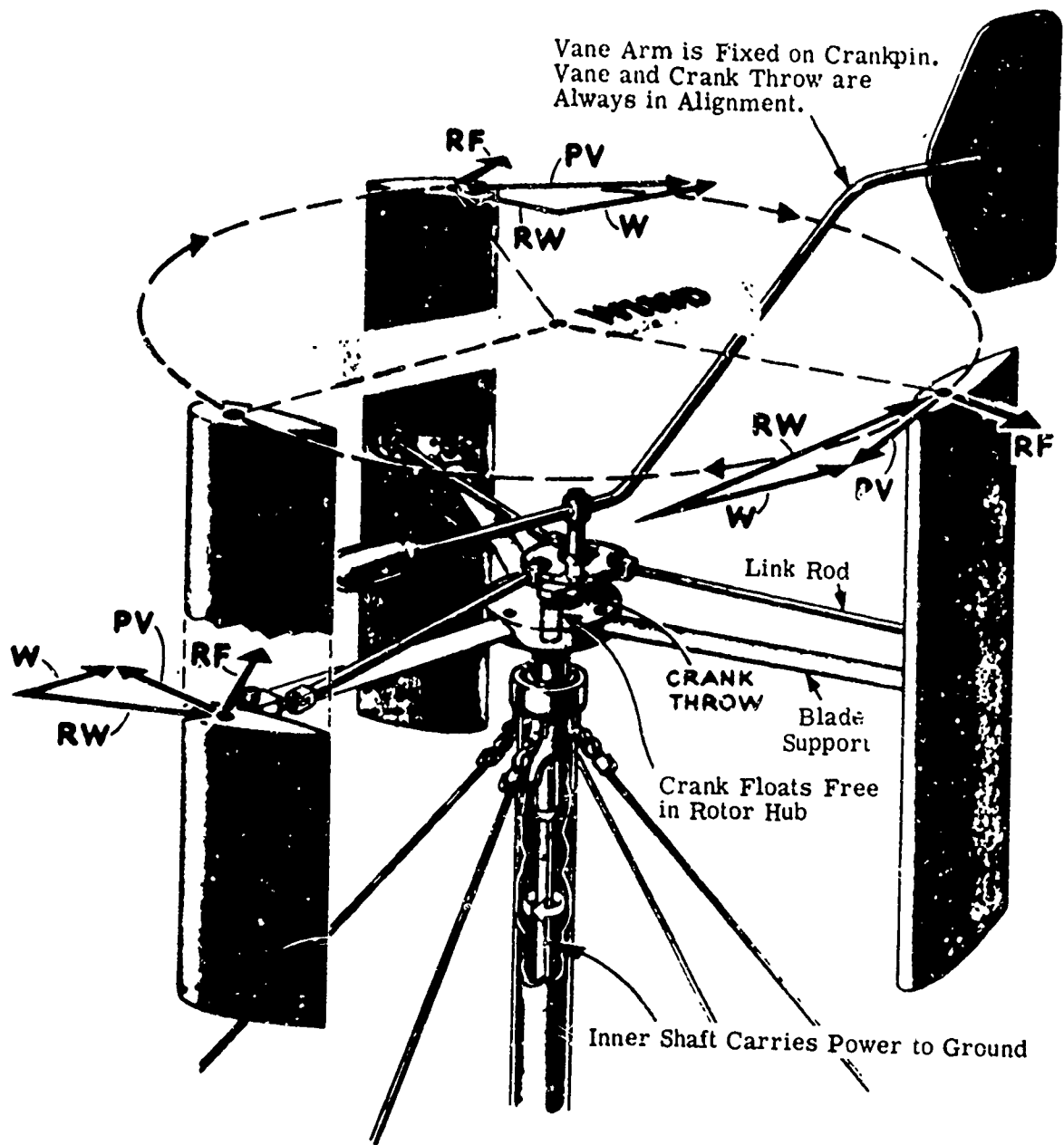
Figure 129. Horizontal Windmill of the Cyclogiro Type by Donaldson (Ref. 19D). Essentially an Autorotating Low-Pitch Cyclogiro Delivering Power Through a Vertical Shaft.
