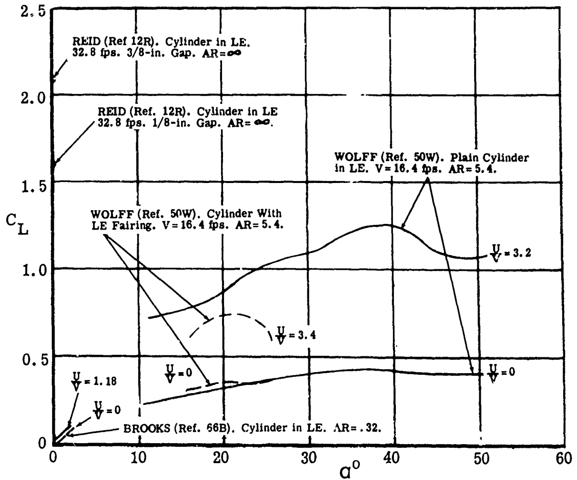
Figure 26. Measured Lift Coefficients Plotted Against Angles of Attack for a Collection of Combination Fixed Wing and Rotating Cylinder Slat System. Cylinder in the Leading Edge.
