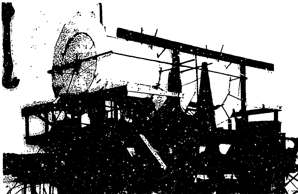
Figure 5. Navy-Assisted Magnus Effect Aircraft by Ames (1910) Mounted Atop Fast Steam Launch (Ref. 26A).
