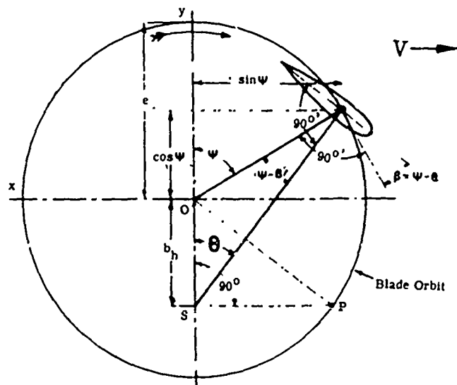
Figure 86. Geometrical Representation of Curtate Trochoidal Motion for a Cycloidal Propeller With Thrust and No Lift.
