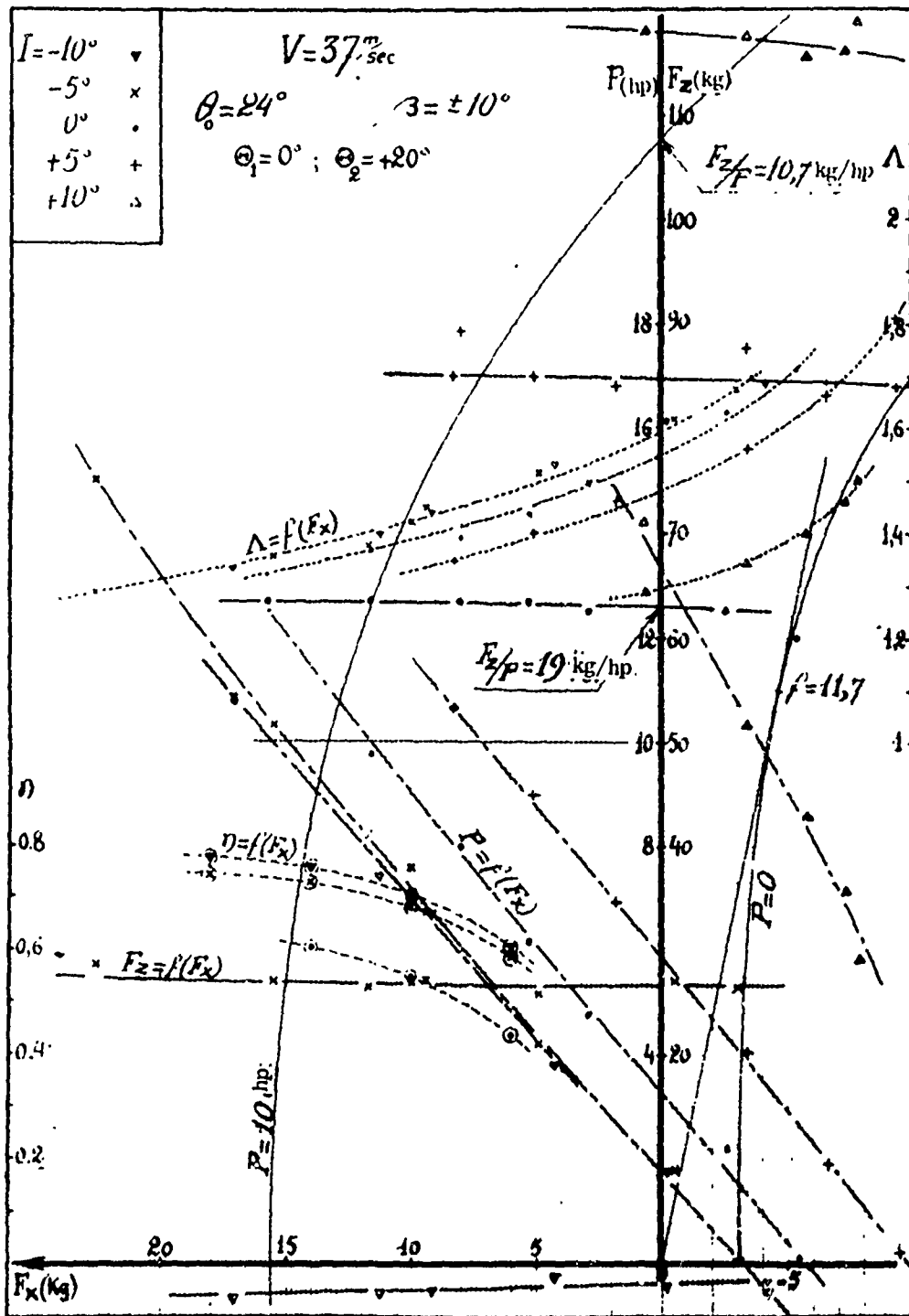
Figure 118. Forward Flight Performance, Horizontal and Inclined-Axis Richard Helicoplane, I = -10^\circ, -5^\circ, 0^\circ, +5^\circ, +10^\circ , O. N. E. R. A. 1948 Tests.
