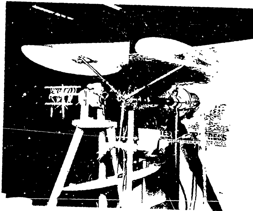
Figure 80. Cook "Cyclodyne" Project (1958-1968) Pictorial Presentation and Vibration Test Arrangement of Three-Bladed Wind Tunnel Model. Rotor Dia. 4 Ft., Span 4 Ft.
