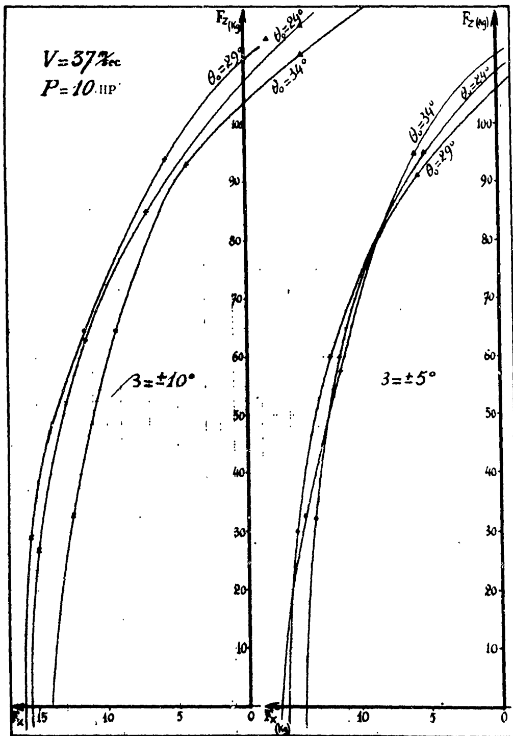
Figure 117. Forward Flight Polar, Horizontal-Axis Richard Helicopters O. N. E. R. A. 1948 Tests.
