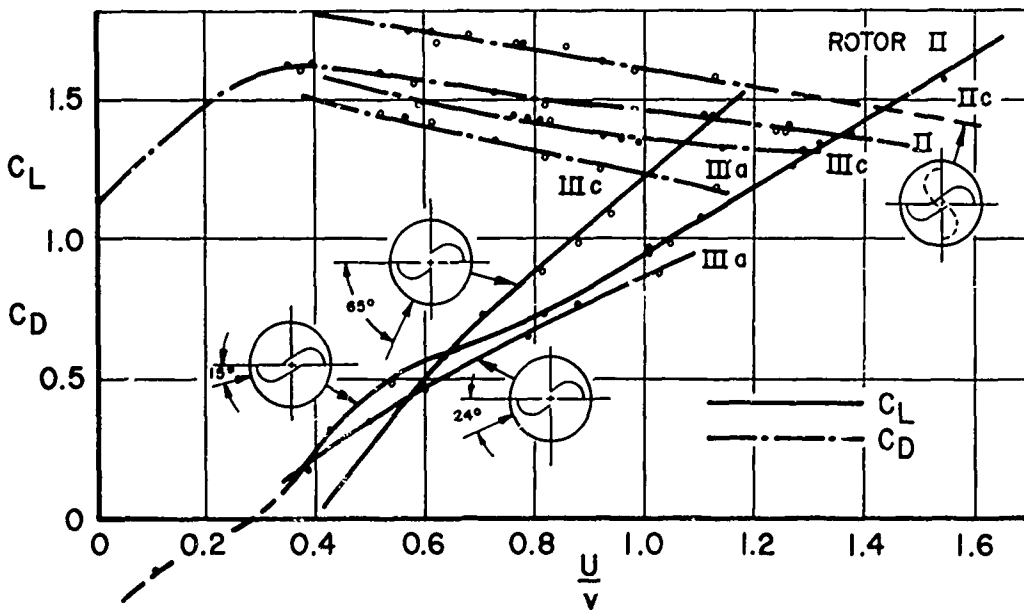
Figure 126. Aerodynamic Performance of a Collection of Basic and Modified Savonius Wing Rotors Through Power Extracting (Braked) U/V Range up to U/V Max. in Free Autorotation. From Ref. 3B.
