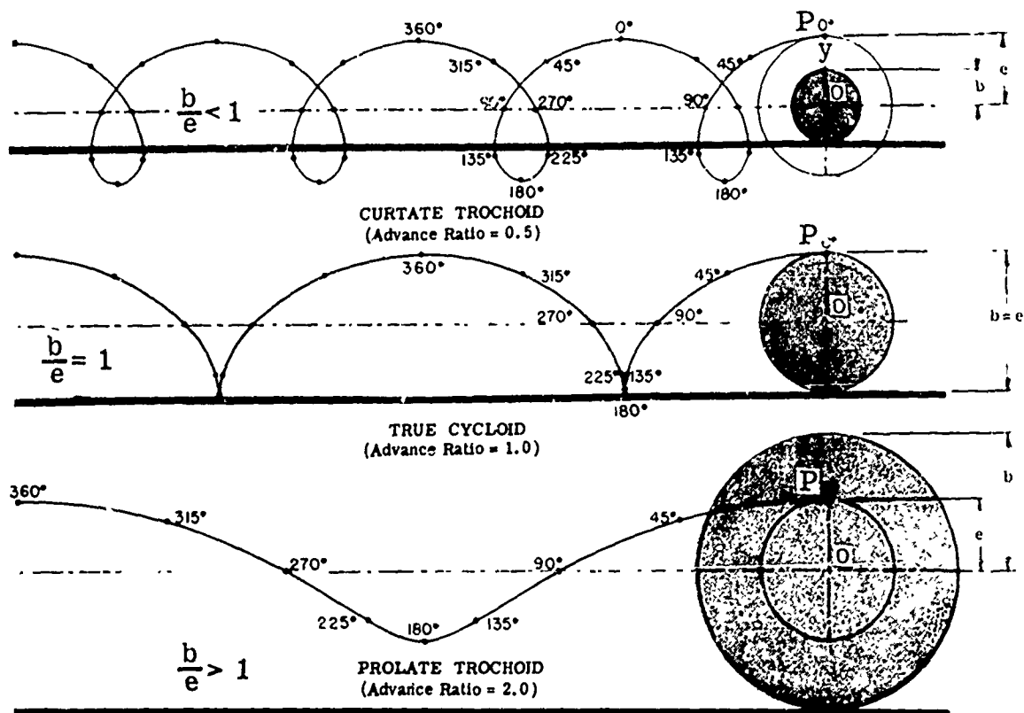
Figure 85. Kinematic Representation of Cycloidal and Trochoidal Motion. Numbers Show Angle thru which Generating Circle has Rotated.
