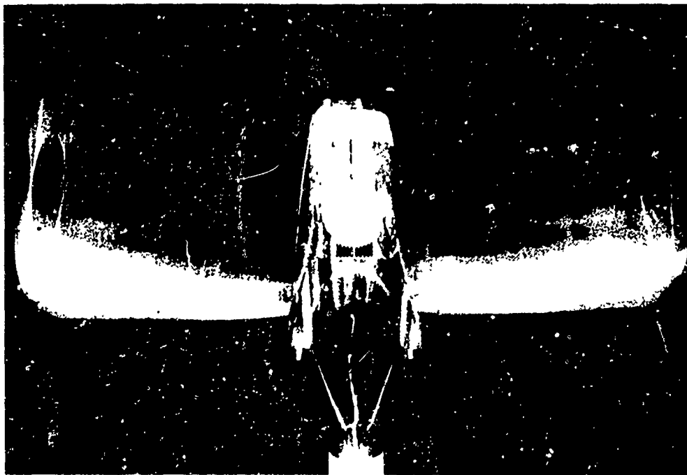
Figure 75. Kirsten-University of Washington Pi-Pitch Cyclogiro Model in Wind Tunnel. Built Before 1934 and Tested in a Variety of Configurations With and Without Tail Rotor. See Fig. 102 for Comparative Tunnel Installations. Also See Ref. 27K.
