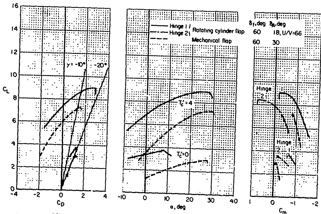
Figure 37. Comparative Performance of RCIF With Mechanical Flap (Ref. 57W).
