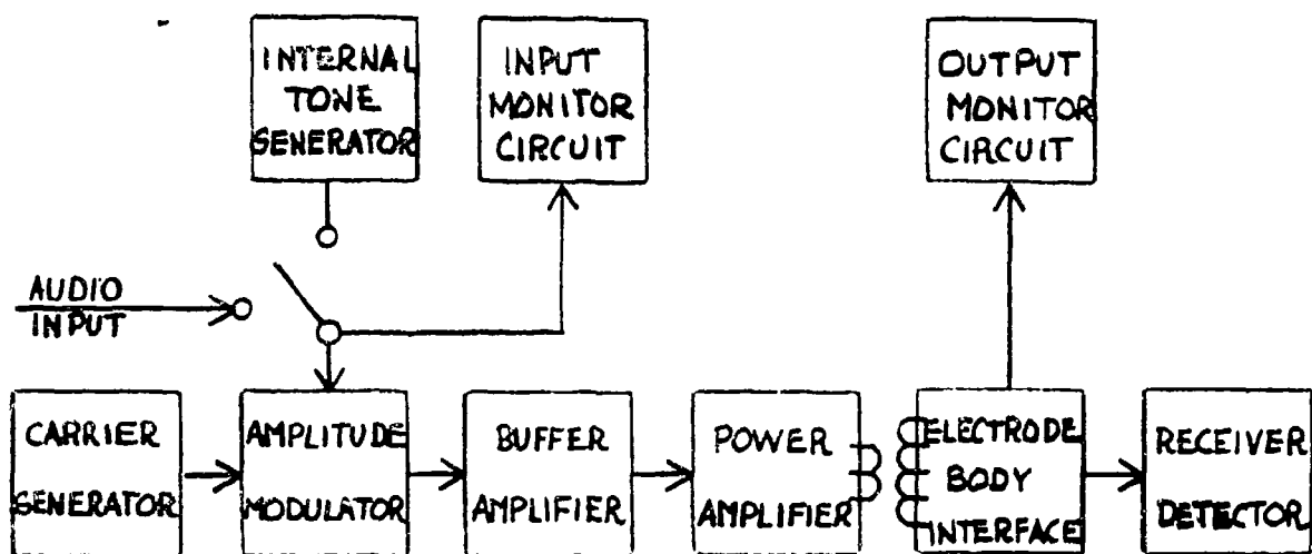
FIGURE 8. TRANS-DERMA-PHONE Block Diagram
