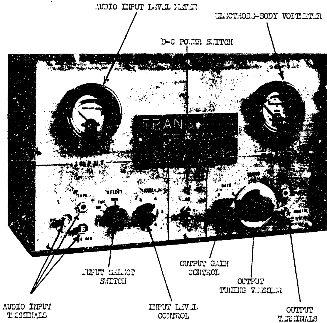
FIGURE 21. Front Panel View of TRANS-DERMAL-PHONE
