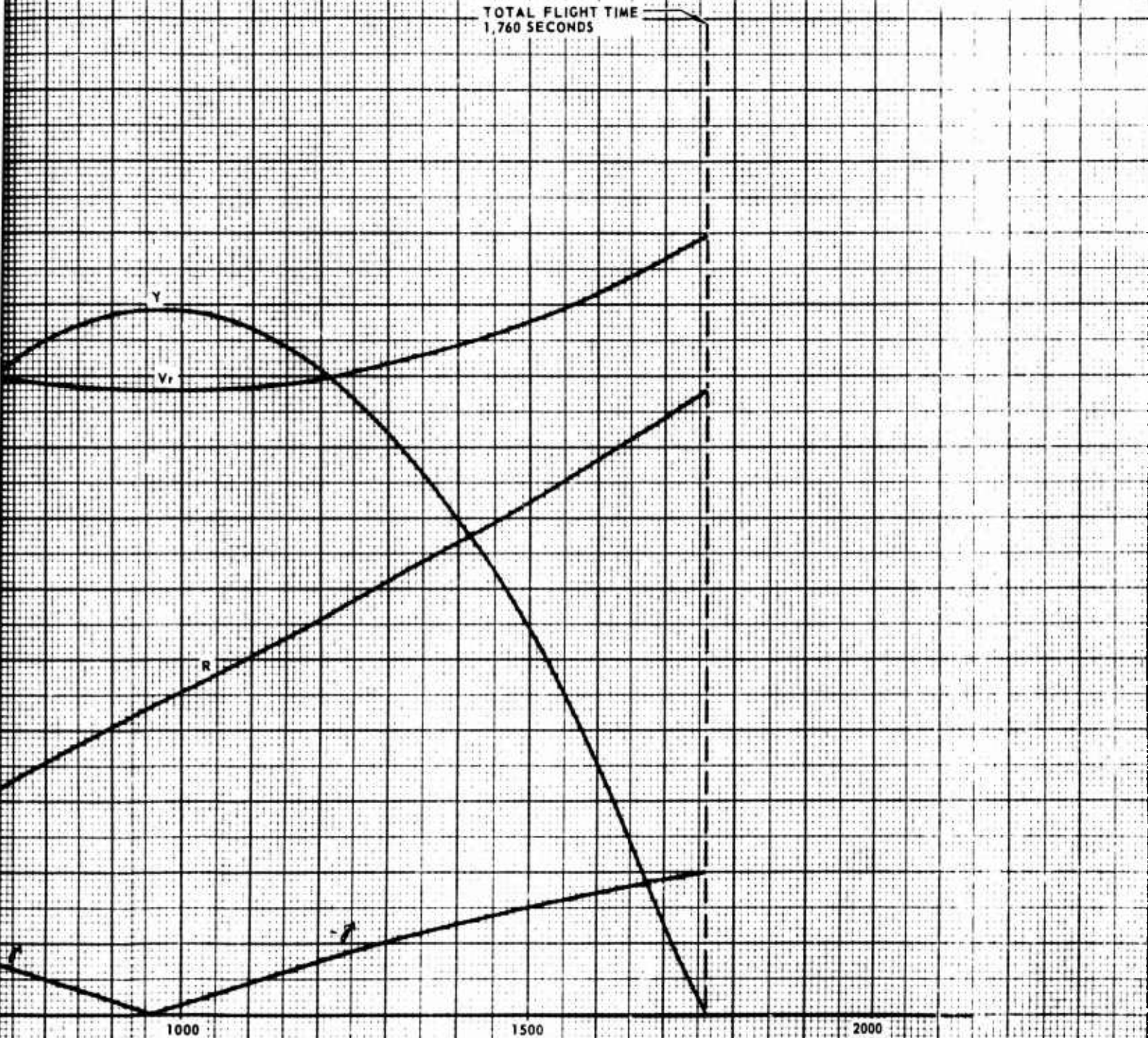
TOTAL FLIGHT PARAMETERS vs. TIME FOR E-R&D MISSILE CARRYING MARK 4 RV, MOD 1 DECOY, AND DUAL SP FOD (4400 NM RANGE) FIGURE 4
