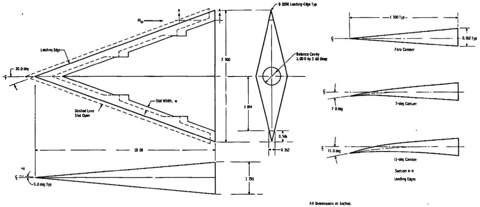
Fig. 2 Model Geometry
