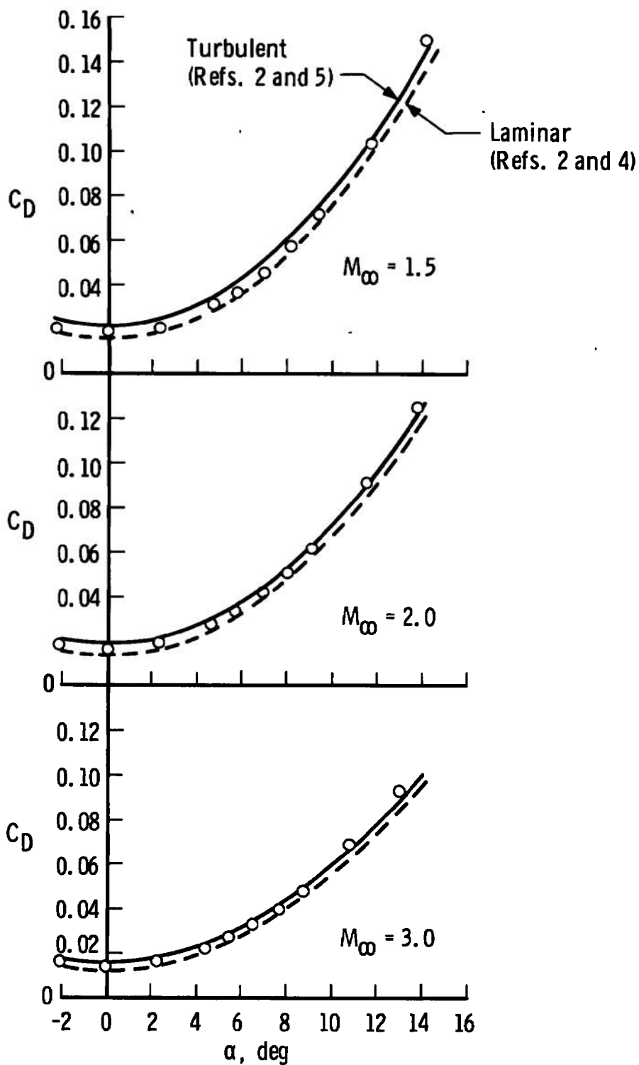
b. Drag Coefficient Fig. 3 Continued
