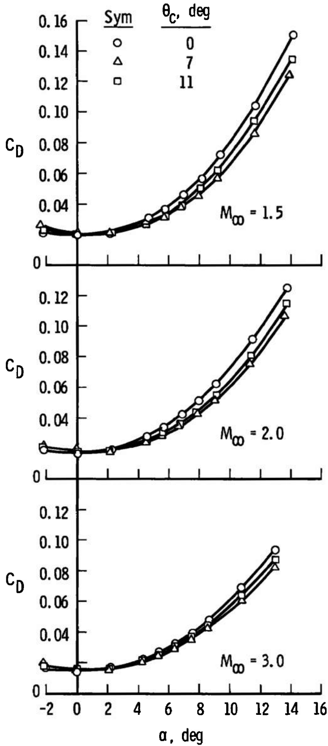
b. Drag Coefficient Fig. 4 Continued
