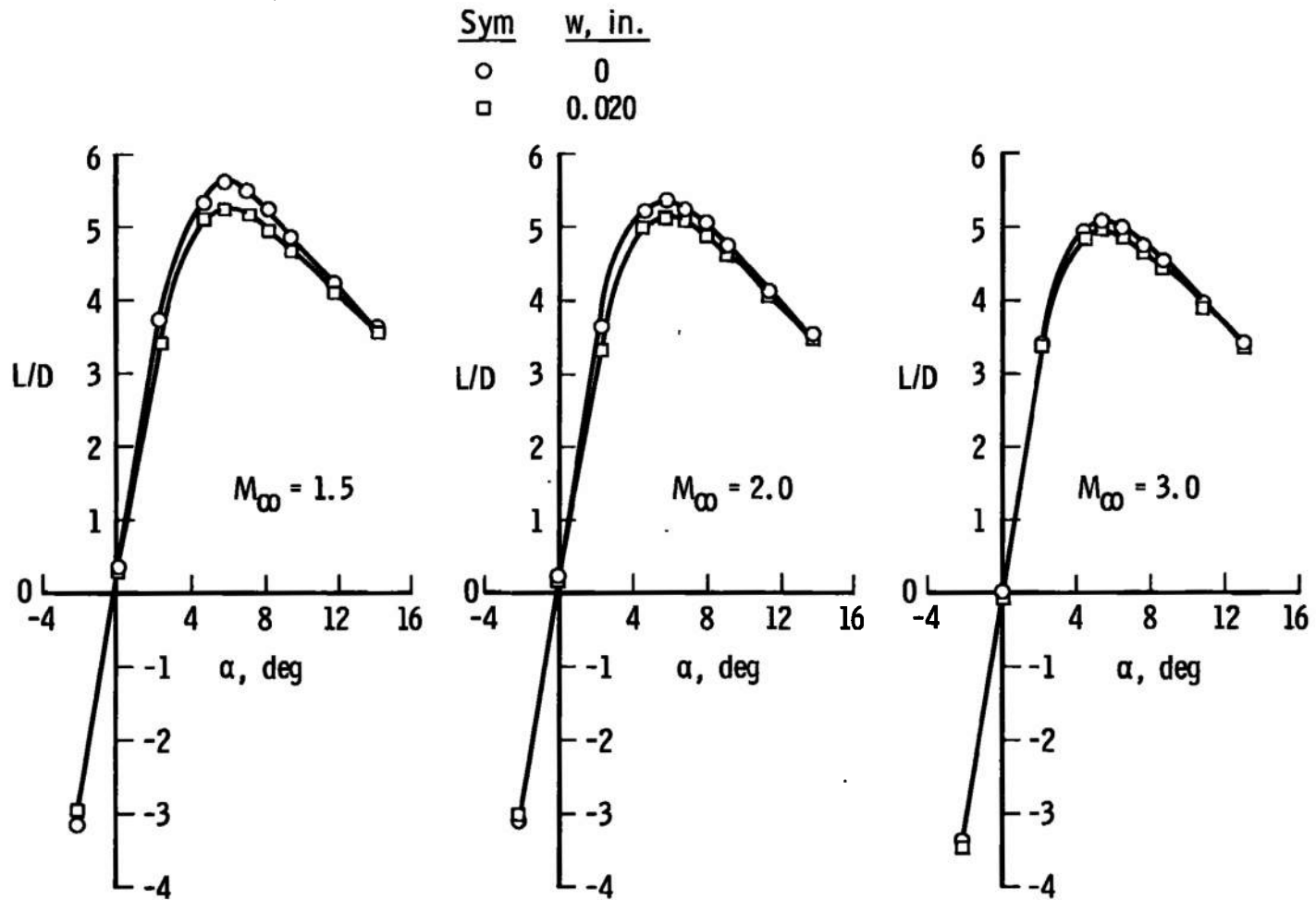
a. Variation of L/D with Angle of Attack
