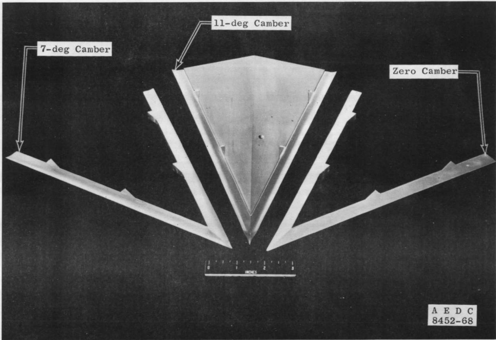
b. Centerbody with Leading Edges Fig. 1 Concluded
