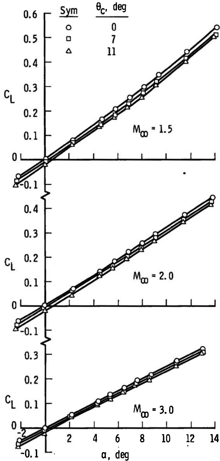
a. Lift Coefficient
