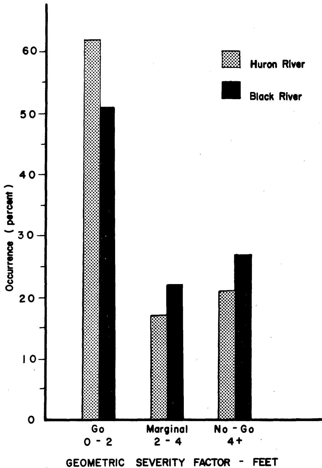
Estimated M-113 exiting performance for the Black and Huron Rivers using the geometric severity factor.
