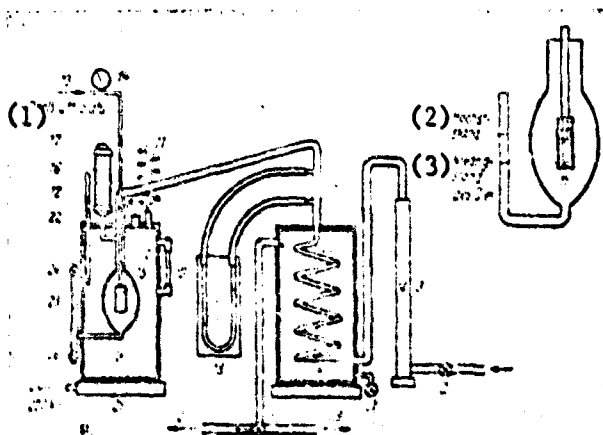
Figure 2. Diagram of fog generator. Legend: (1) compressed air, 5 ato; (2) maximum level; (3) low oil level.
