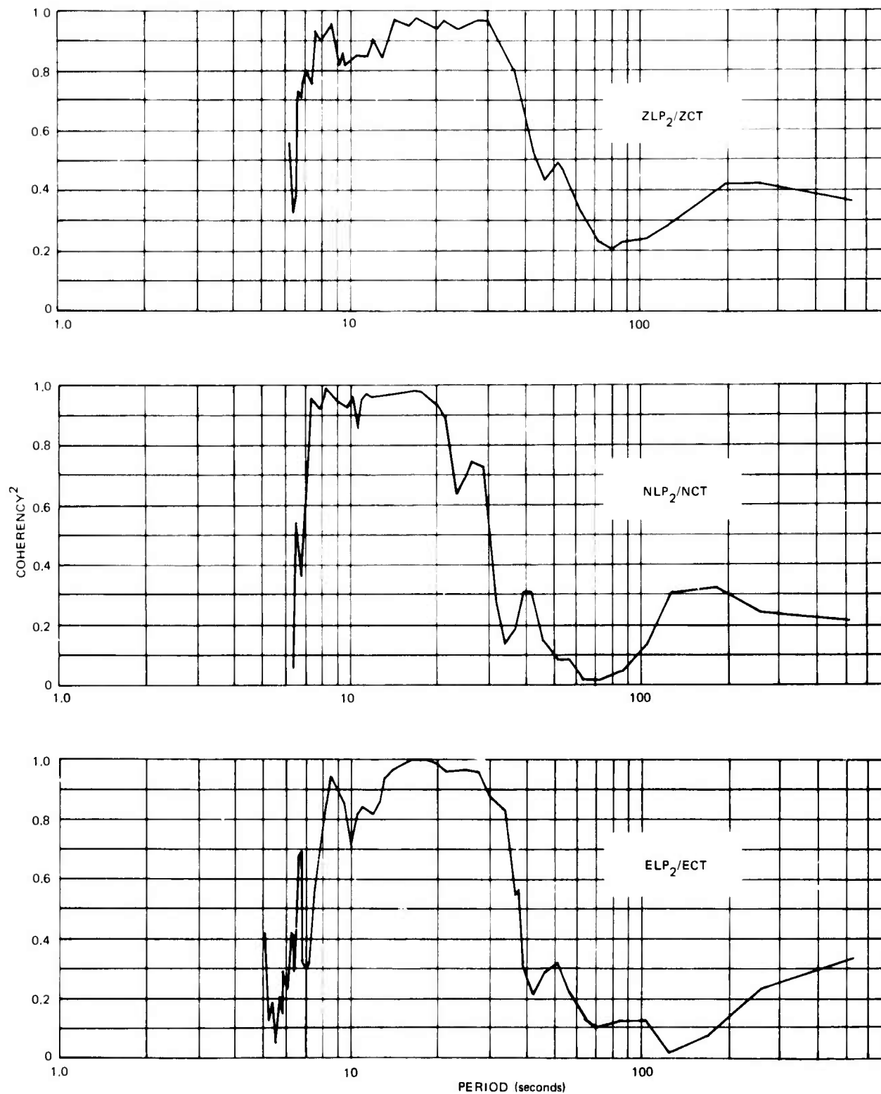
Figure 2. Coherency of the noise as recorded by the triaxial transformed (NCT, ECT, ZCT) and the standard (NLP 2 , ELP 2 , ZLP 2 ) long-period seismographs operating at UBSO during a wind free (wind velocity less than 5 mph) period
