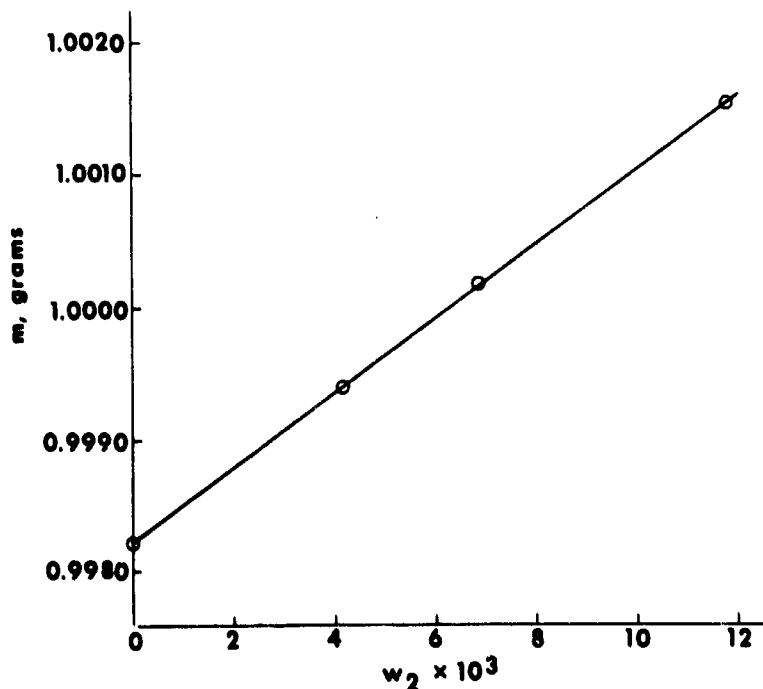
Figure 1. Plot of Mass of Pycnometer Contents (Normalized to 1 ml) Against Weight Fraction, w_2 , of Staphylococcal Enterotoxin B in Distilled Water.
