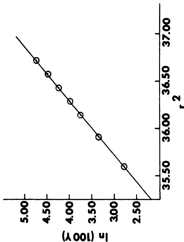
Figure 12. Plot of \log_e Fringe Displacements (100 Times the Fringe Displacement in Millimeters on the Photographic Plate) versus Square of Radial Position (in Centimeters) During Sedimentation Equilibrium of Staphylococcal Enterotoxin B. The toxin protein was run at a concentration of 7/12 mg/ml in 0.1 ionic strength Veronal buffer for 19 hours at a speed of 30,000 rpm and at 20 C. The molecular weight of the protein, calculated from the slope of the straight line, is 32,700 \pm 200 daltons.
