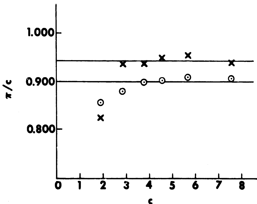
Figure 4. Plots of Specific Osmotic Pressure ( \pi/c ) versus c for Two Osmometry Experiments on Staphylococcal Enterotoxin B Suspended in 0.1 Ionic Strength, pH 8.6 Veronal Buffer. The horizontal, straight, least squares lines were drawn through the five points representing the final measurements made after equilibration of the membranes. Units: \pi in centimeters Veronal buffer, c in grams per liter.
