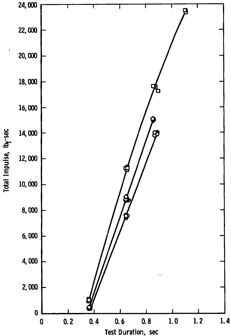
Fig. 20 Total Impulse of Bit Firings
