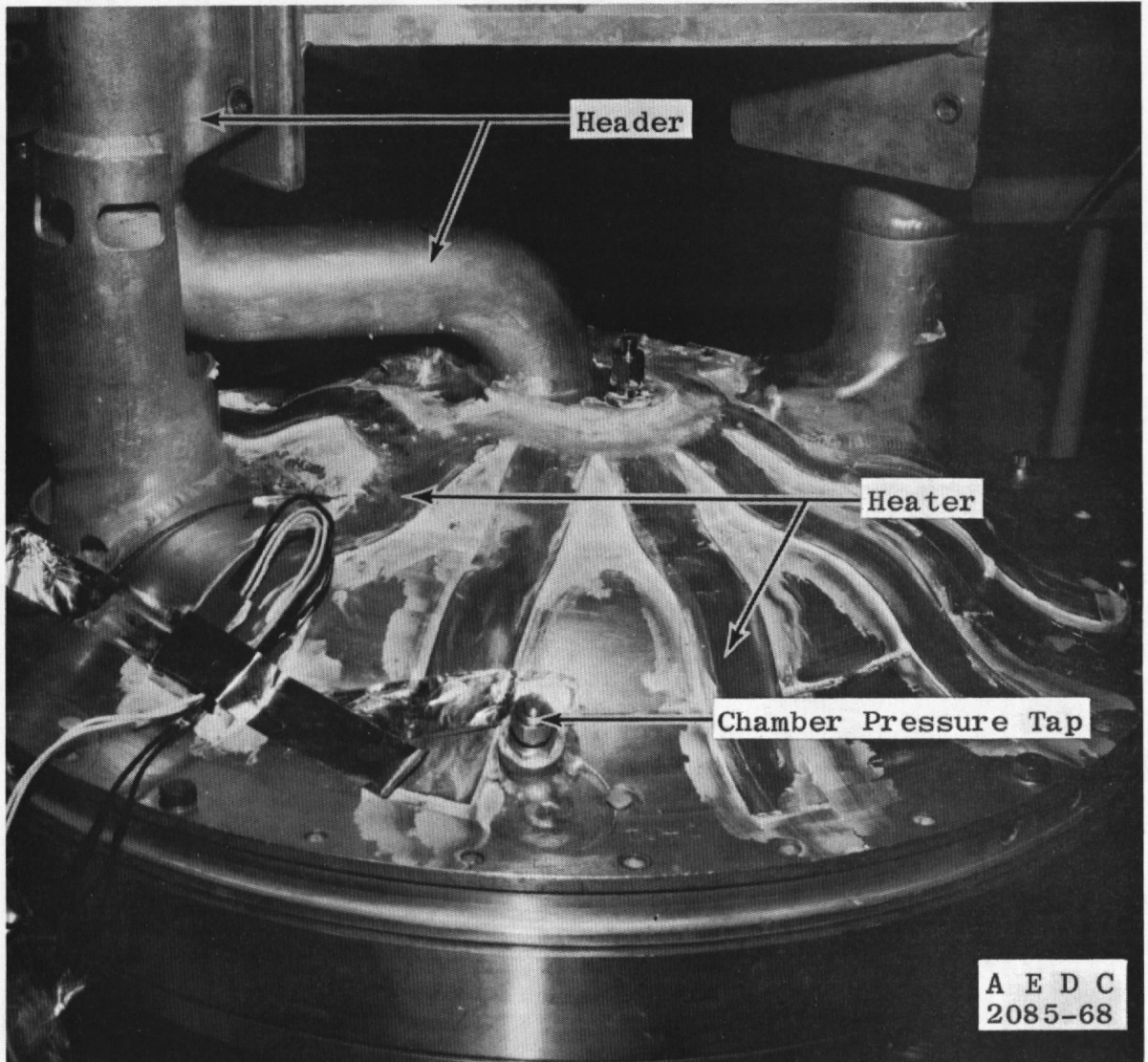
b. Injector Heater Installation Fig. 6 Concluded
