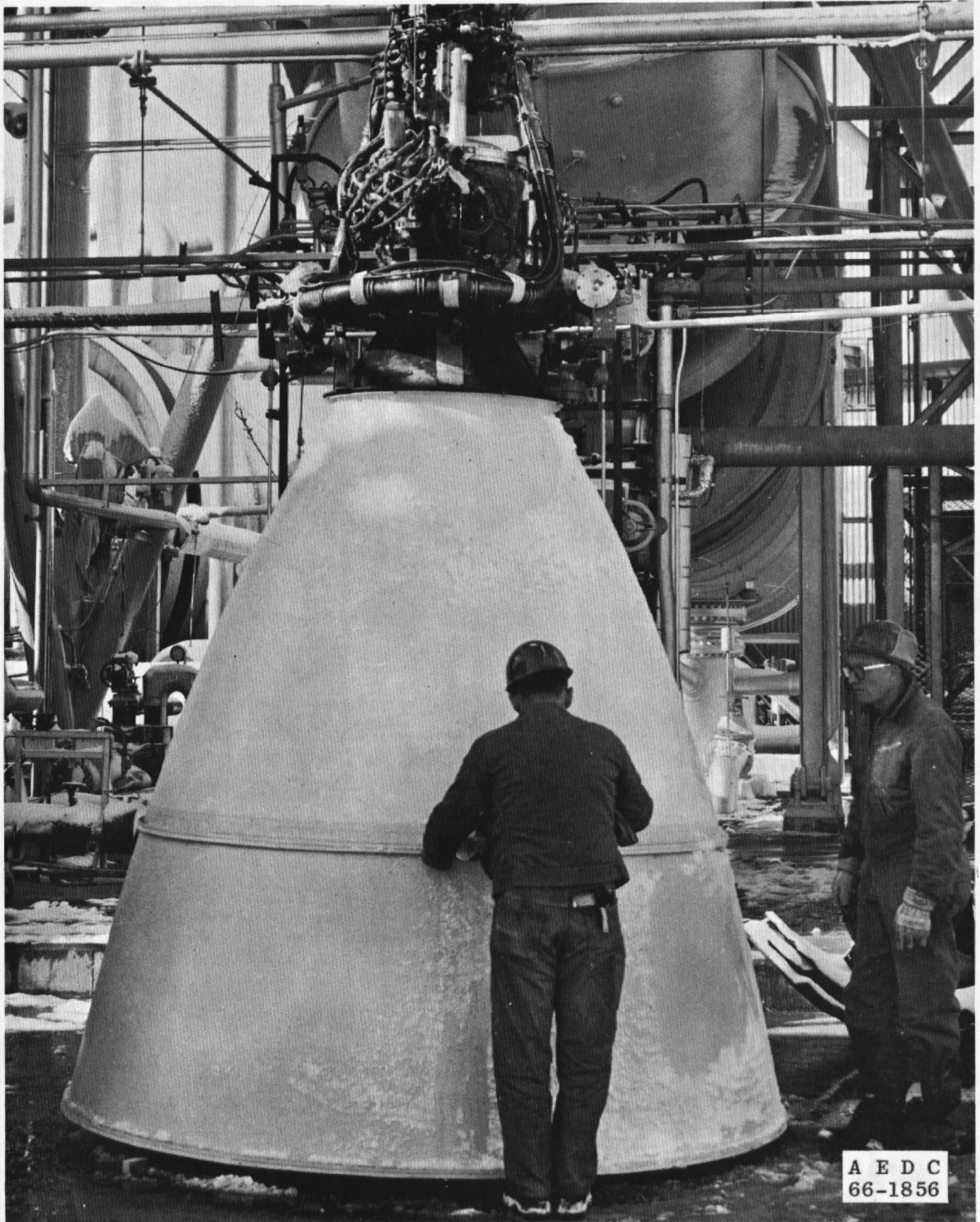
Fig. 1 The Apollo SPS Block II Engine
