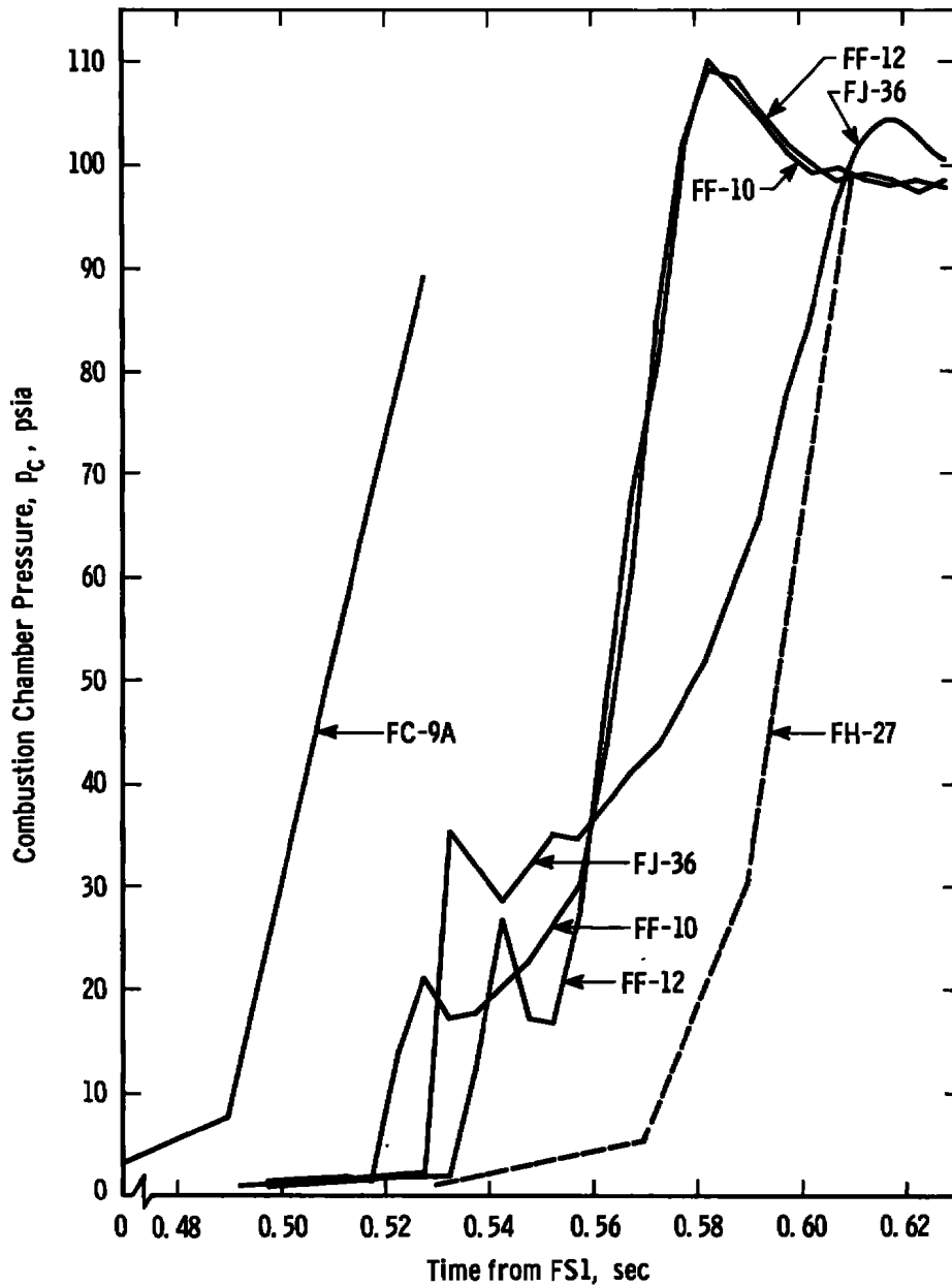
Fig. 17 Ignition Transient Chamber Pressure Profiles
