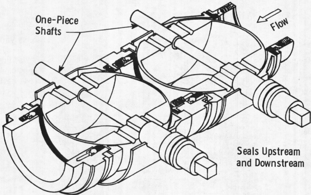
b. Mod I-C Design (Phase VI)
