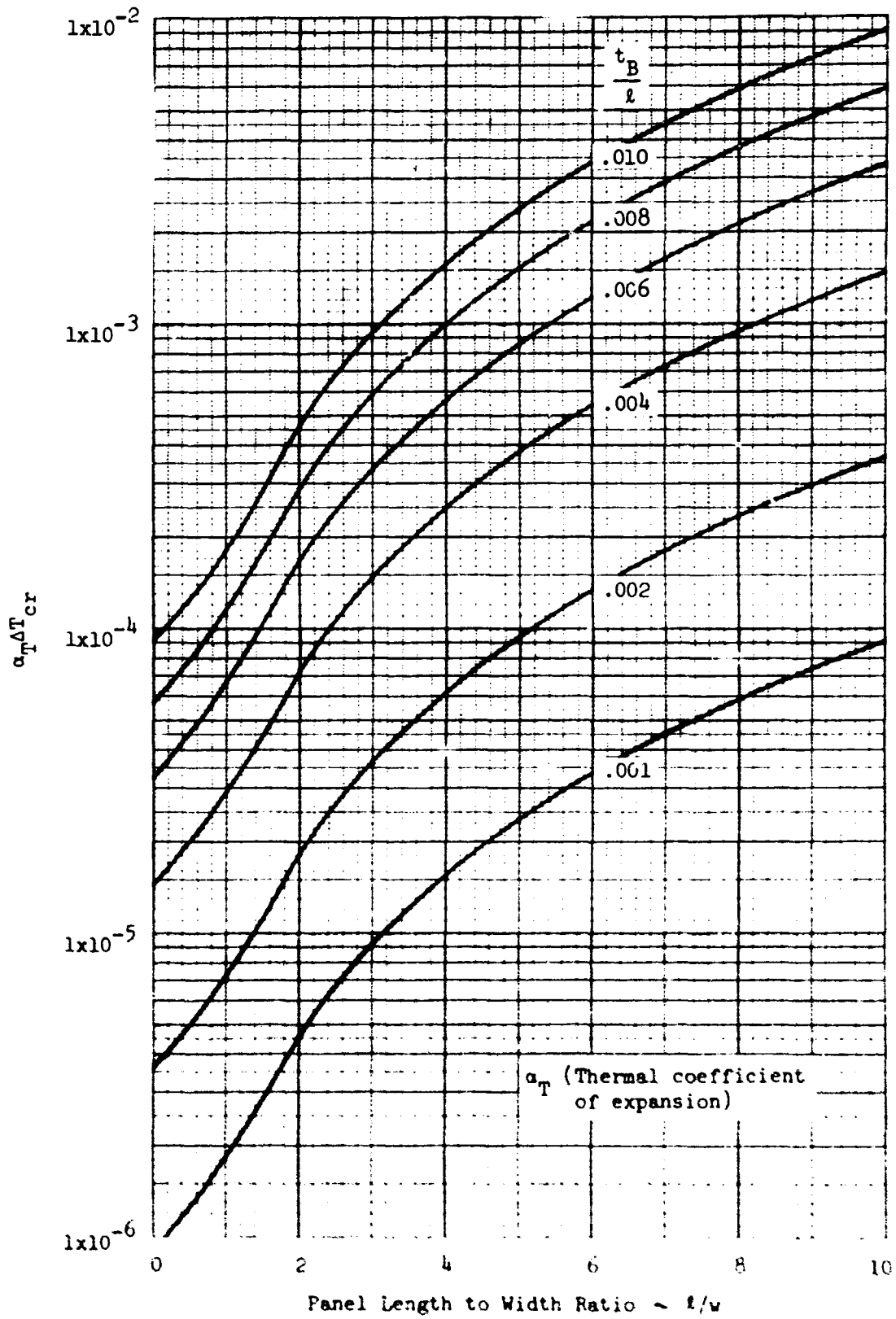
Figure 18 - Critical Differential Temperature of Simply Supported Rectangular Panel with Restrained Edges
