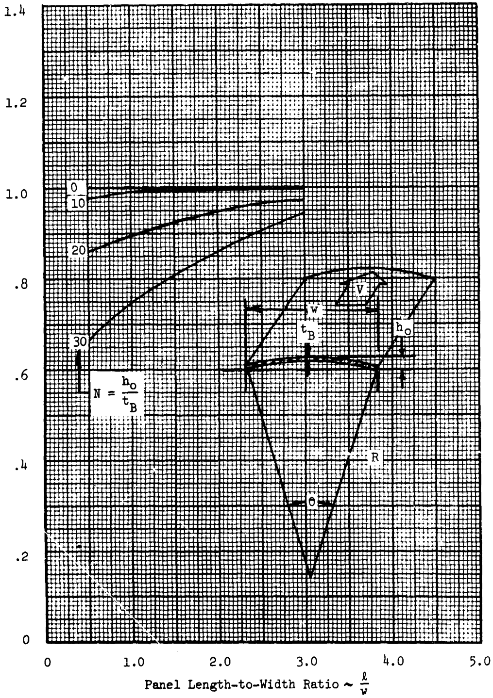
Figure 6 - Thickness Correction Factor for Curvature
