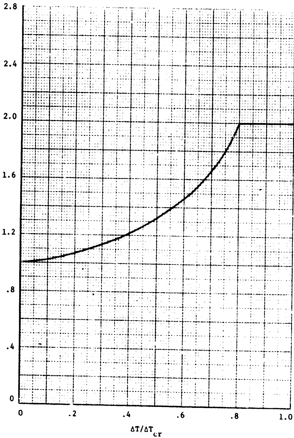
Figure 19 - Thickness Correction Factor for Differential Temperature
