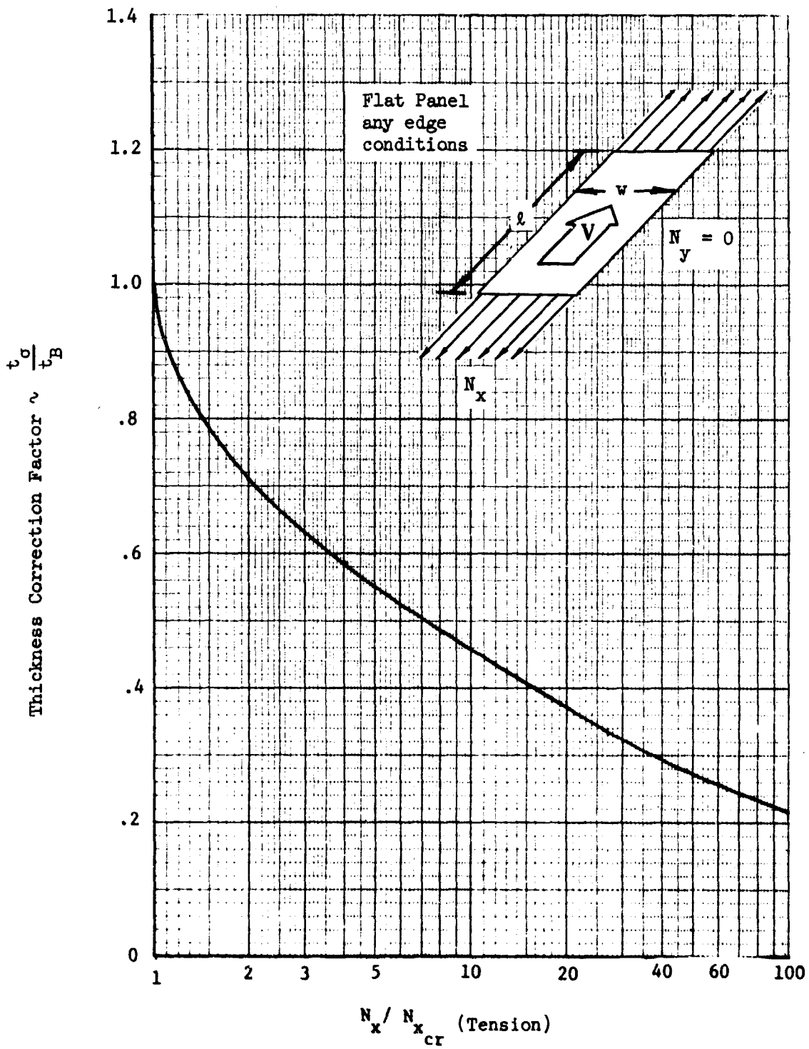
Figure 9 - Thickness Correction Factor for Stress (Tension)
