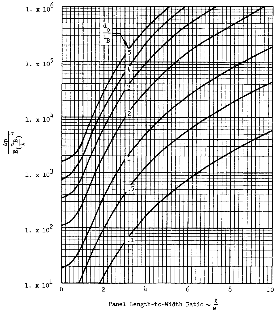
Figure 15 - Relationship Between \frac{d_0}{t_B} , \Delta p , and Panel Geometric-Physical Characteristics
