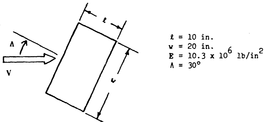
Figure 24. Panel Configuration for Sample Design Number 1
