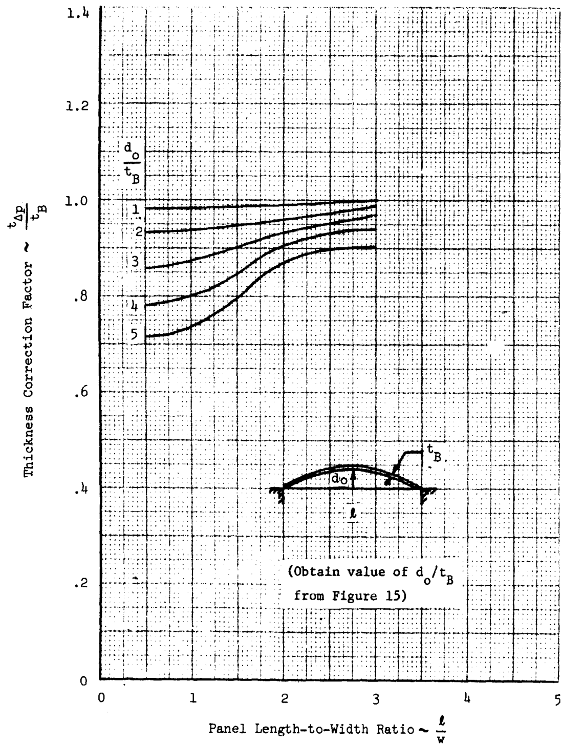
Figure 16 - Thickness Correction Factor for Differential Pressure
