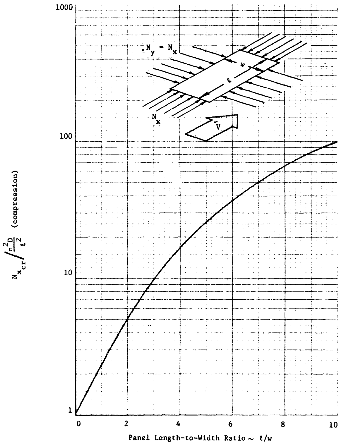
Figure 14 - Critical Inplane Compression Load for Simply Supported Panel, N_y = N_x
