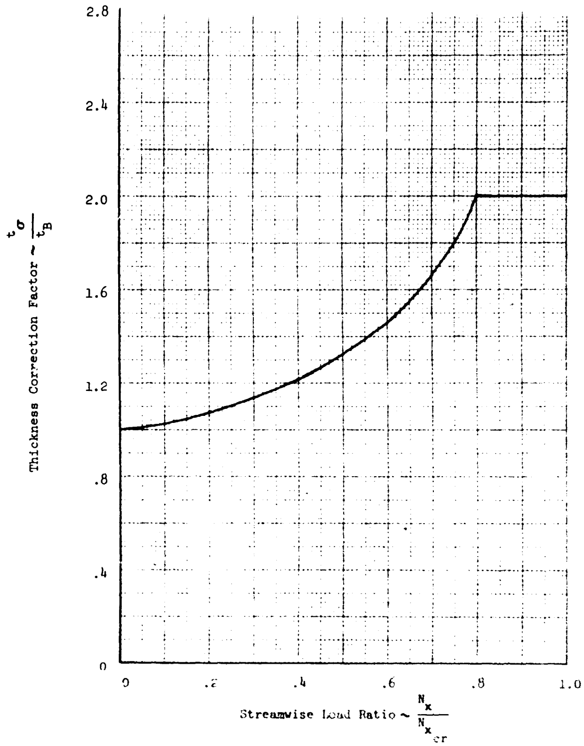
Figure 10 - Thickness Correction Factor for Inplane Stress (Compression)
