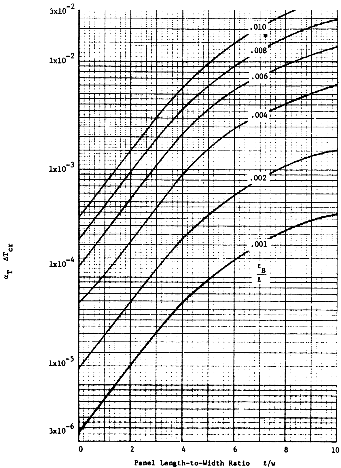
Figure 17 - Critical Differential Temperature of Clamped Panel with Restrained Edges
