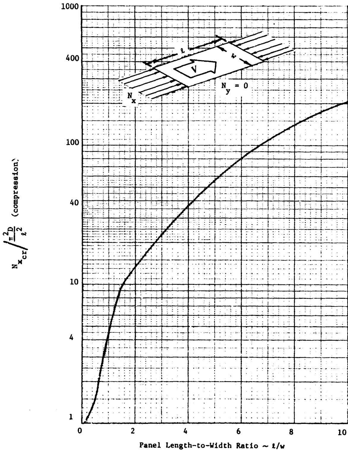
Figure 13 - Critical Inplane Compression Load for Simply Supported Panel, N_y = 0
