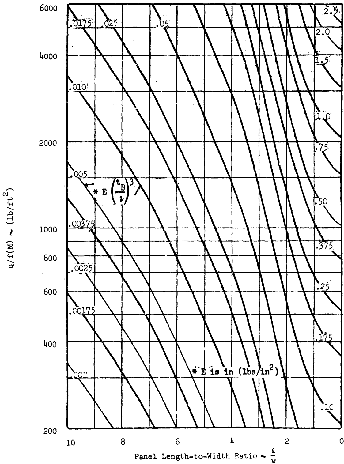
Figure 4 - Aerodynamic Parameter q/f(M) versus l/w with Variation in Structural Parameter E \left( \frac{t_B}{l} \right)^3
