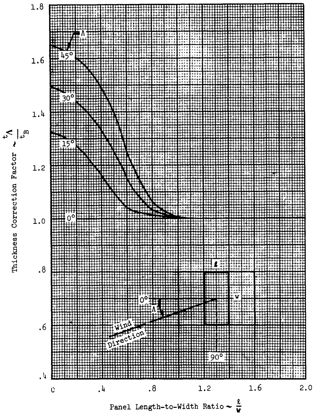
Figure 7 - Thickness Correction Factor for Flow Angularity
