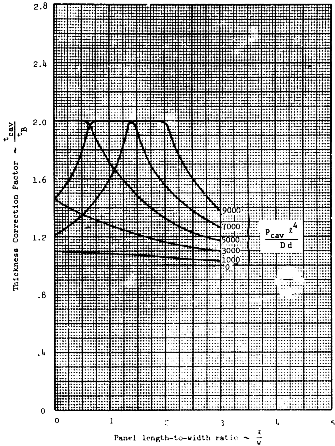
Figure 20 - Thickness Correction For an Enclosed Cavity
