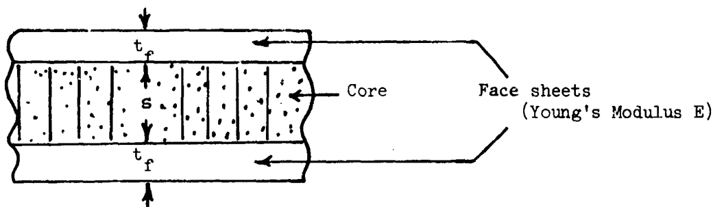
Figure 21 -Honeycomb Configuration for Analyzing Stiffness
