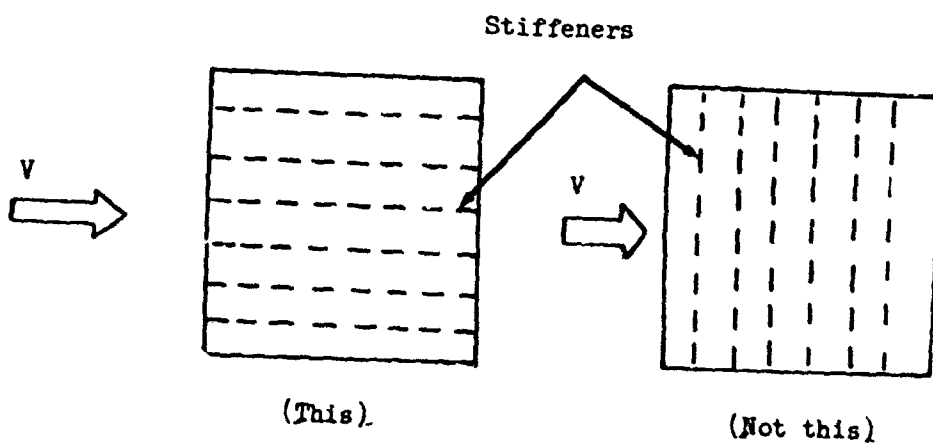
Figure 23. Orientation of Stiffeners to Obtain Higher Flutter Speed
