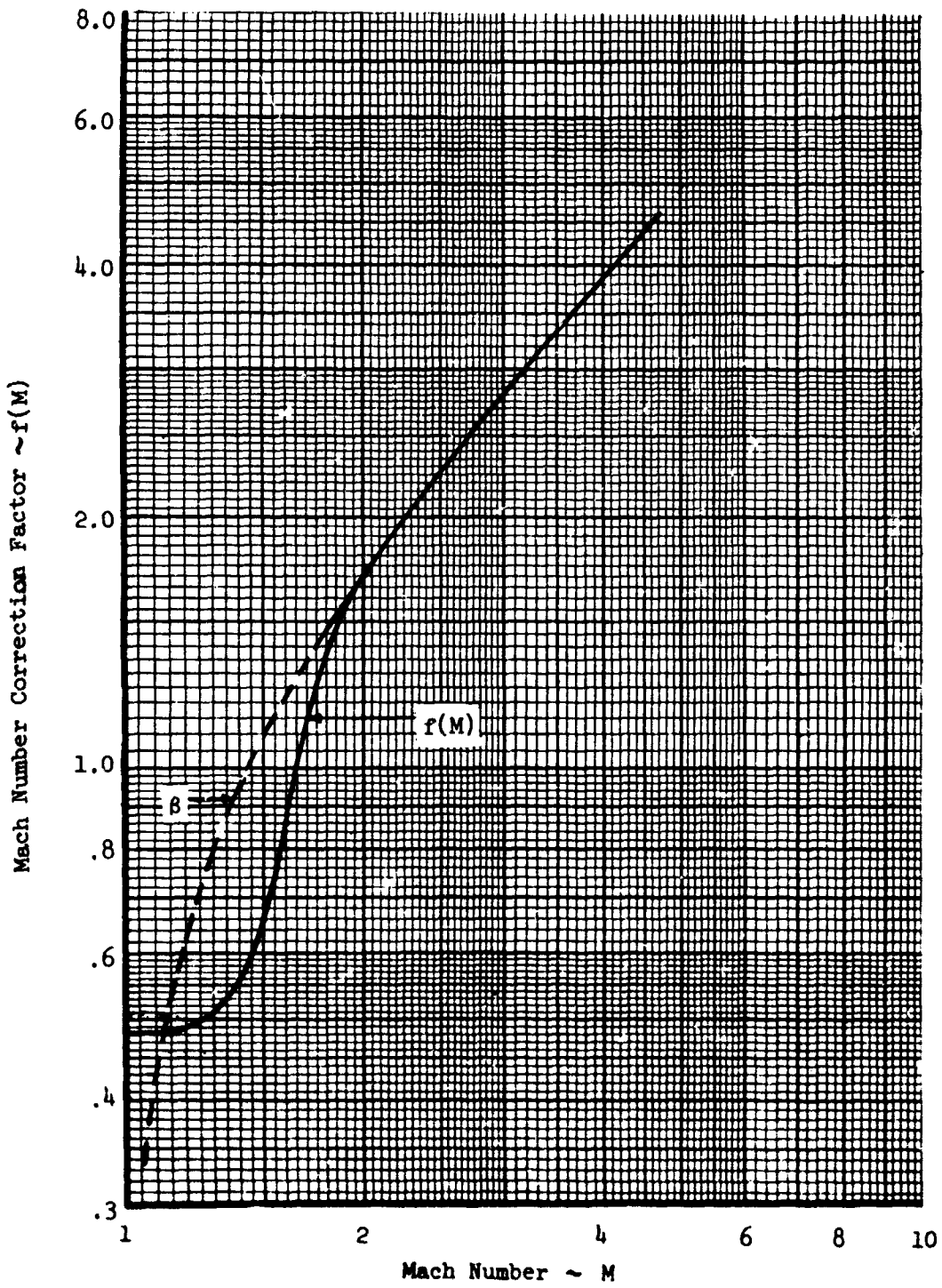
Figure 1 - Mach Number Correction Factor Versus Mach Number
