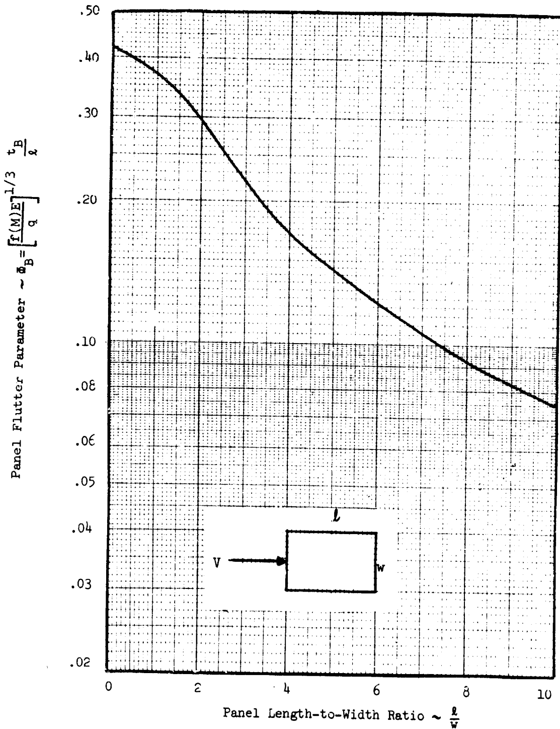
Figure 3 - "Baseline" Design Curve
