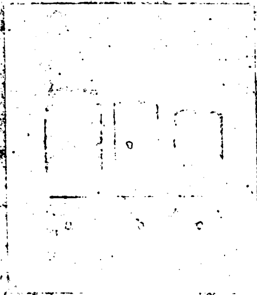
Figure 2. Electrophorograms of milk proteins from mastitis milk (a) and of proteins that went over into the fatty layer in the California test (b,c).
