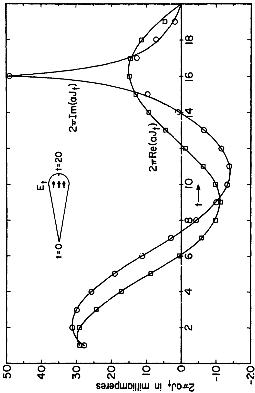
Figure 6. Current density on a conducting cone-sphere excited by one volt across a slot at the cone-to-sphere junction.
