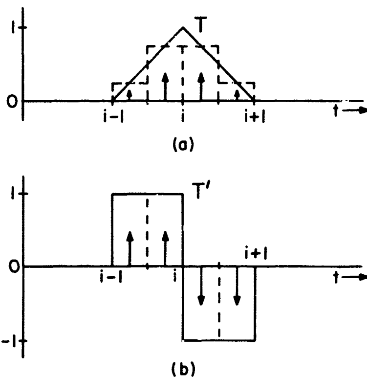
Figure 2. (a) Triangle function (solid), four-pulse approximation (dashed), impulse approximation (arrows). (b) Derivative of triangle function (solid), four-pulse representation (dashed), impulse approximation (arrows).
