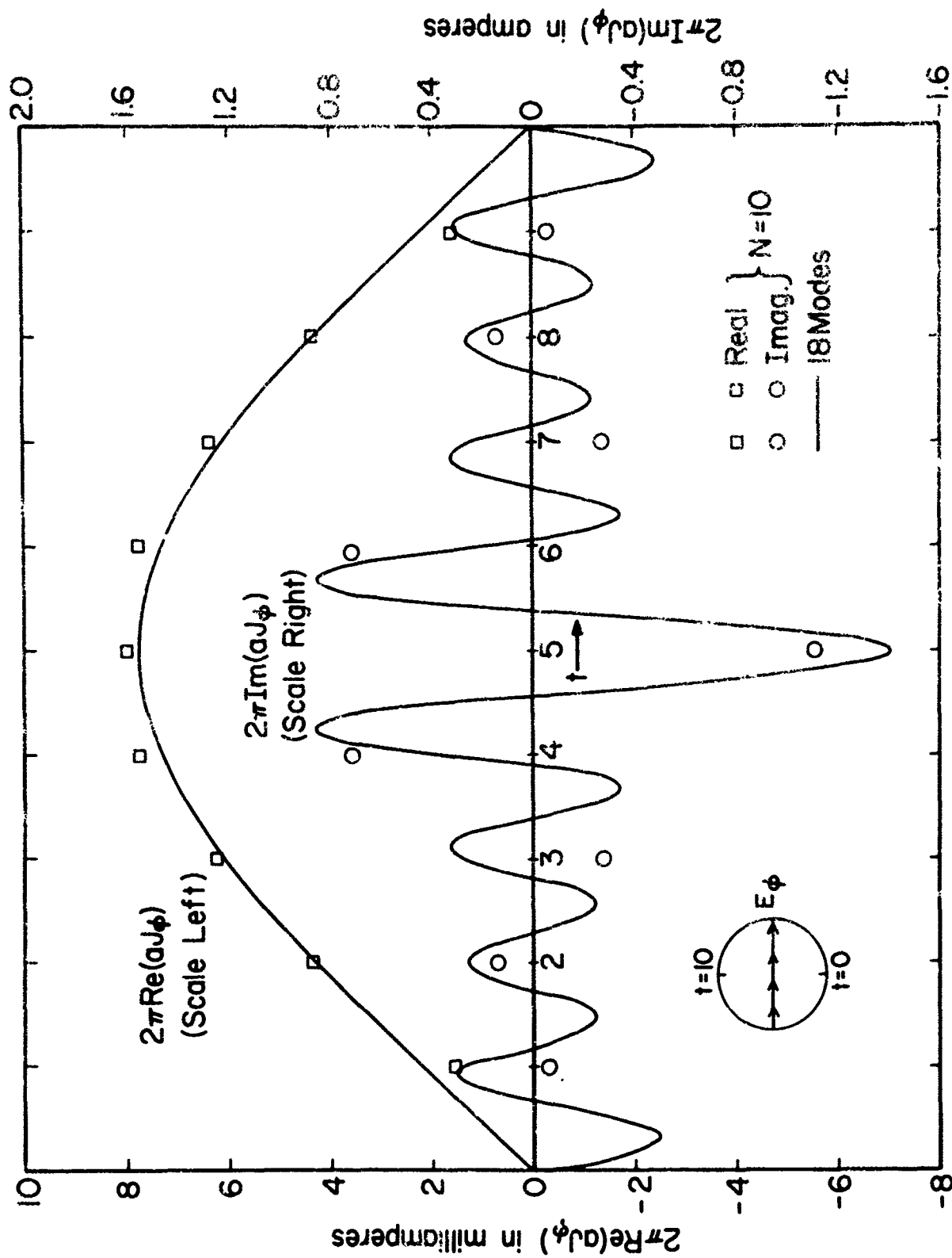
Figure 5. Current density on a conducting sphere of radius 0.1, excited by an impulsive E_\phi in an equatorial slot.
