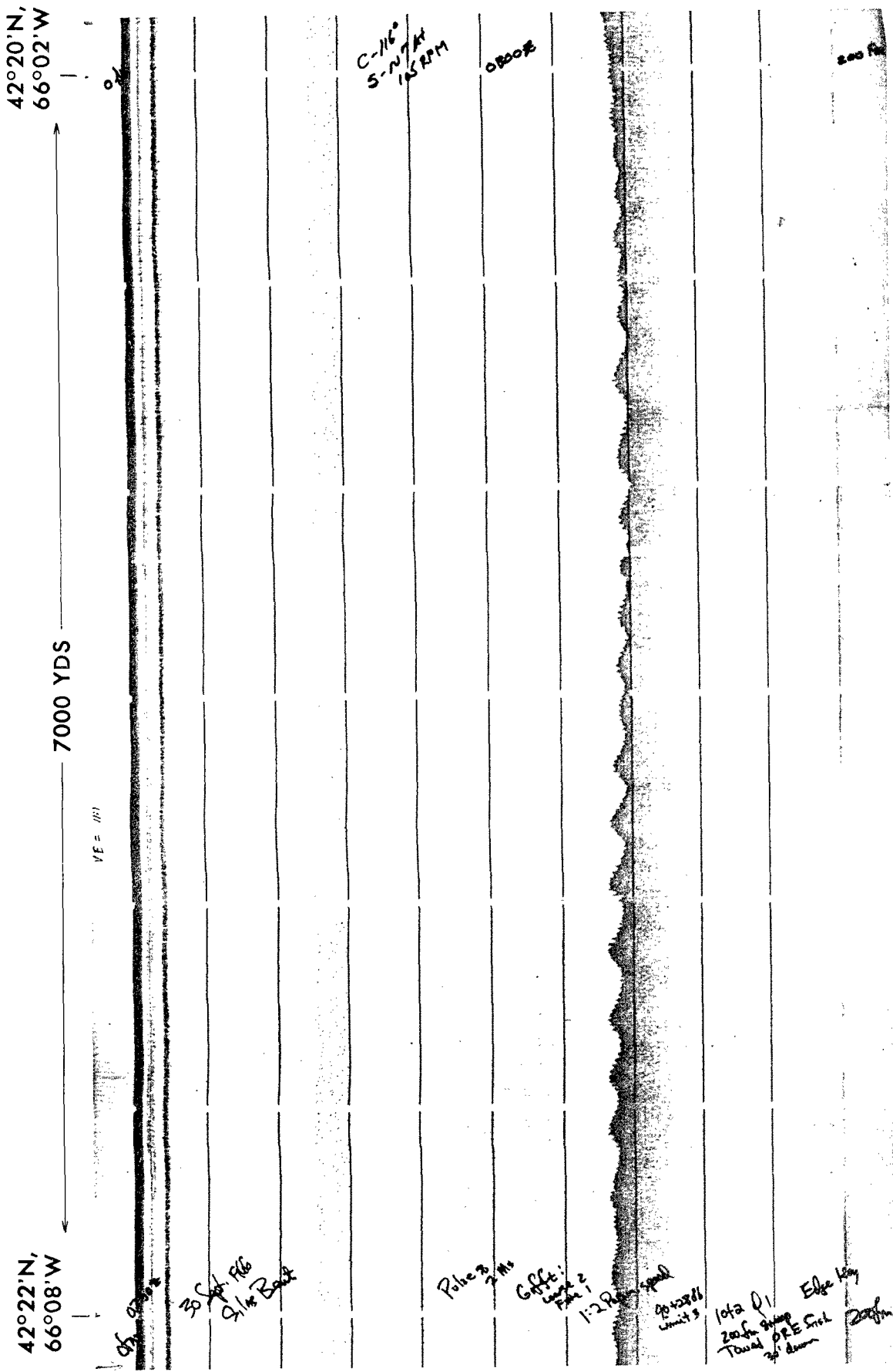
FIGURE 11 SAND WAVES — EASTERN CHANNEL, GULF OF MAINE
