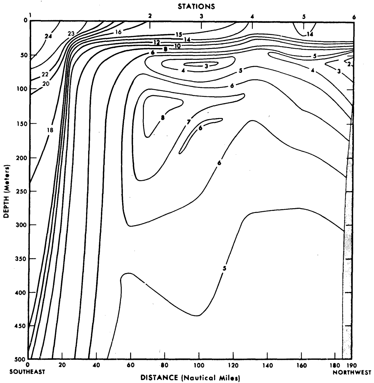
FIGURE 9 TEMPERATURE CROSS-SECTION, UPPER 500 METERS — SOHM ABYSSAL PLAIN TO BROWN'S BANK
