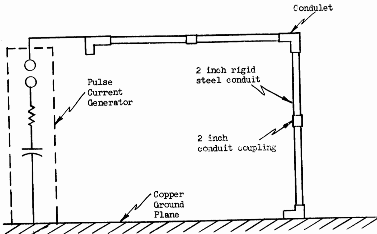
a. Test setup for four lengths of 2 inch conduit
