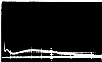
FIGURE 9 Wave Shapes of Conductor-to-Conduit Induced Voltages Showing Effect of Conduit Saturation. Applied Pulse Current - 1755 amperes
