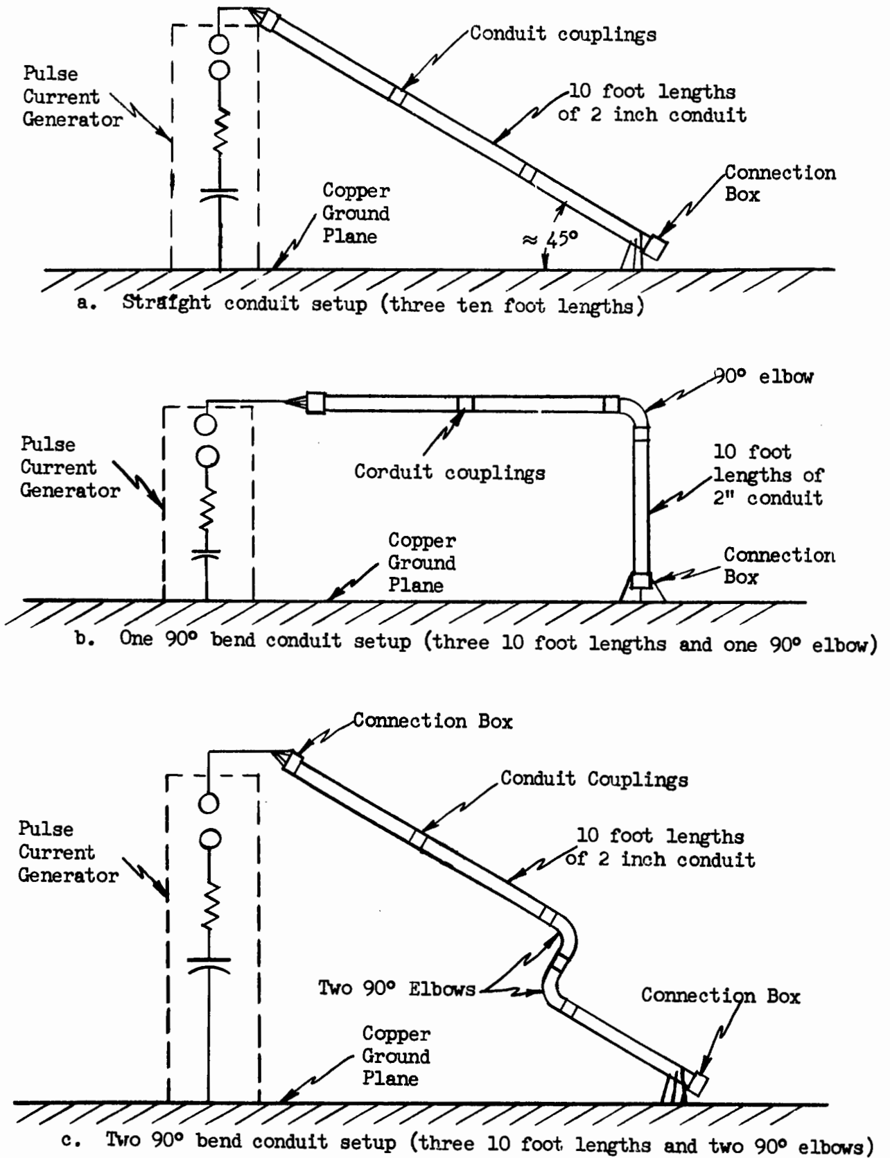
FIGURE 3 Various Conduit Test Configurations
