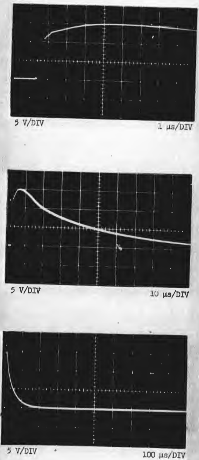
FIGURE 32 Phase Conductor-to-Shield Induced Voltage (1 - 5) - Test Condition 2. Applied Pulse Current - 1420 Amperes
