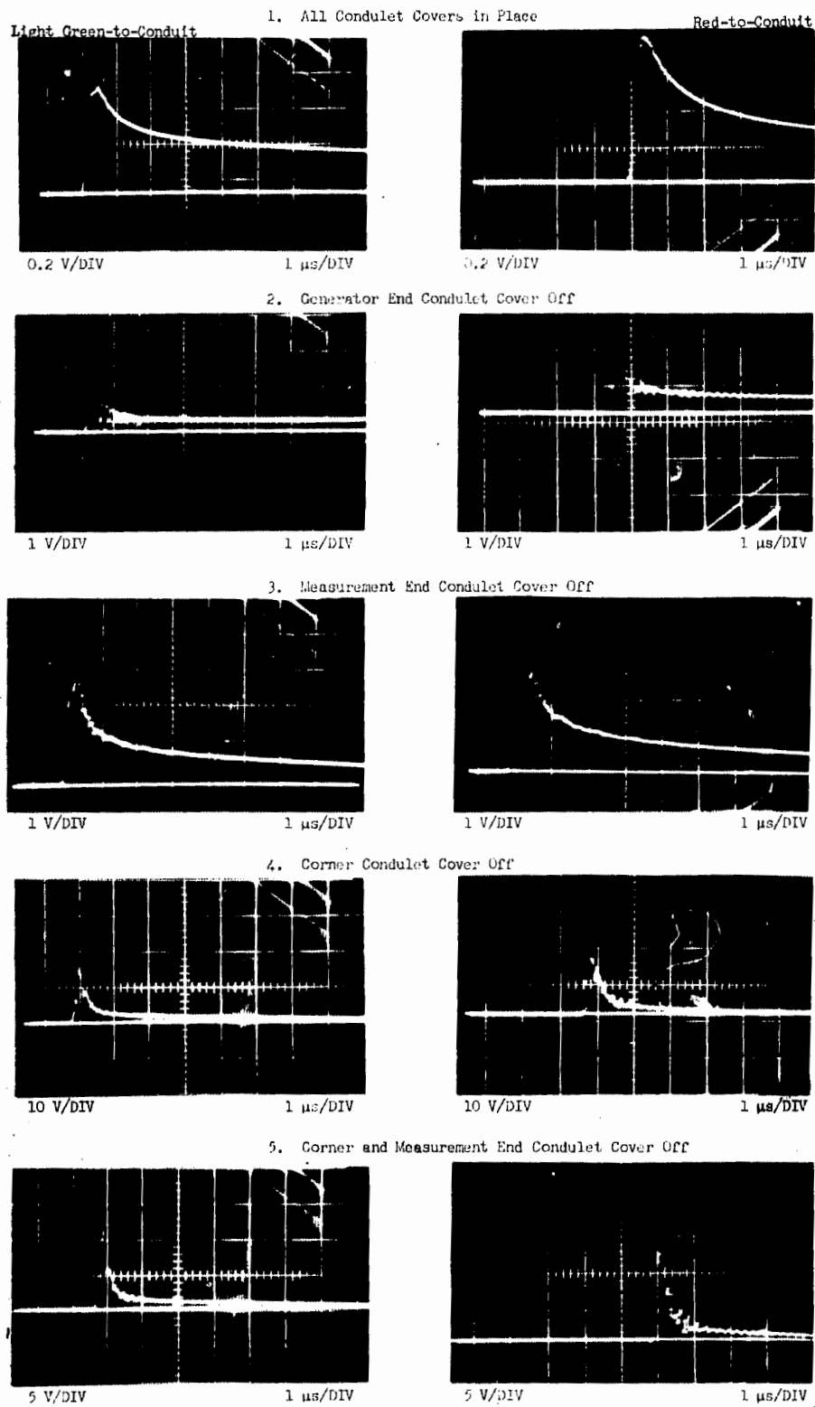
FIGURE 13 Wave Shape of Induced Conductor-to-Conduit Voltage Showing Effect of Openings in the Conduit System. Applied Pulse Current - 1750 amperes
