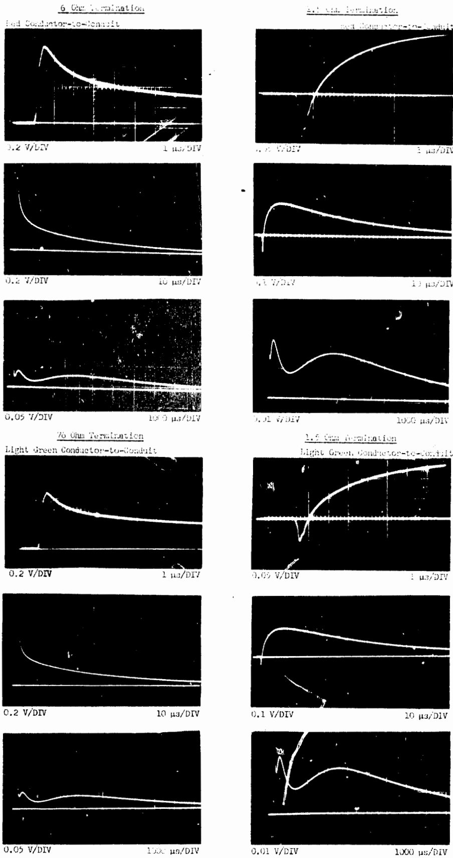
FIGURE 10 Wave Shapes of Conductor-to-Conduit Induced Voltages Showing Effects of Terminating Impedance. Applied Pulse Current - 1700 amperes
