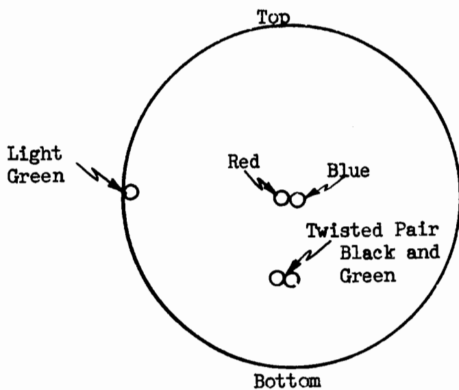
b. Conductor arrangement within the conduit cross section
