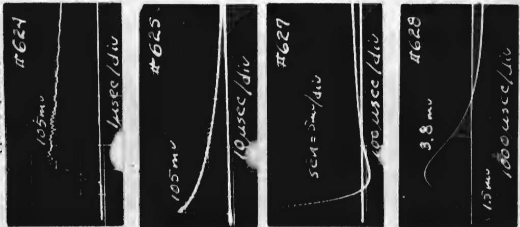
FIGURE 44 Comparison of Conductor-to-Conduit Induced Voltages in Bottom Half of Conduit Loop with Induced Current Flowing in the Conduit Loop
