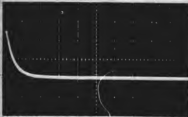
FIGURE 28 Neutral Wires-to-Armor Induced Voltage (4-8) - Test Condition 1 Applied Pulse Current - 1420 Amperes
