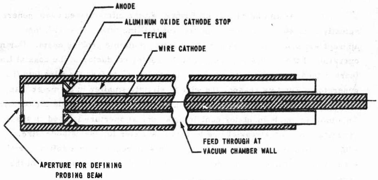
Figure 18 MINIATURIZED ATOMIC-BEAM GENERATOR
