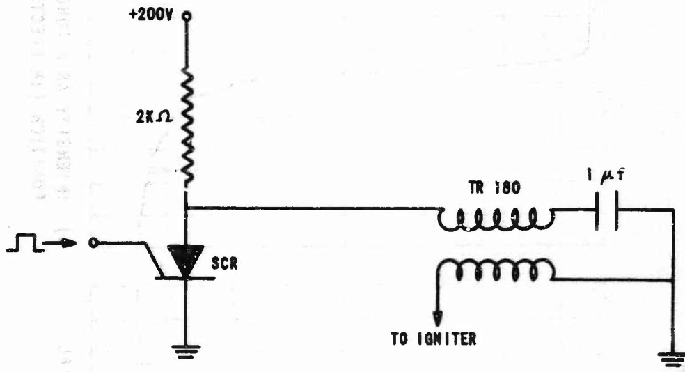
Figure 10 IGNITER CIRCUIT
