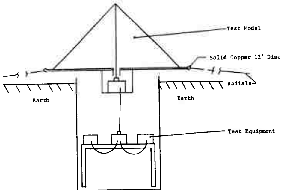
Figure 24. Test Facility
