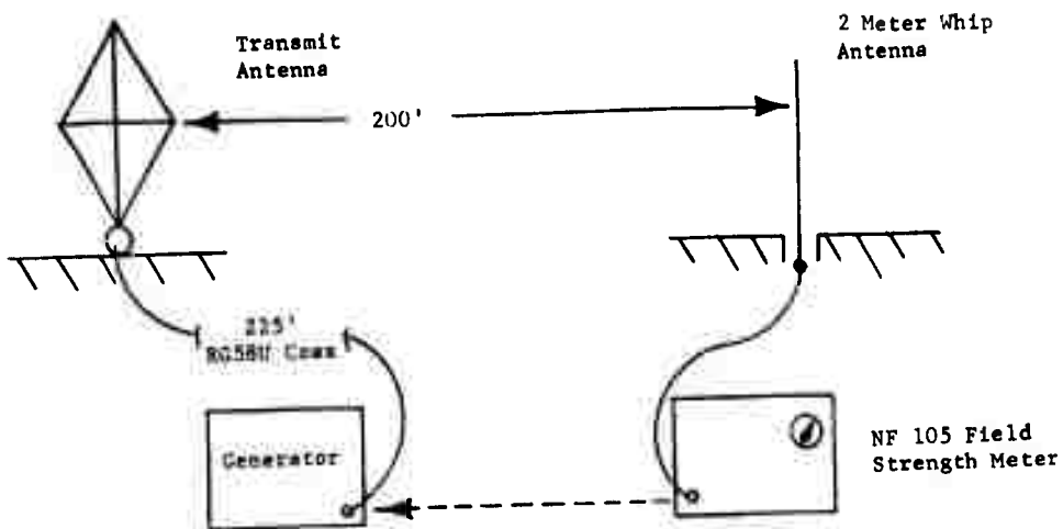
Figure 28. Standard Whip Voltage Measurement
