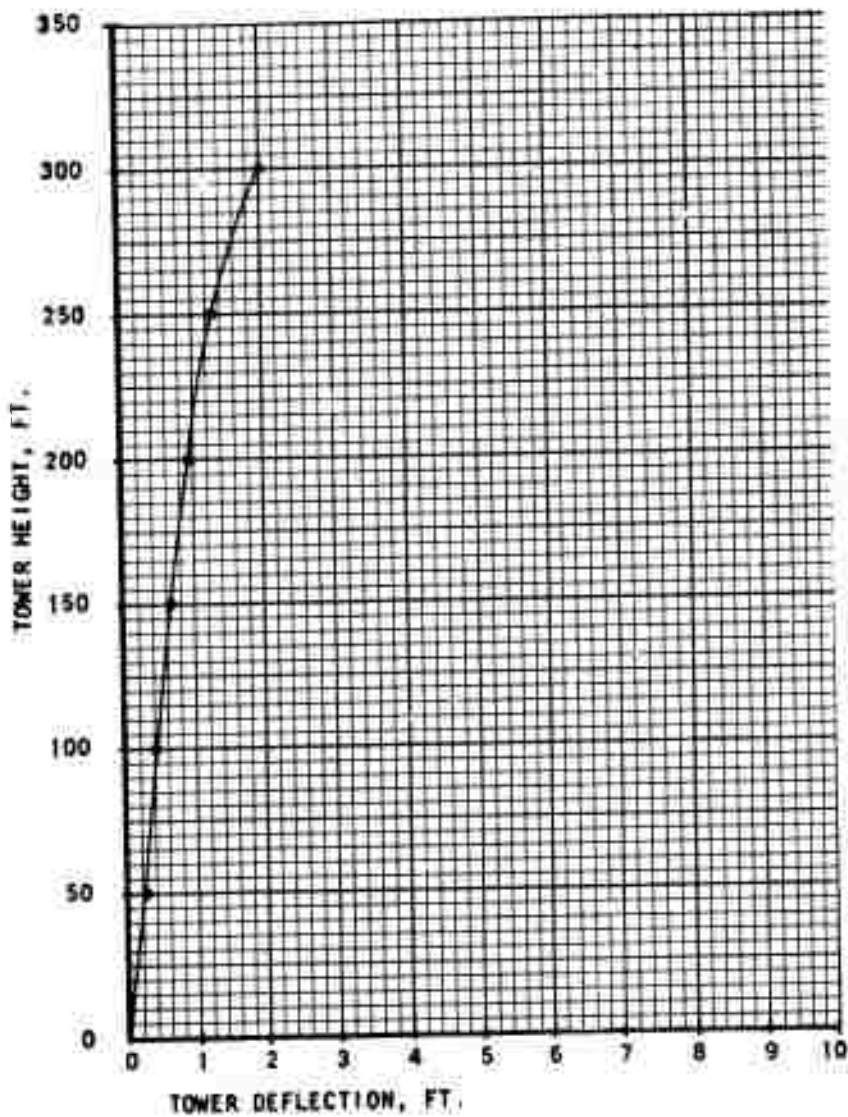
Figure 57. Computer Run #18
