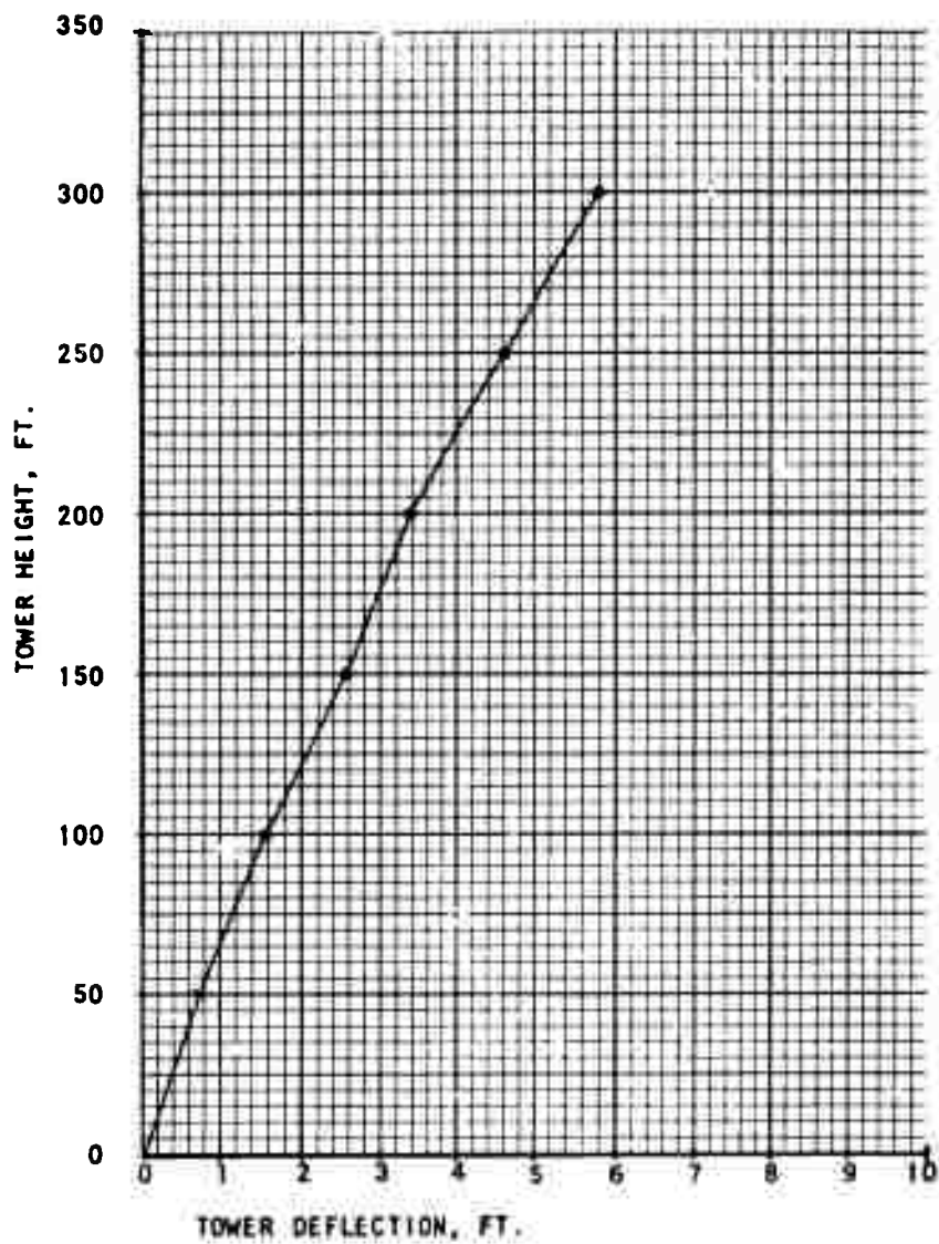
Figure 62. Computer Run #23
