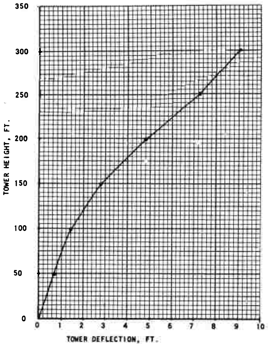
Figure 41. Computer Run #2
