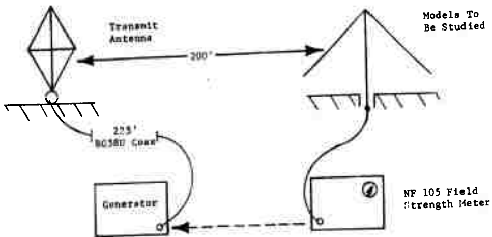
Figure 29. Model Antenna Voltage Measurement
