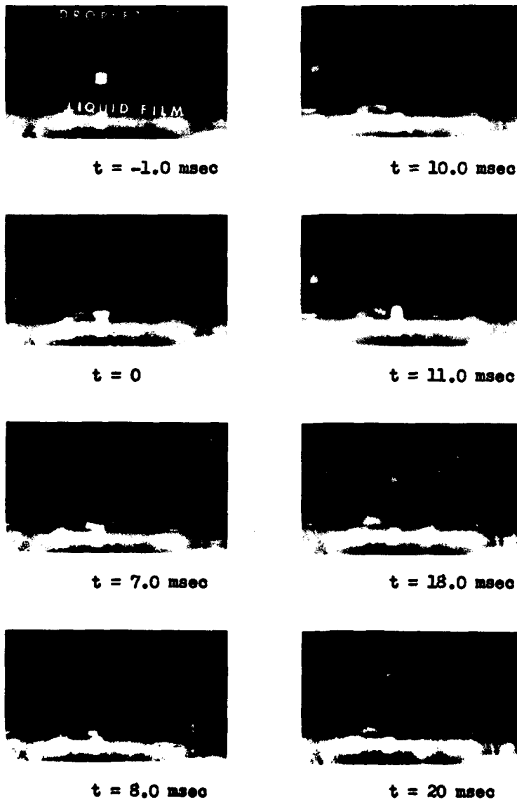
Fig 7 Droplet Bounce-Splash Characteristic: d = 325 \mu , V_d = 4.6 \text{ ft/sec} , m_v = 5.8 \times 10^{-9} \text{ lb}_f\text{-sec}
