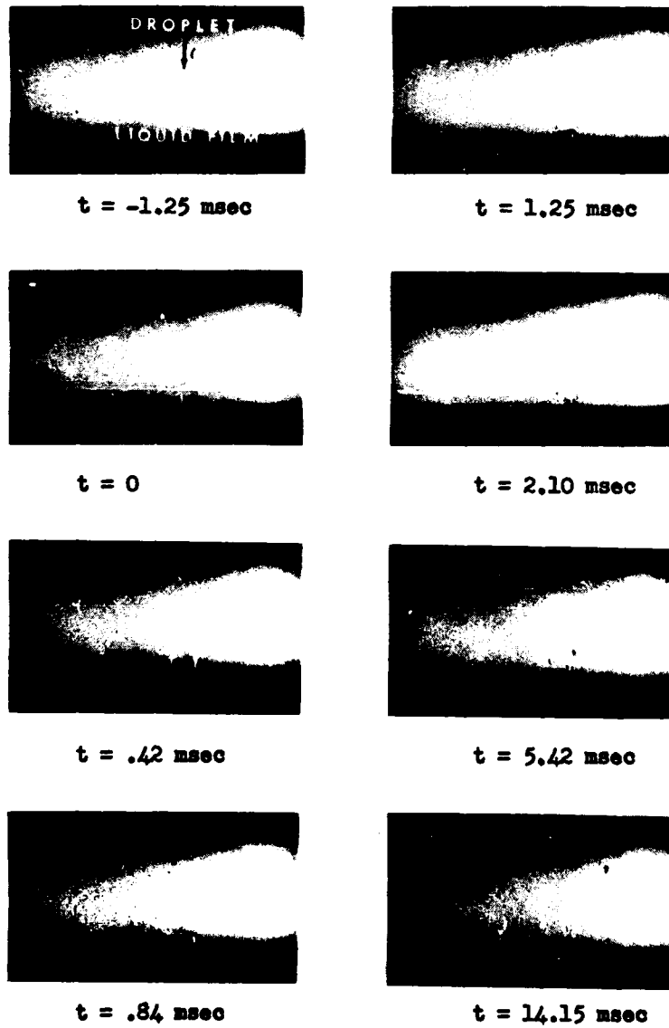
Fig 8 Droplet Splash Characteristic: d = 350 \mu , V_d = 38.4 ft/sec, m_v = 61.0 \times 10^{-9} lb f -sec
