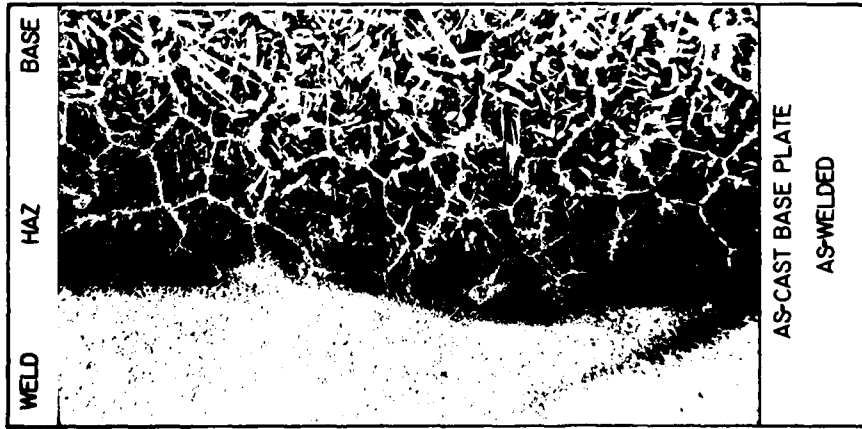
FIG. 14 PHOTOMICROGRAPHS OF WELD-BASE INTERFACE OF CLASS 4 BASE PLATE AND CODE 4 FILLER WIRE WELDMENTS AFTER SEA WATER EXPOSURE (50X)
