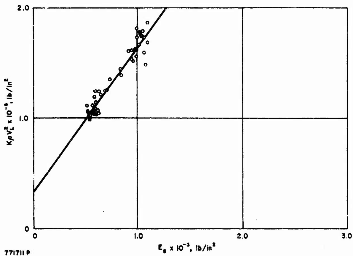
Figure 11-5. RELATIONSHIP OF K\rho v_L^2 AND E_s FOR ATJ GRADE GRAPHITE
