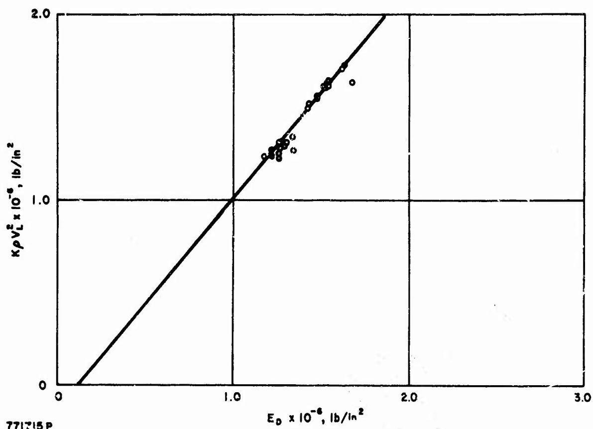
Figure 11-9. RELATIONSHIP OF K_p V_L^2 AND E_0 FOR RVA GRADE GRAPHITE
