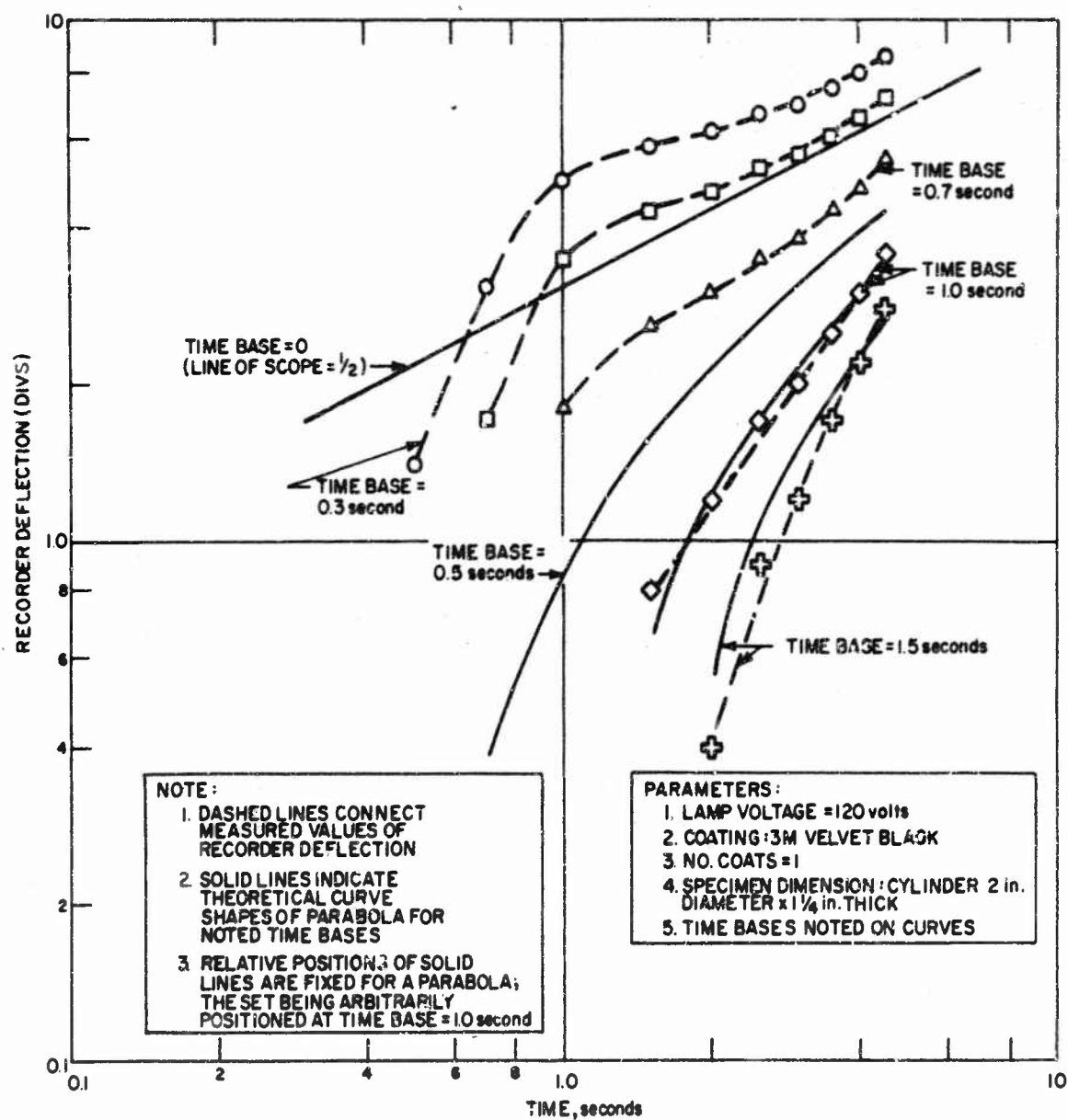
Figure 10. SURFACE TEMPERATURE HISTORIES FOR A/J GRAPHITE (FOR SEVERAL TIME BASES)
