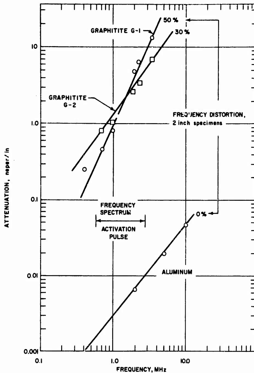
Figure 38. SPECIMEN ATTENUATION CHARACTERISTICS AND THE RESULTING FREQUENCY DISTORTION FOR PATH LENGTH OF 2 INCHES
