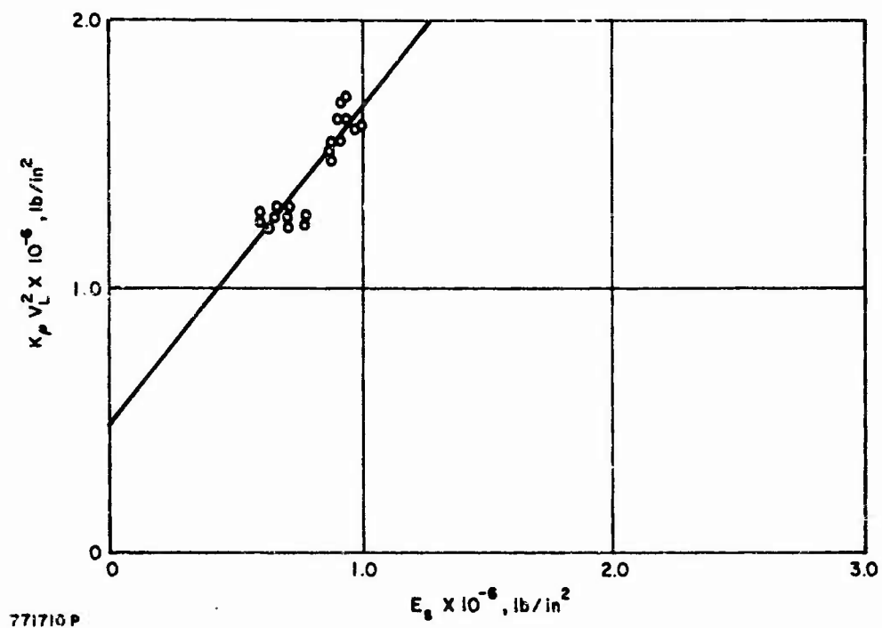
Figure 11-4. RELATIONSHIP OF K_p V_L^2 AND E_s FOR RVA GRADE GRAPHITE
