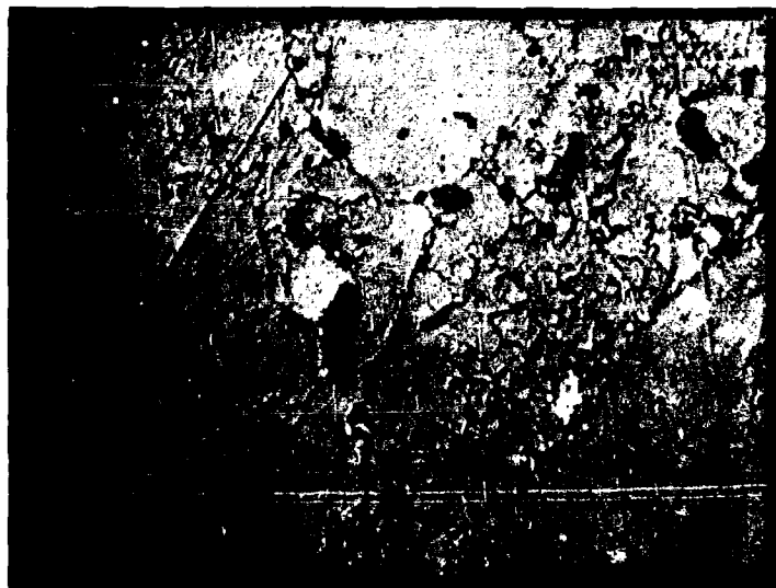
FIGURE 14. Microstructure of Hot-Pressed Chemically Pure Strontium Zirconate (1600X)
