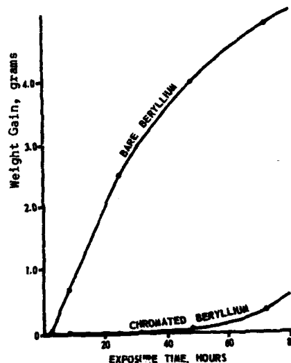
FIGURE 2. OXIDATION OF BARE AND CHROMATED BERYLLIUM IN MOIST AIR AT 900 C (1652 F) (8)
