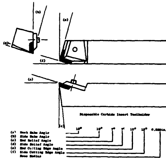
FIGURE 1. BERYLLIUM TURNING TOOL--HIGH RAKE GEOMETRY. (2)
