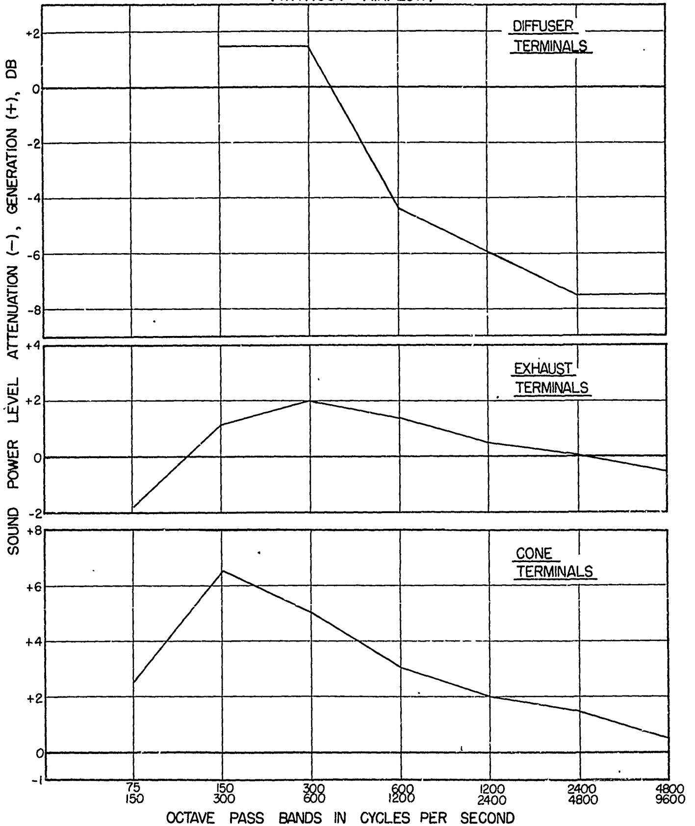
FIGURE 6 SOUND POWER LEVEL ATTENUATION OR GENERATION CHARACTERISTICS OF NAVY STANDARD DIFFUSER, EXHAUST AND CONE TYPE TERMINALS (WITHOUT AIRFLOW)
