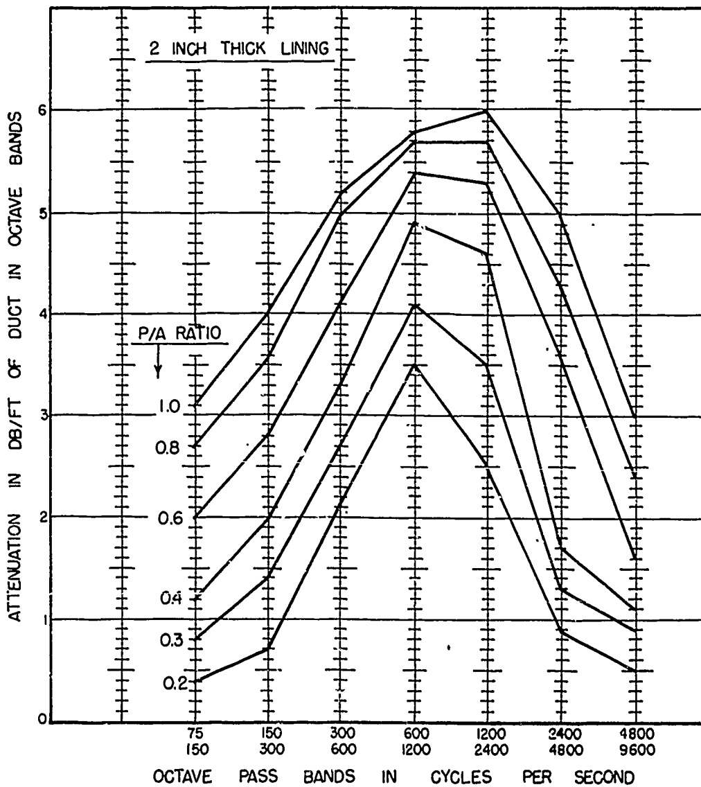
FIGURE II SOUND POWER LEVEL ATTENUATION IN OCTAVE BANDS IN STRAIGHT DUCTS LINED ON FOUR SIDES WITH 2" THICK NAVY STANDARD FIBERGLASS AND PERFORATED ALUMINUM, NO AIRFLOW
