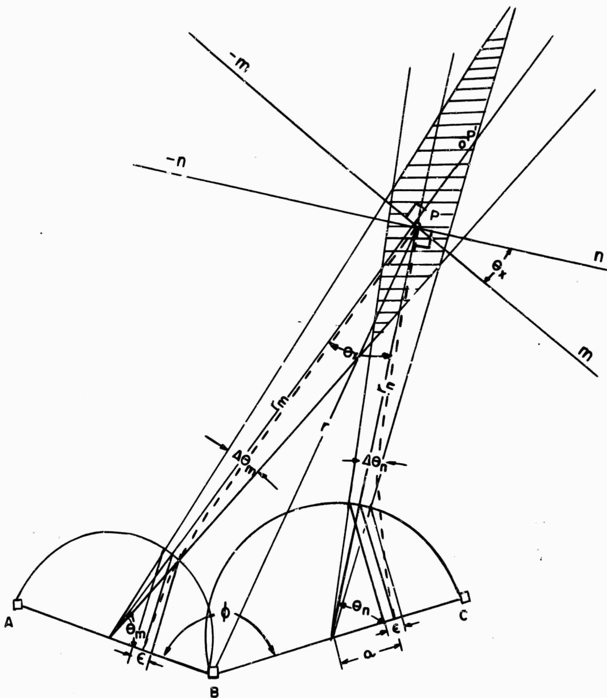
Figure 2. Basic Error Geometry (Three Observers)
